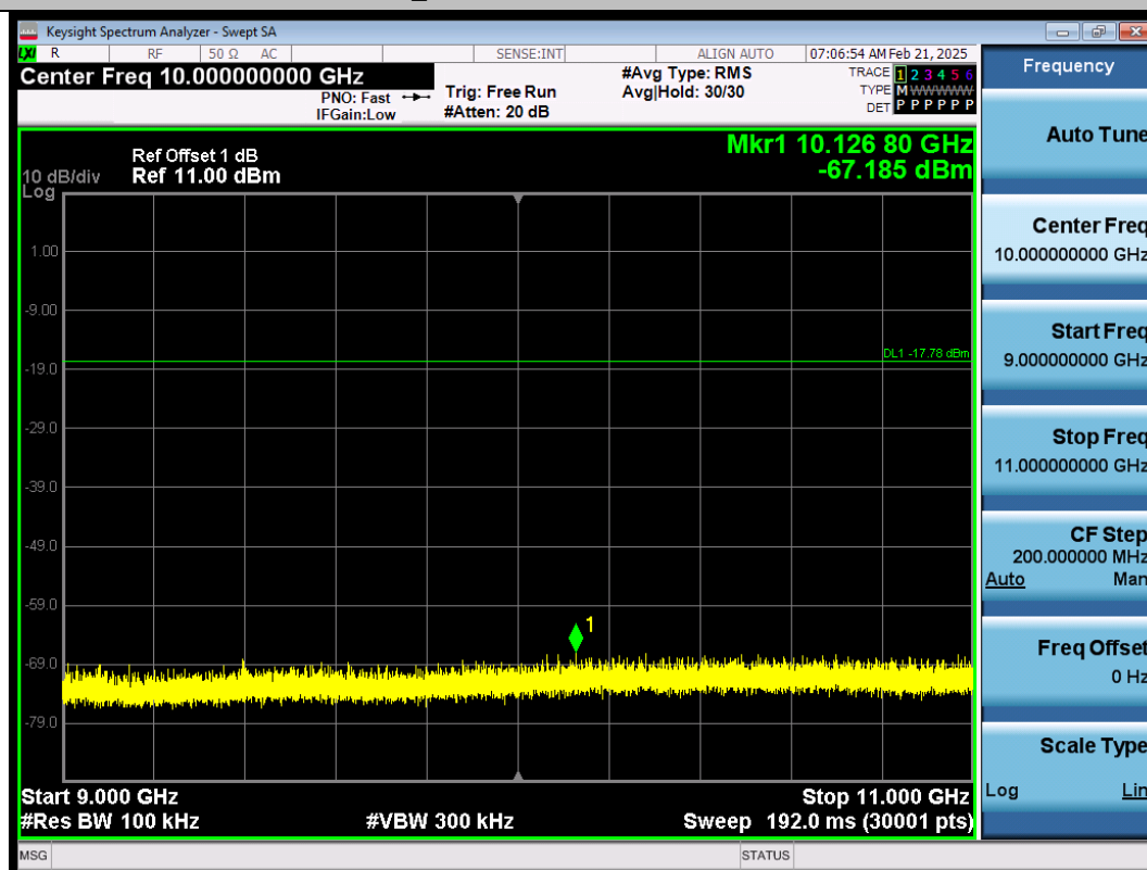
BLE_1M-Ant1-2480-9000~11000-PASS
