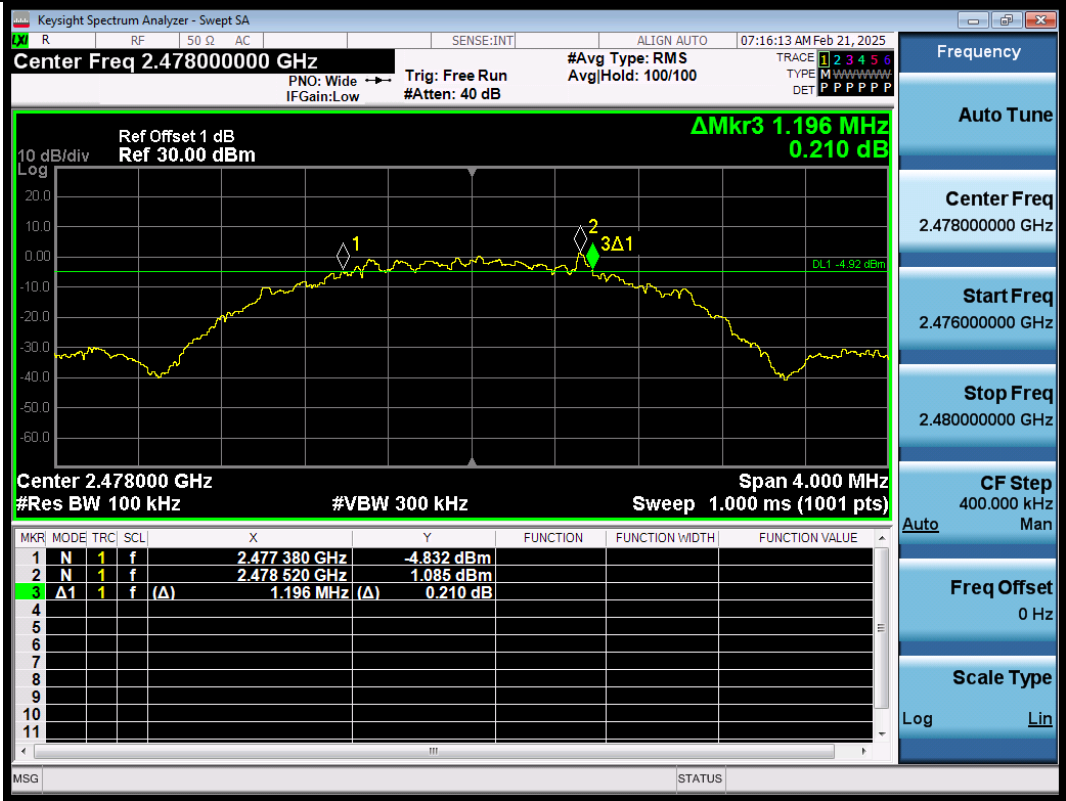
BLE_2M-Ant1-2478-PASS
