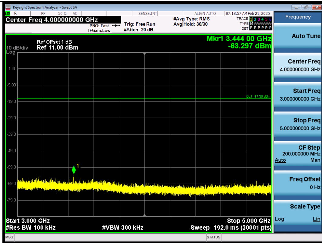
BLE_2M-Ant1-2440-3000~5000-PASS
