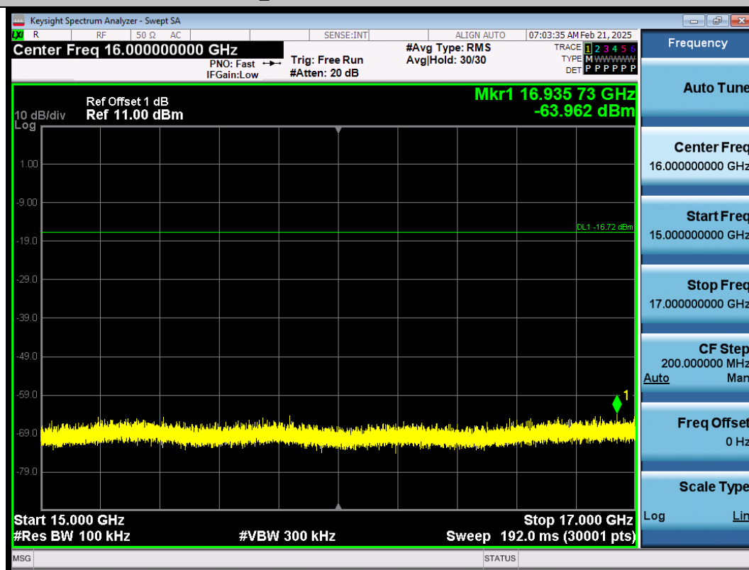
BLE_1M-Ant1-2440-15000~17000-PASS
