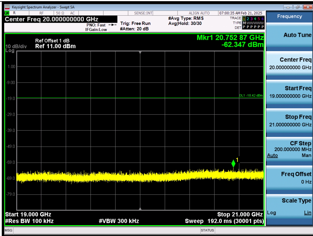
BLE_1M-Ant1-2402-19000~21000-PASS
