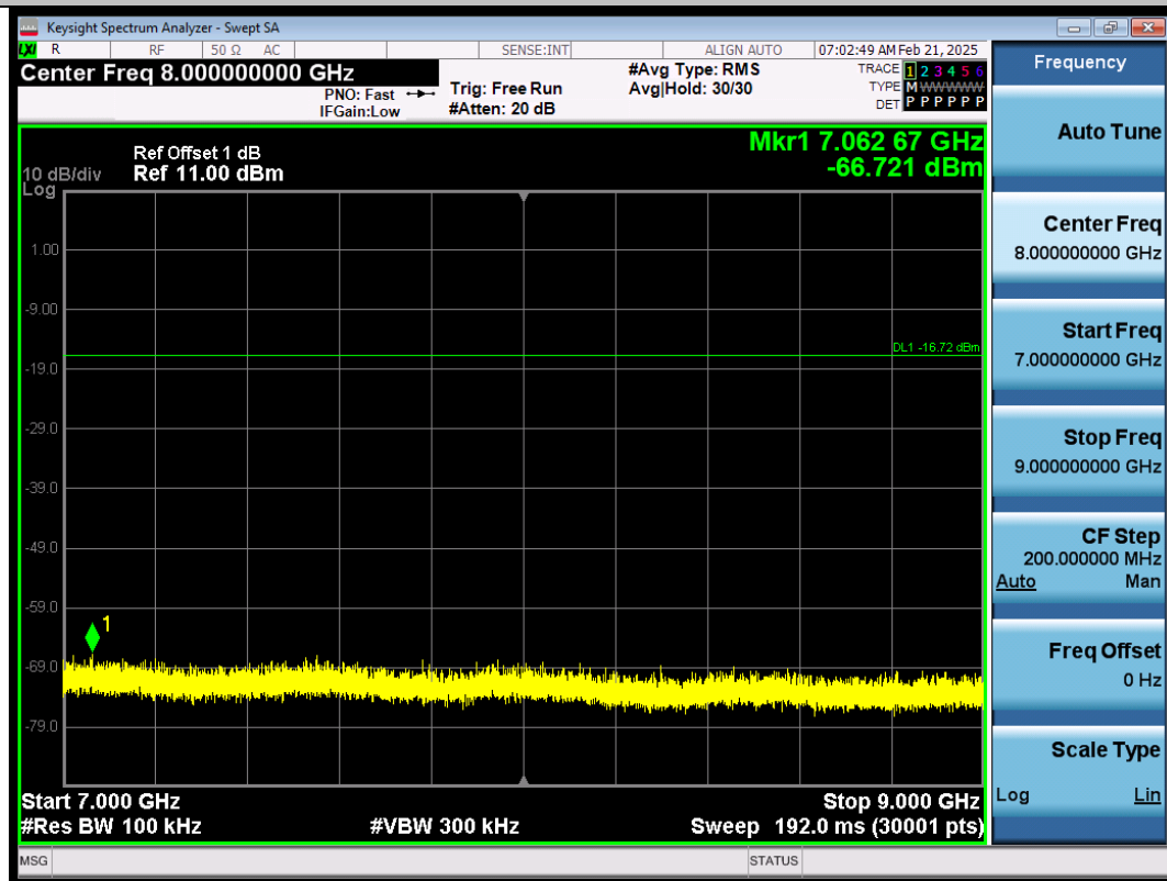
BLE_1M-Ant1-2440-7000~9000-PASS
