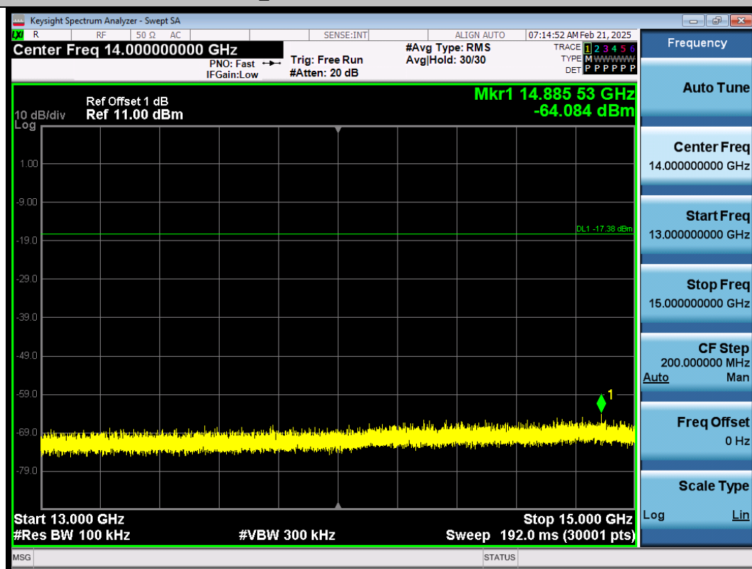
BLE_2M-Ant1-2440-13000~15000-PASS
