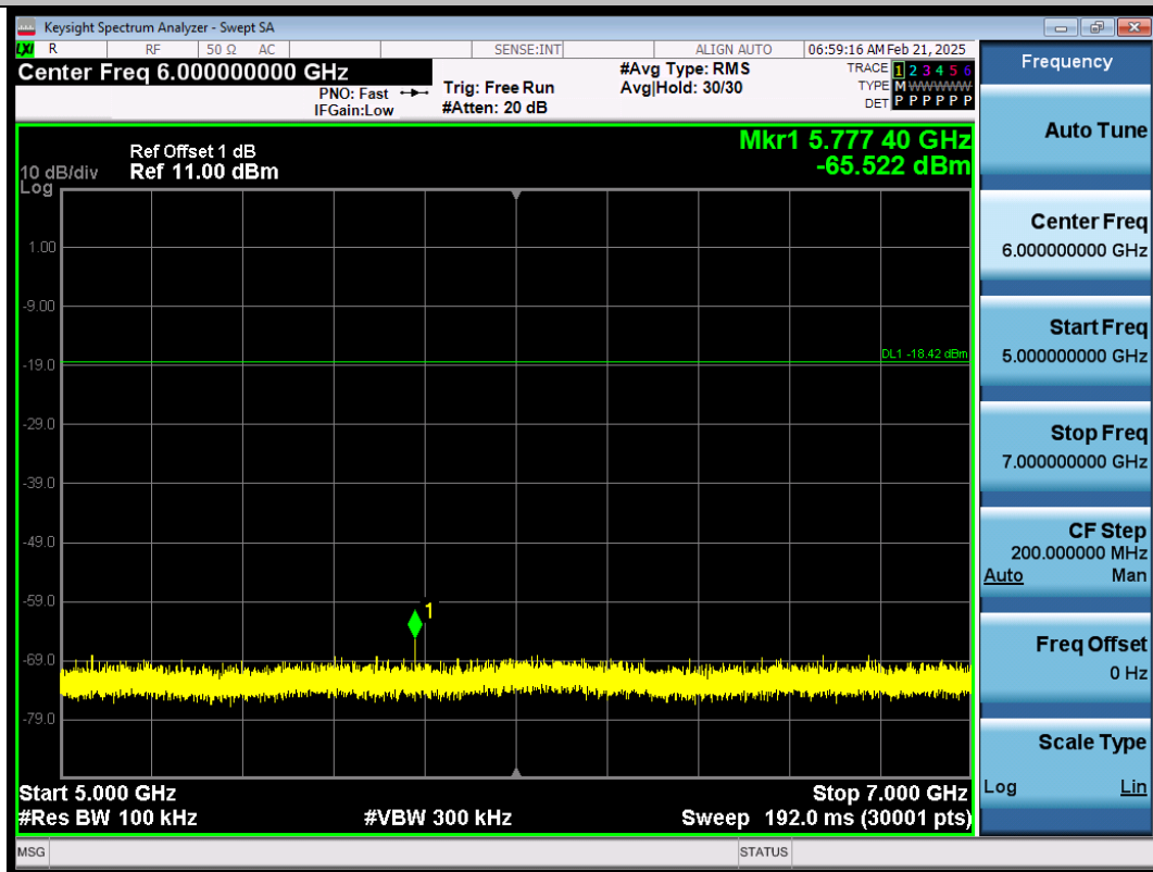
BLE_1M-Ant1-2402-5000~7000-PASS
