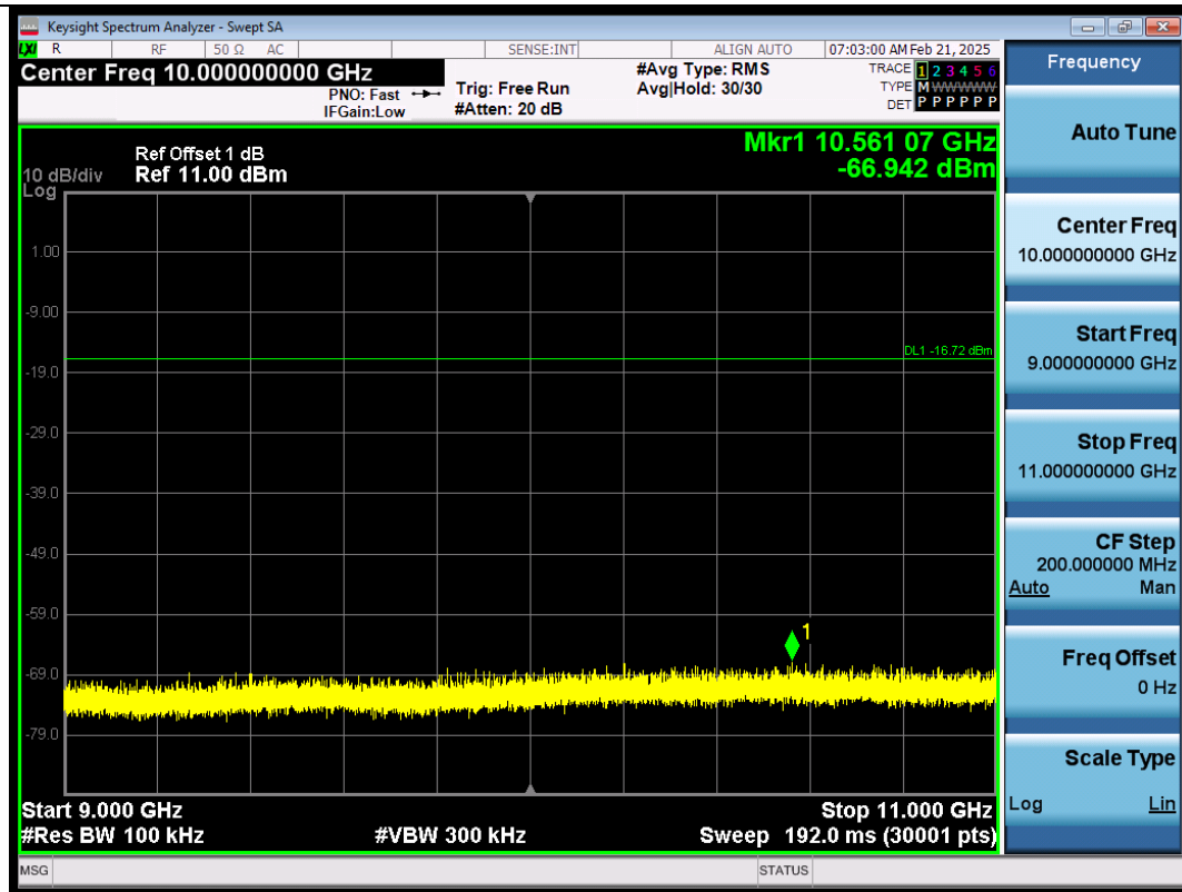
BLE_1M-Ant1-2440-9000~11000-PASS
