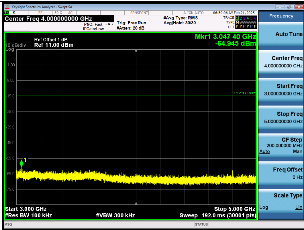
BLE_1M-Ant1-2402-3000~5000-PASS
