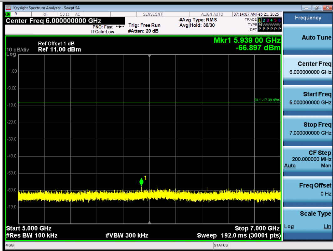
BLE_2M-Ant1-2440-5000~7000-PASS
