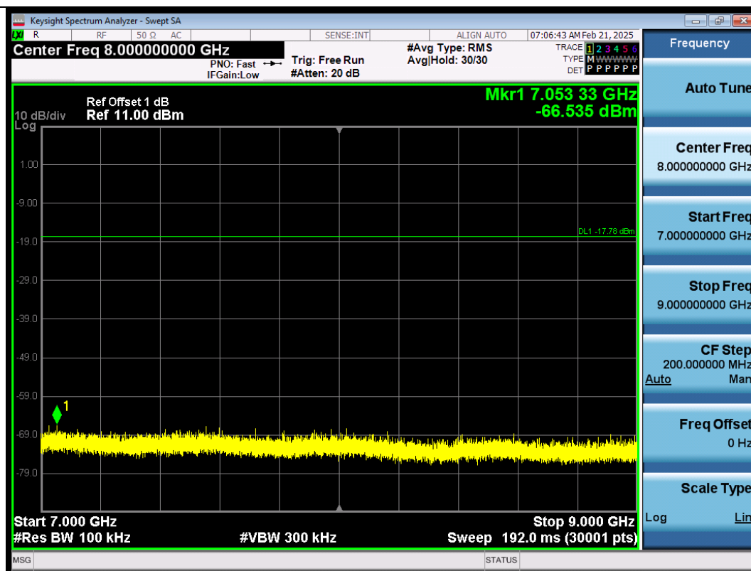
BLE_1M-Ant1-2480-7000~9000-PASS
