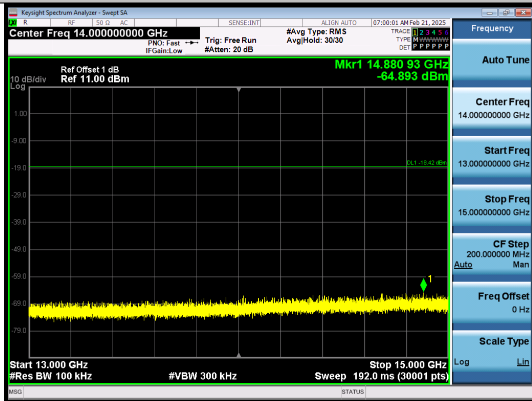
BLE_1M-Ant1-2402-13000~15000-PASS
