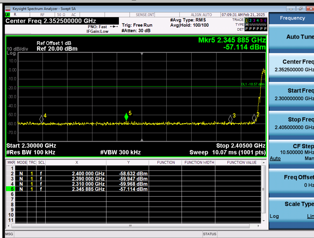
BLE_2M-Ant1-2404-PASS
