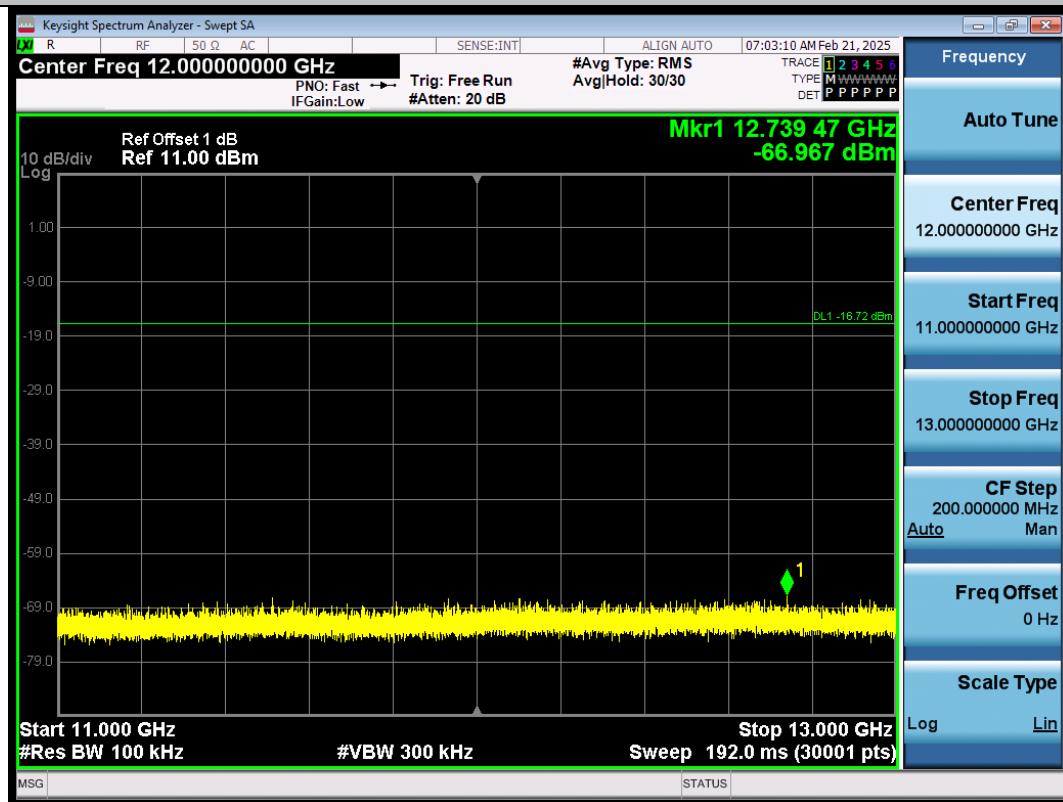
BLE_1M-Ant1-2440-11000~13000-PASS
