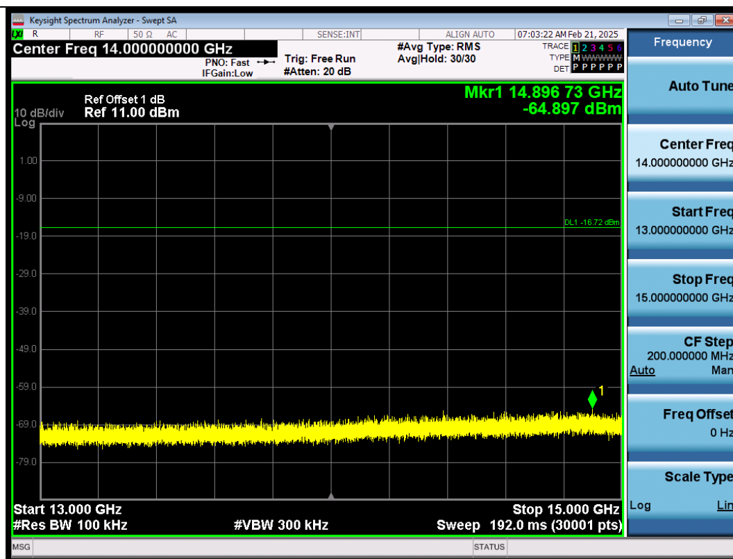
BLE_1M-Ant1-2440-13000~15000-PASS
