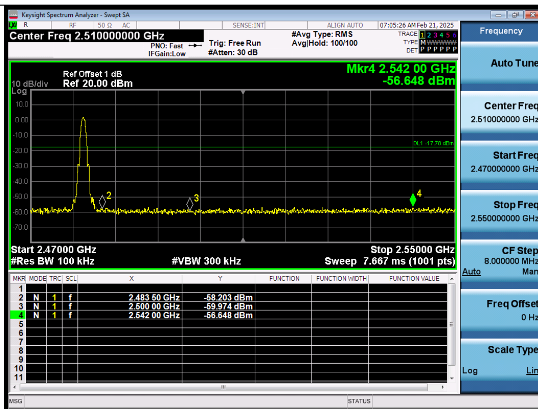
BLE_1M-Ant1-2480-PASS
