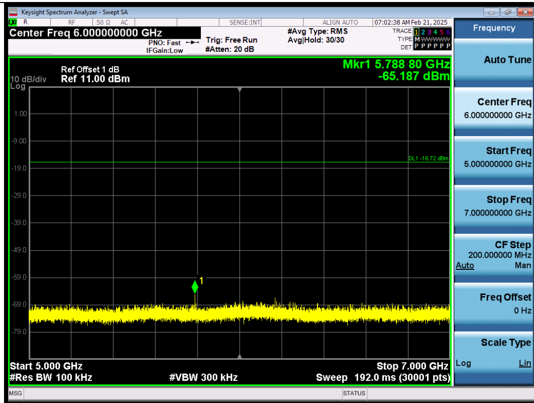
BLE_1M-Ant1-2440-5000~7000-PASS
