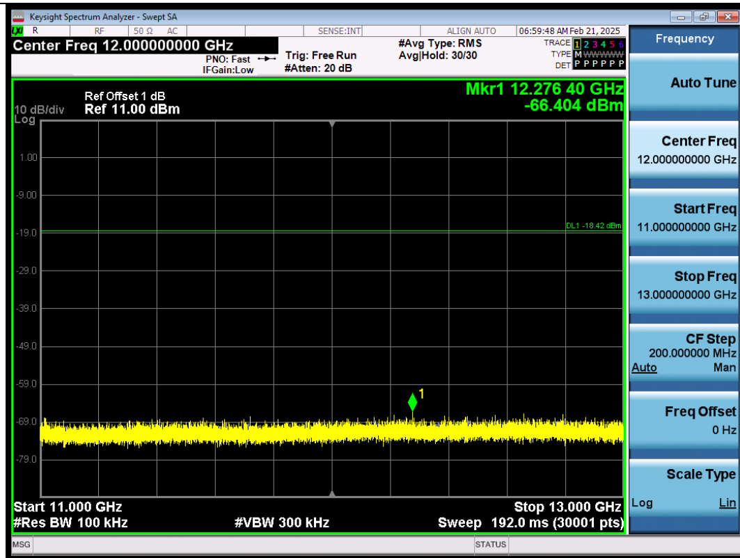
BLE_1M-Ant1-2402-11000~13000-PASS
