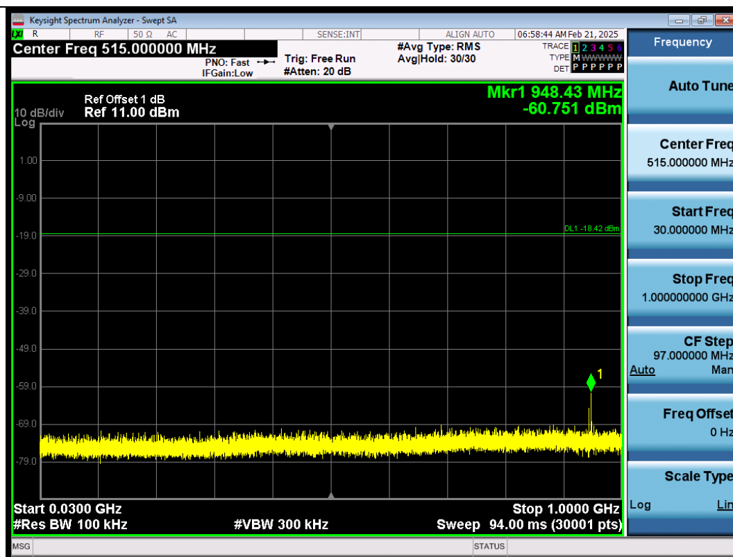
BLE_1M-Ant1-2402-30~1000-PASS
