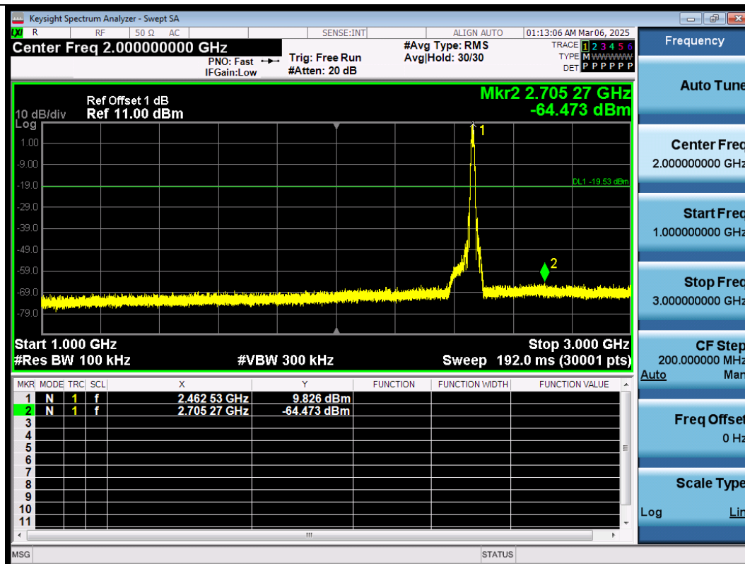
11B-Ant1-2462-1000~3000-PASS
