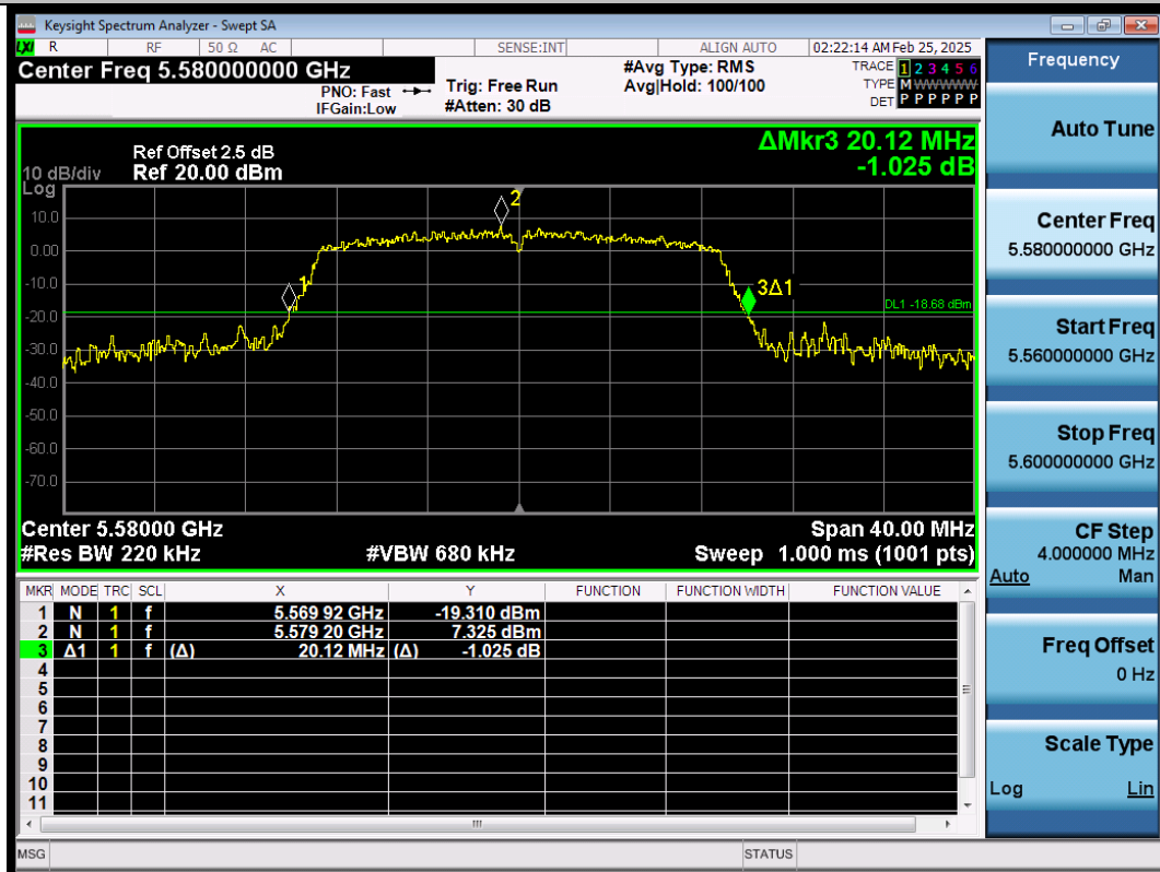
11AC20SISO-Ant1-5580
