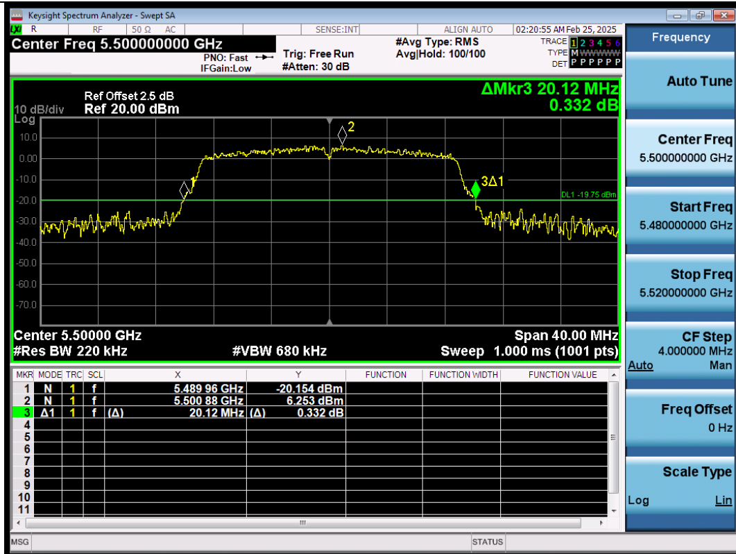
11AC20SISO-Ant1-5500
