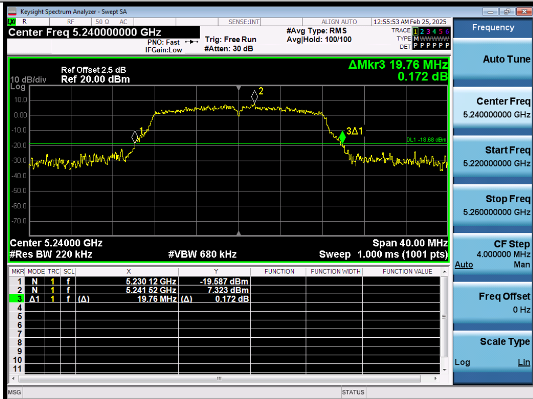
11A-Ant1-5240
