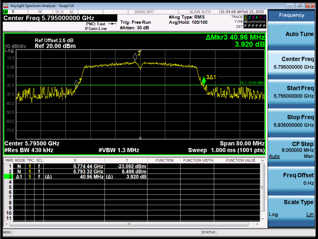
11N40SISO-Ant1-5795
