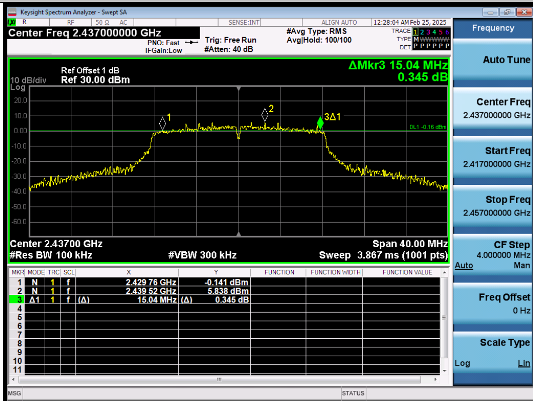
11G-Ant1-2437-PASS
