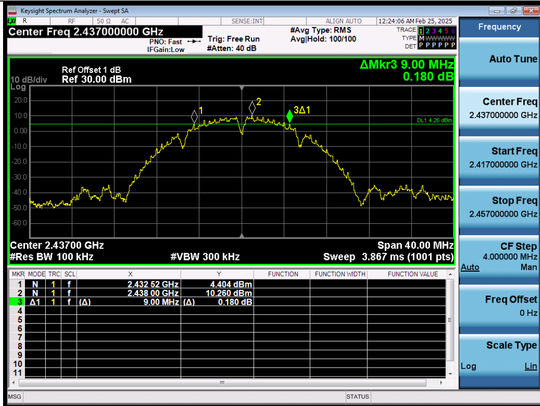
11B-Ant1-2437-PASS
