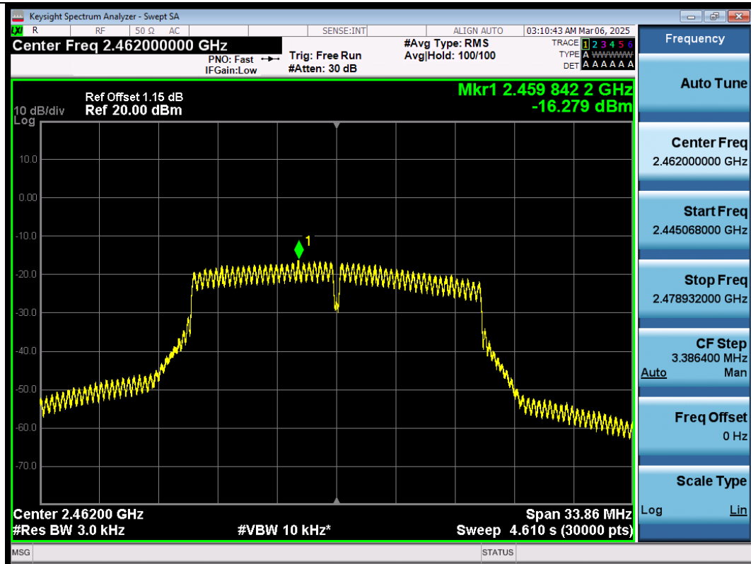
11G-Ant1-2462-PASS
