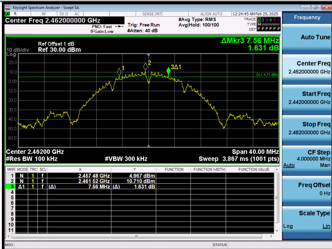
11B-Ant1-2462-PASS
