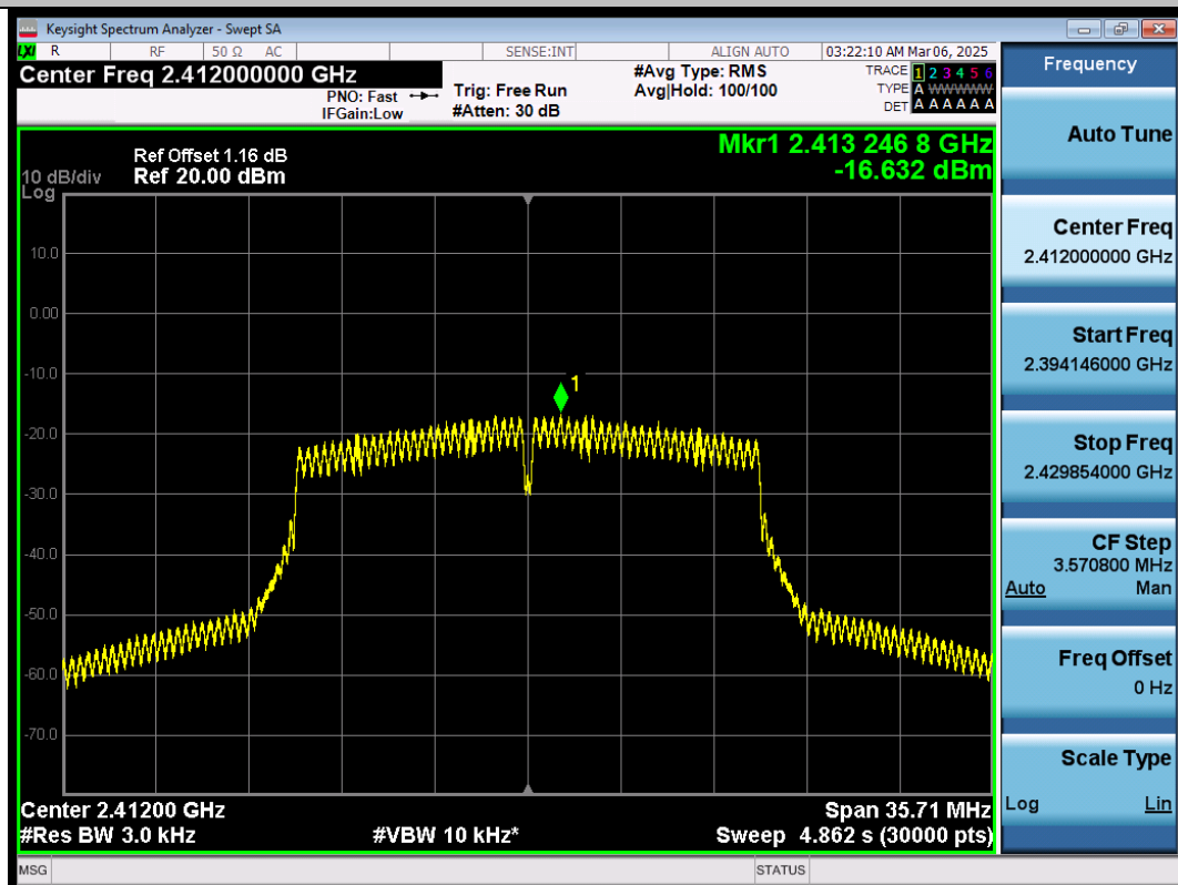
11N20SISO-Ant1-2412-PASS
