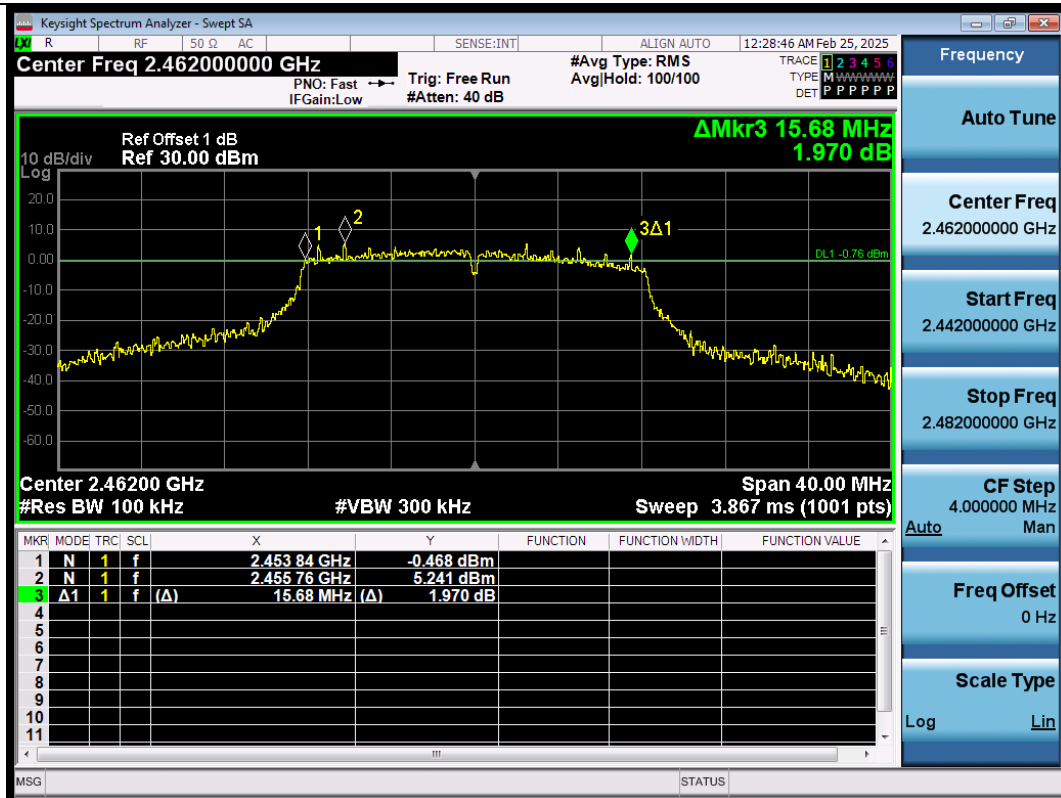
11G-Ant1-2462-PASS
