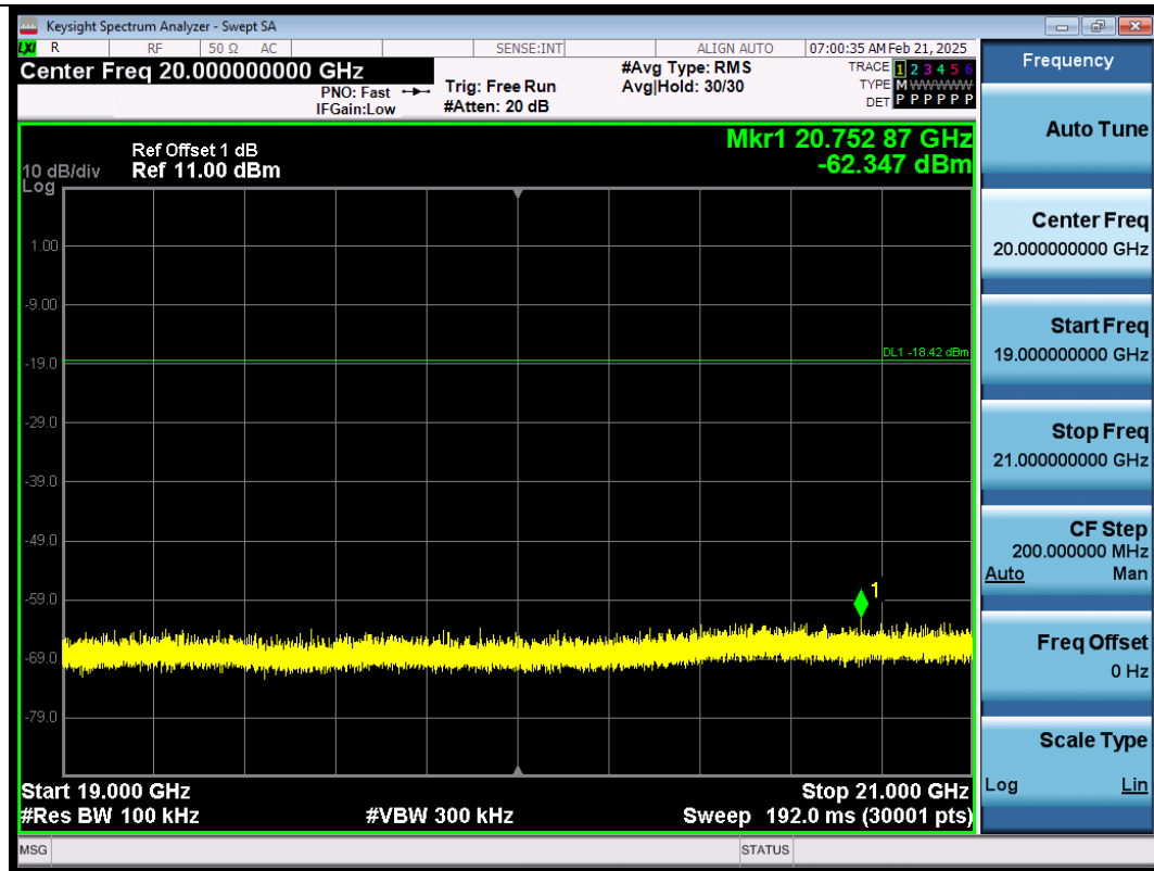
BLE_1M-Ant1-2402-19000~21000-PASS
