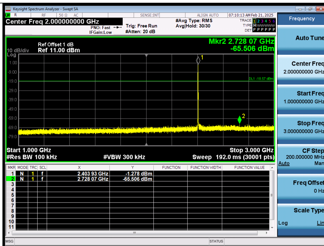
BLE_2M-Ant1-2404-1000~3000-PASS
