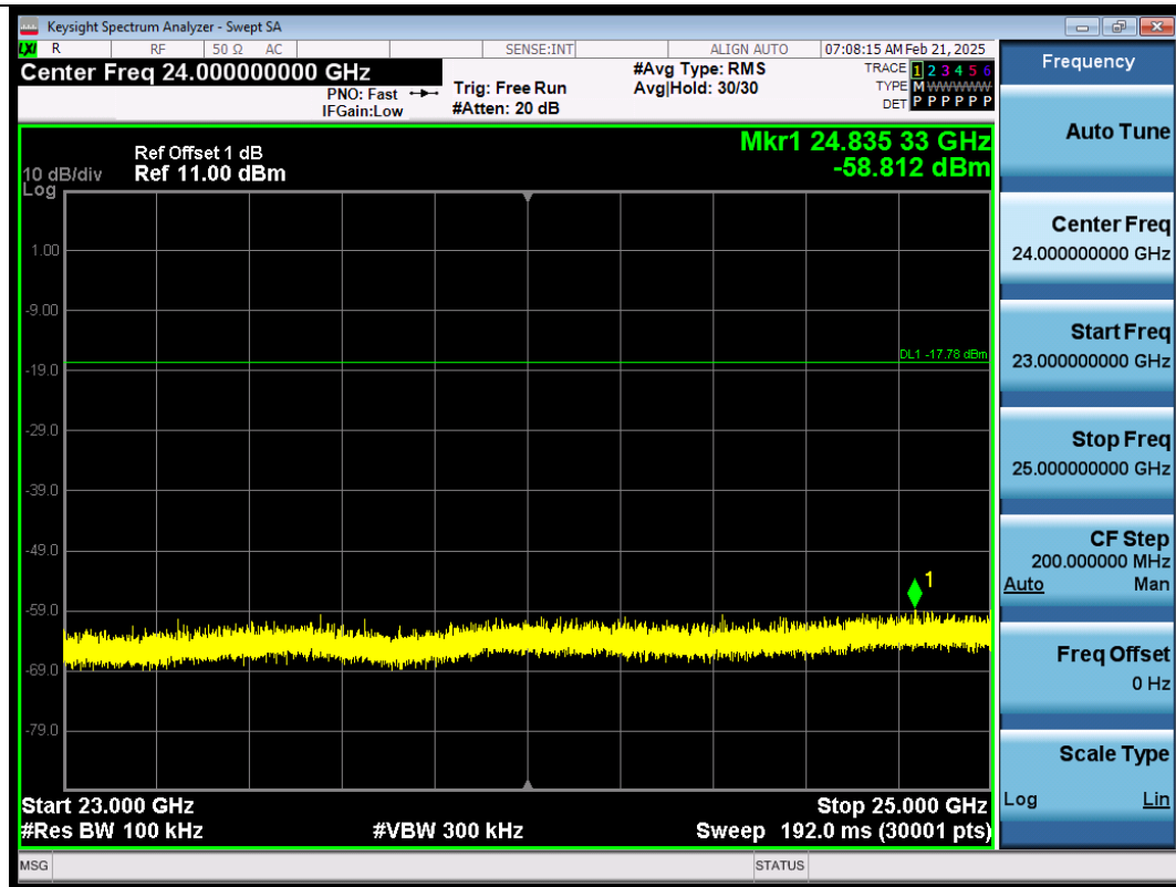
BLE_1M-Ant1-2480-23000~25000-PASS
