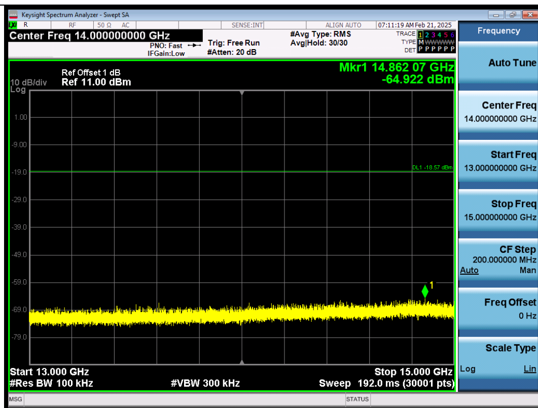
BLE_2M-Ant1-2404-13000~15000-PASS
