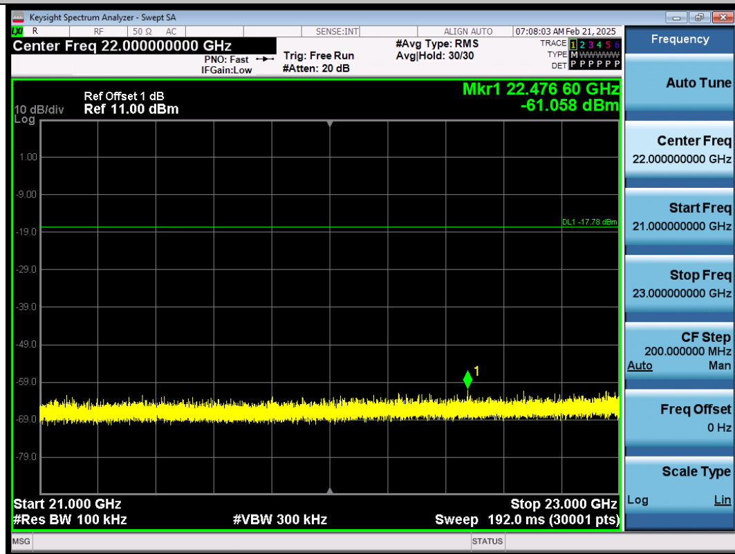
BLE_1M-Ant1-2480-21000~23000-PASS
