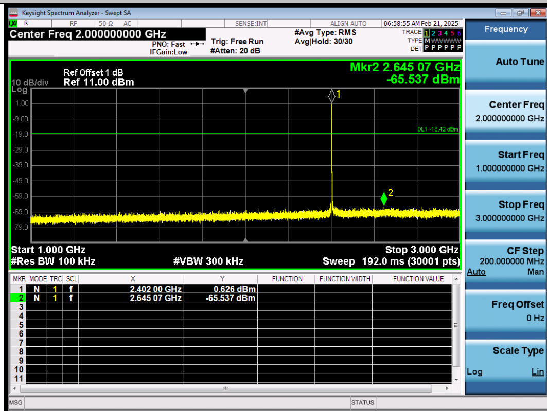
BLE_1M-Ant1-2402-1000~3000-PASS
