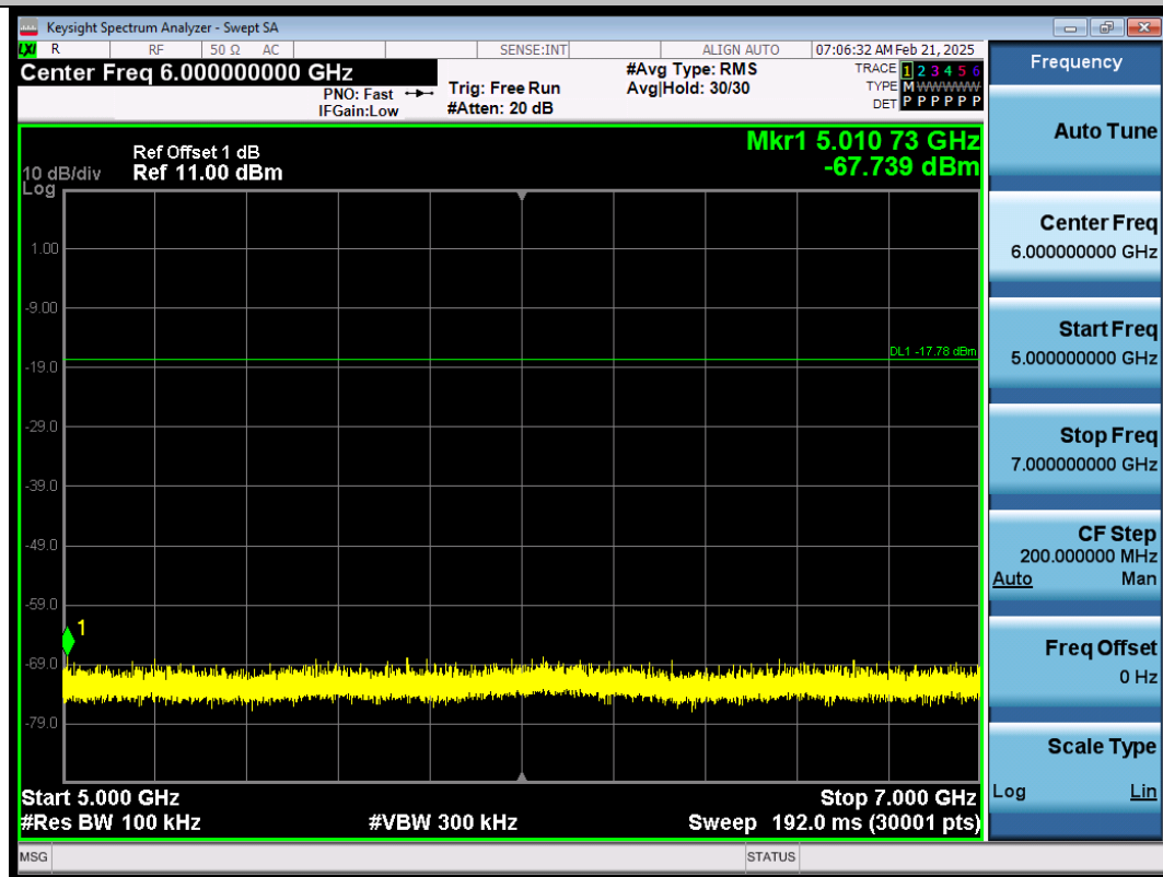
BLE_1M-Ant1-2480-5000~7000-PASS
