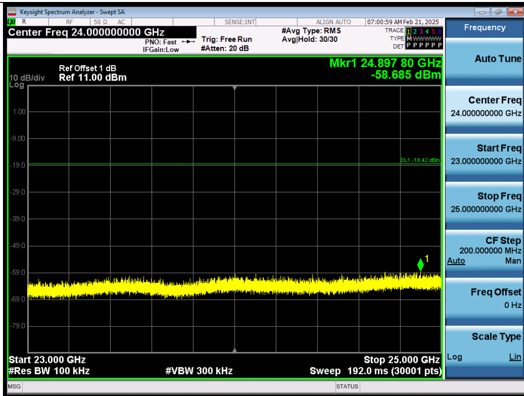
BLE_1M-Ant1-2402-23000~25000-PASS
