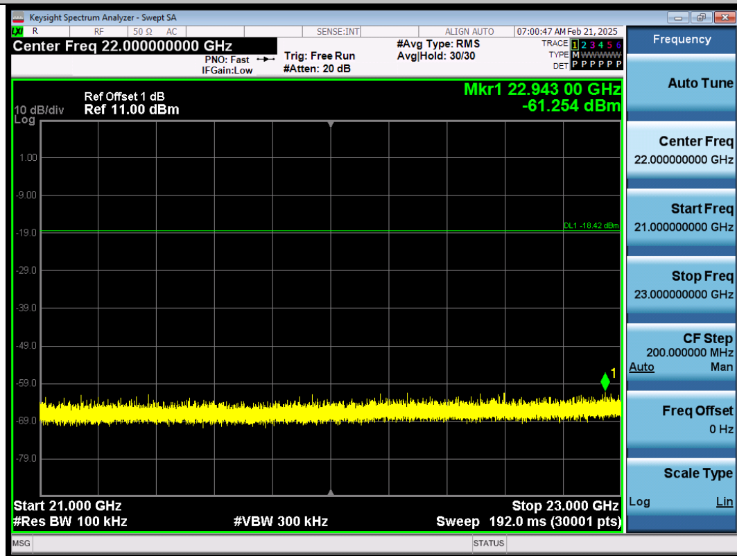
BLE_1M-Ant1-2402-21000~23000-PASS
