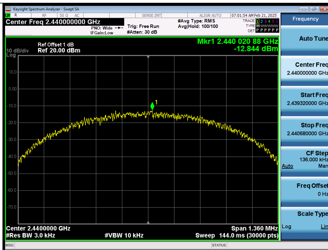
BLE_1M-Ant1-2440-PASS
