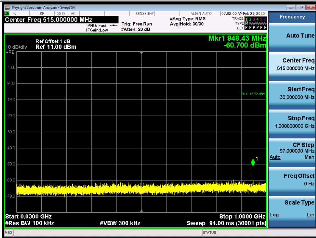
BLE_1M-Ant1-2440-30~1000-PASS
