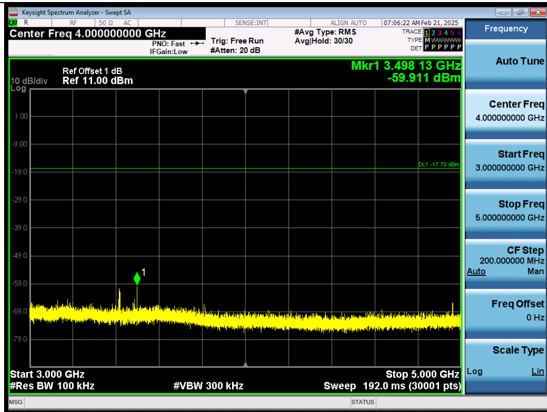
BLE_1M-Ant1-2480-3000~5000-PASS
