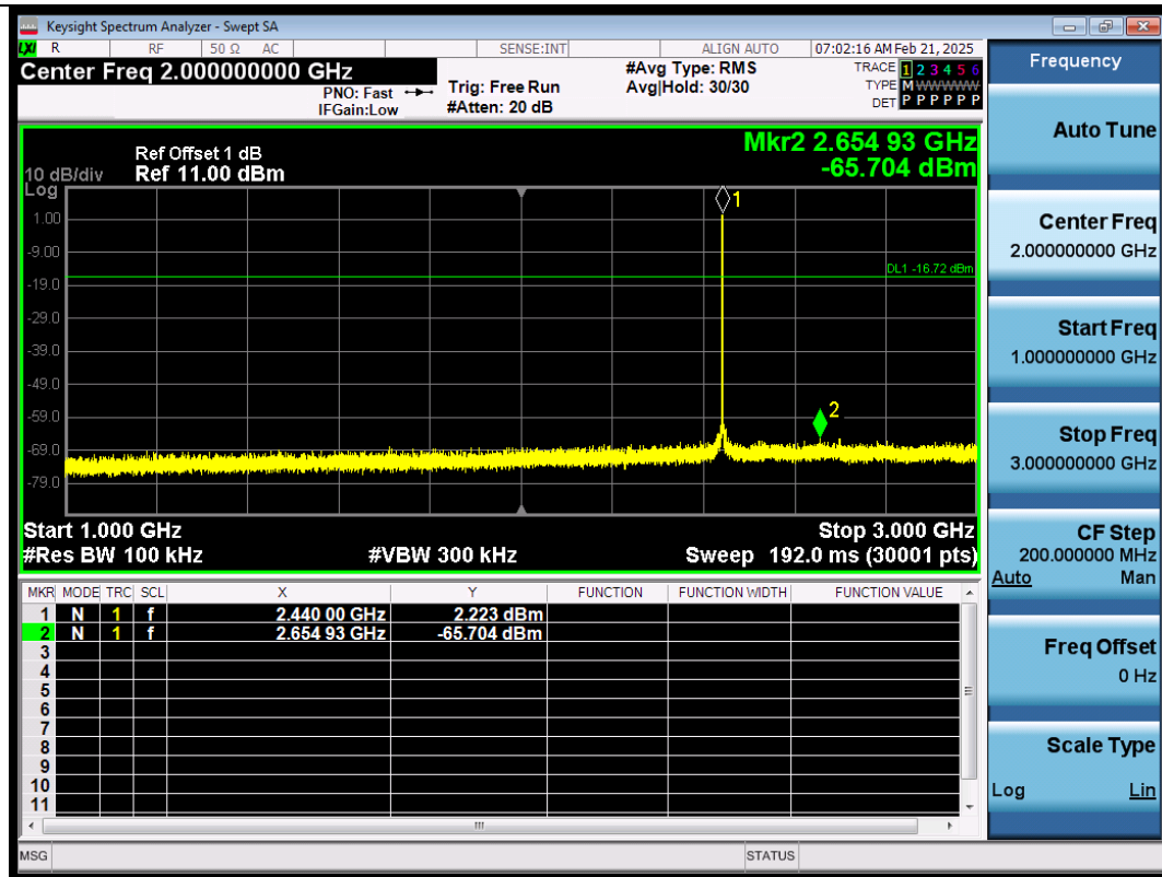
BLE_1M-Ant1-2440-1000~3000-PASS
