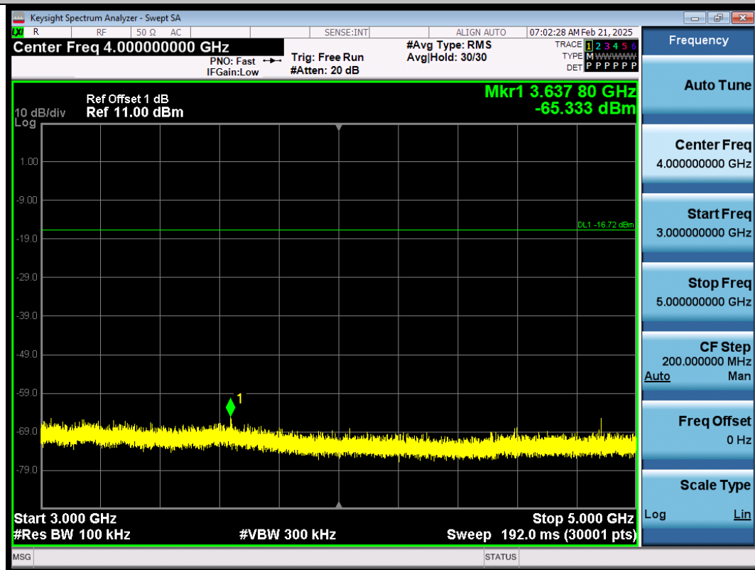
BLE_1M-Ant1-2440-3000~5000-PASS
