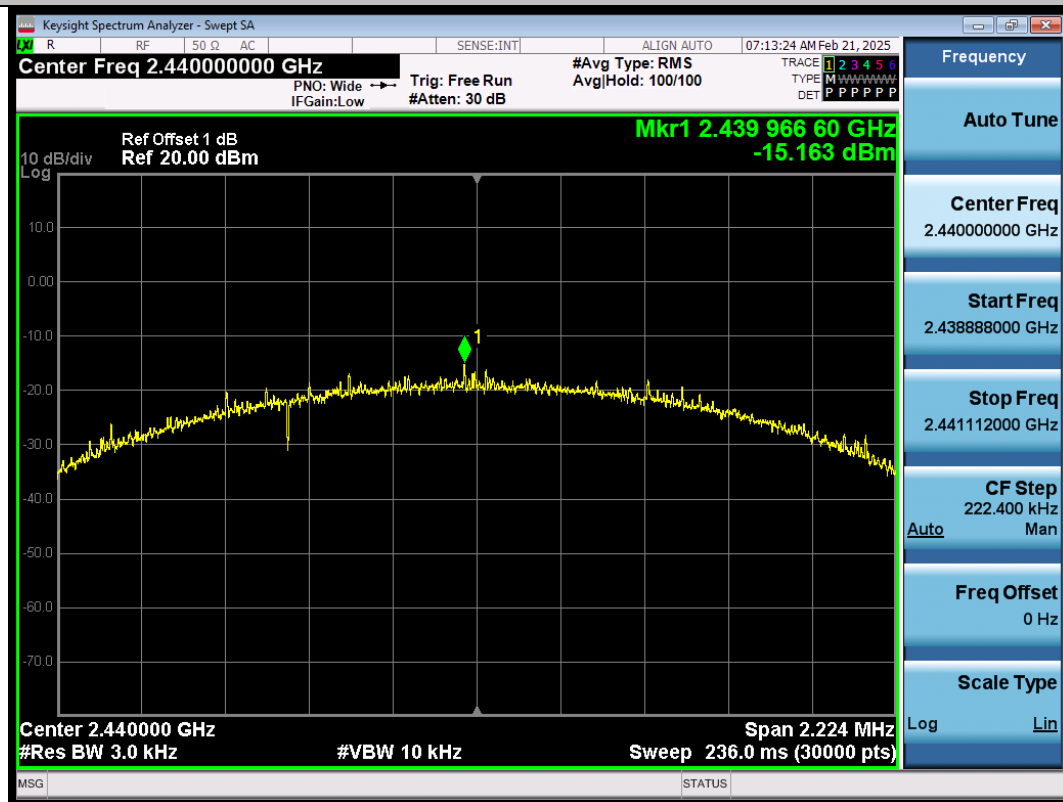
BLE_2M-Ant1-2440-PASS
