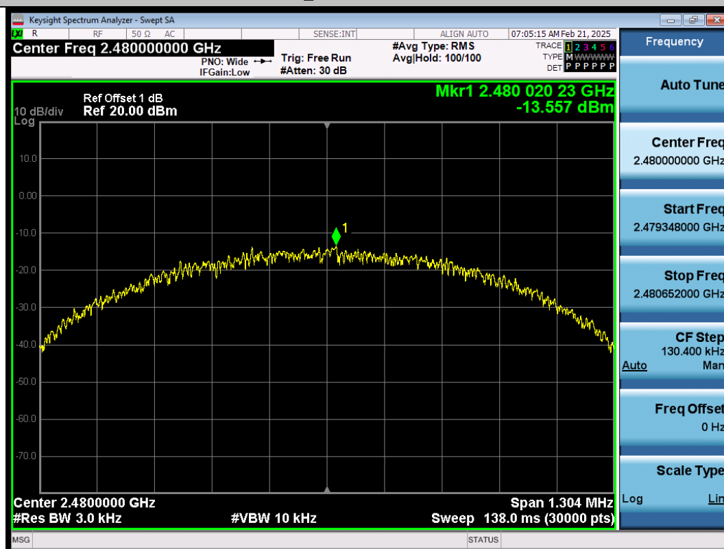
BLE_1M-Ant1-2480-PASS
