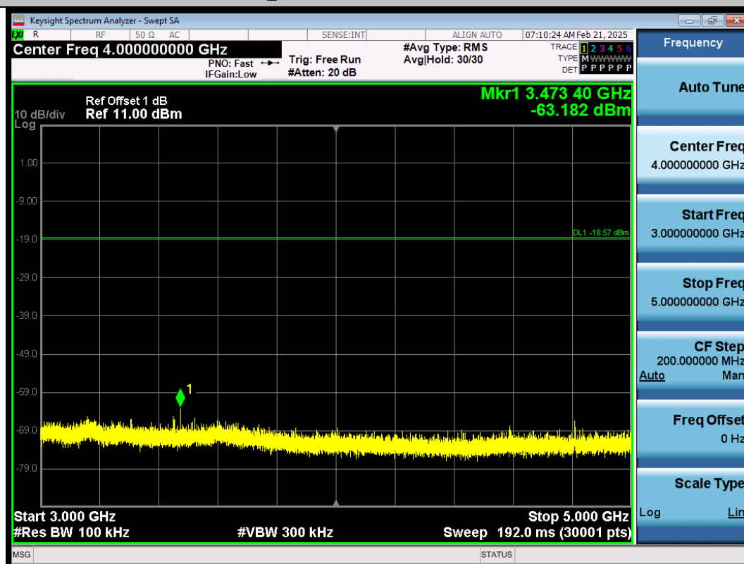
BLE_2M-Ant1-2404-3000~5000-PASS
