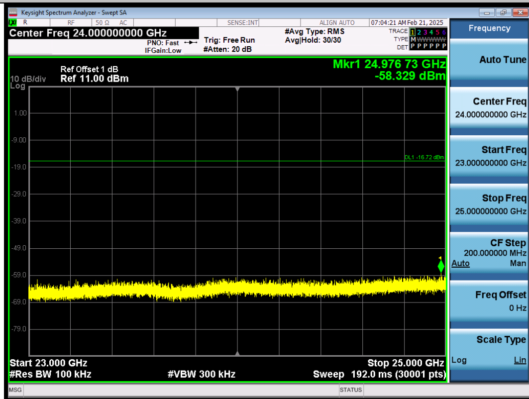
BLE_1M-Ant1-2440-23000~25000-PASS
