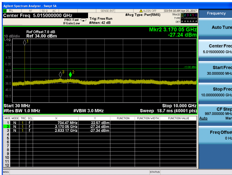
LTE Band 17 / 5MHz / QPSK - RB Size/Offset (12/0) – Low Channel
