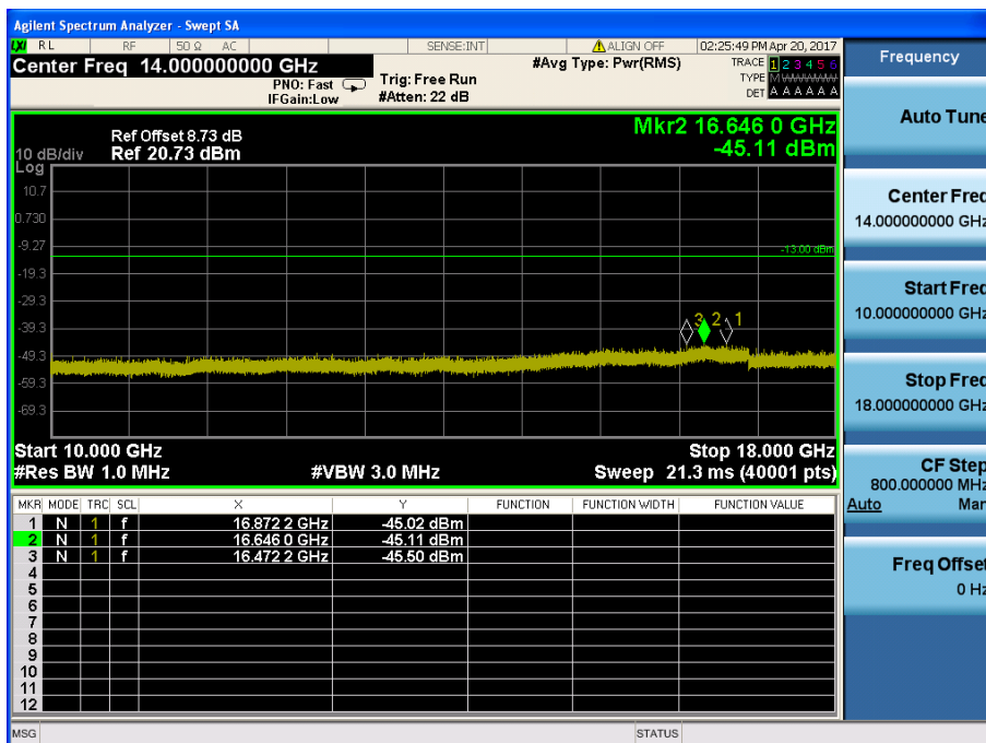
LTE Band 4 / 15MHz / 16QAM - RB Size/Offset (36/19)-Low Channel
