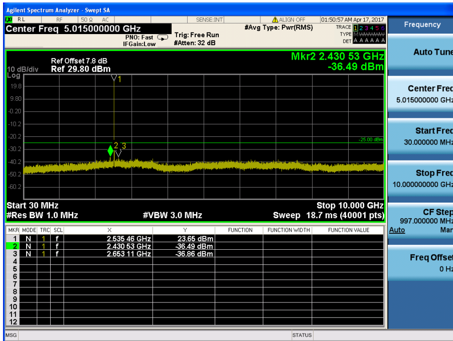
LTE Band 7 / 15MHz / QPSK - RB Size/Offset (1/37) – Mid Channel
