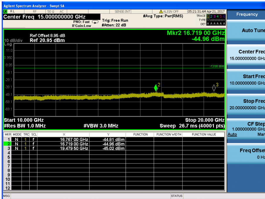
LTE Band 2 / 10MHz / QPSK - RB Size/Offset (25/12) – Mid Channel
