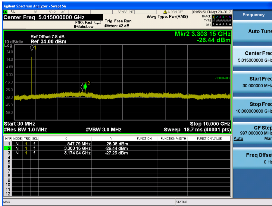
LTE Band 5 / 3MHz / QPSK - RB Size/Offset (8/3) – High Channel
