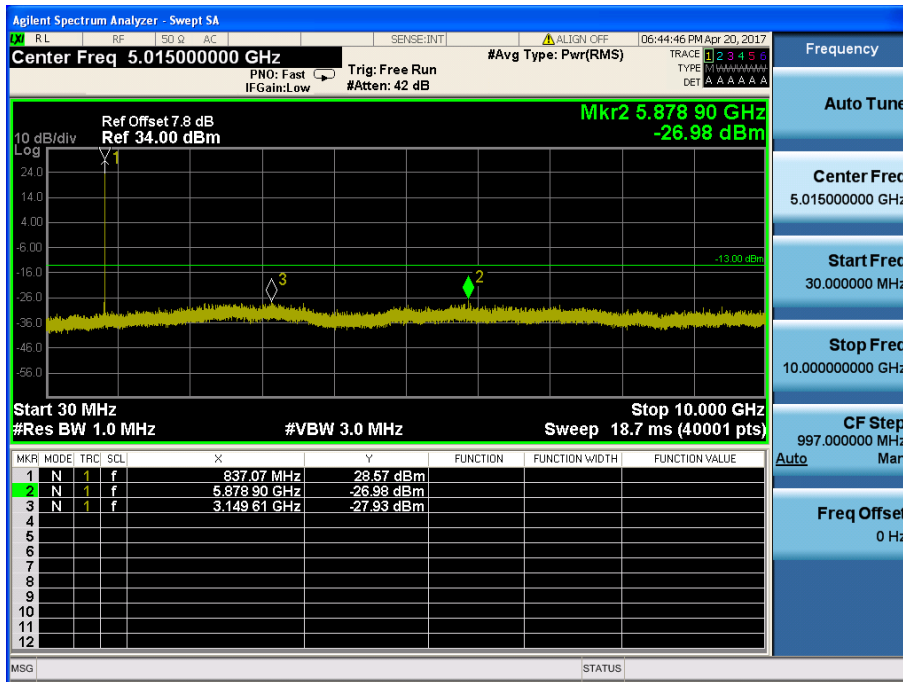
LTE Band 5 / 1.4MHz / 16QAM - RB Size/Offset (1/5) – Mid Channel
