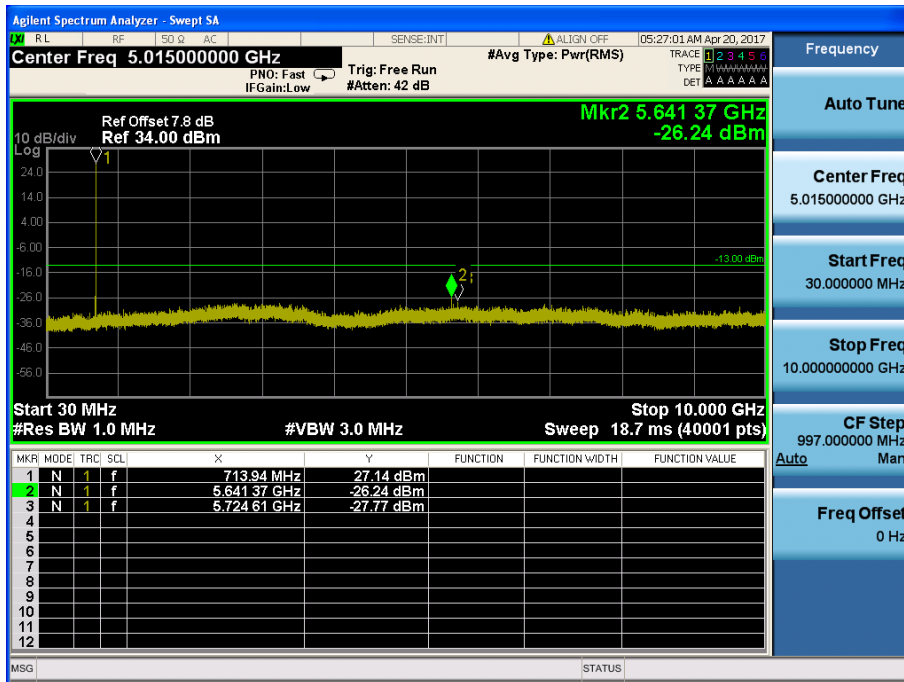
LTE Band 17 / 5MHz / 16QAM - RB Size/Offset (1/25) – High Channel
