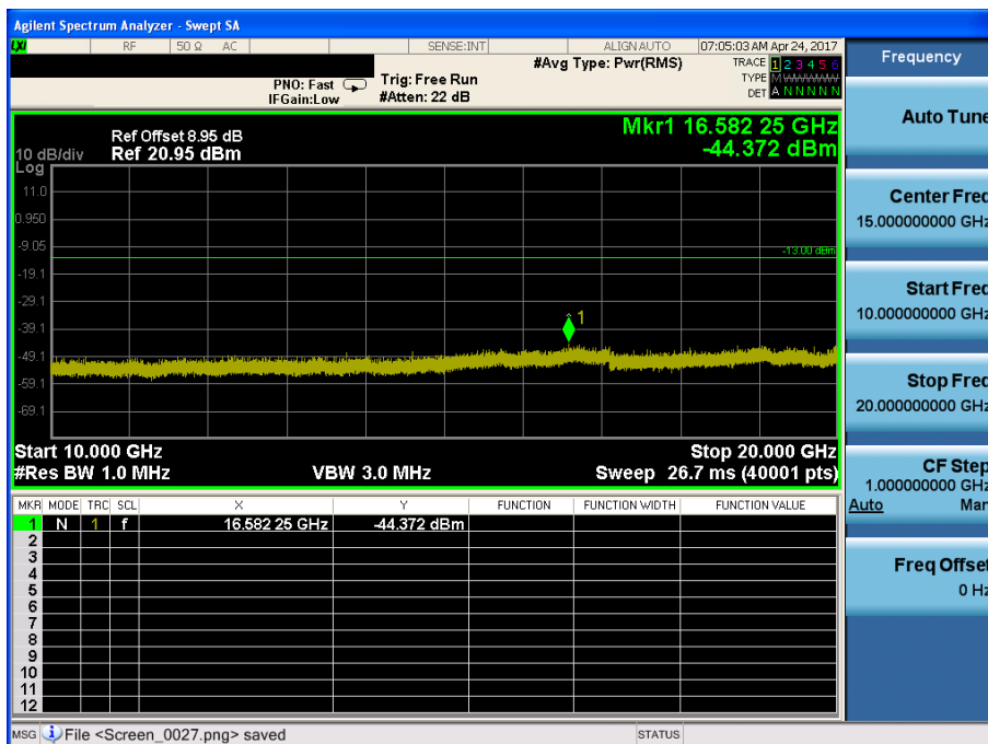
LTE Band 2 / 3MHz / 16QAM - RB Size/Offset (8/3) – High Channel
