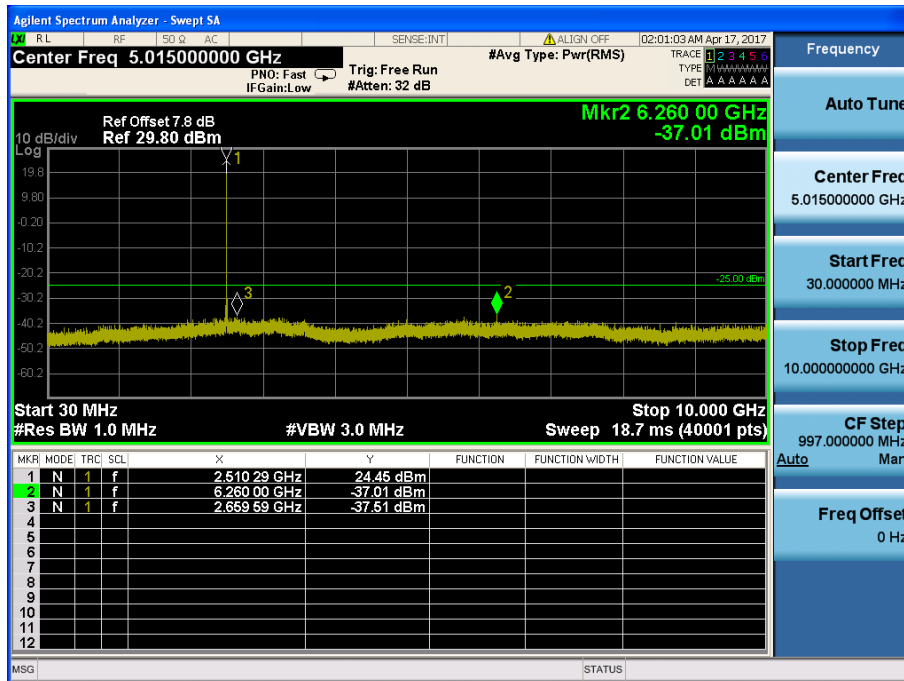
LTE Band 7 / 20MHz / QPSK - RB Size/Offset (1/50) – Low Channel
