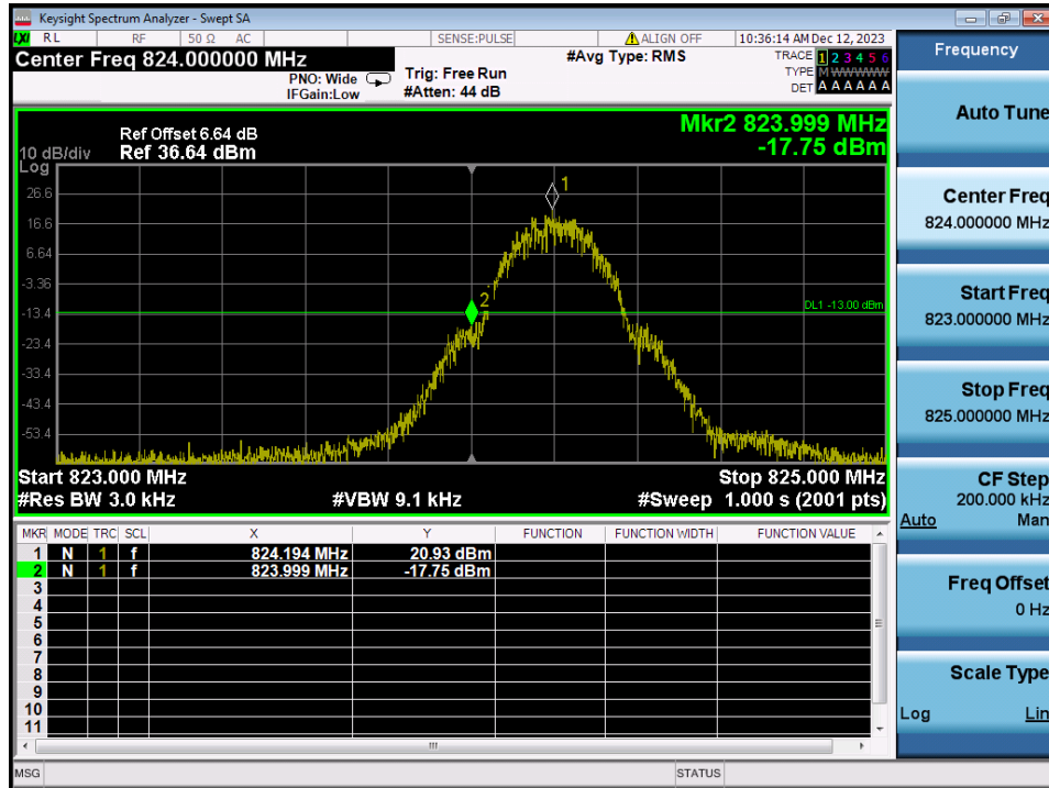
GSM850 & Channel: 128
