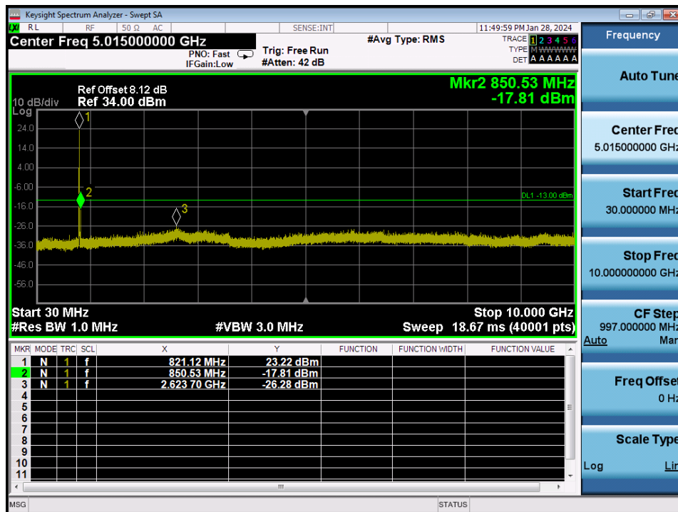
LTE Band 26 / 10 MHz / 16QAM - RB Size/Offset (25/25) - Low Channel
