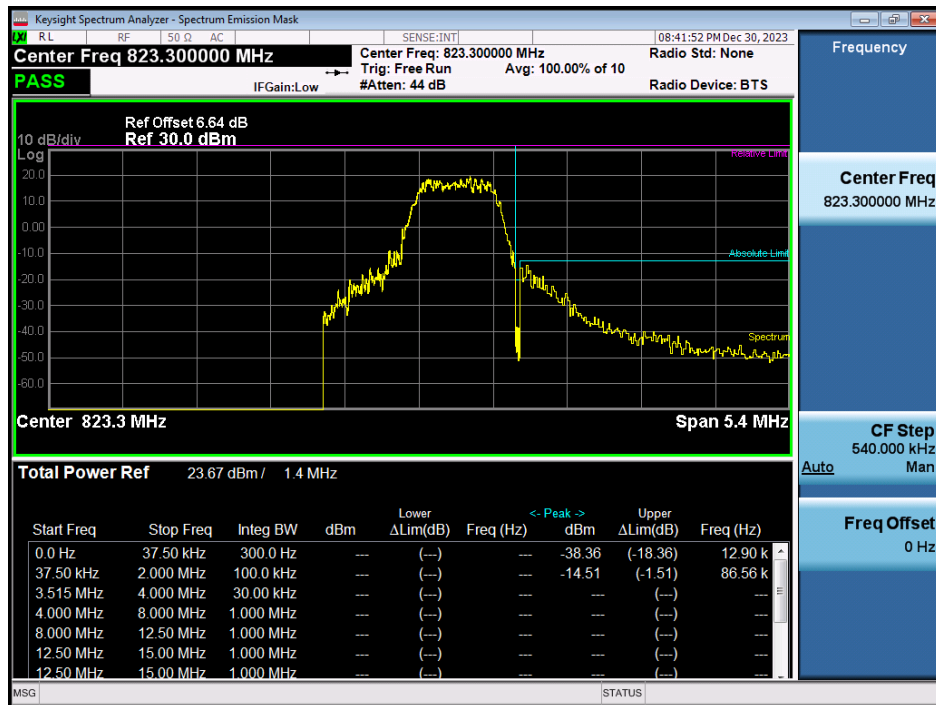
LTE Band 26 / 1.4 MHz / QPSK - RB Size/Offset (3/3)
