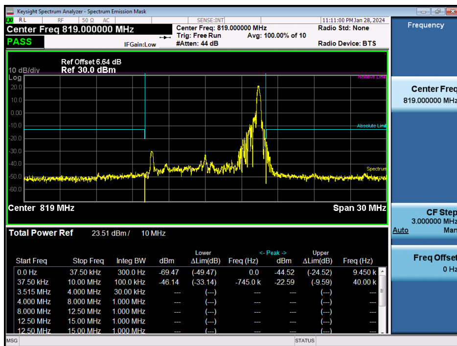
LTE Band 26 / 10 MHz / QPSK- RB Size/Offset (1/49)
