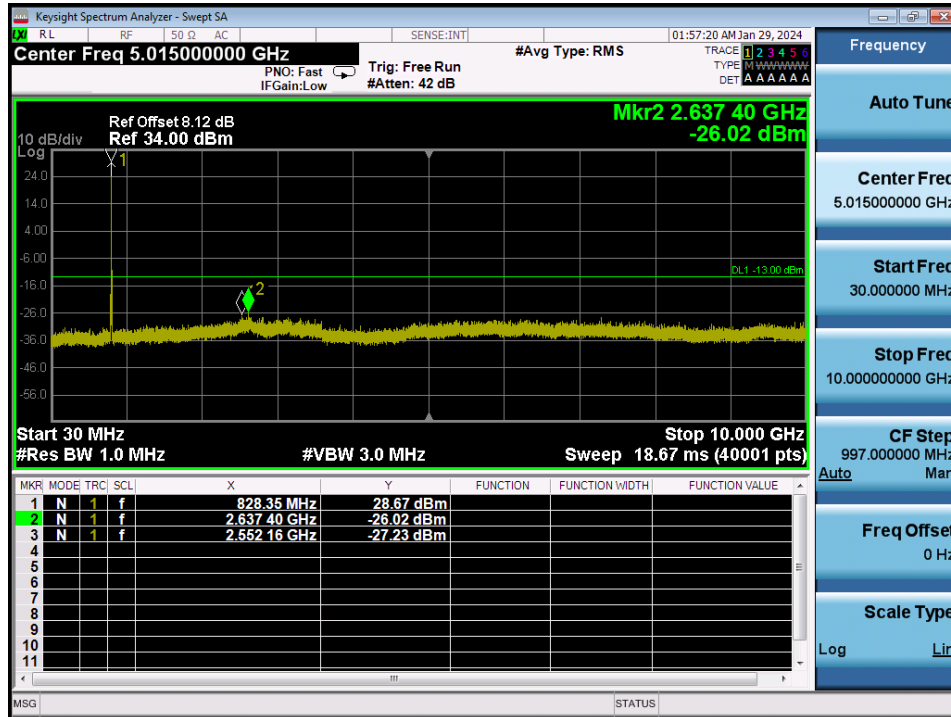
LTE Band 26 / 15 MHz / 64QAM - RB Size/Offset (1/74) - Low Channel
