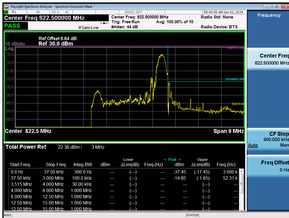
LTE Band 26 / 3 MHz / 16QAM - RB Size/Offset (1/14)
