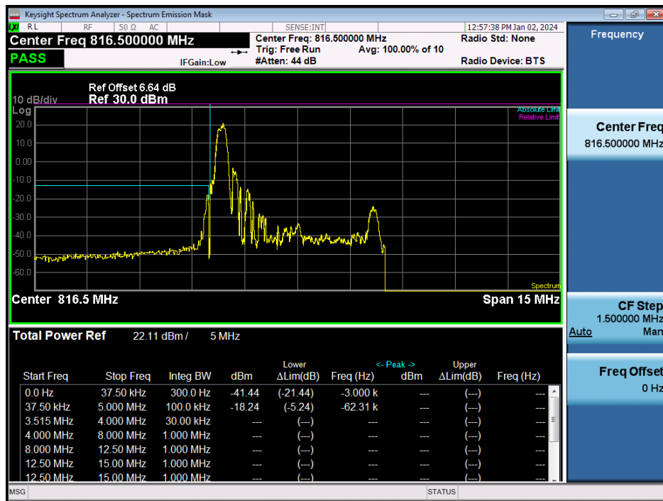
LTE Band 26 / 5 MHz / 64QAM - RB Size/Offset (1/0)
