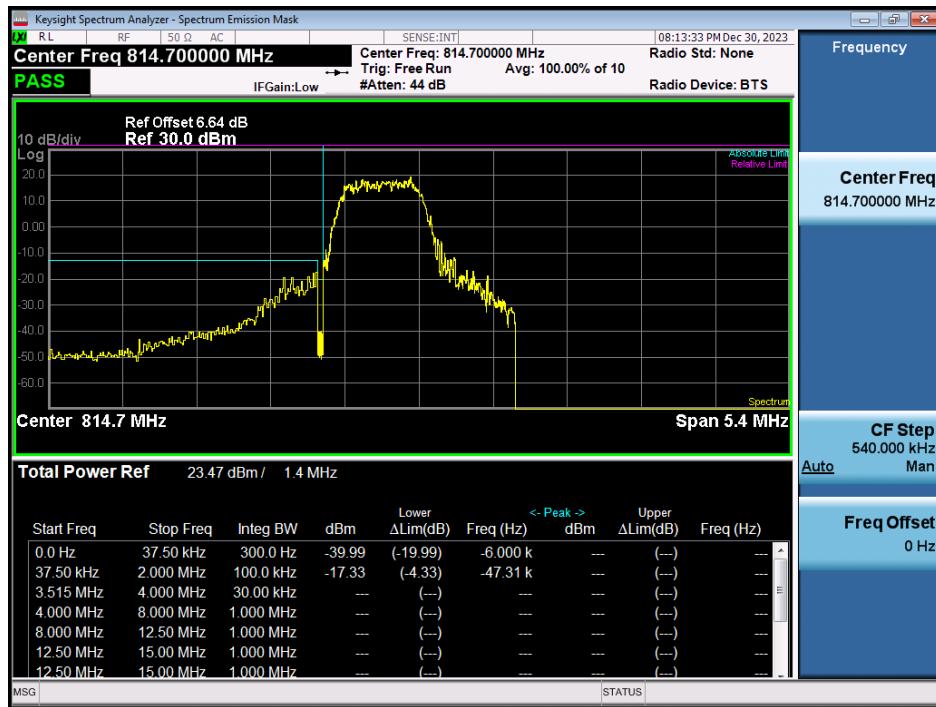
LTE Band 26 / 1.4 MHz / QPSK - RB Size/Offset (3/0)
