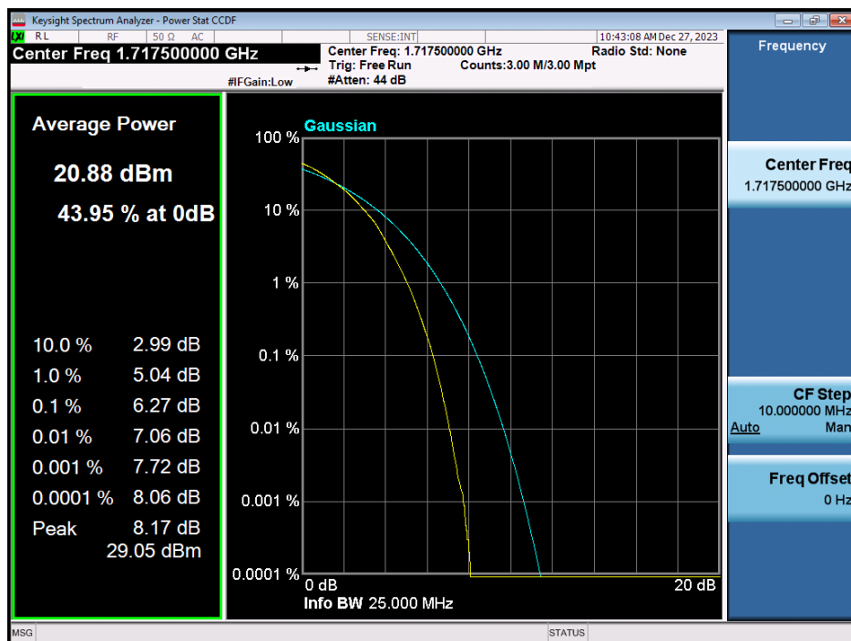
LTE Band 66 / 15MHz / 64QAM - RB Size 75
