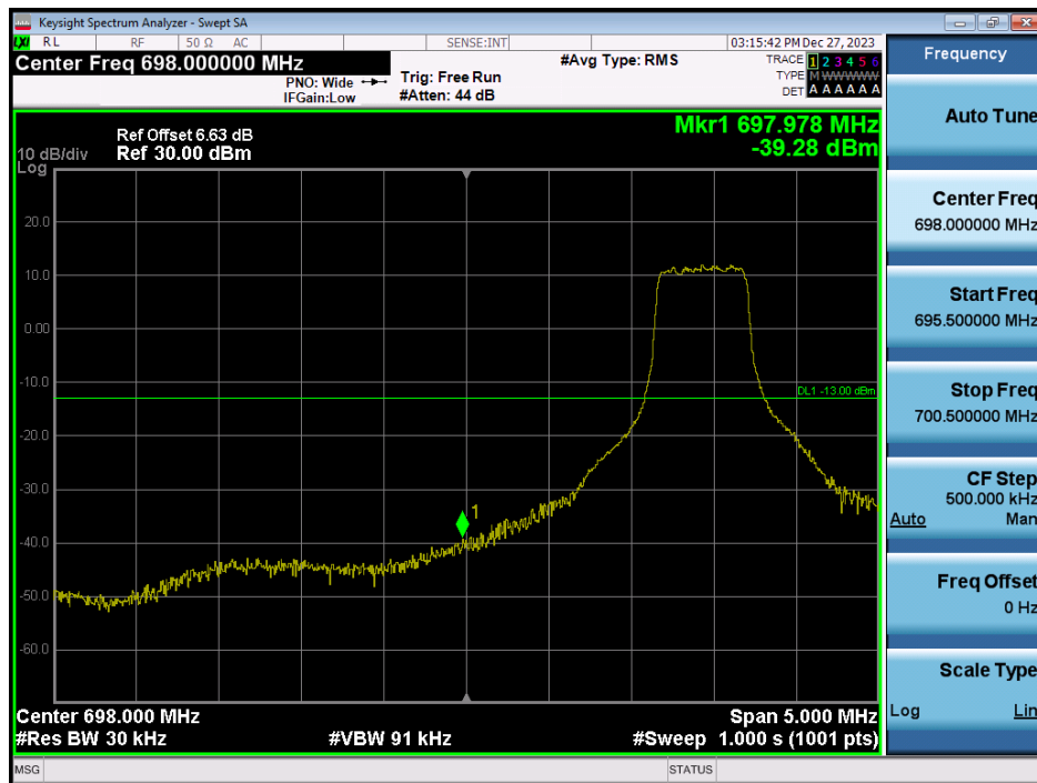
LTE Band 12 / 1.4MHz / 16QAM - RB Size/Offset (3/0)
