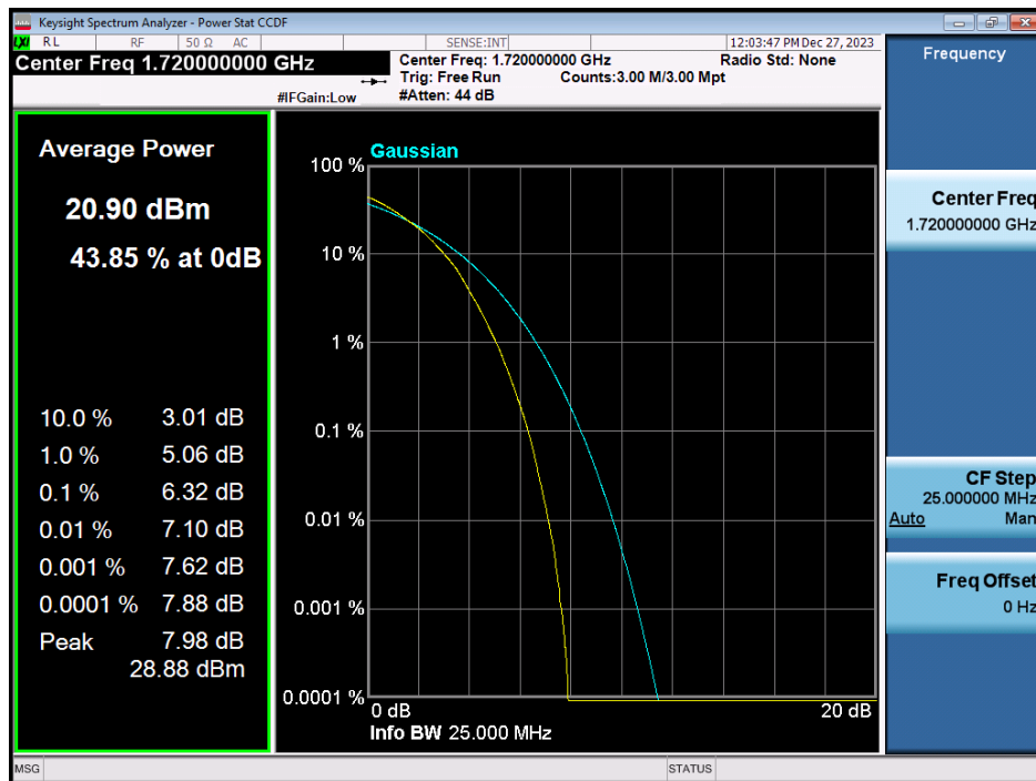
LTE Band 66 / 20MHz / 64QAM - RB Size 100
