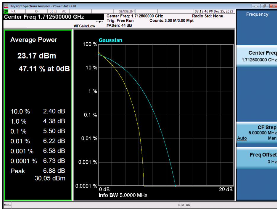
LTE Band 66 / 5MHz / QPSK - RB Size 25
