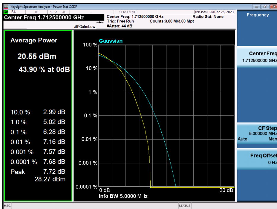
LTE Band 66 / 5MHz / 64QAM - RB Size 25
