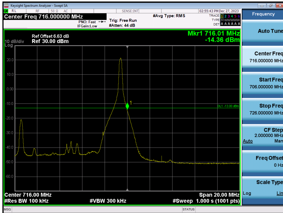
LTE Band 12 / 10MHz / QPSK - RB Size/Offset (1/49)
