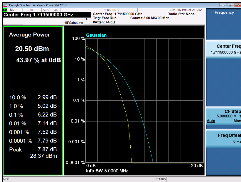
LTE Band 66 / 3MHz / 64QAM - RB Size 15
