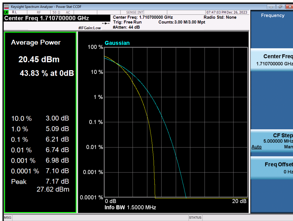
LTE Band 66 / 1.4MHz / 64QAM - RB Size 6
