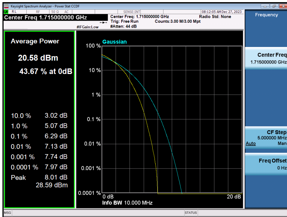
LTE Band 66 / 10MHz / 64QAM - RB Size 50
