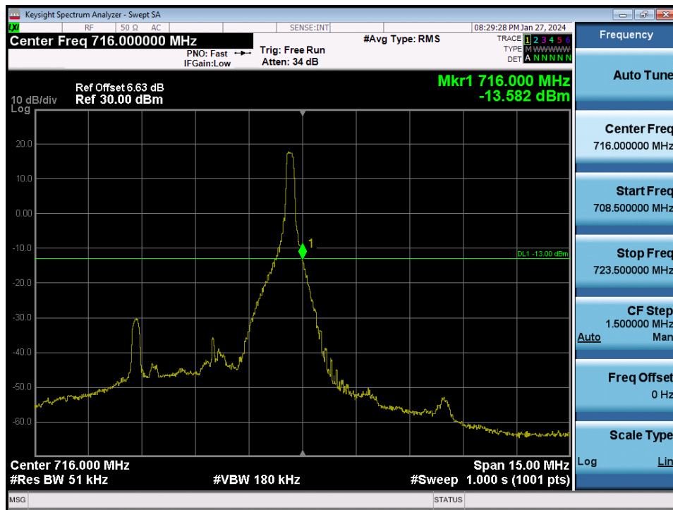
LTE Band 12 / 5MHz / QPSK - RB Size/Offset (1/24)
