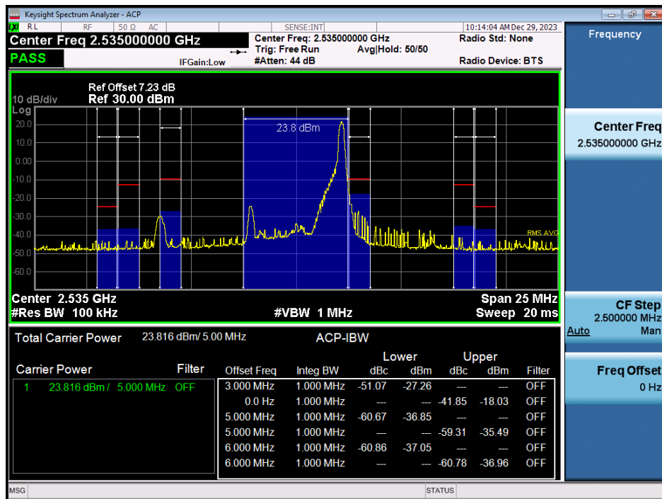
LTE Band 7 / 5MHz / QPSK - RB Size/Offset (1/24)
