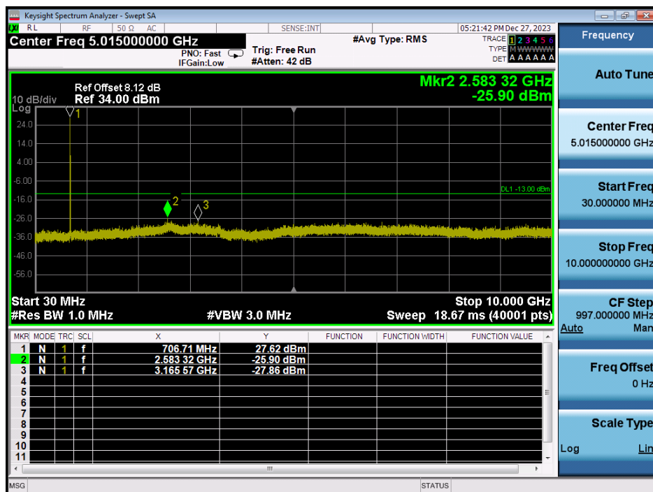
LTE Band 12 / 10MHz / 16QAM - RB Size/Offset (1/0) – High Channel
