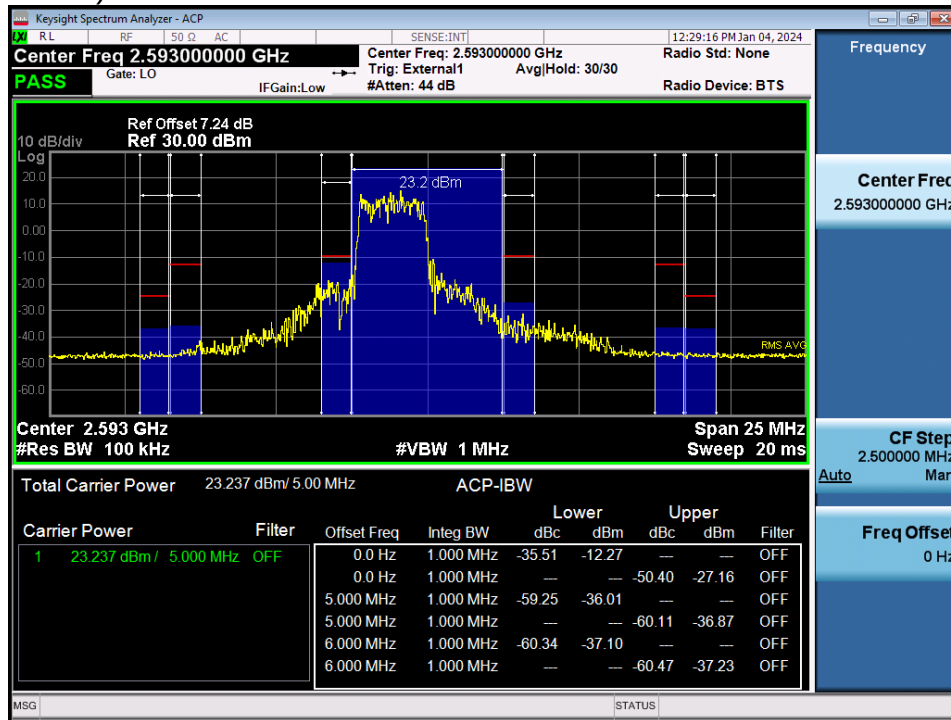
LTE Band 41 / 5MHz / QPSK - RB Size/Offset (12/0)
