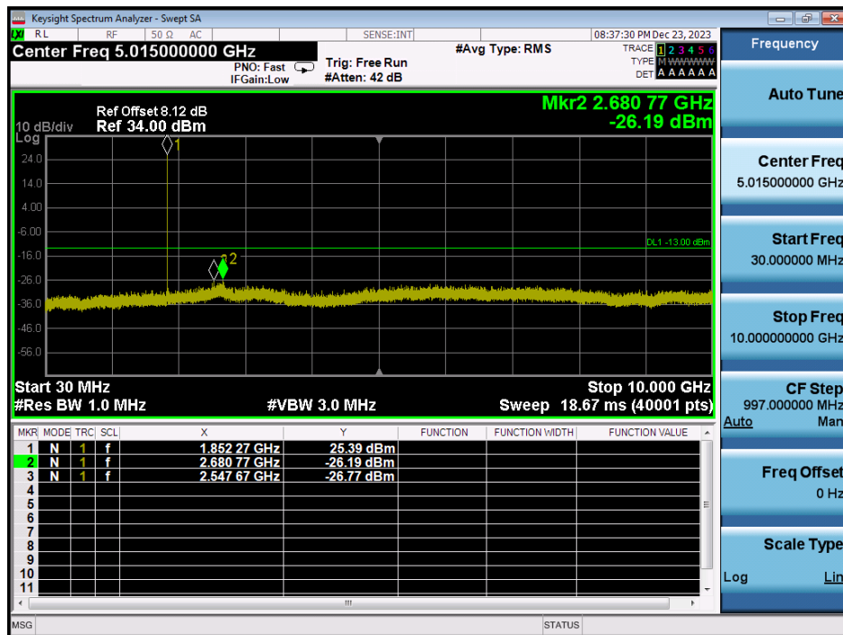
LTE Band 25 / 3MHz / QPSK - RB Size/Offset (8/7) - Low Channel
