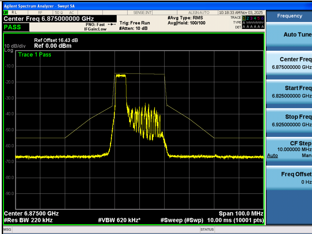
NTNV-11AX20SISO-Ant3-6875-52Tone-RU37-PASS
