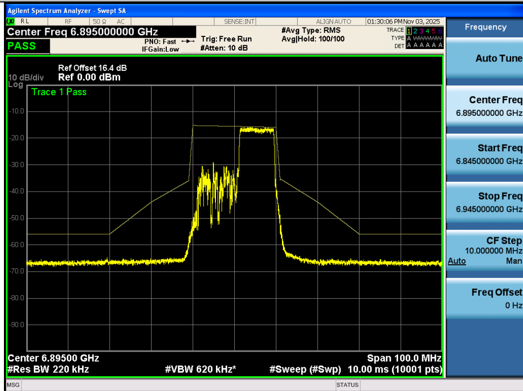
NTNV-11AX20SISO-Ant3-6895-106Tone-RU54-PASS
