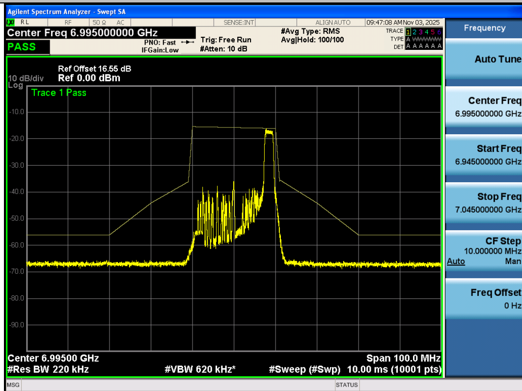
NTNV-11AX20SISO-Ant3-6995-26Tone-RU8-PASS
