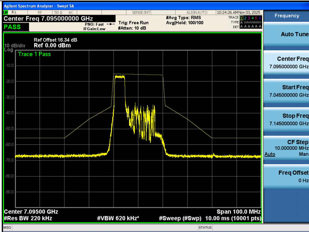
NTNV-11AX20SISO-Ant3-7095-52Tone-RU37-PASS
