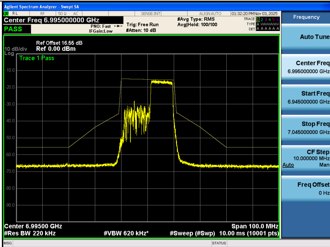
NTNV-11AX20SISO-Ant3-6995-106Tone-RU54-PASS
