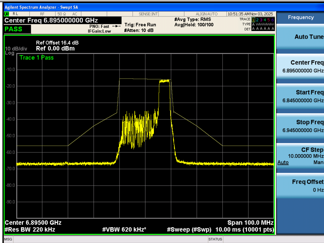
NTNV-11AX20SISO-Ant3-6895-52Tone-RU40-PASS
