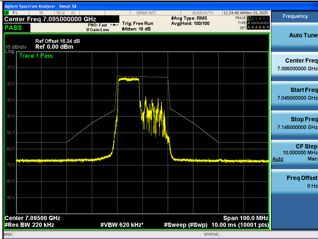
NTNV-11AX20SISO-Ant3-7095-106Tone-RU53-PASS
