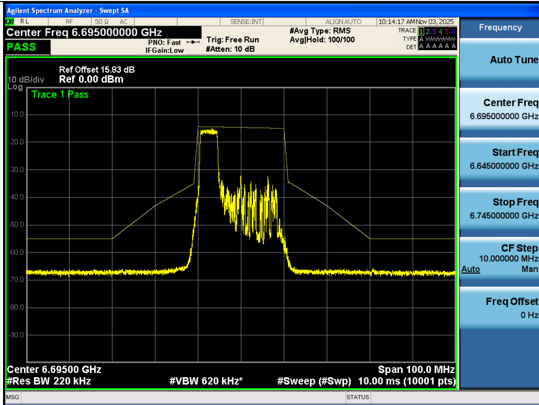
NTNV-11AX20SISO-Ant3-6695-52Tone-RU37-PASS
