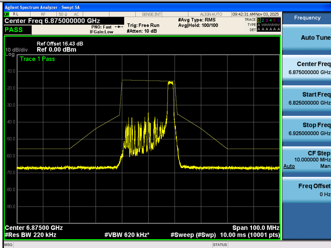
NTNV-11AX20SISO-Ant3-6875-26Tone-RU8-PASS
