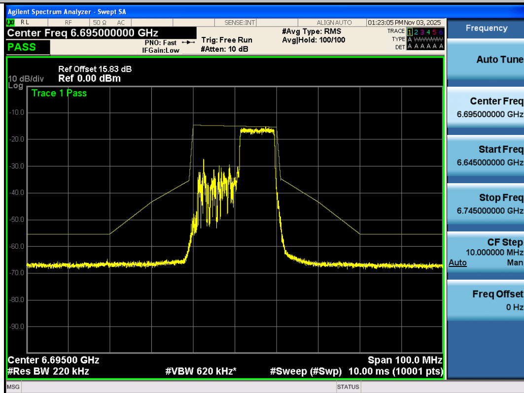
NTNV-11AX20SISO-Ant3-6695-106Tone-RU54-PASS
