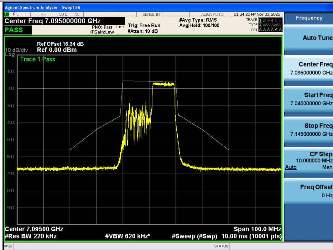
NTNV-11AX20SISO-Ant3-7095-106Tone-RU54-PASS
