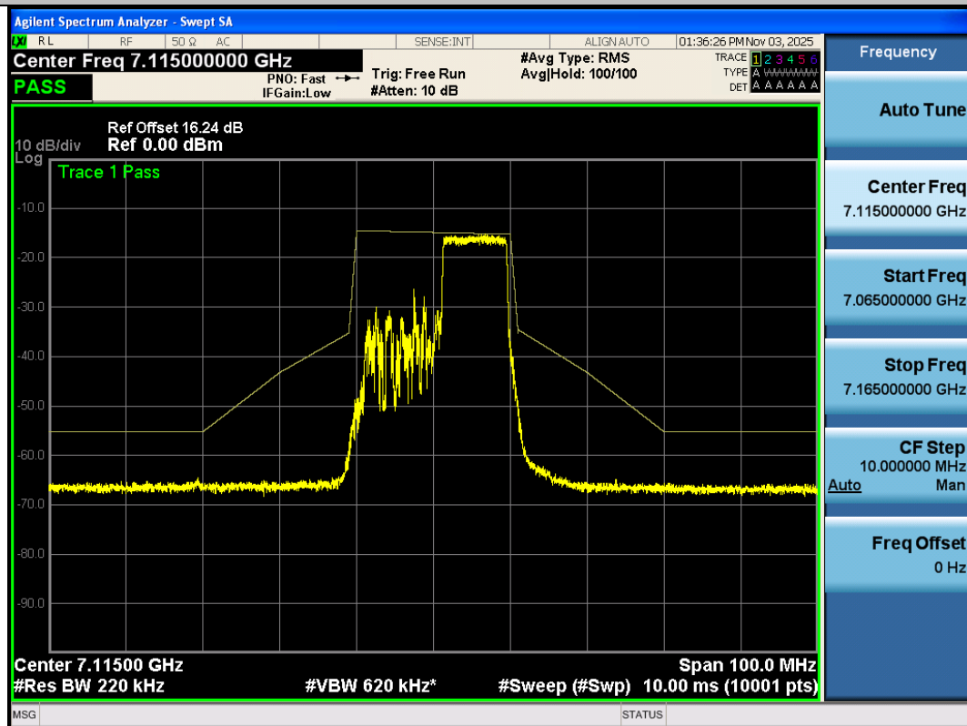
NTNV-11AX20SISO-Ant3-7115-106Tone-RU54-PASS
