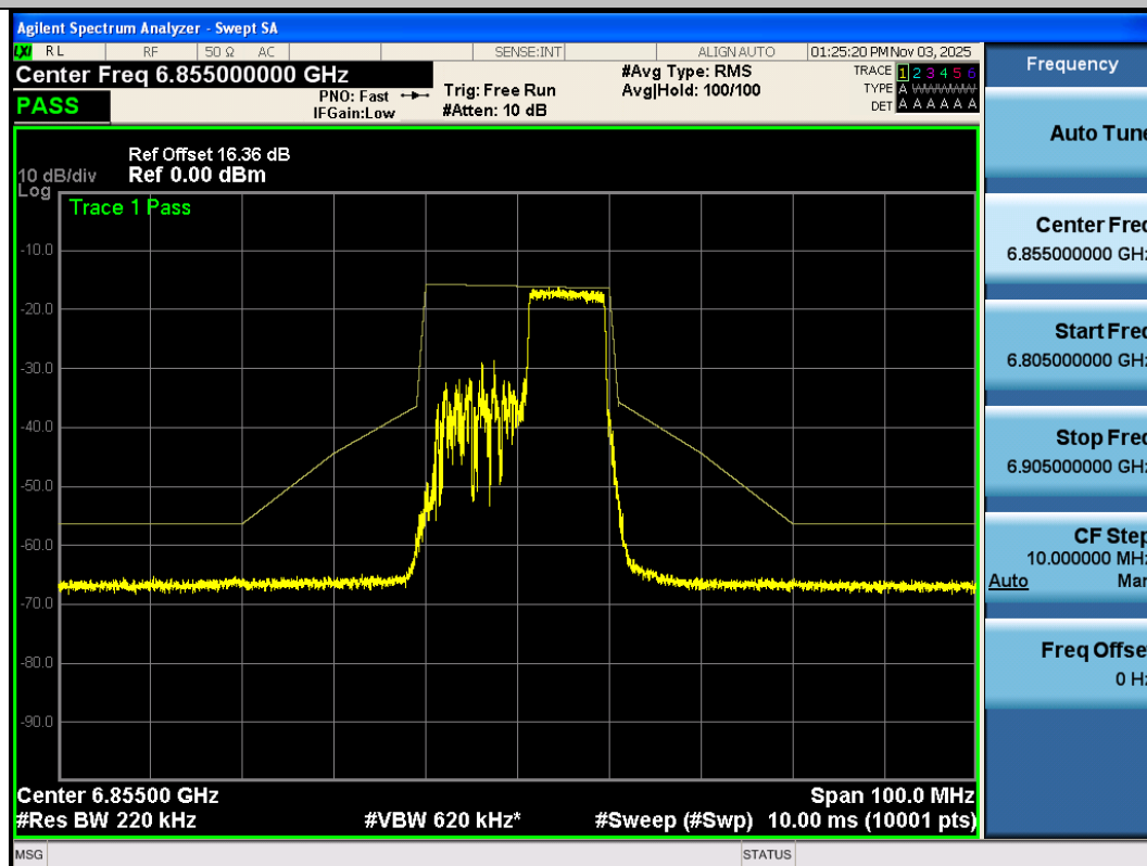
NTNV-11AX20SISO-Ant3-6855-106Tone-RU54-PASS
