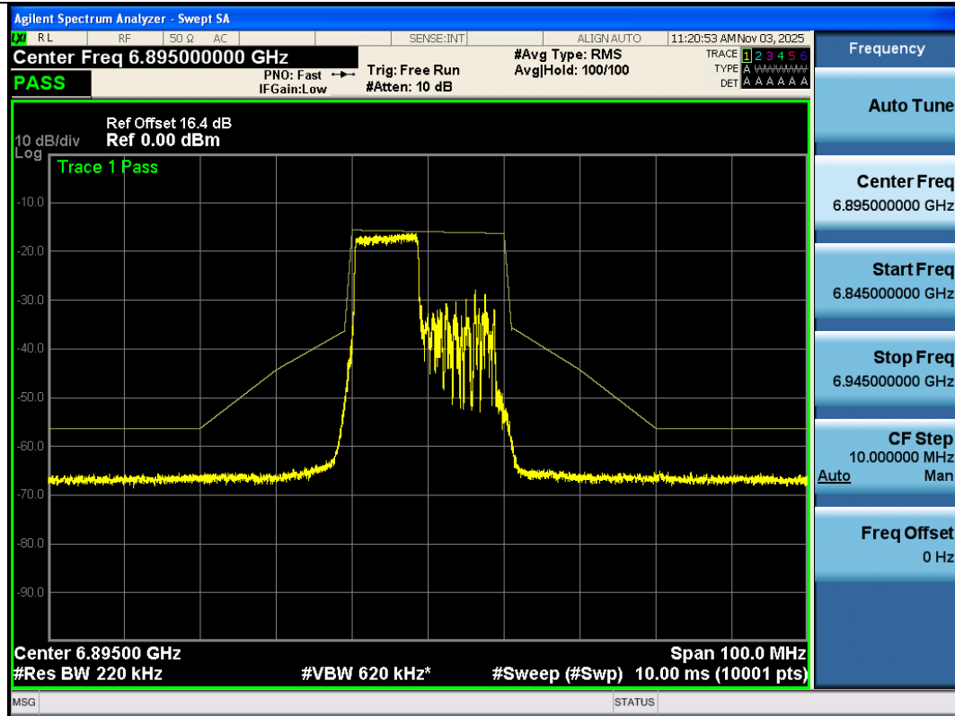
NTNV-11AX20SISO-Ant3-6895-106Tone-RU53-PASS
