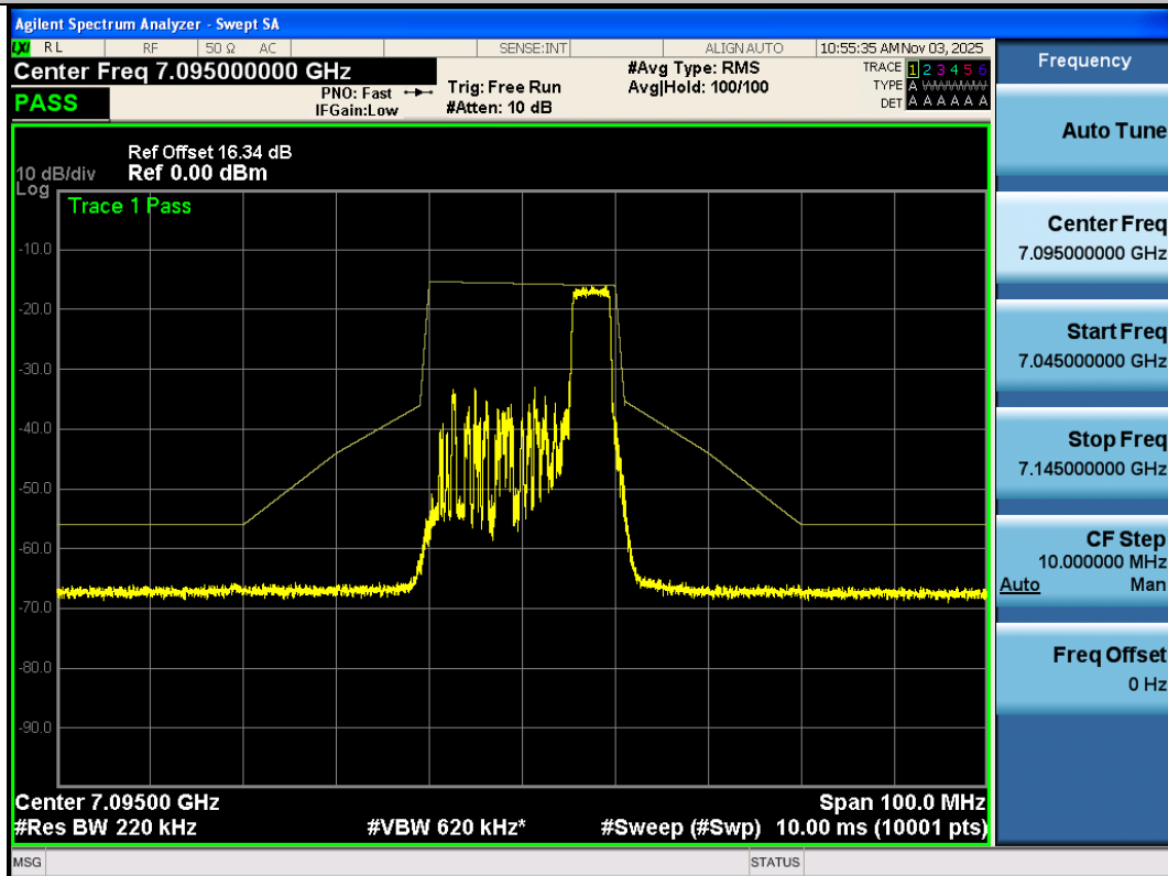
NTNV-11AX20SISO-Ant3-7095-52Tone-RU40-PASS
