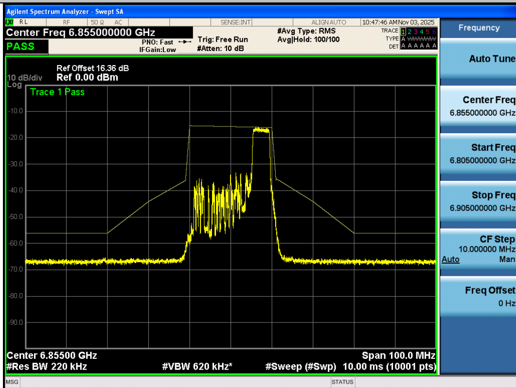
NTNV-11AX20SISO-Ant3-6855-52Tone-RU40-PASS
