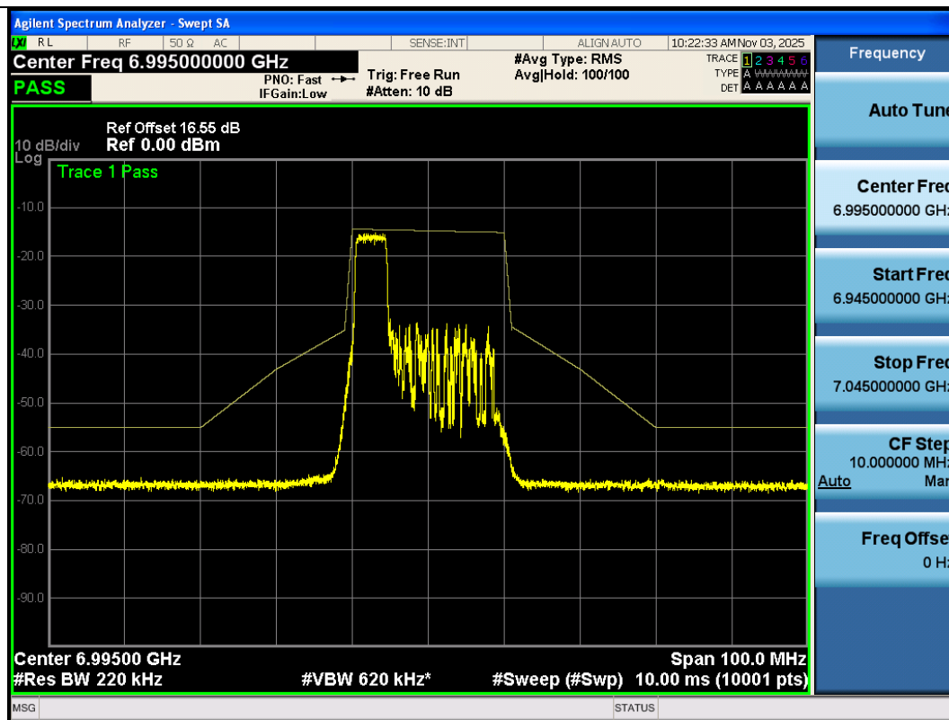
NTNV-11AX20SISO-Ant3-6995-52Tone-RU37-PASS
