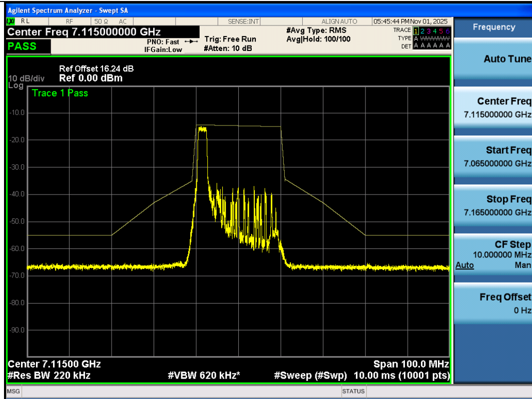
NTNV-11AX20SISO-Ant3-7115-26Tone-RU0-PASS
