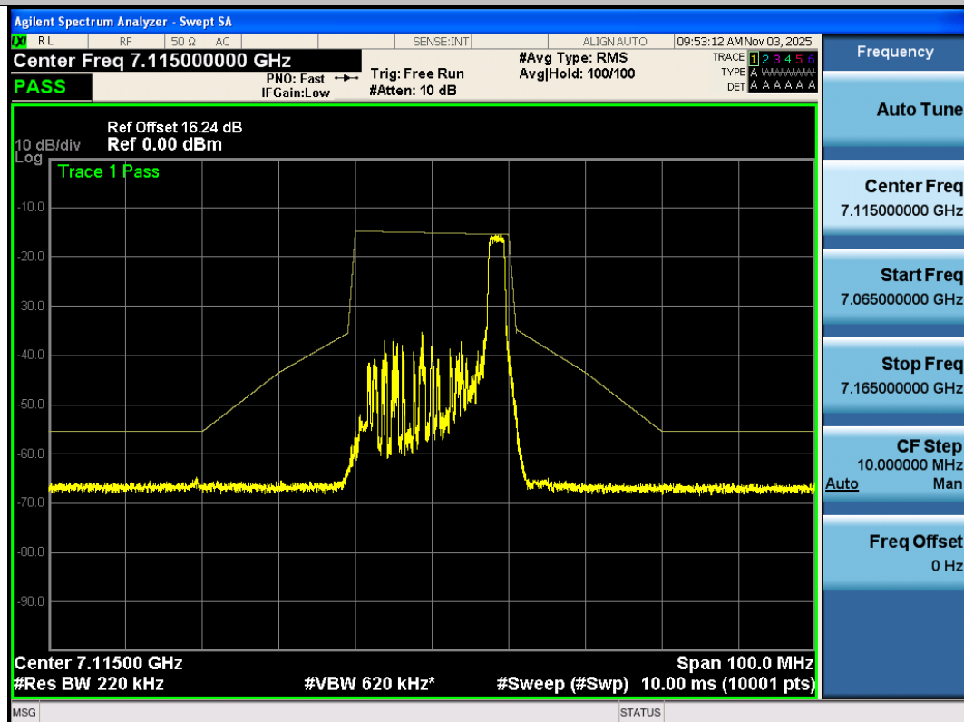
NTNV-11AX20SISO-Ant3-7115-26Tone-RU8-PASS
