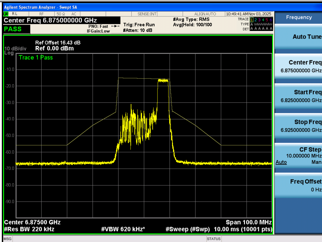
NTNV-11AX20SISO-Ant3-6875-52Tone-RU40-PASS
