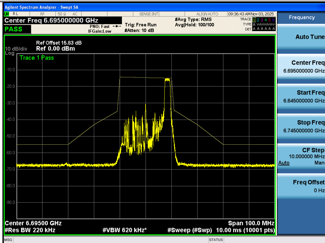
NTNV-11AX20SISO-Ant3-6695-26Tone-RU8-PASS
