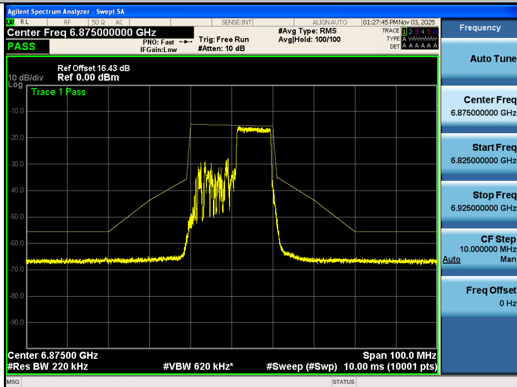
NTNV-11AX20SISO-Ant3-6875-106Tone-RU54-PASS
