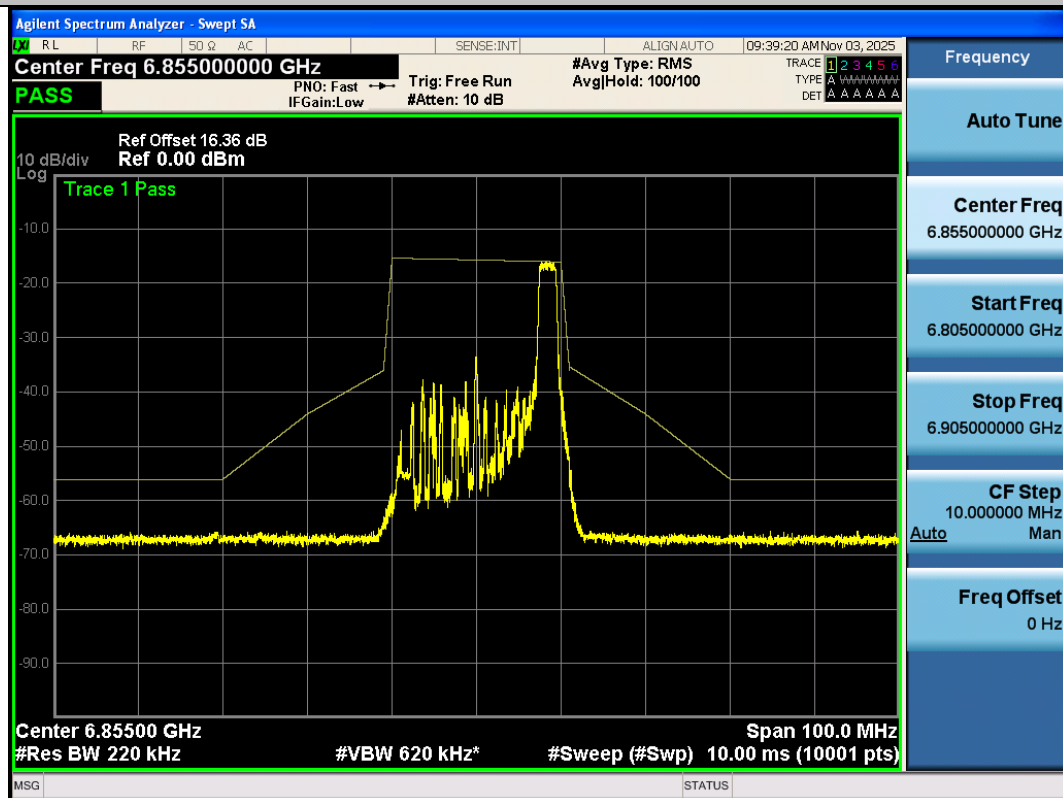
NTNV-11AX20SISO-Ant3-6855-26Tone-RU8-PASS
