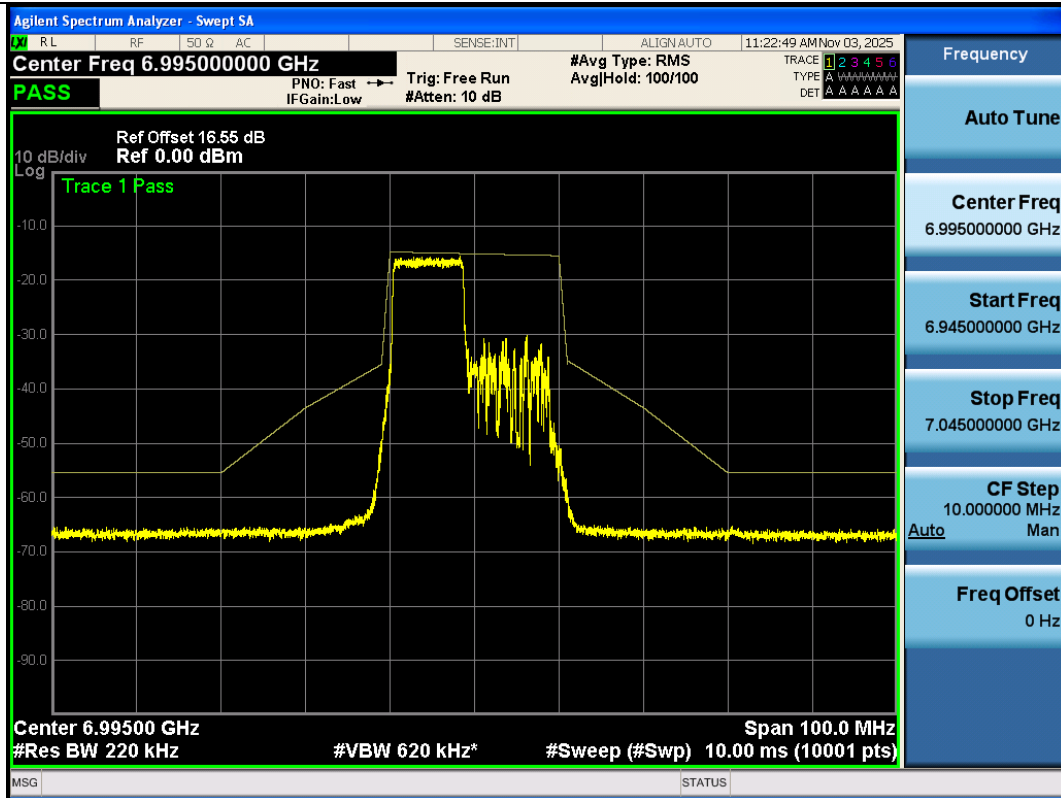
NTNV-11AX20SISO-Ant3-6995-106Tone-RU53-PASS
