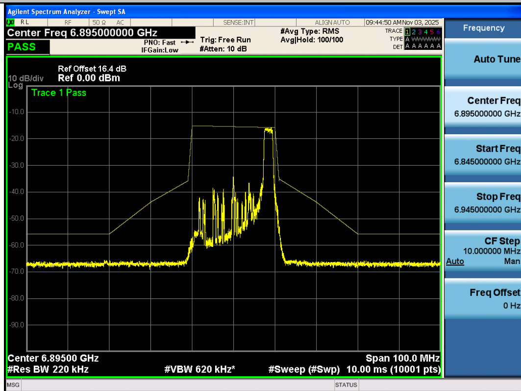
NTNV-11AX20SISO-Ant3-6895-26Tone-RU8-PASS
