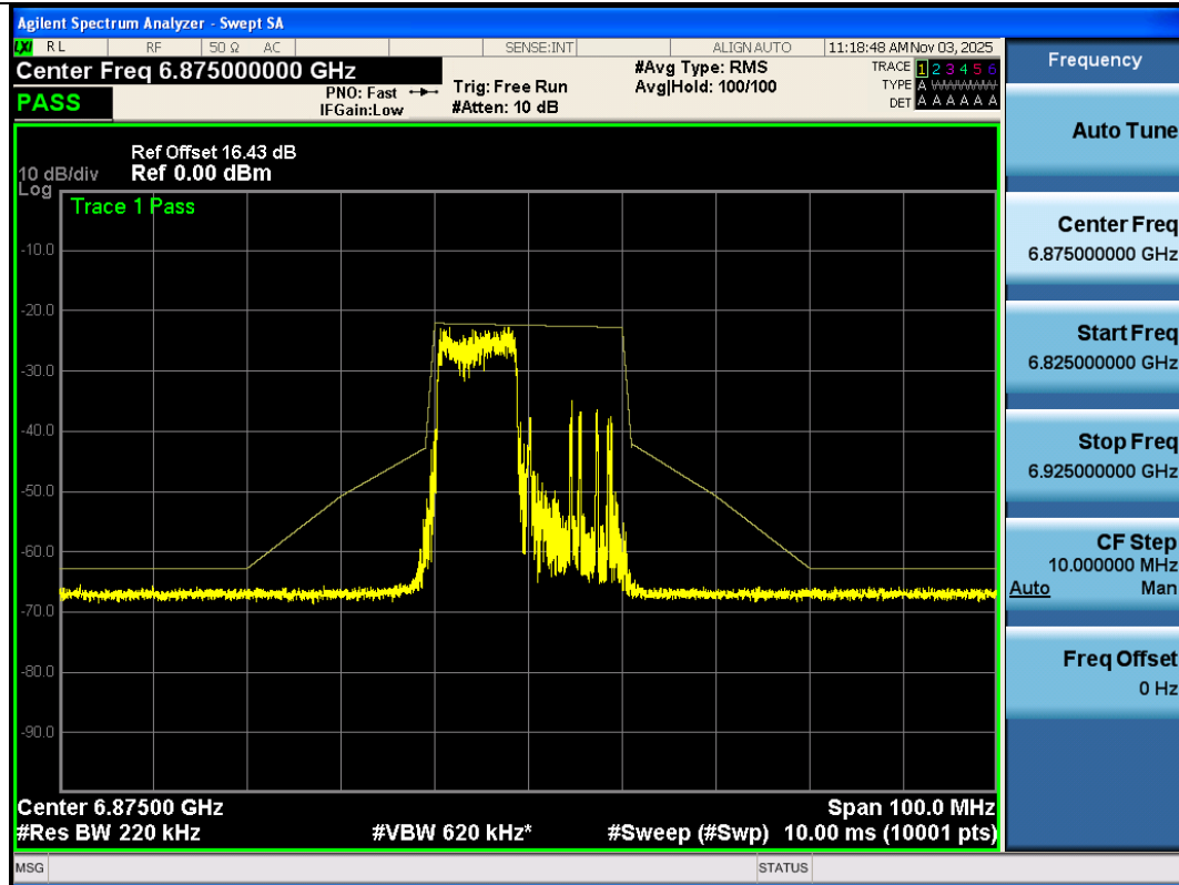
NTNV-11AX20SISO-Ant3-6875-106Tone-RU53-PASS
