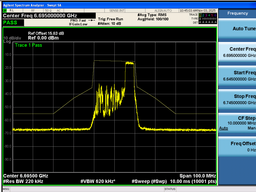
NTNV-11AX20SISO-Ant3-6695-52Tone-RU40-PASS
