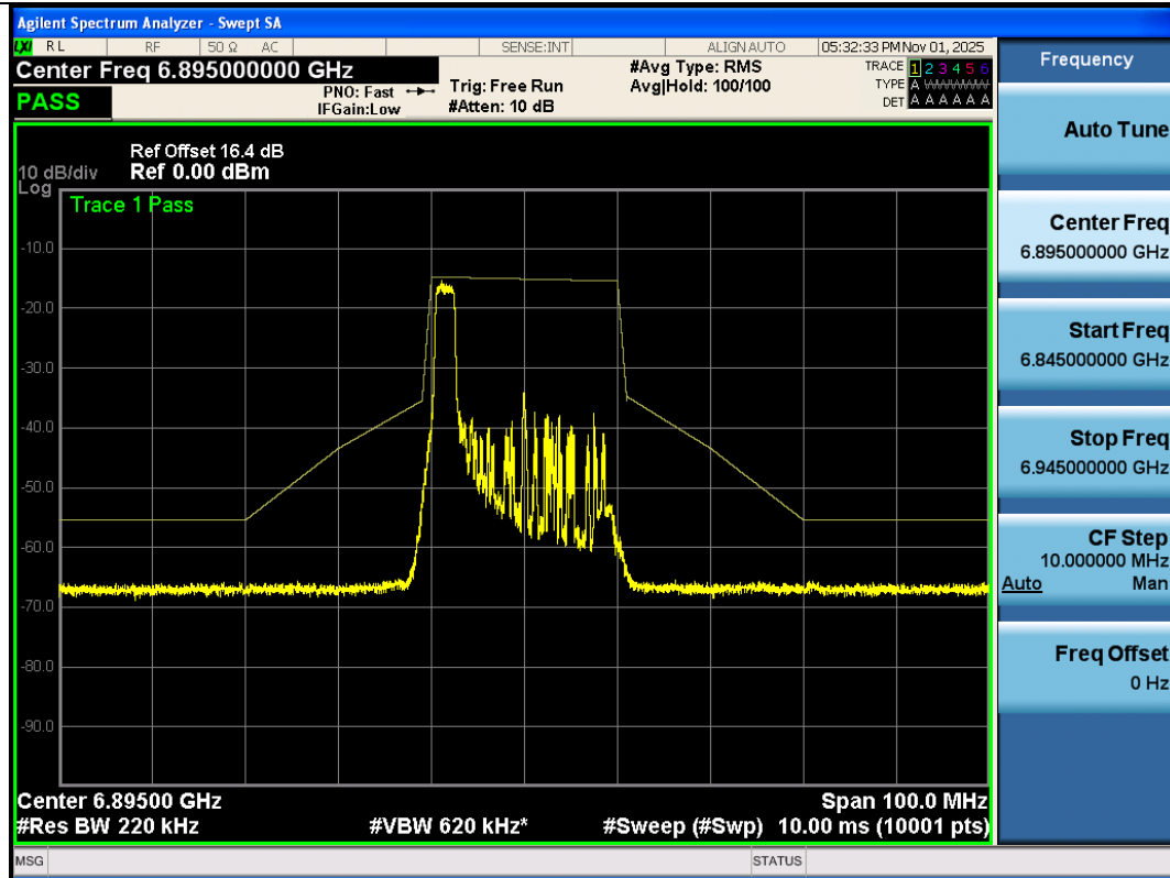
NTNV-11AX20SISO-Ant3-6895-26Tone-RU0-PASS
