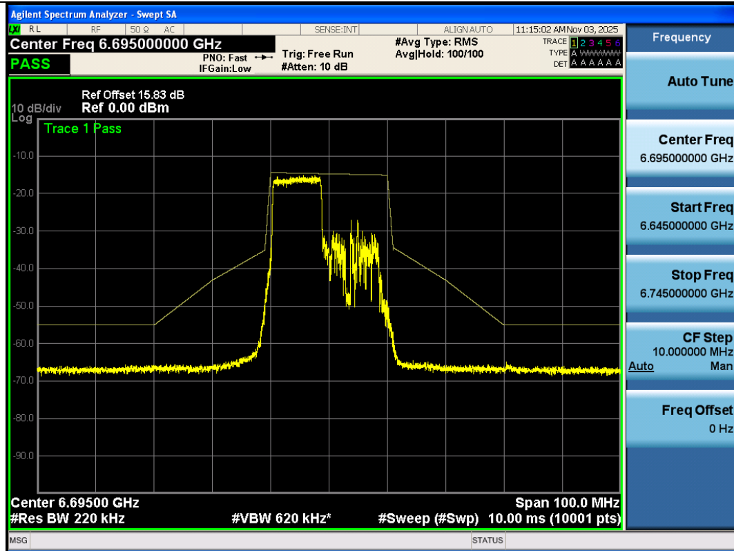
NTNV-11AX20SISO-Ant3-6695-106Tone-RU53-PASS
