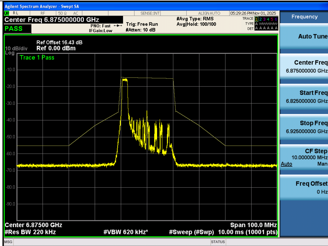
NTNV-11AX20SISO-Ant3-6875-26Tone-RU0-PASS
