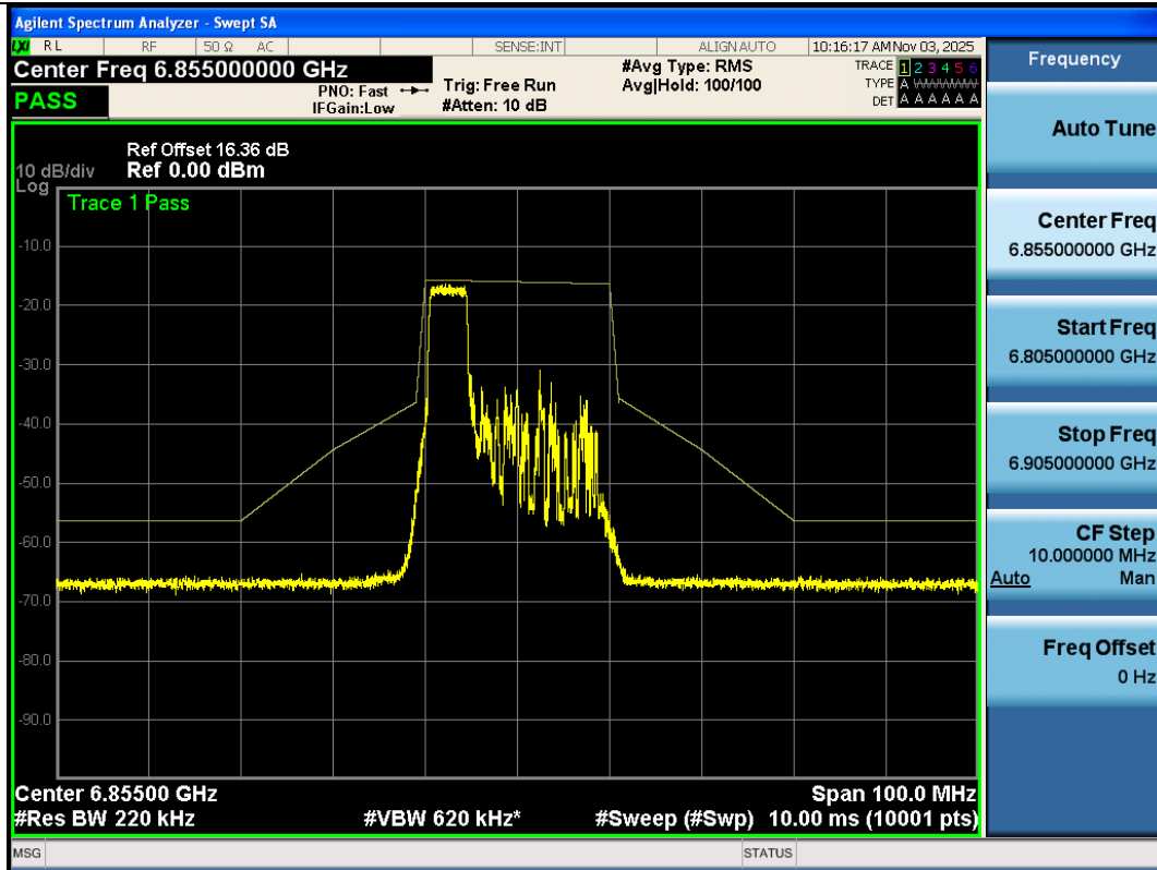
NTNV-11AX20SISO-Ant3-6855-52Tone-RU37-PASS
