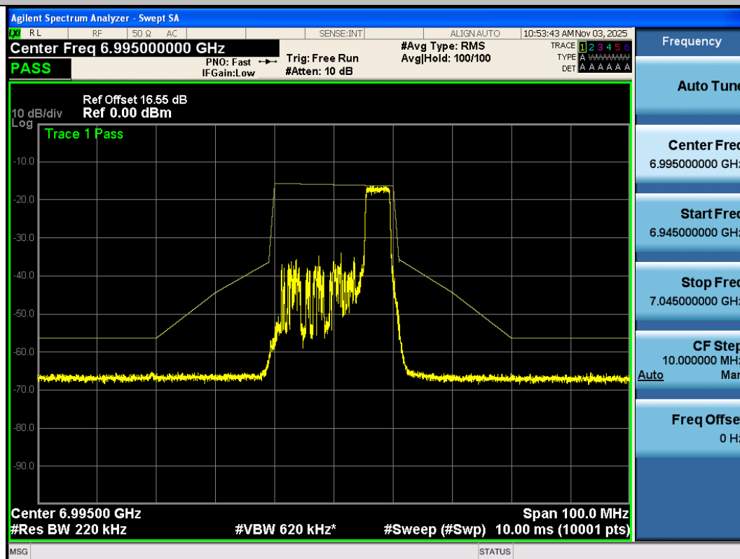
NTNV-11AX20SISO-Ant3-6995-52Tone-RU40-PASS
