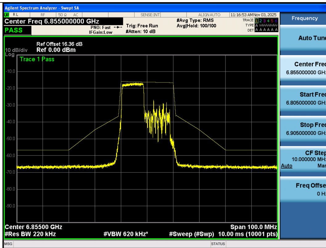
NTNV-11AX20SISO-Ant3-6855-106Tone-RU53-PASS
