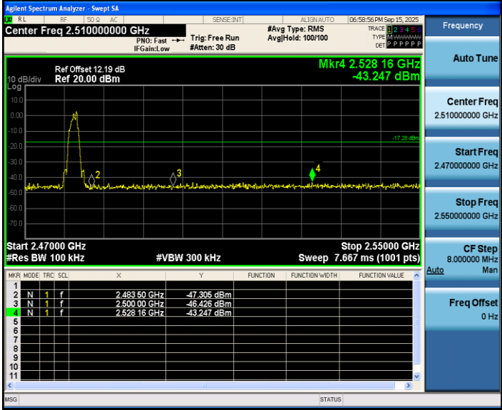
BLE_2M_Ant2_High_2480
