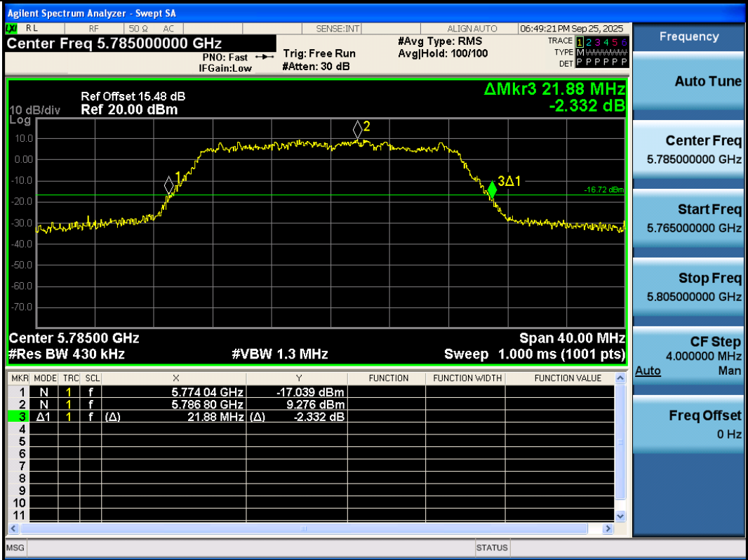
11N20SISO-Ant3-5785
