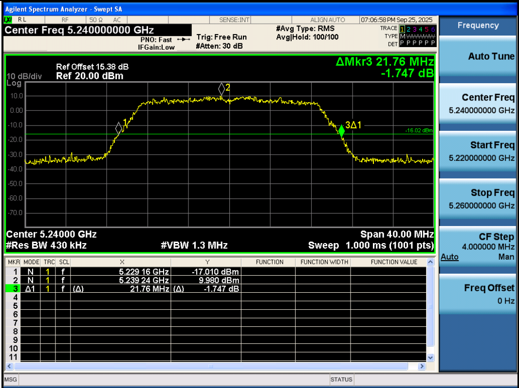
11AC20SISO-Ant3-5240
