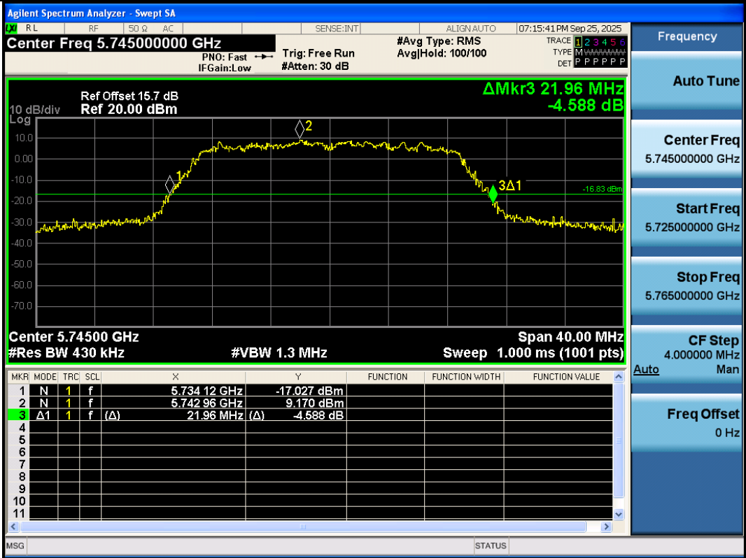
11AC20SISO-Ant3-5745
