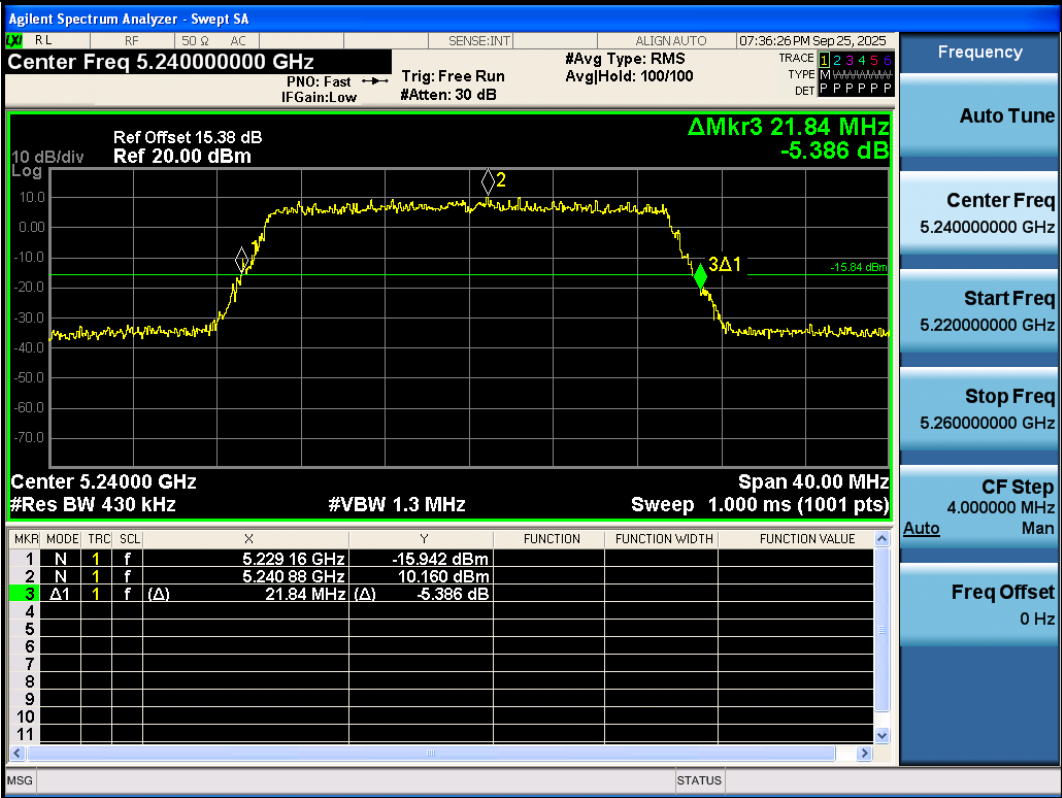
11AX20SISO-Ant3-5240
