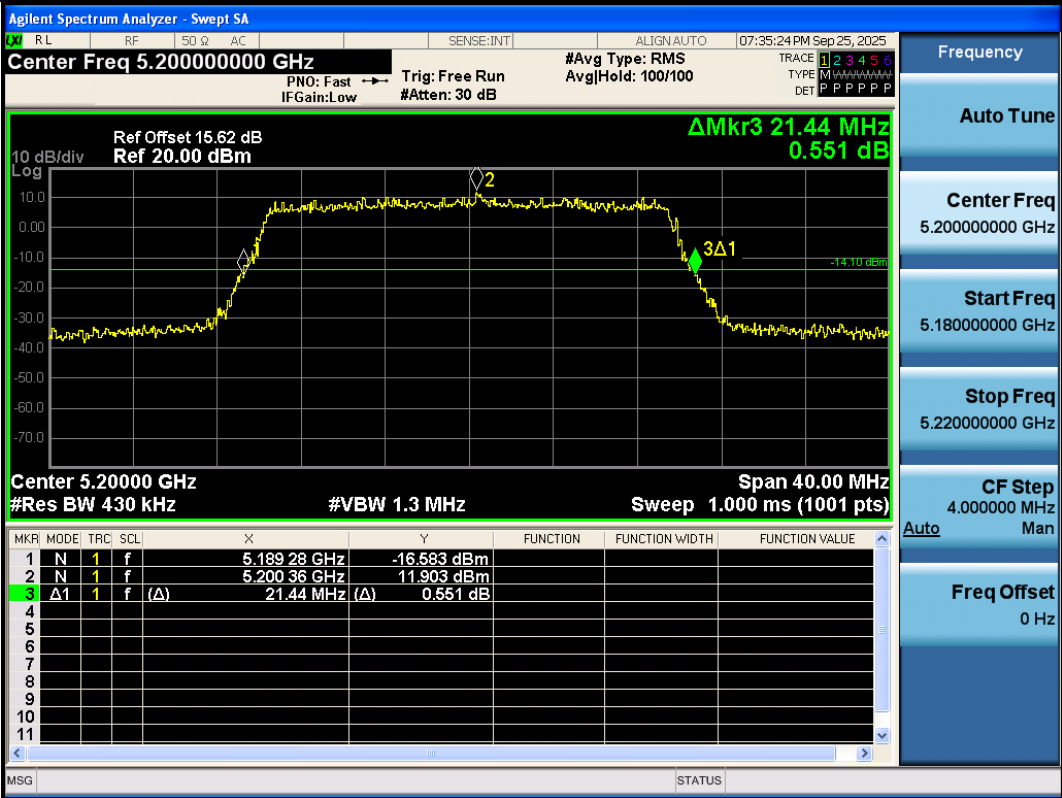
11AX20SISO-Ant3-5200
