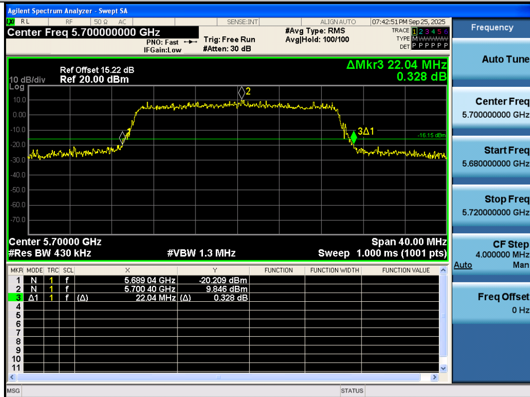
11AX20SISO-Ant3-5700
