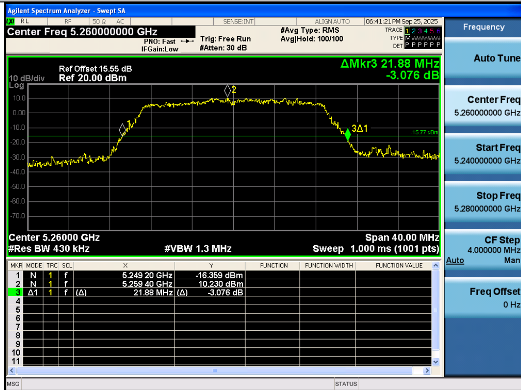
11N20SISO-Ant3-5260
