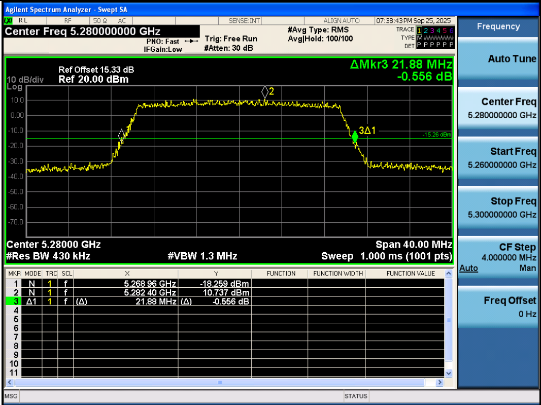
11AX20SISO-Ant3-5280
