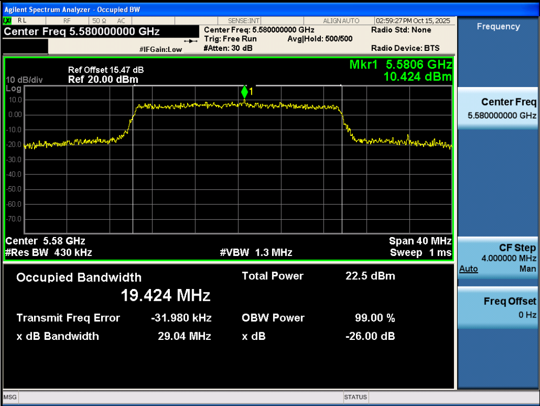
11AX20SISO-Ant3-5580
