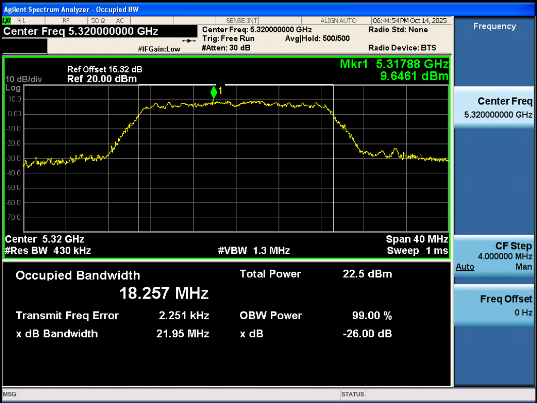
11N20SISO-Ant3-5320
