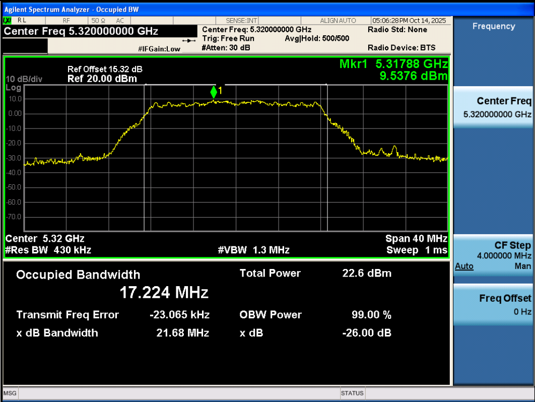
11A-Ant3-5320
