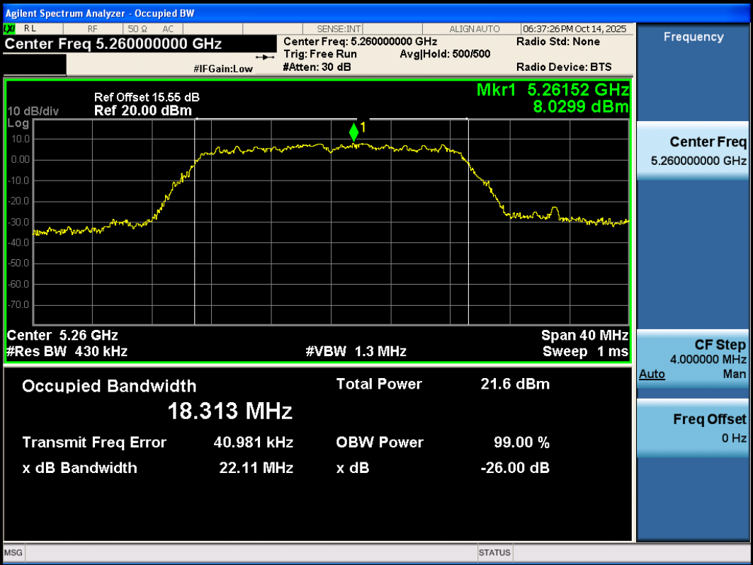
11N20SISO-Ant3-5260
