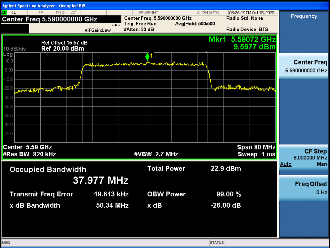
11AX40SISO-Ant3-5590
