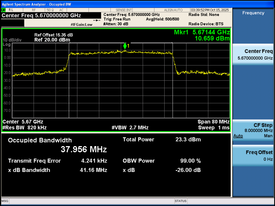
11AX40SISO-Ant3-5670
