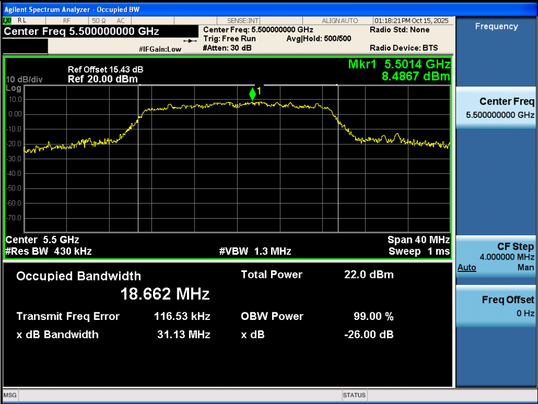
11AC20SISO-Ant3-5500
