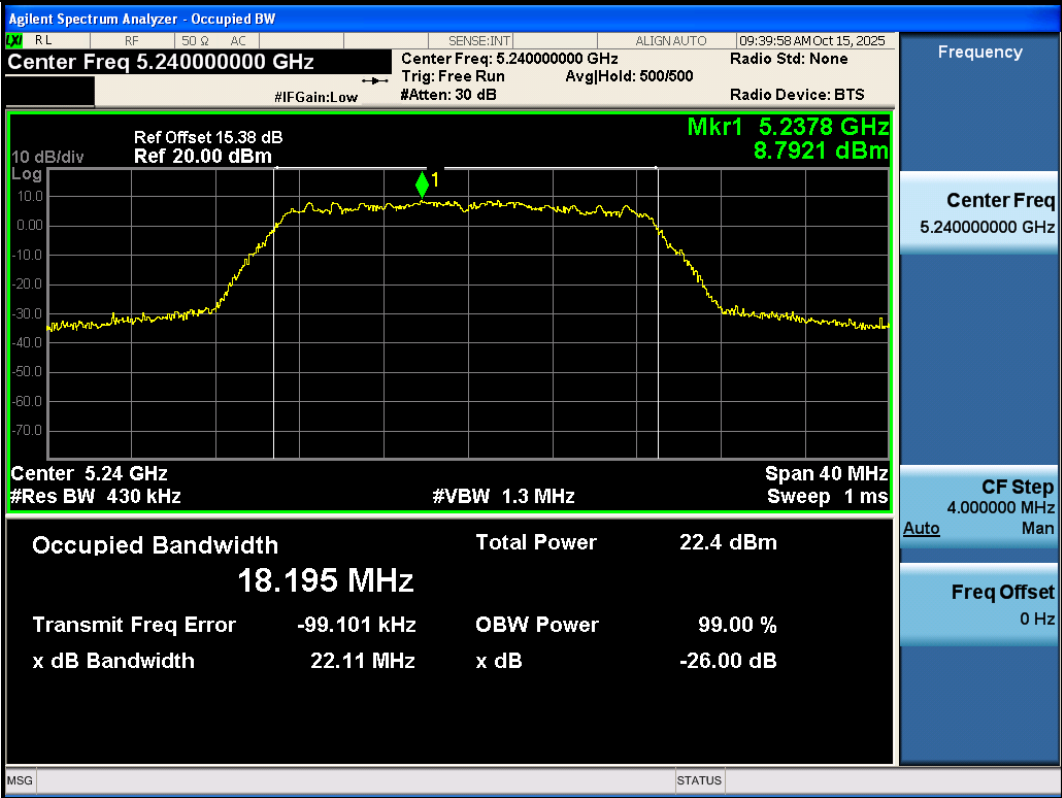
11AC20SISO-Ant3-5240
