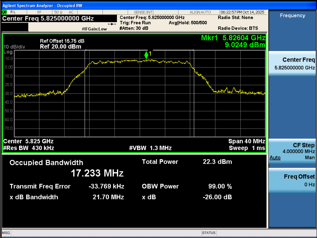
11A-Ant3-5825
