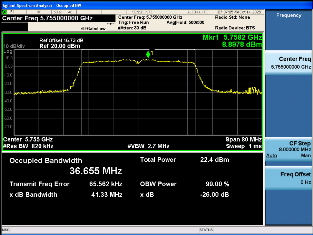
11N40SISO-Ant3-5755
