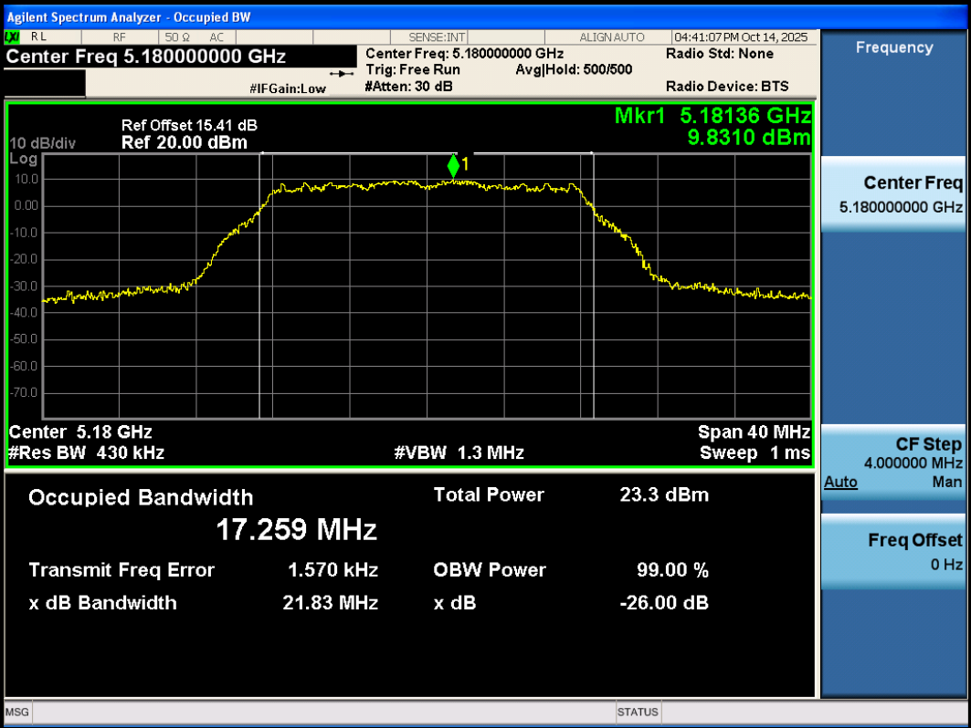
11A-Ant3-5180
