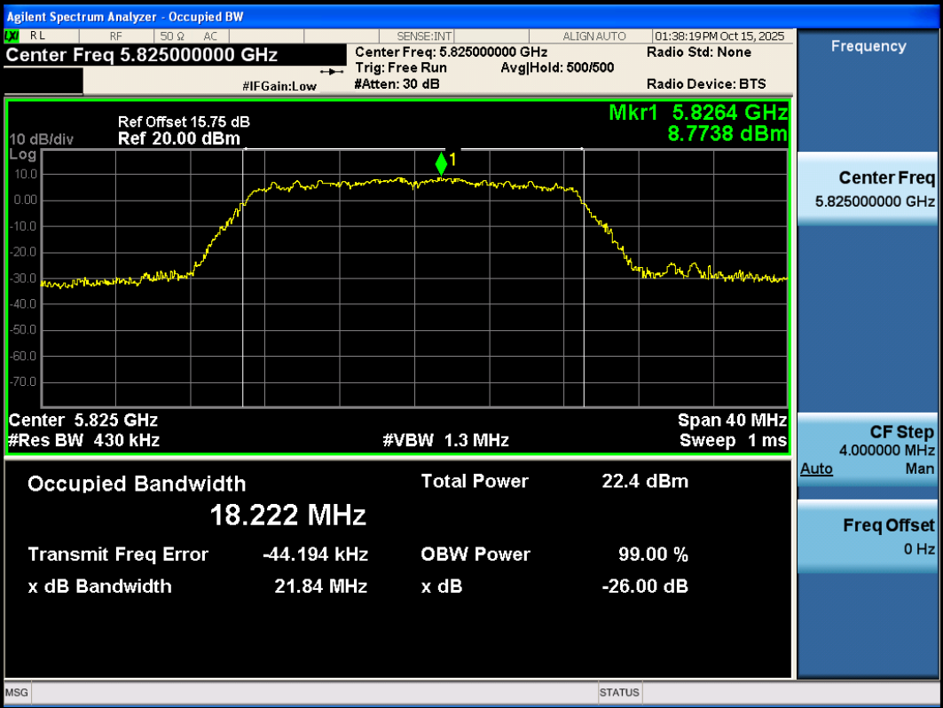
11AC20SISO-Ant3-5825
