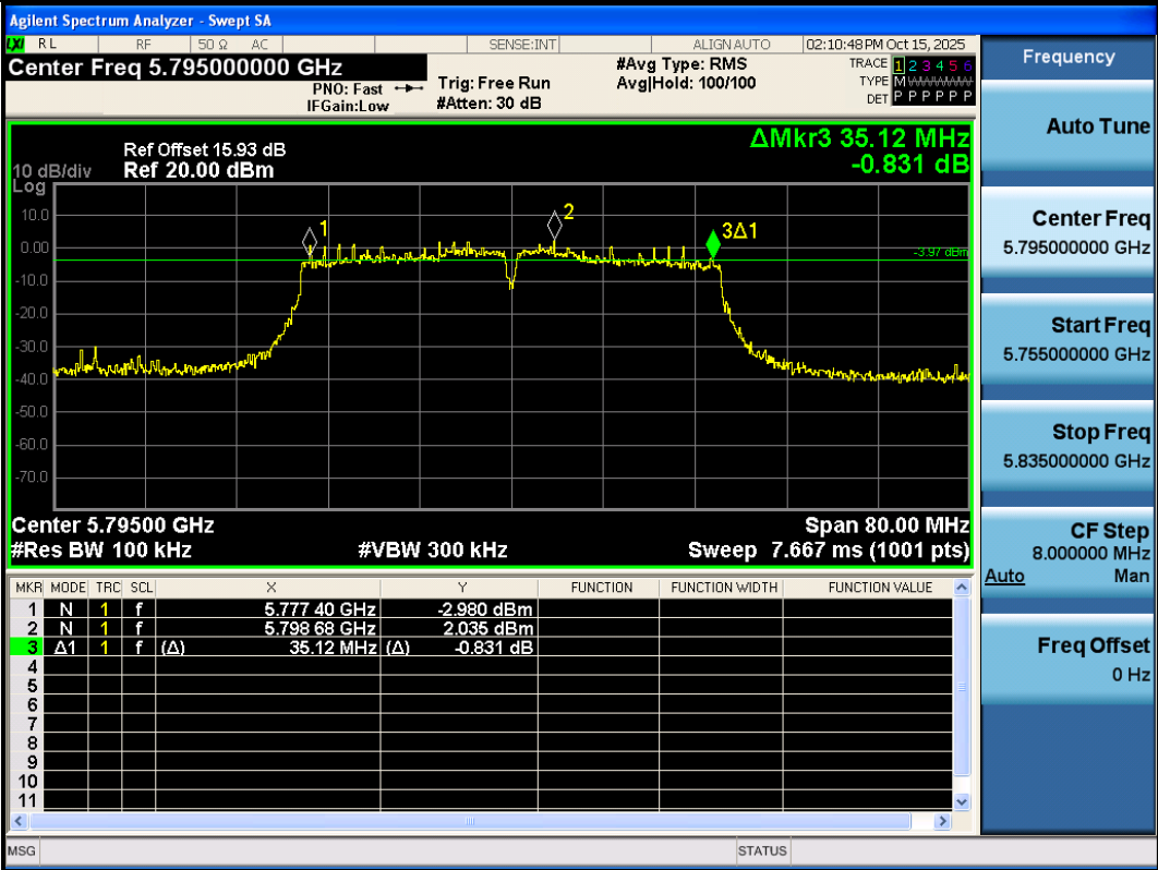
11AC40SISO-Ant3-5795-PASS
