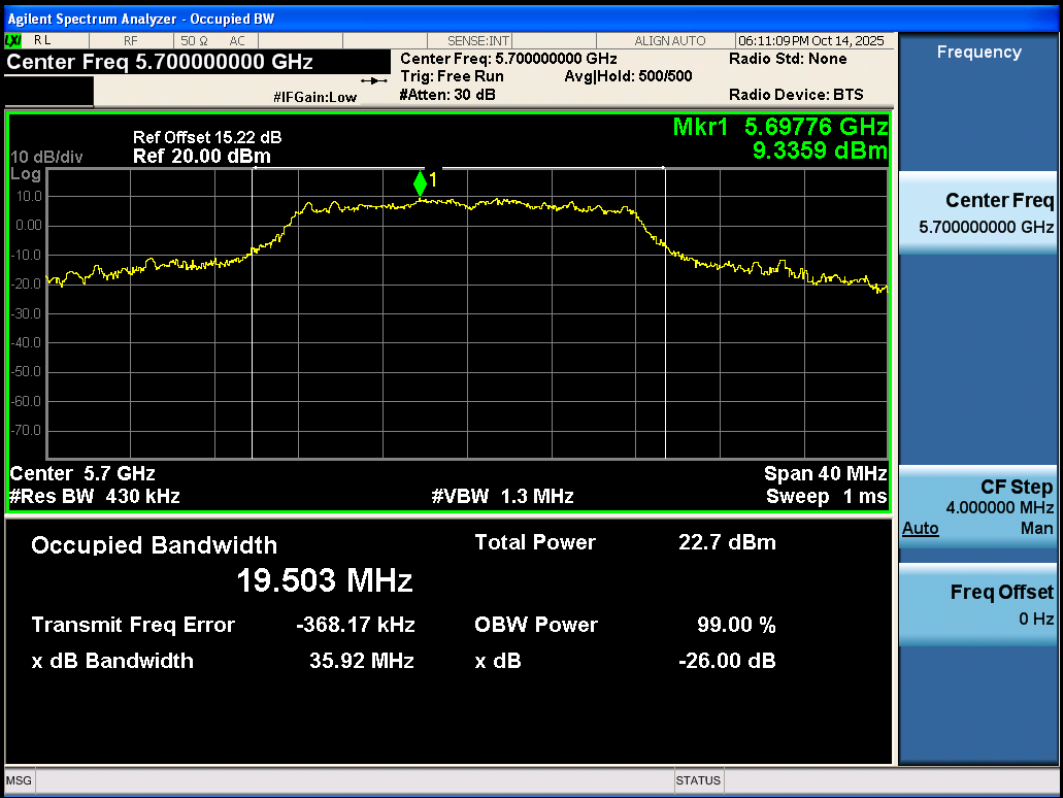
11A-Ant3-5700
