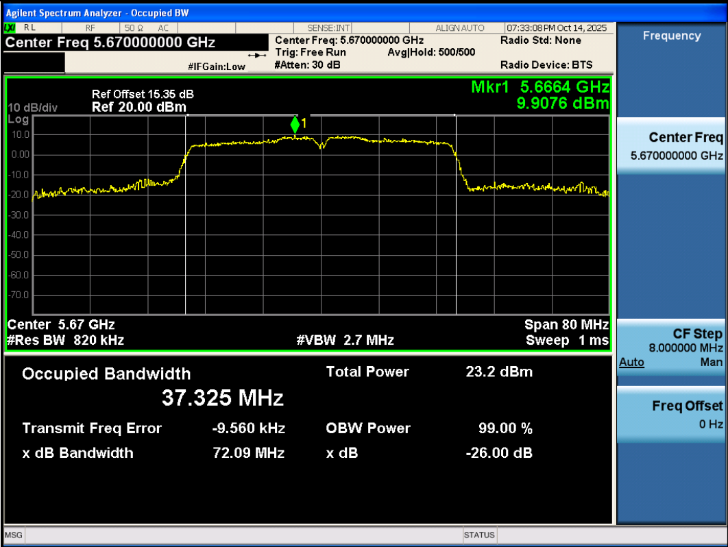
11N40SISO-Ant3-5670
