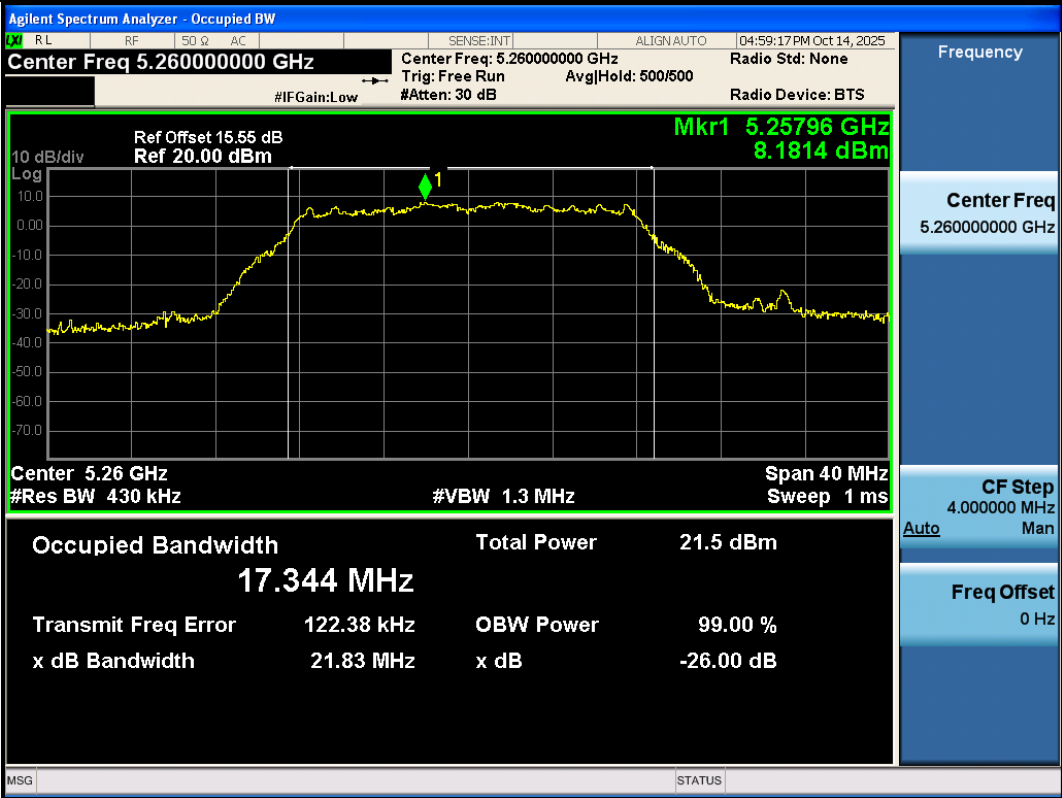
11A-Ant3-5260
