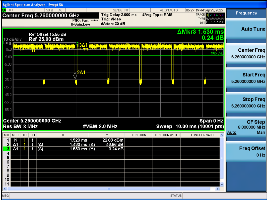
NTNV-11A-Ant3-5260
