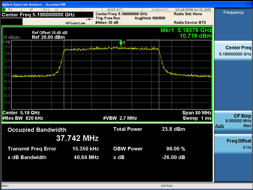
11AX40SISO-Ant3-5190
