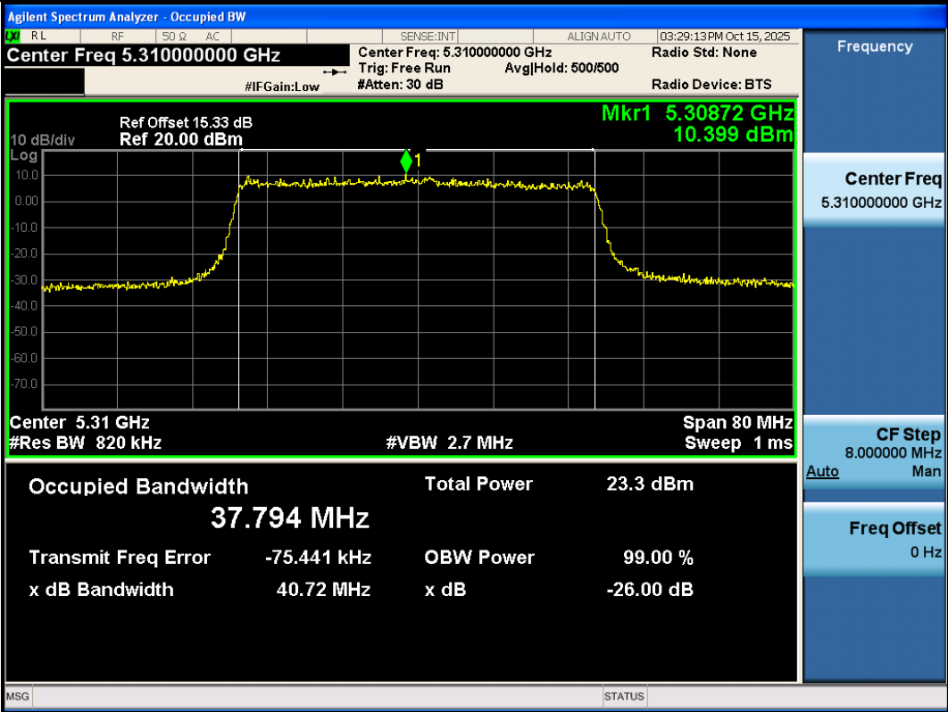
11AX40SISO-Ant3-5310
