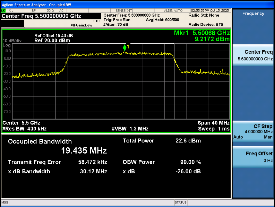
11AX20SISO-Ant3-5500
