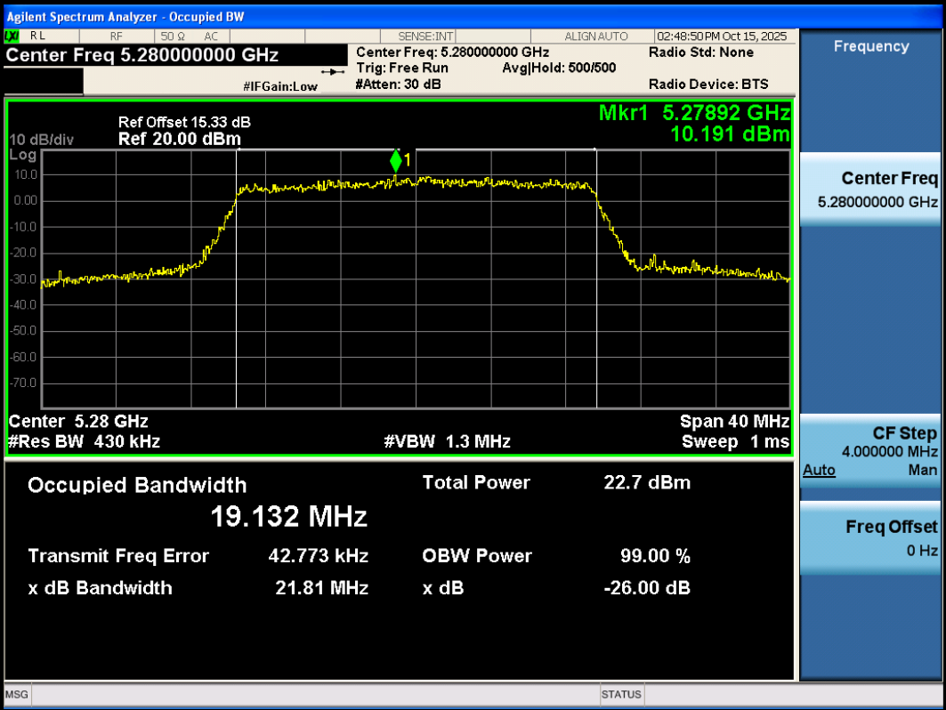
11AX20SISO-Ant3-5280
