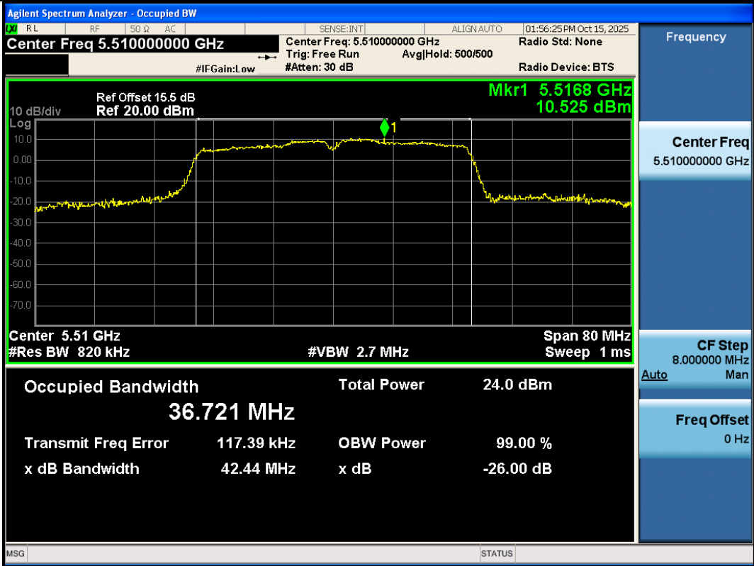
11AC40SISO-Ant3-5510
