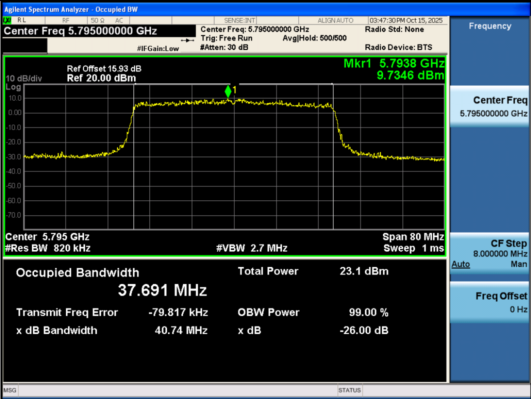
11AX40SISO-Ant3-5795
