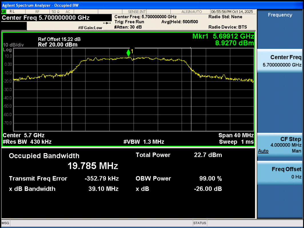
11N20SISO-Ant3-5700
