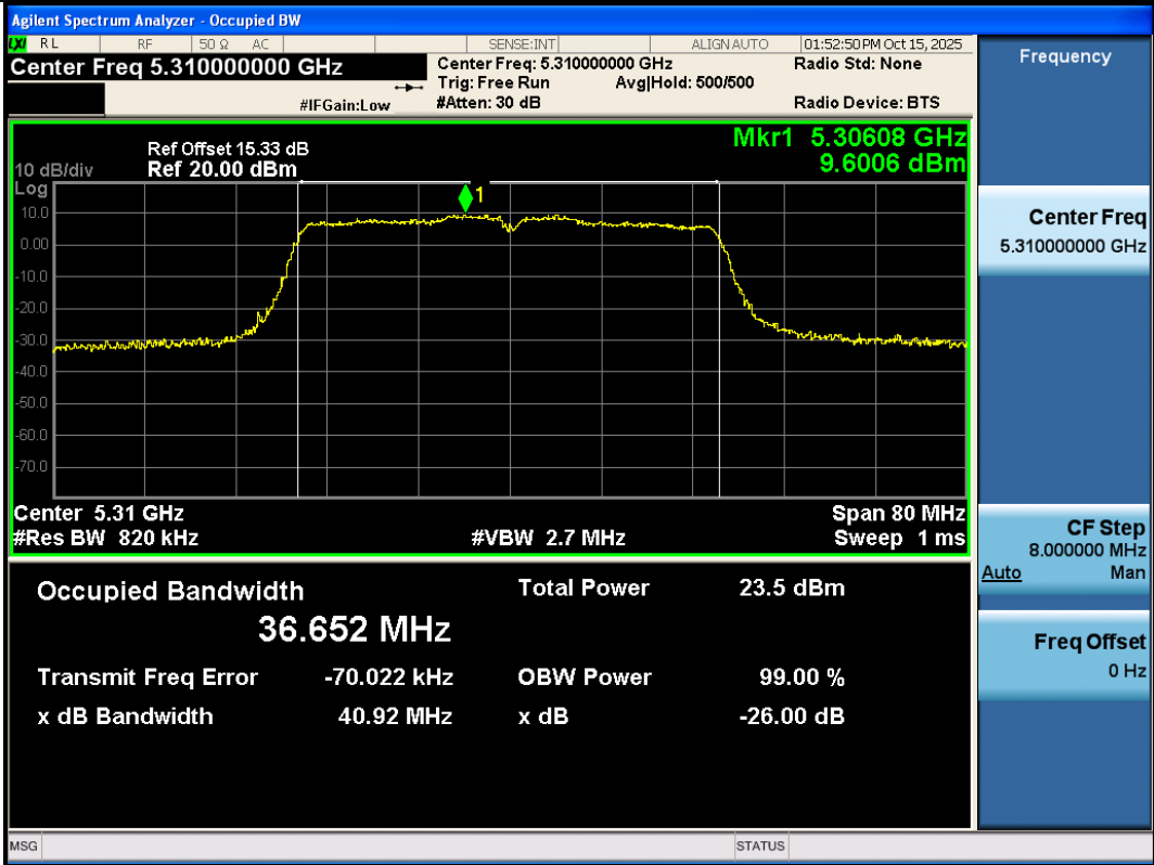
11AC40SISO-Ant3-5310
