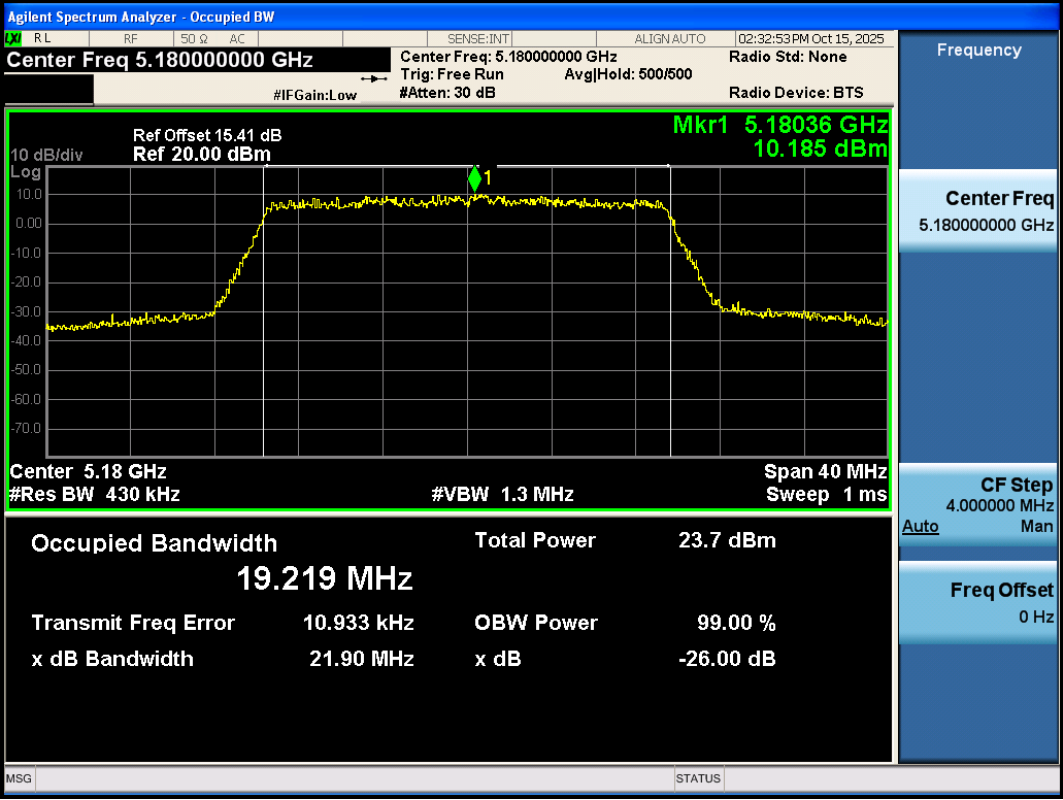
11AX20SISO-Ant3-5180
