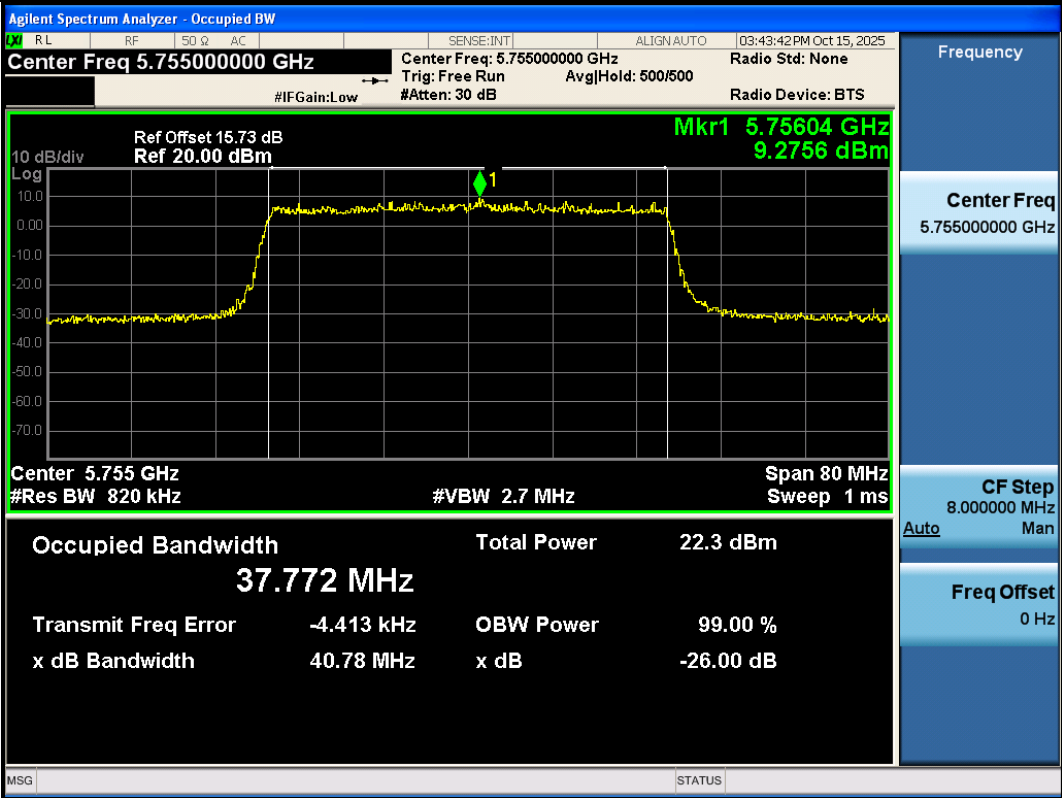
11AX40SISO-Ant3-5755
