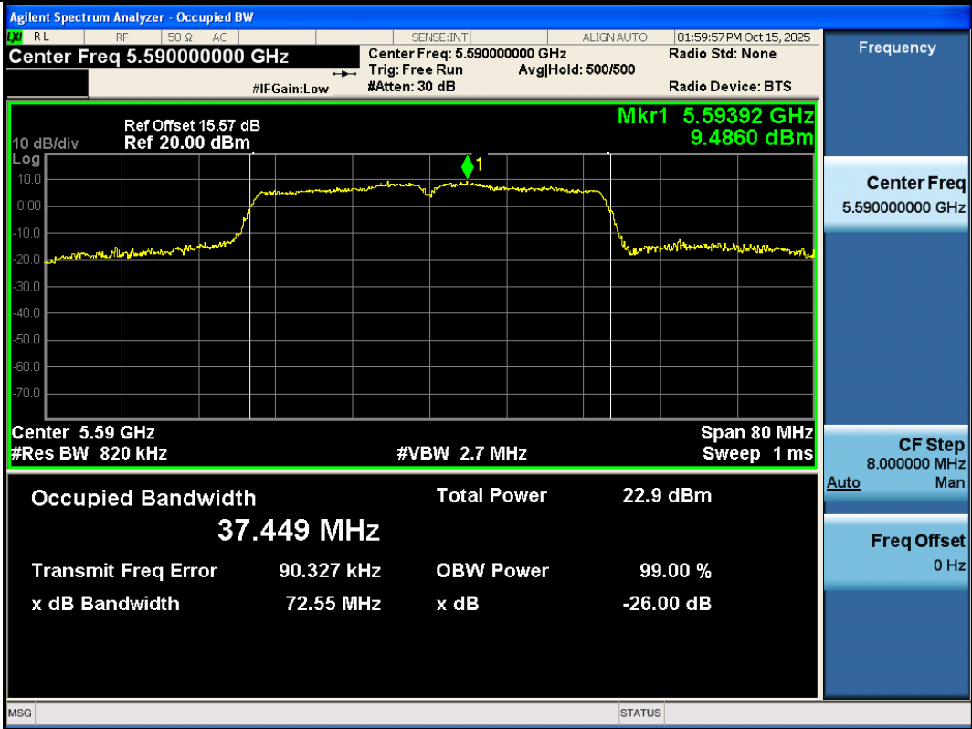
11AC40SISO-Ant3-5590
