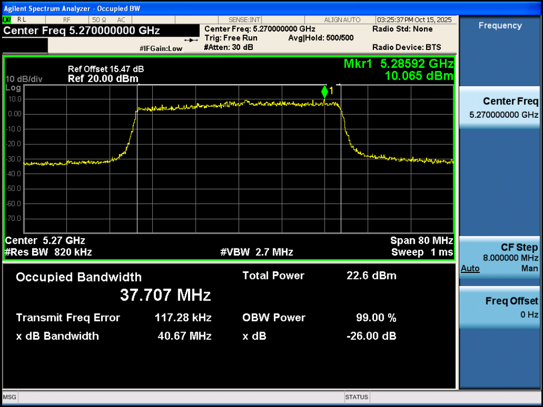
11AX40SISO-Ant3-5270
