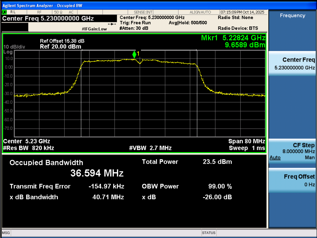
11N40SISO-Ant3-5230
