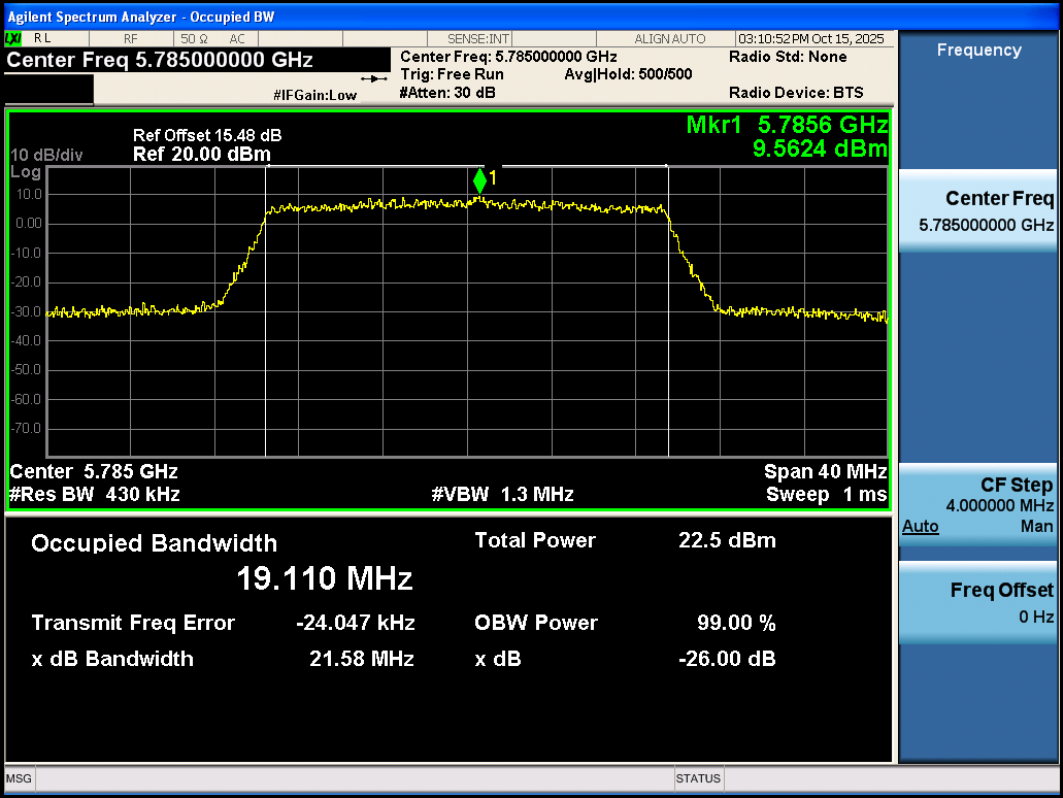
11AX20SISO-Ant3-5785
