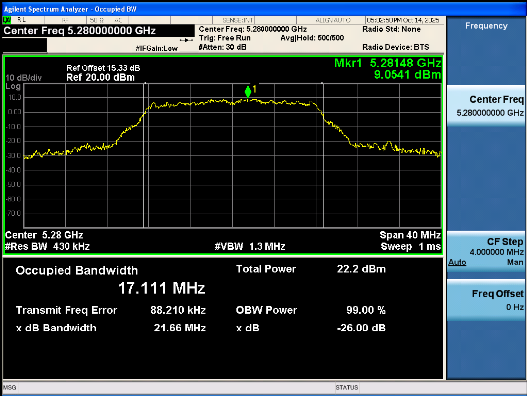
11A-Ant3-5280
