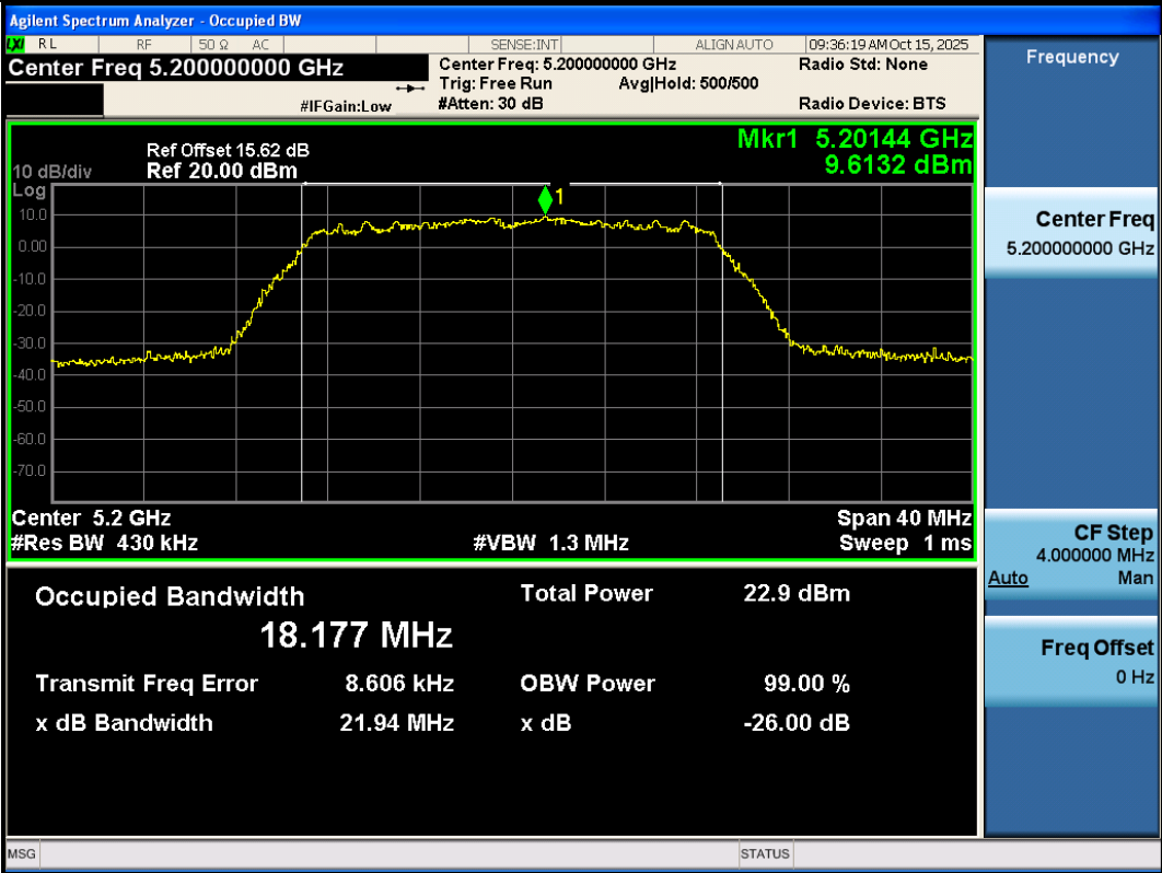
11AC20SISO-Ant3-5200
