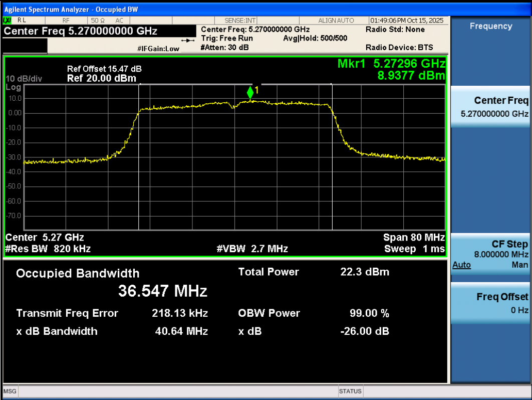
11AC40SISO-Ant3-5270
