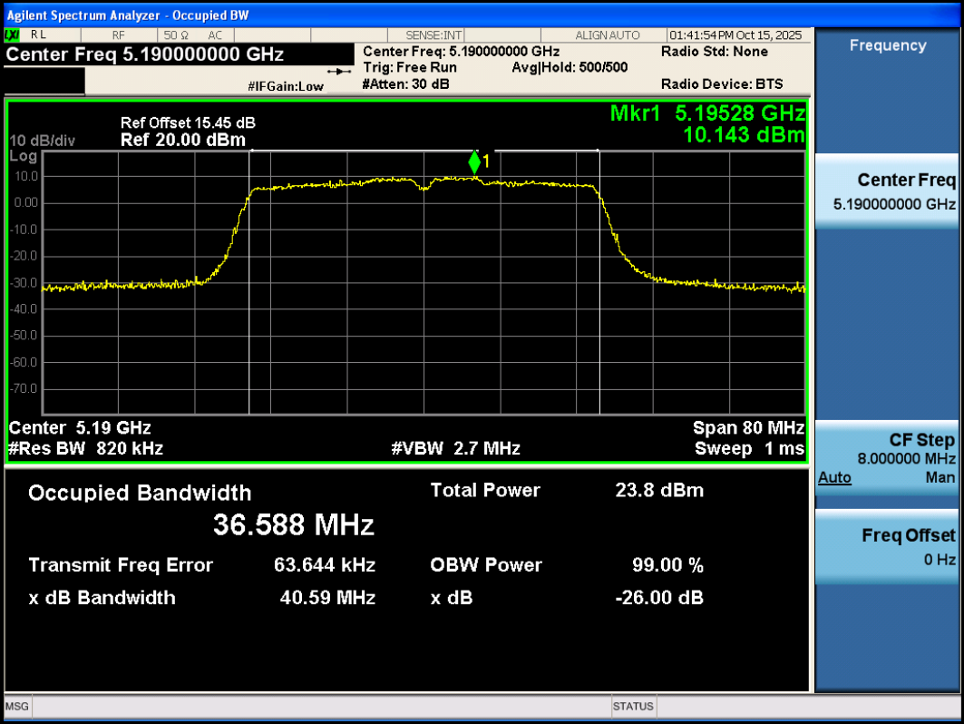
11AC40SISO-Ant3-5190
