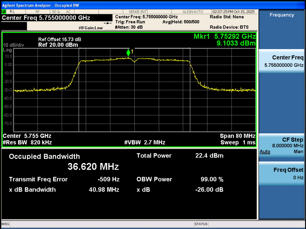
11AC40SISO-Ant3-5755
