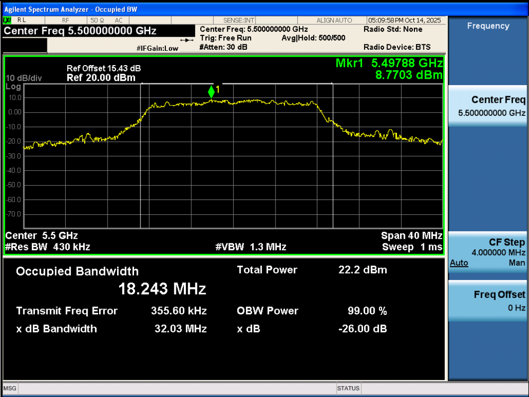
11A-Ant3-5500
