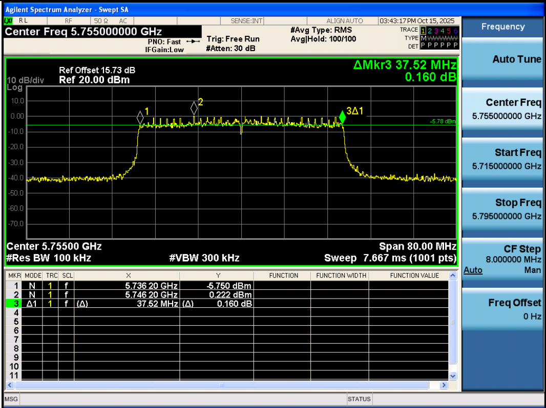
11AX40SISO-Ant3-5755-PASS
