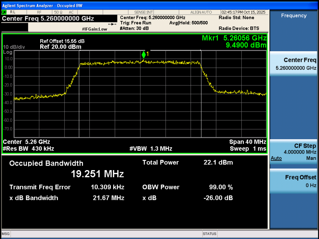
11AX20SISO-Ant3-5260
