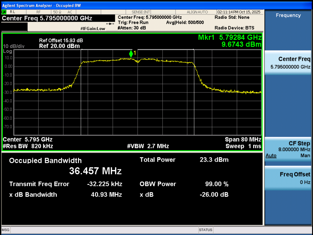
11AC40SISO-Ant3-5795
