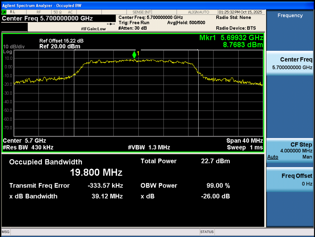
11AC20SISO-Ant3-5700
