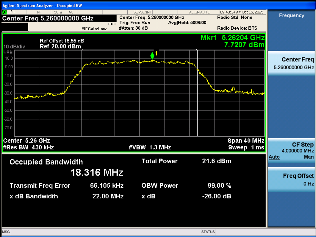
11AC20SISO-Ant3-5260
