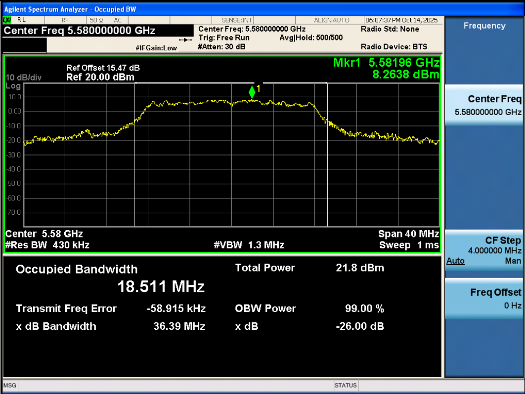
11A-Ant3-5580
