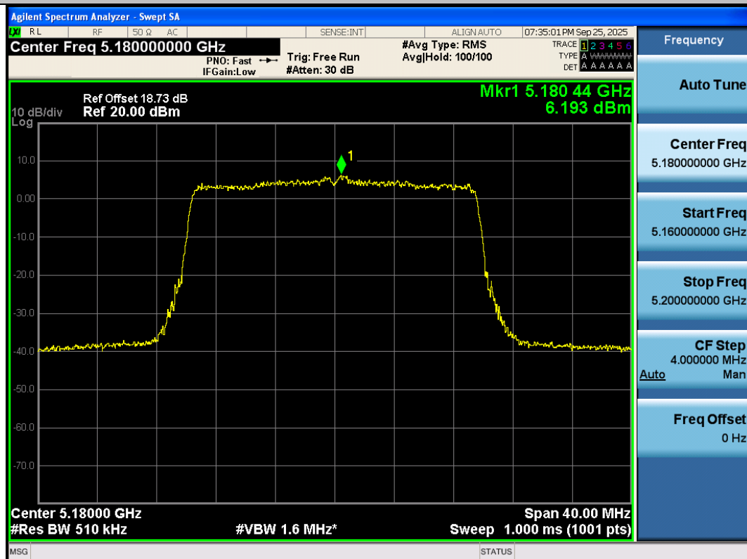
11AX20SISO-Ant3-5180-PASS
