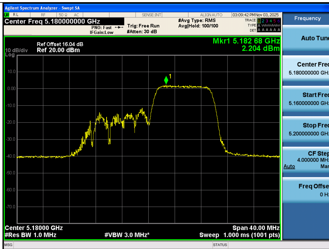
11AX20SISO-Ant3-5180-106Tone-RU54-PASS
