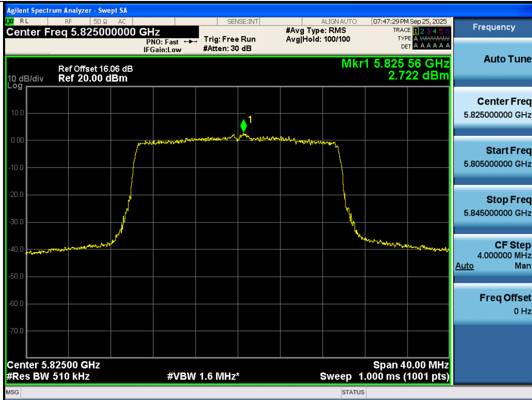
11AX20SISO-Ant3-5825-PASS
