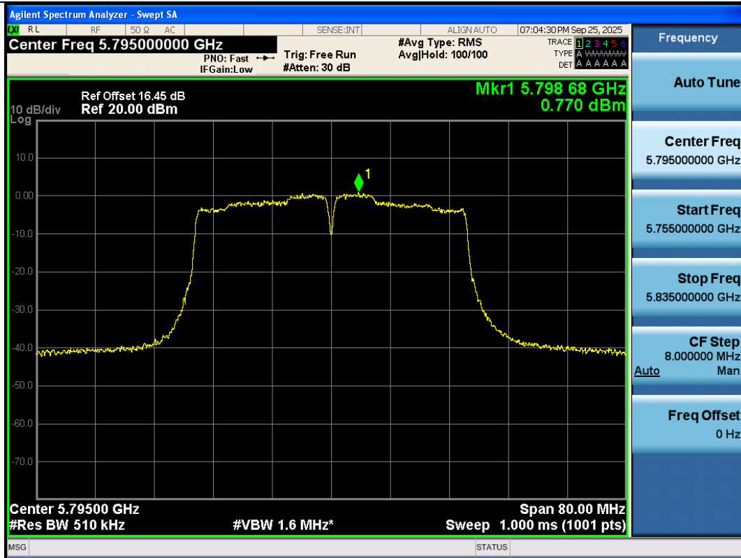
11N40SISO-Ant3-5795-PASS
