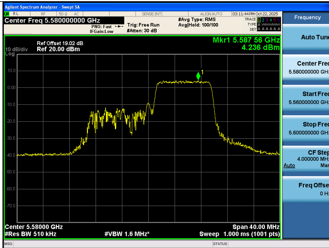
11AX20SISO-Ant3-5580-106Tone-RU54-PASS
