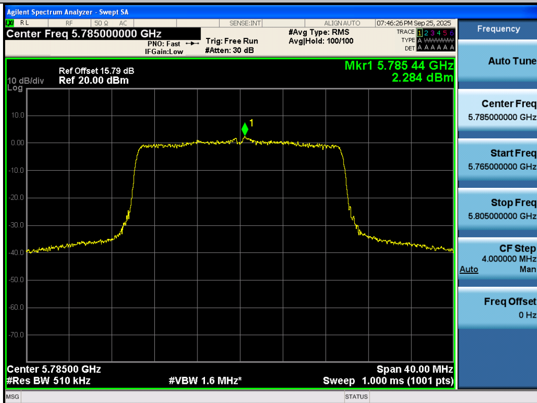
11AX20SISO-Ant3-5785-PASS
