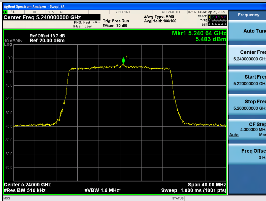
11AX20SISO-Ant3-5240-PASS
