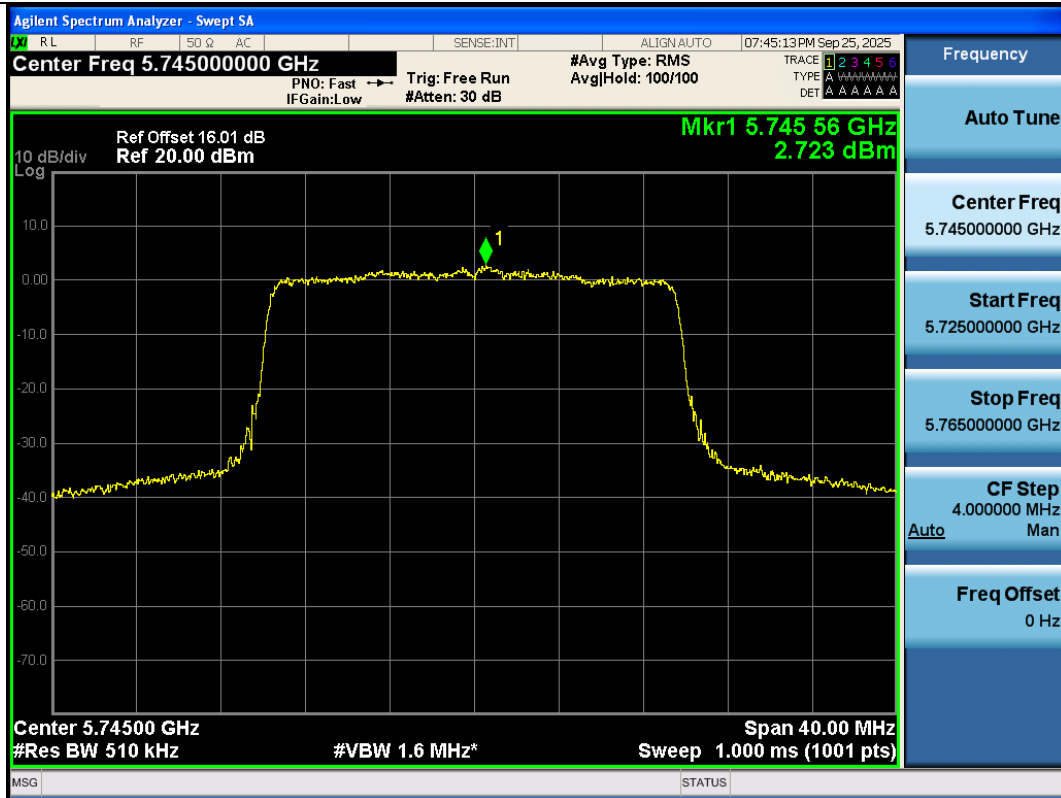
11AX20SISO-Ant3-5745-PASS
