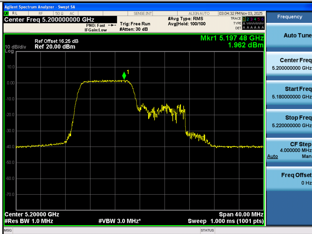
11AX20SISO-Ant3-5200-106Tone-RU53-PASS
