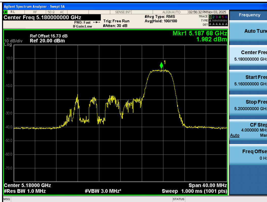
11AX20SISO-Ant3-5180-52Tone-RU40-PASS
