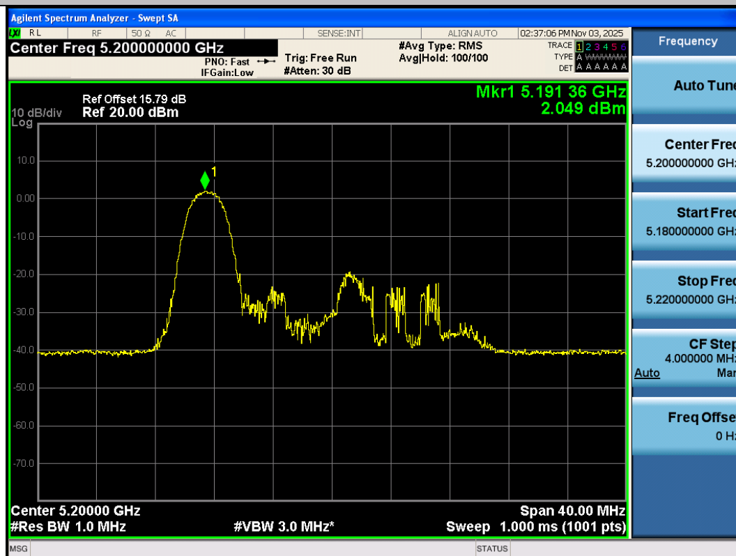
11AX20SISO-Ant3-5200-26Tone-RU0-PASS
