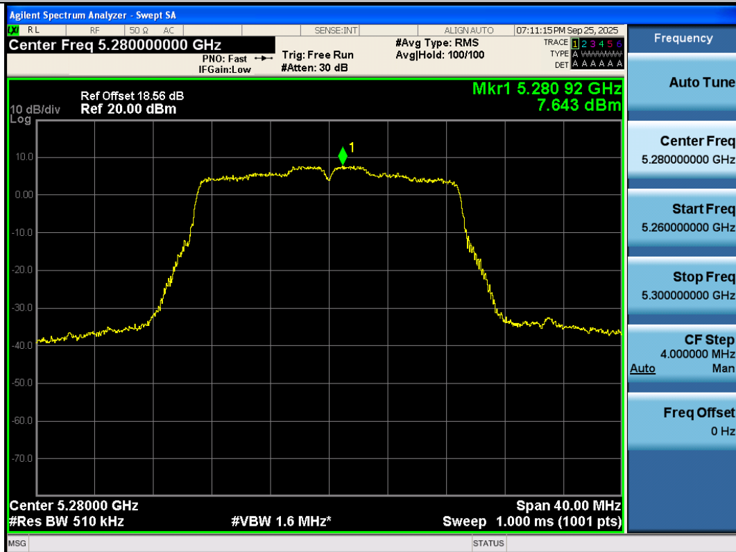
11AC20SISO-Ant3-5280-PASS
