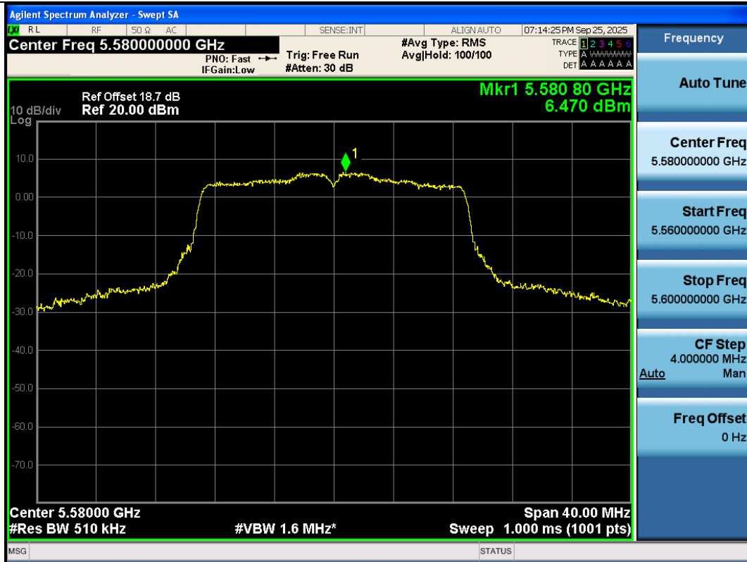
11AC20SISO-Ant3-5580-PASS
