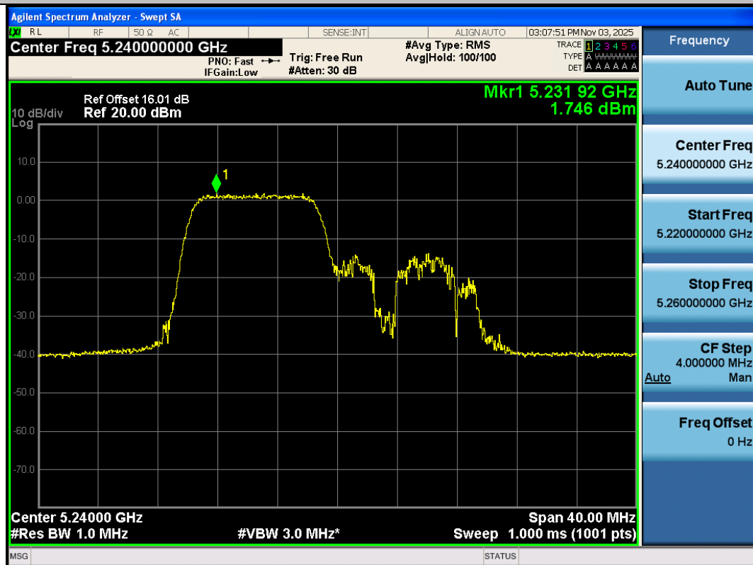
11AX20SISO-Ant3-5240-106Tone-RU53-PASS
