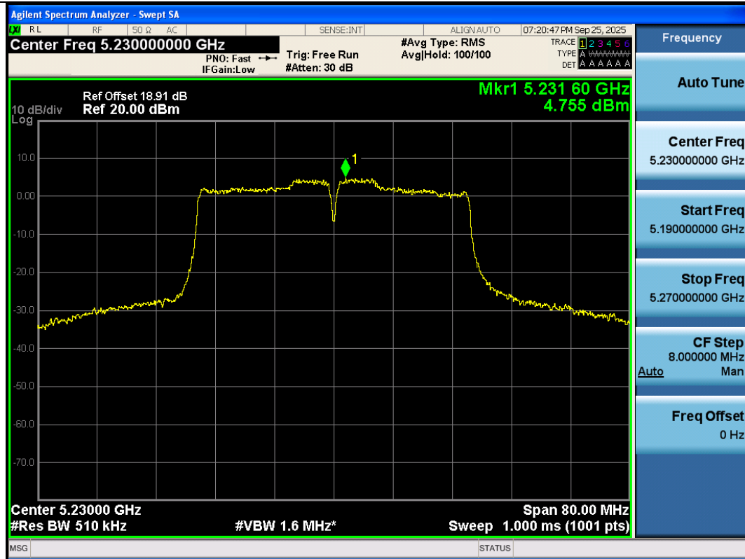
11AC40SISO-Ant3-5230-PASS
