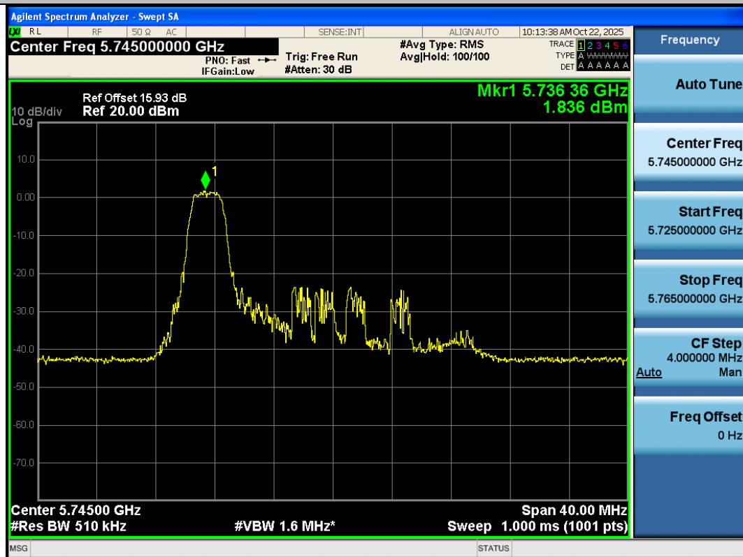
11AX20SISO-Ant3-5745-26Tone-RU0-PASS
