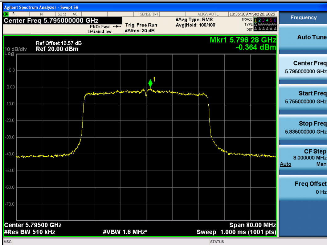
11AX40SISO-Ant3-5795-PASS
