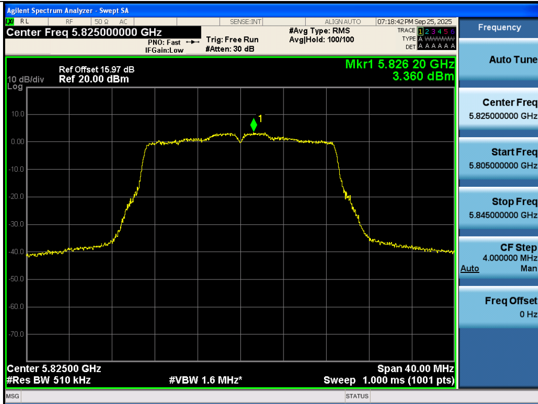
11AC20SISO-Ant3-5825-PASS
