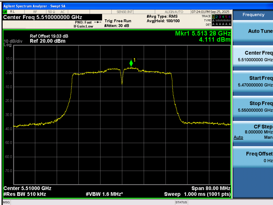
11AC40SISO-Ant3-5510-PASS
