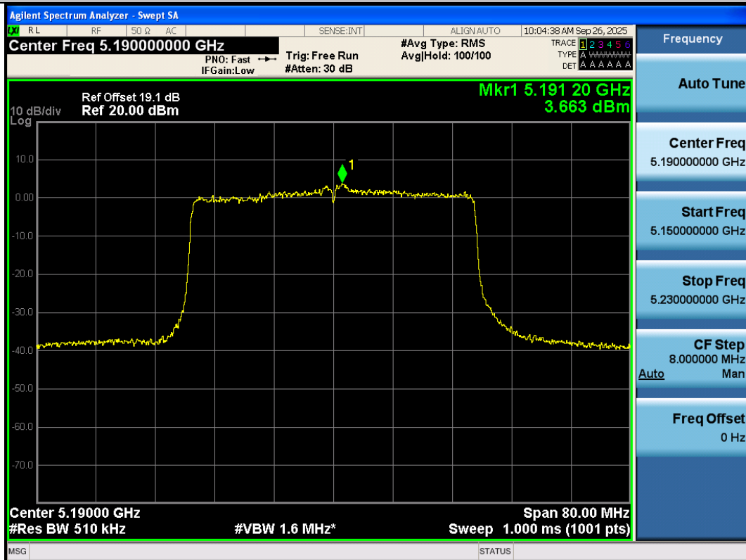
11AX40SISO-Ant3-5190-PASS
