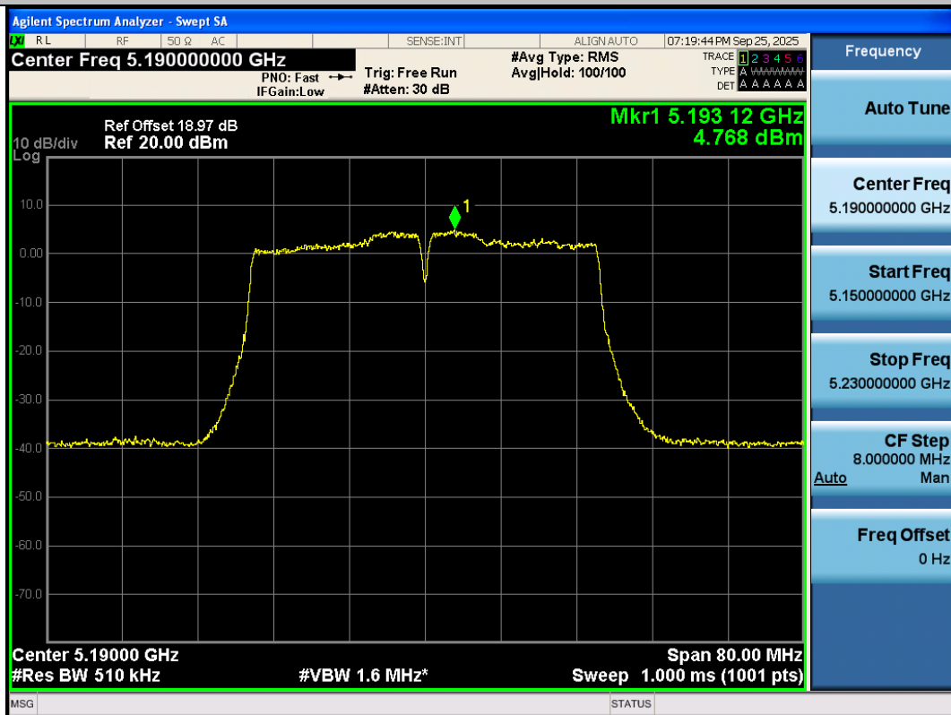
11AC40SISO-Ant3-5190-PASS
