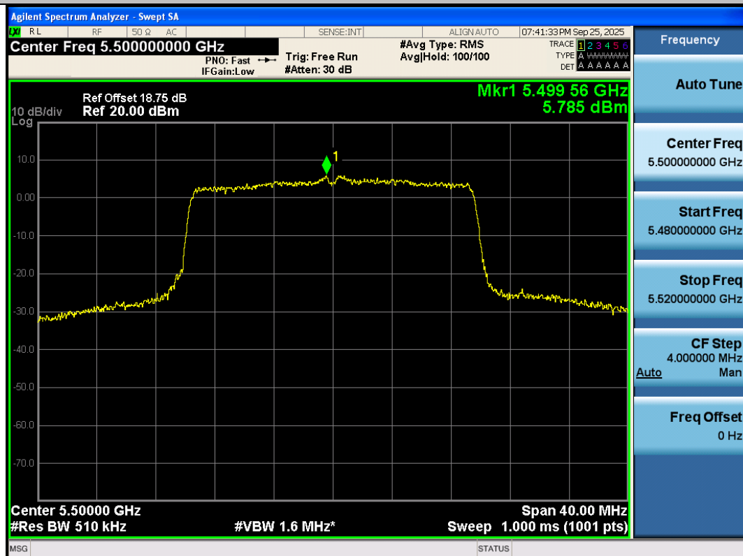
11AX20SISO-Ant3-5500-PASS
