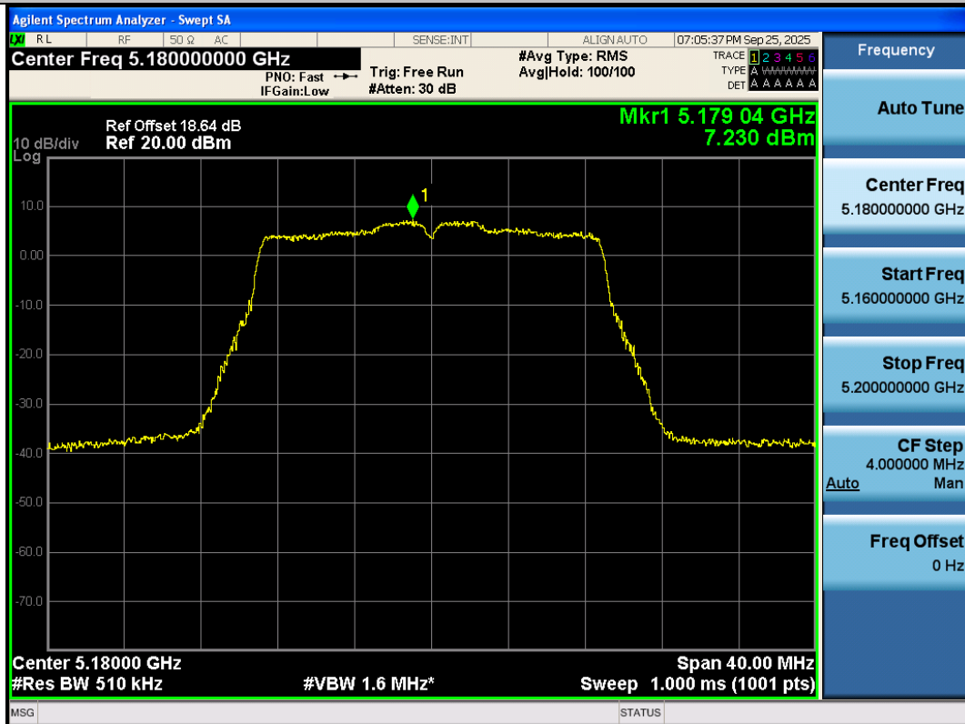
11AC20SISO-Ant3-5180-PASS
