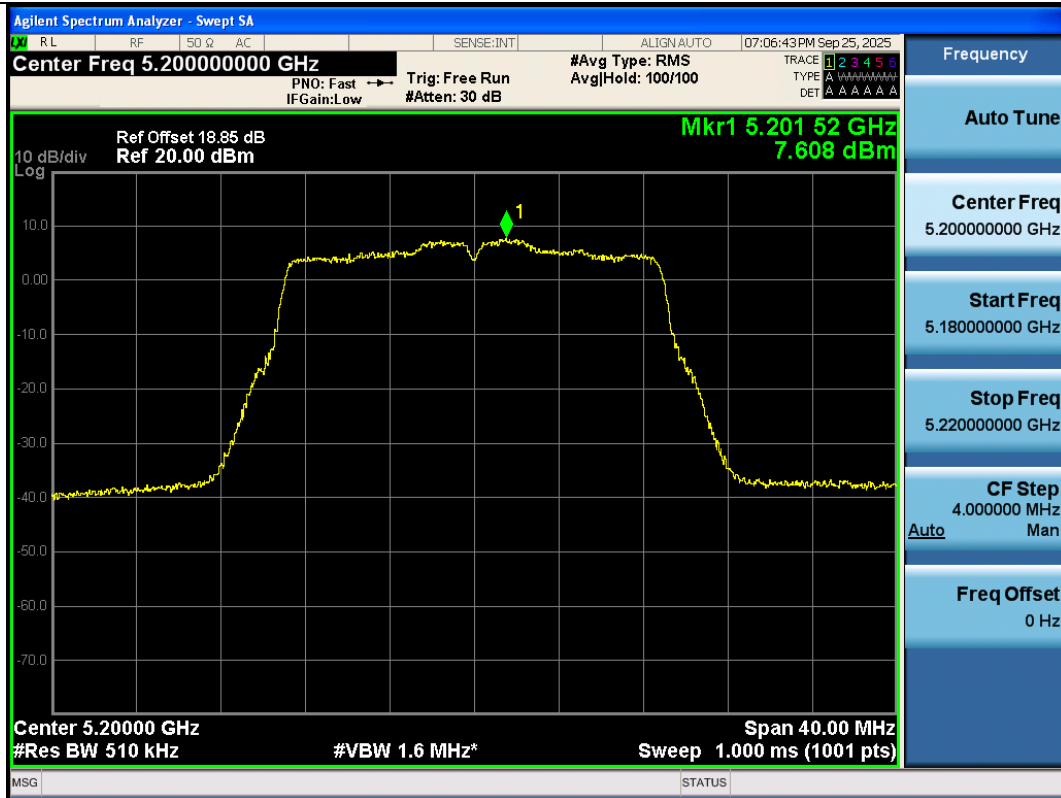
11AC20SISO-Ant3-5200-PASS
