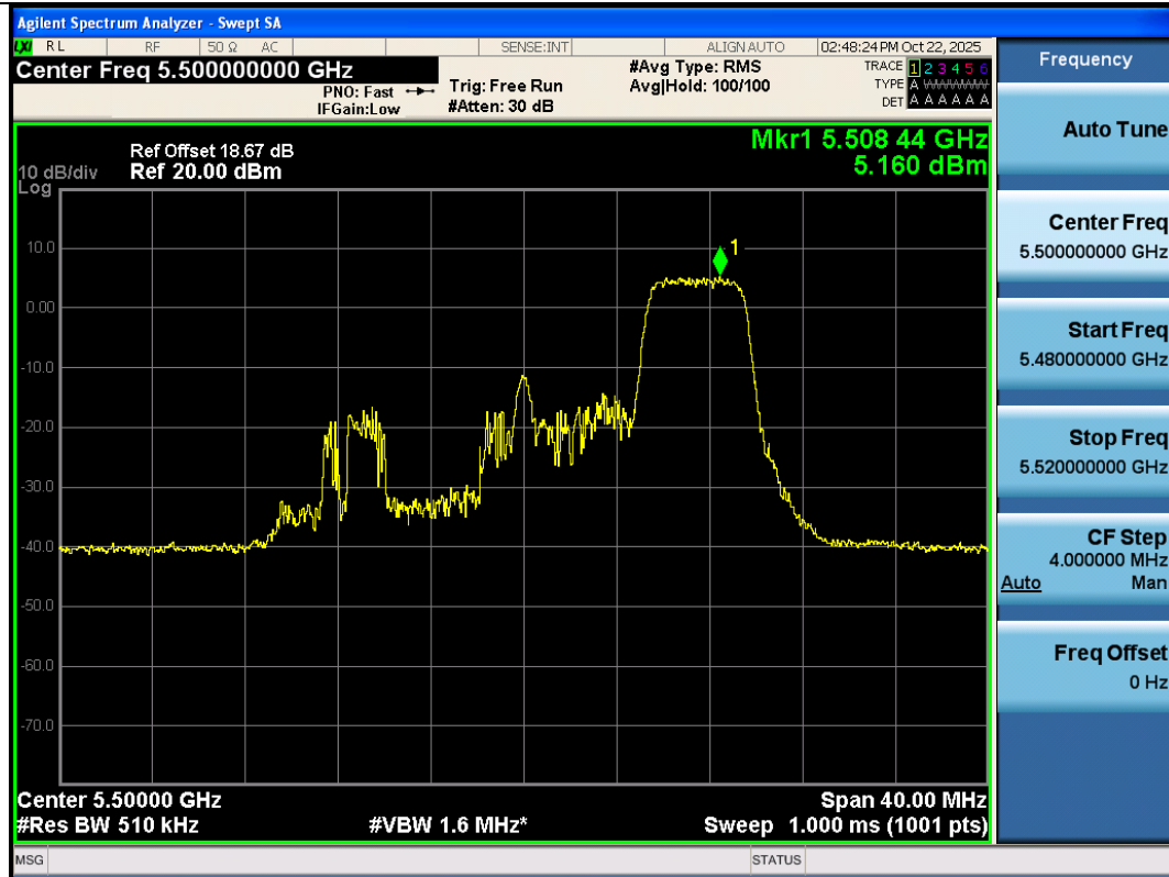
11AX20SISO-Ant3-5500-52Tone-RU40-PASS
