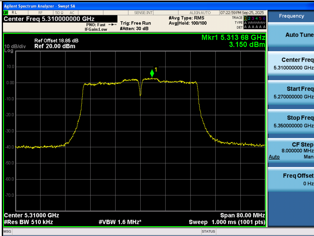
11AC40SISO-Ant3-5310-PASS
