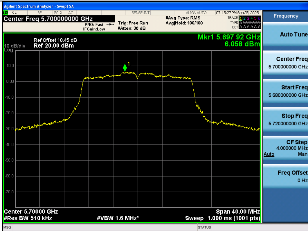
11AC20SISO-Ant3-5700-PASS
