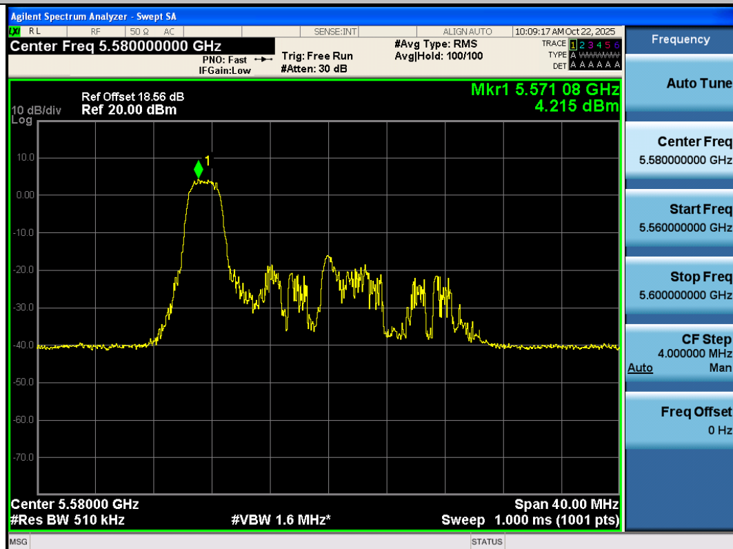
11AX20SISO-Ant3-5580-26Tone-RU0-PASS
