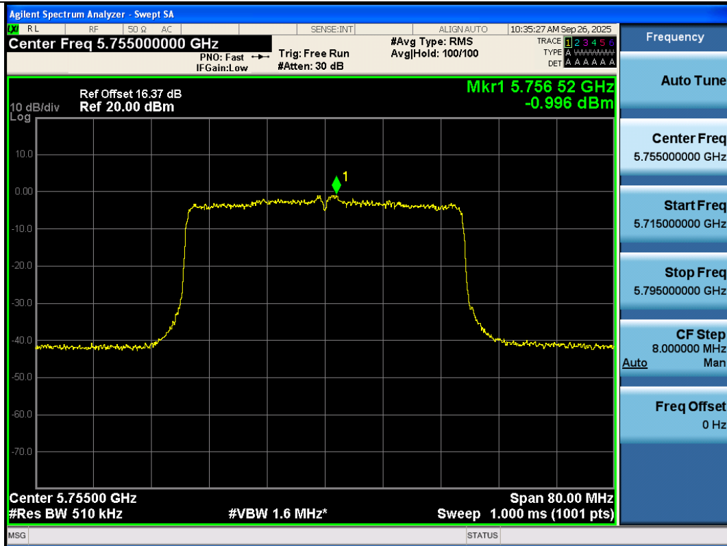
11AX40SISO-Ant3-5755-PASS
