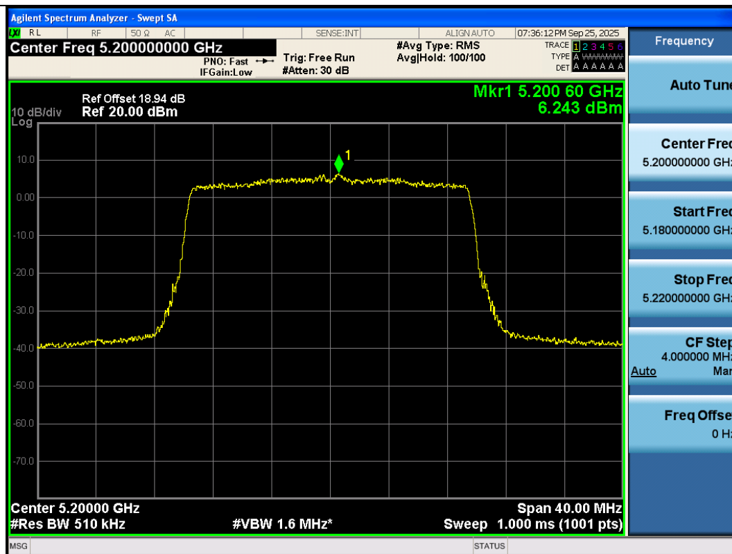
11AX20SISO-Ant3-5200-PASS
