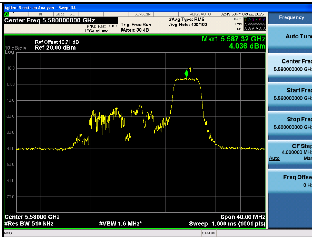
11AX20SISO-Ant3-5580-52Tone-RU40-PASS
