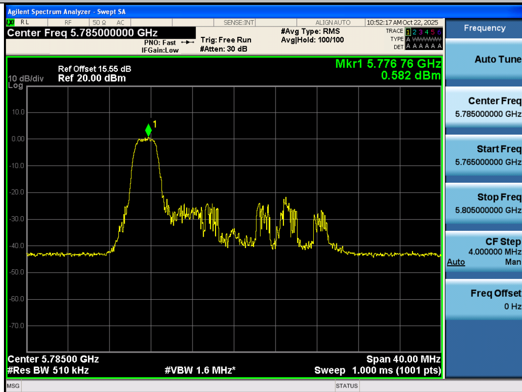
11AX20SISO-Ant3-5785-26Tone-RU0-PASS
