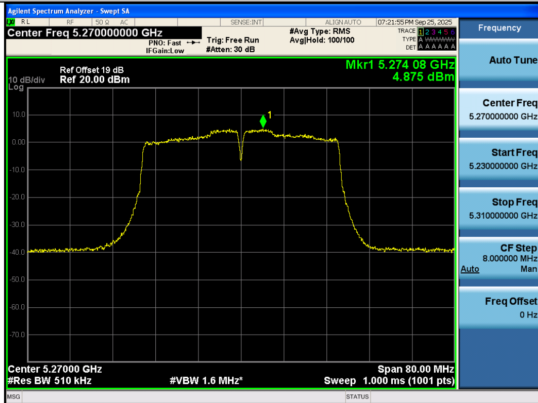
11AC40SISO-Ant3-5270-PASS
