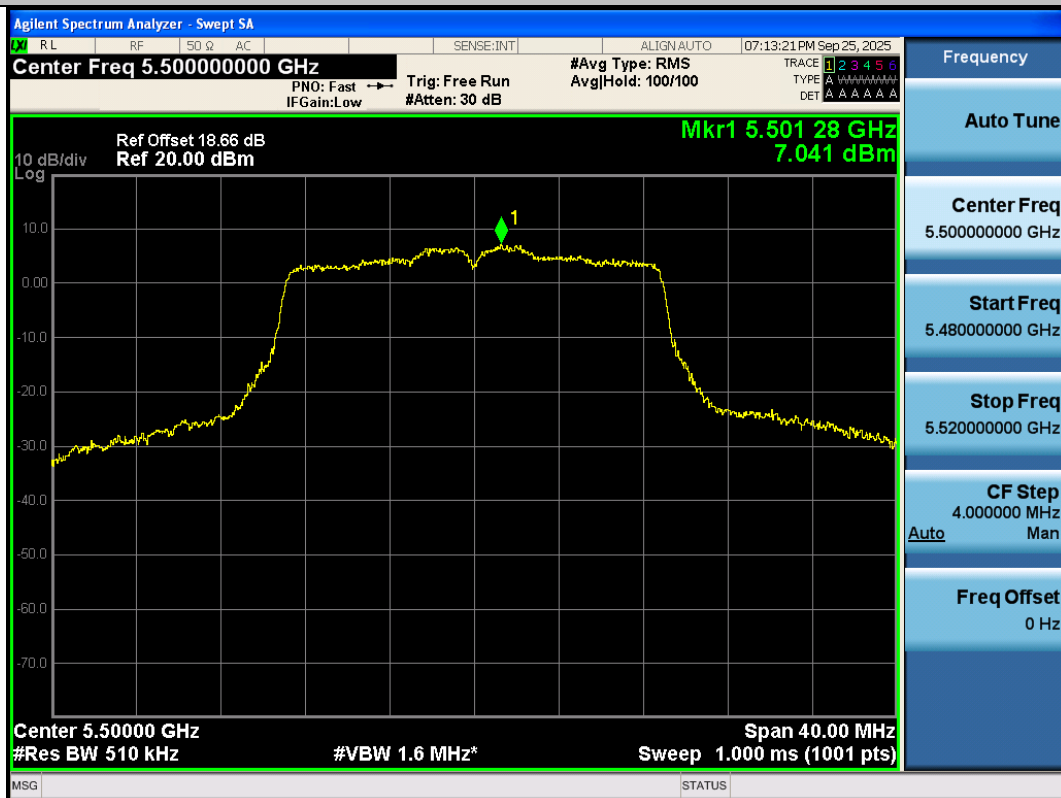
11AC20SISO-Ant3-5500-PASS
