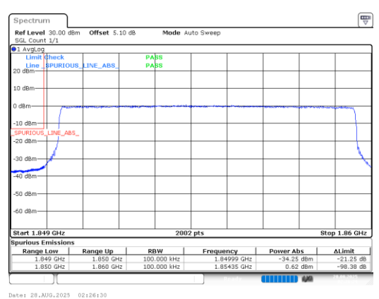
Band25-10MHz-64QAM-26090-50RB#0-PASS
