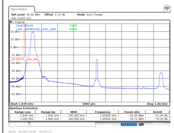
Band25-10MHz-16QAM-26090-1RB#0-PASS
