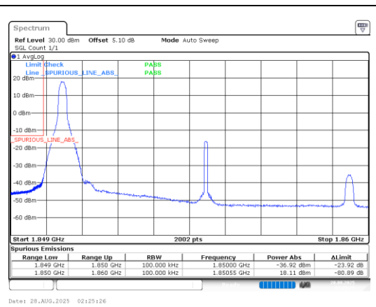
Band25-10MHz-64QAM-26090-1RB#0-PASS
