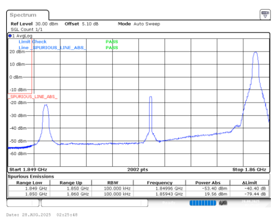
Band25-10MHz-16QAM-26090-1RB#49-PASS
