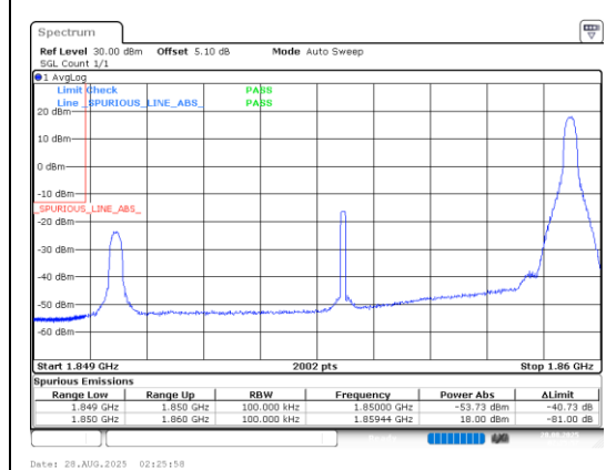
Band25-10MHz-64QAM-26090-1RB#49-PASS
