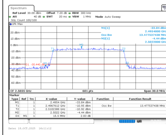
Band41-15MHz-16QAM-39725-75RB#0-PASS
