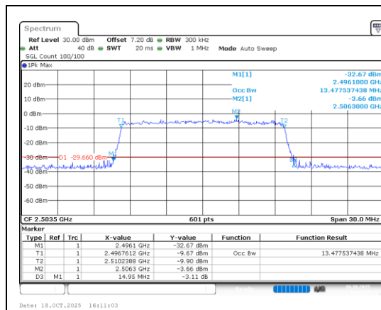
Band41-15MHz-QPSK-39725-75RB#0-PASS
