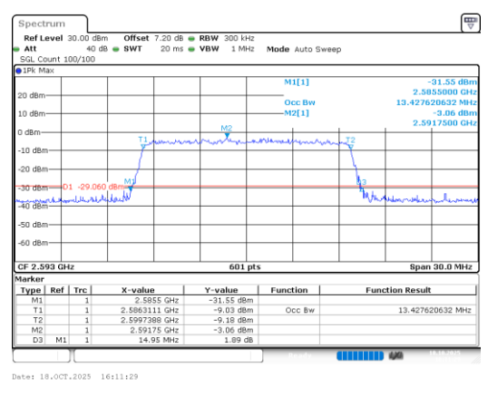
Band41-15MHz-QPSK-40620-75RB#0-PASS
