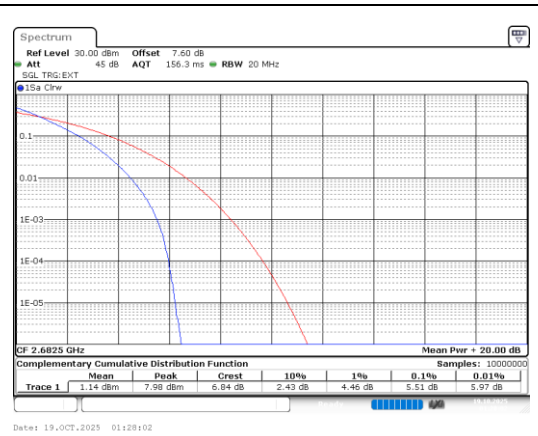
Band41-15MHz-QPSK-41515-75RB#0-PASS
