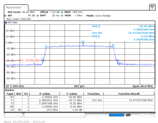
Band41-15MHz-16QAM-40620-75RB#0-PASS
