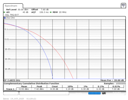
Band41-15MHz-64QAM-41515-75RB#0-PASS
