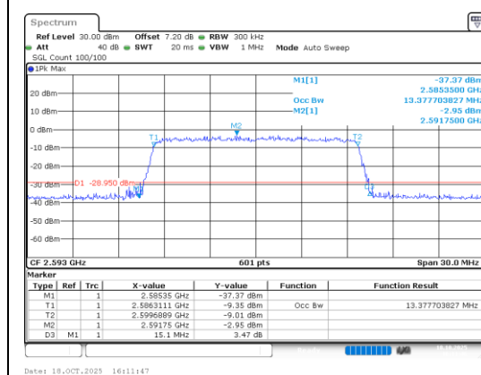
Band41-15MHz-64QAM-40620-75RB#0-PASS
