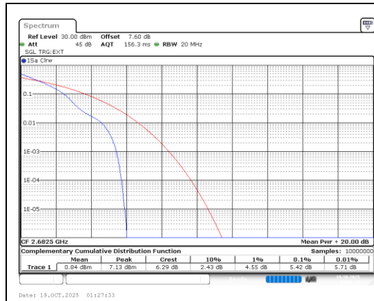
Band41-15MHz-QPSK-41515-1RB#0-PASS
