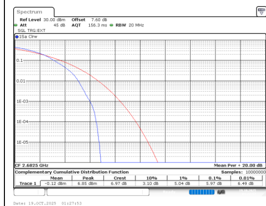
Band41-15MHz-64QAM-41515-1RB#0-PASS
