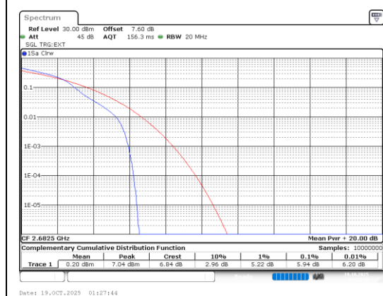
Band41-15MHz-16QAM-41515-1RB#0-PASS
