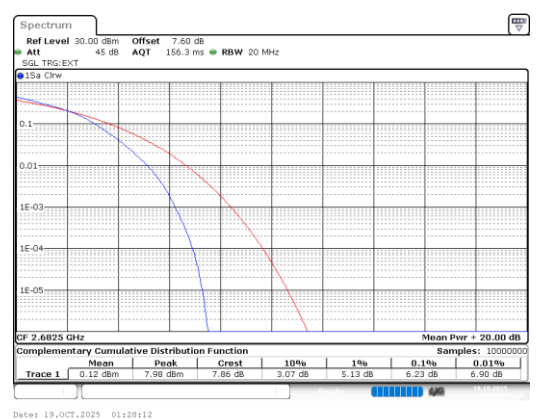
Band41-15MHz-16QAM-41515-75RB#0-PASS
