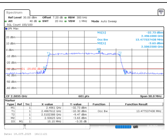
Band41-15MHz-64QAM-39725-75RB#0-PASS
