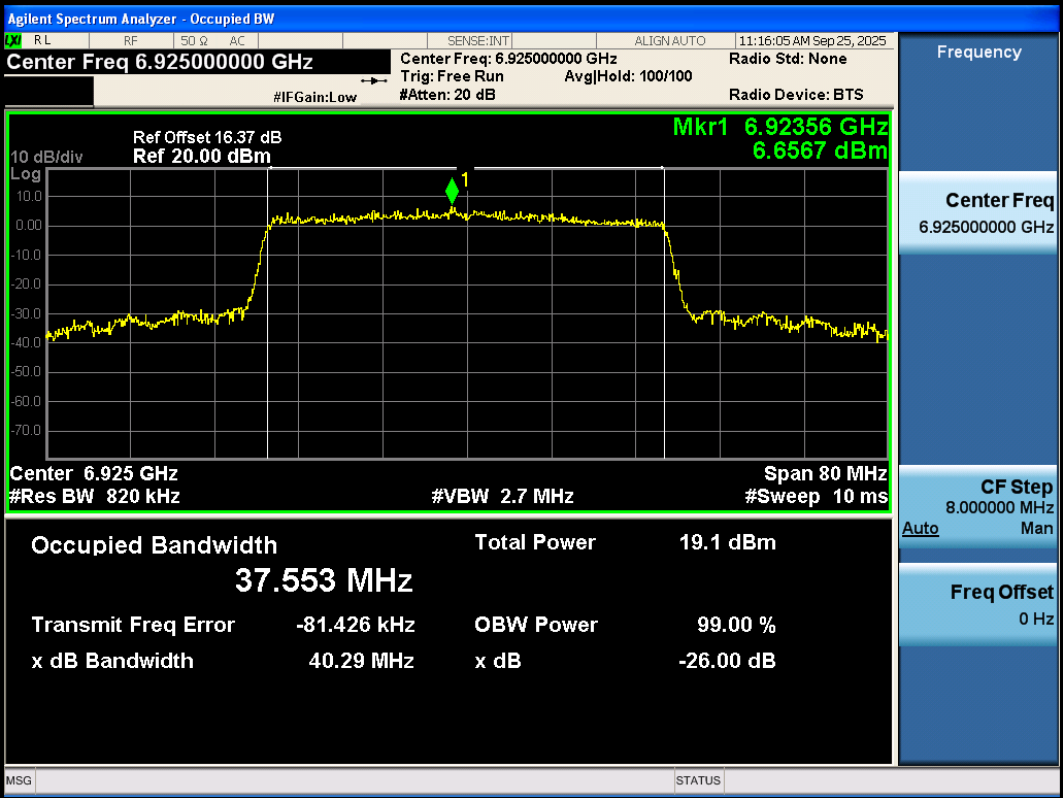
11AX40SISO-Ant3-6925-PASS
