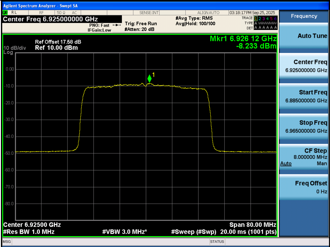
11AX40SISO-Ant3-6925-PASS
