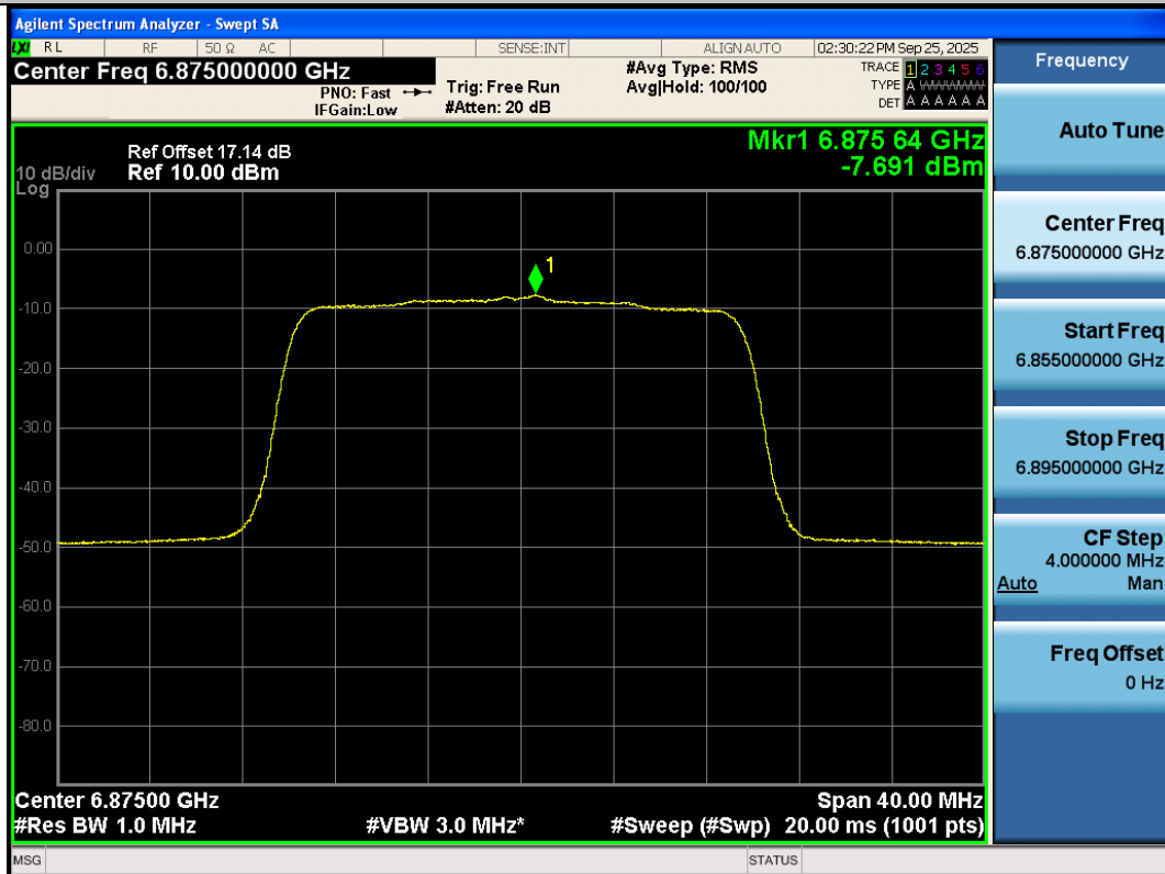
11AX20SISO-Ant3-6875-PASS
