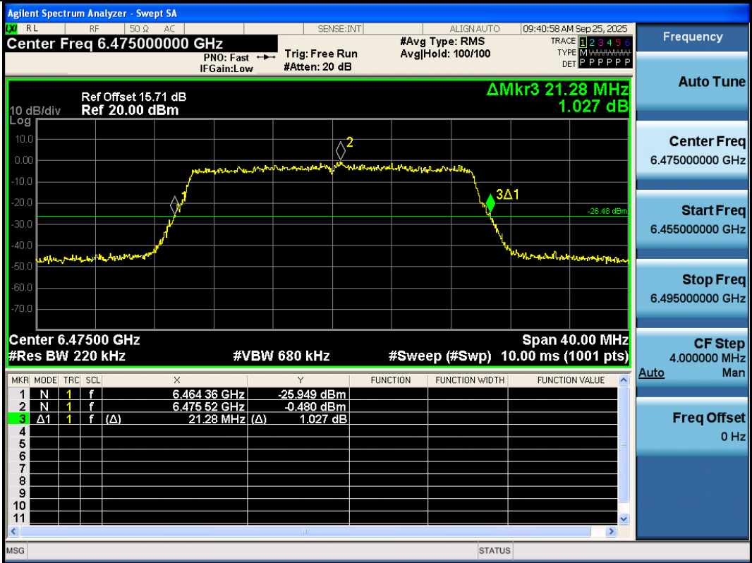
11AX20SISO-Ant3-6475
