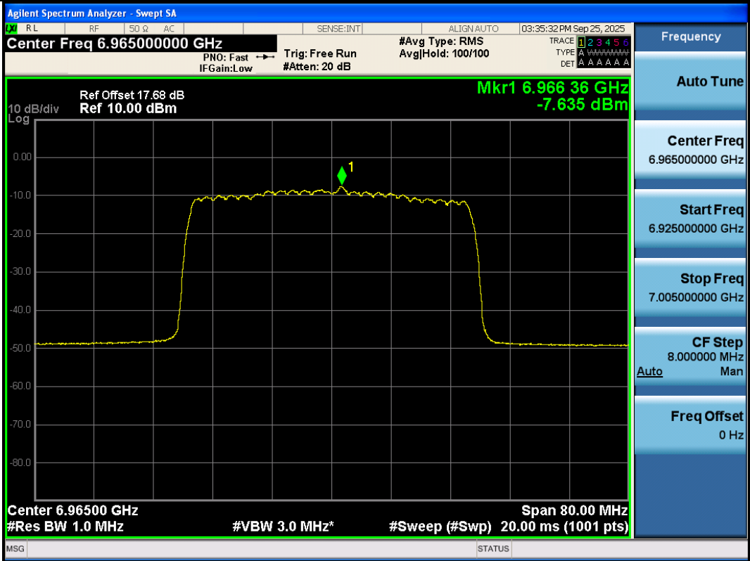
11AX40SISO-Ant3-6965-PASS
