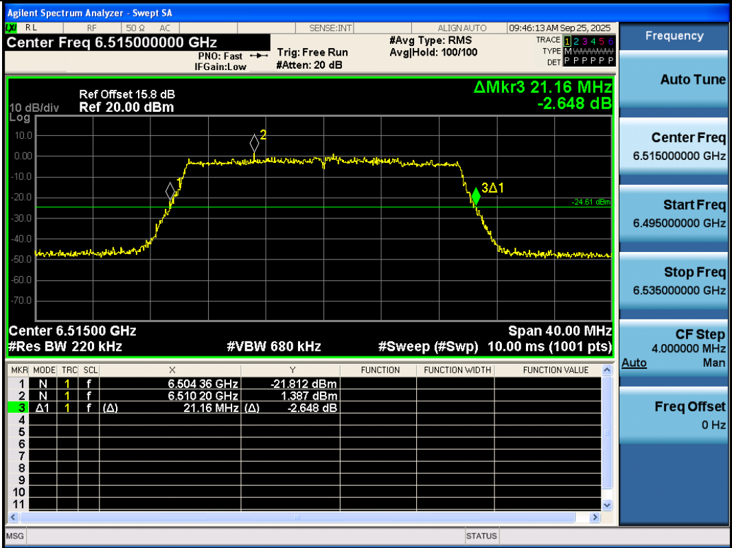
11AX20SISO-Ant3-6515
