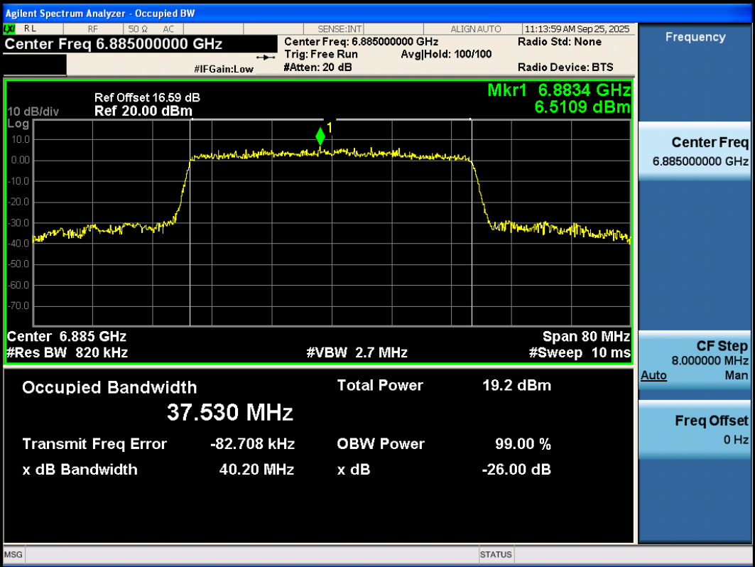
11AX40SISO-Ant3-6885-PASS
