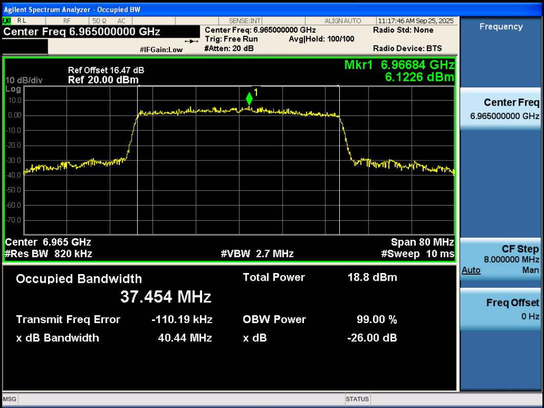
11AX40SISO-Ant3-6965-PASS
