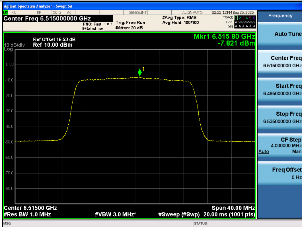
11AX20SISO-Ant3-6515-PASS
