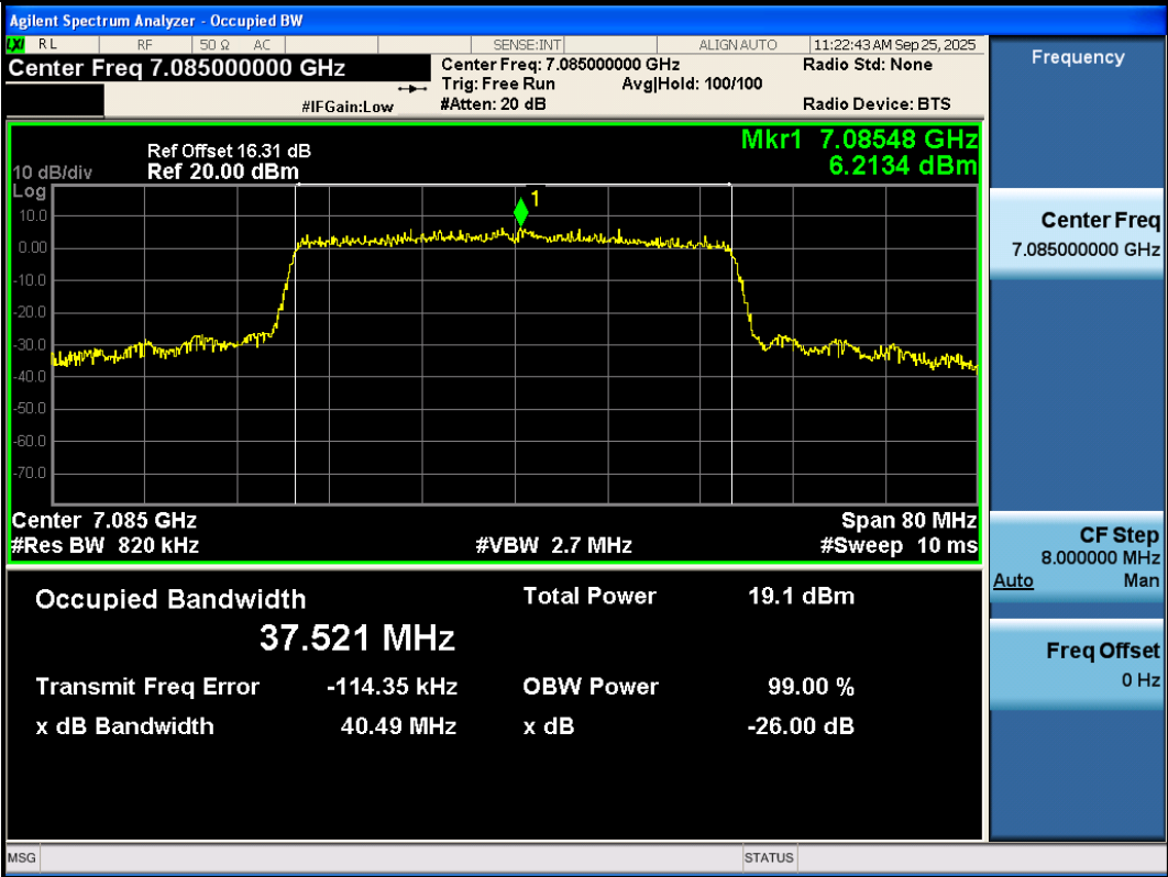
11AX40SISO-Ant3-7085-PASS
