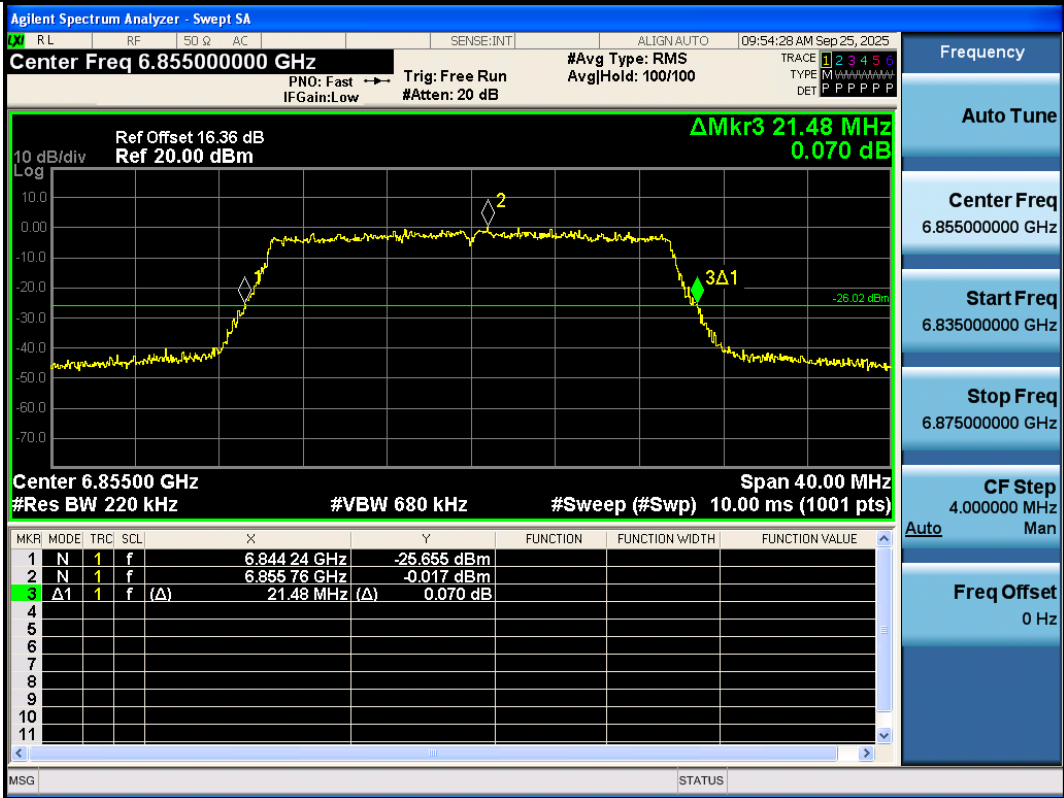
11AX20SISO-Ant3-6855
