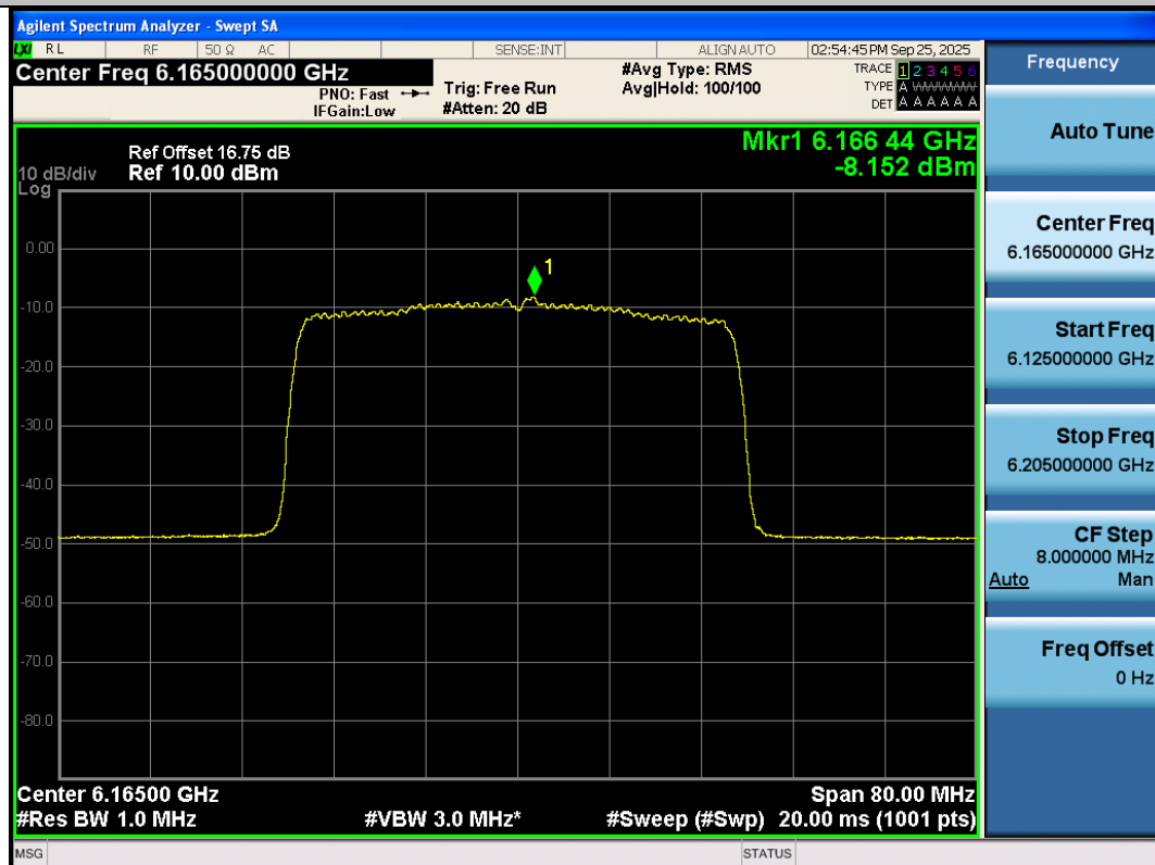
11AX40SISO-Ant3-6165-PASS
