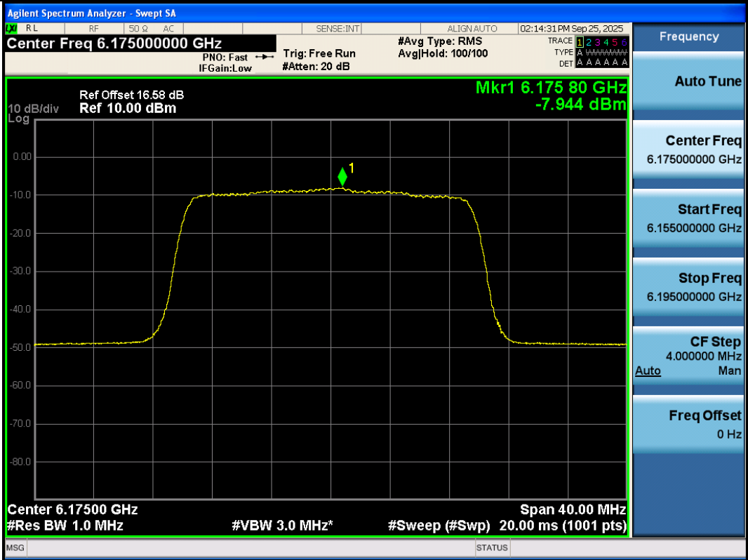
11AX20SISO-Ant3-6175-PASS
