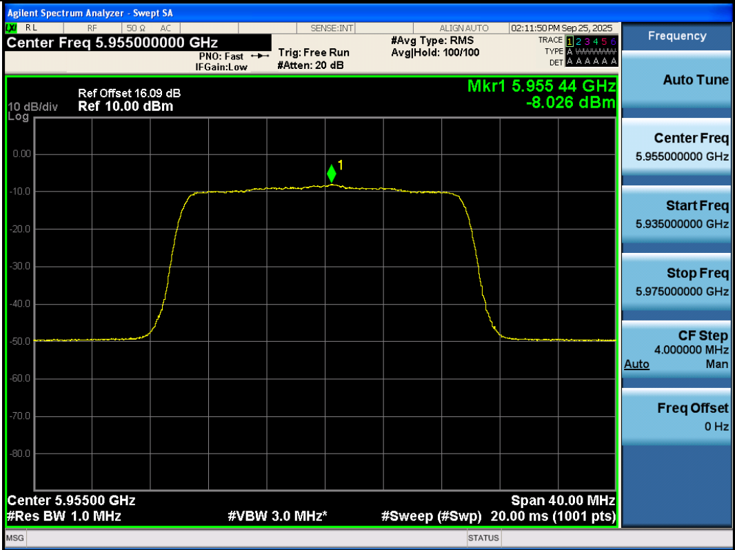
11AX20SISO-Ant3-5955-PASS
