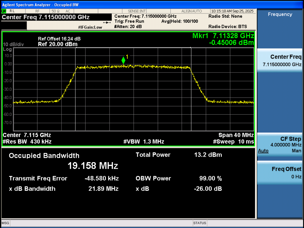
11AX20SISO-Ant3-7115-PASS
