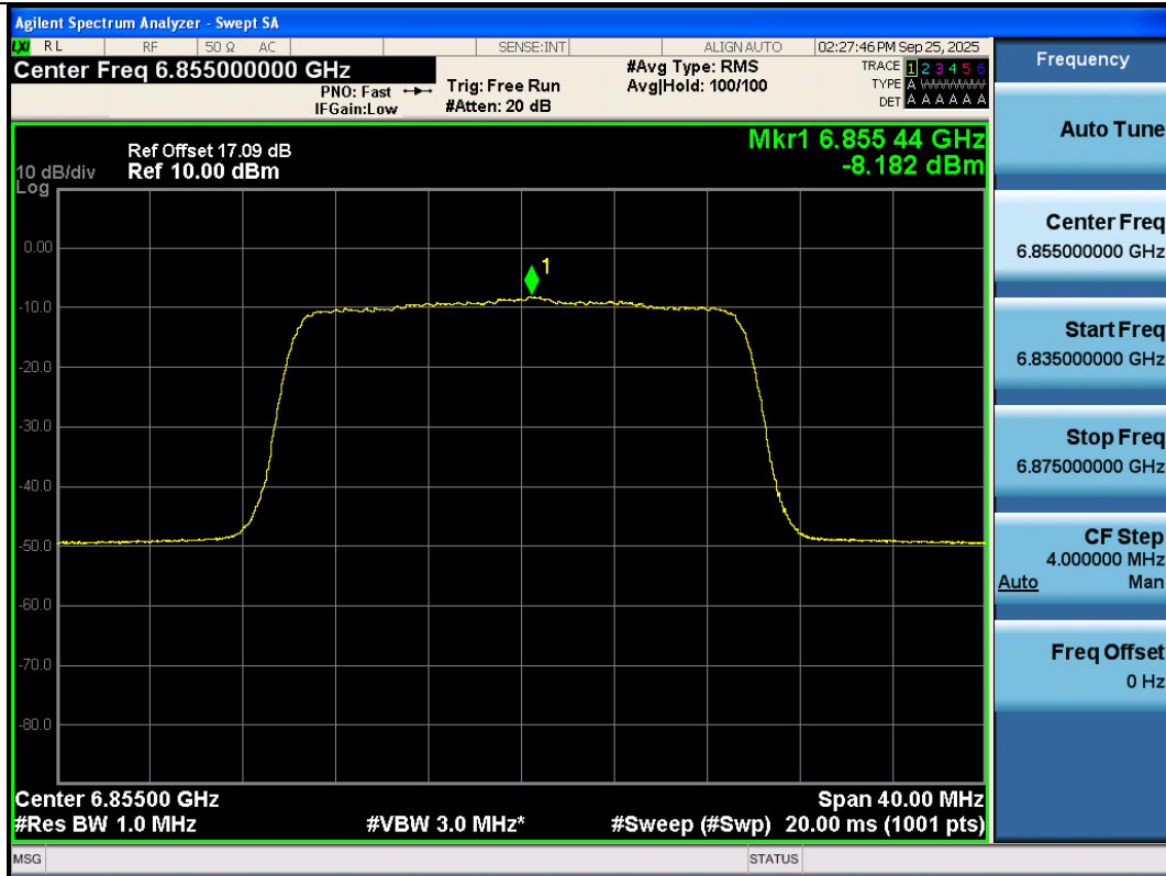
11AX20SISO-Ant3-6855-PASS
