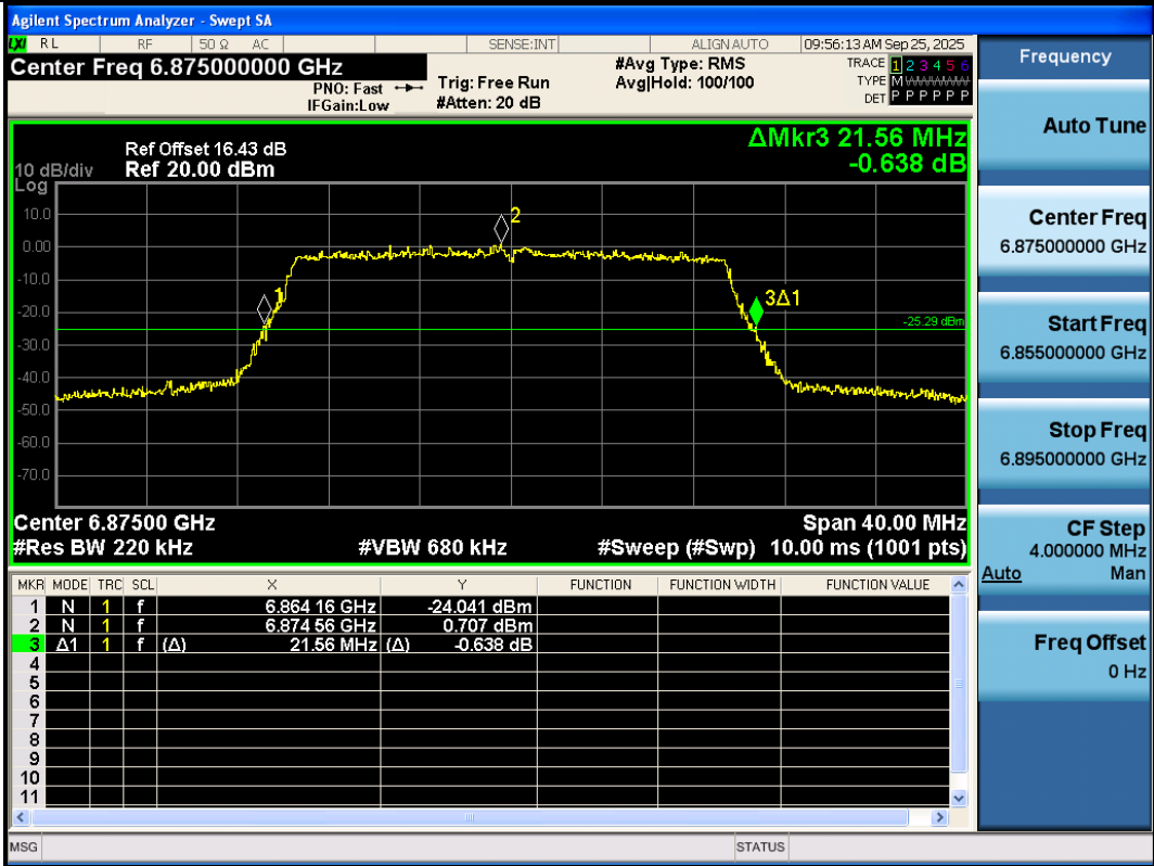
11AX20SISO-Ant3-6875
