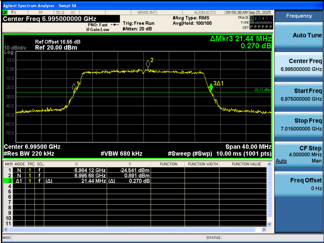
11AX20SISO-Ant3-6995
