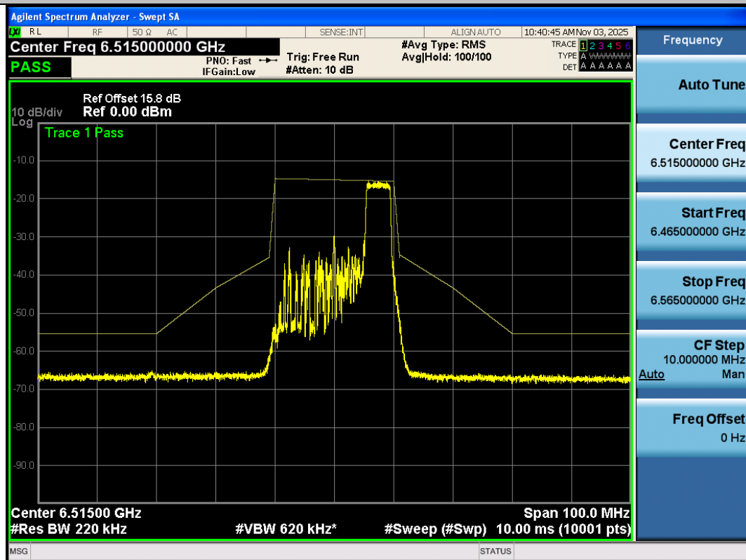
NTNV-11AX20SISO-Ant3-6515-52Tone-RU40-PASS
