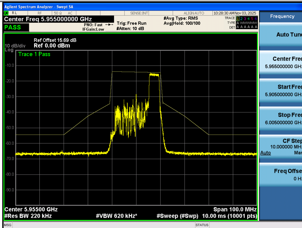
NTNV-11AX20SISO-Ant3-5955-52Tone-RU40-PASS
