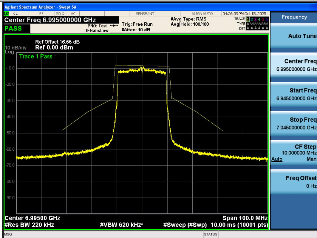
NTNV-11AX20SISO-Ant3-6995-PASS
