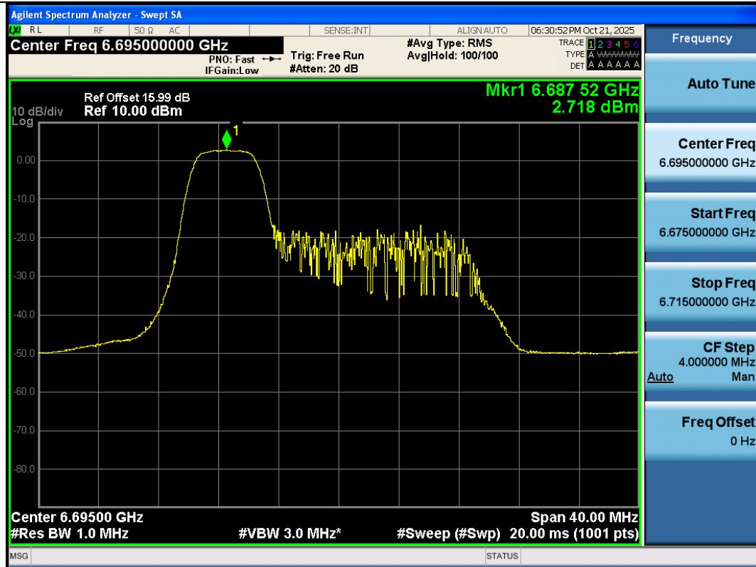
11AX20SISO-Ant2-6695-52Tone-RU37-PASS
