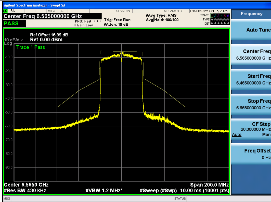
NTNV-11AX40SISO-Ant3-6565-PASS
