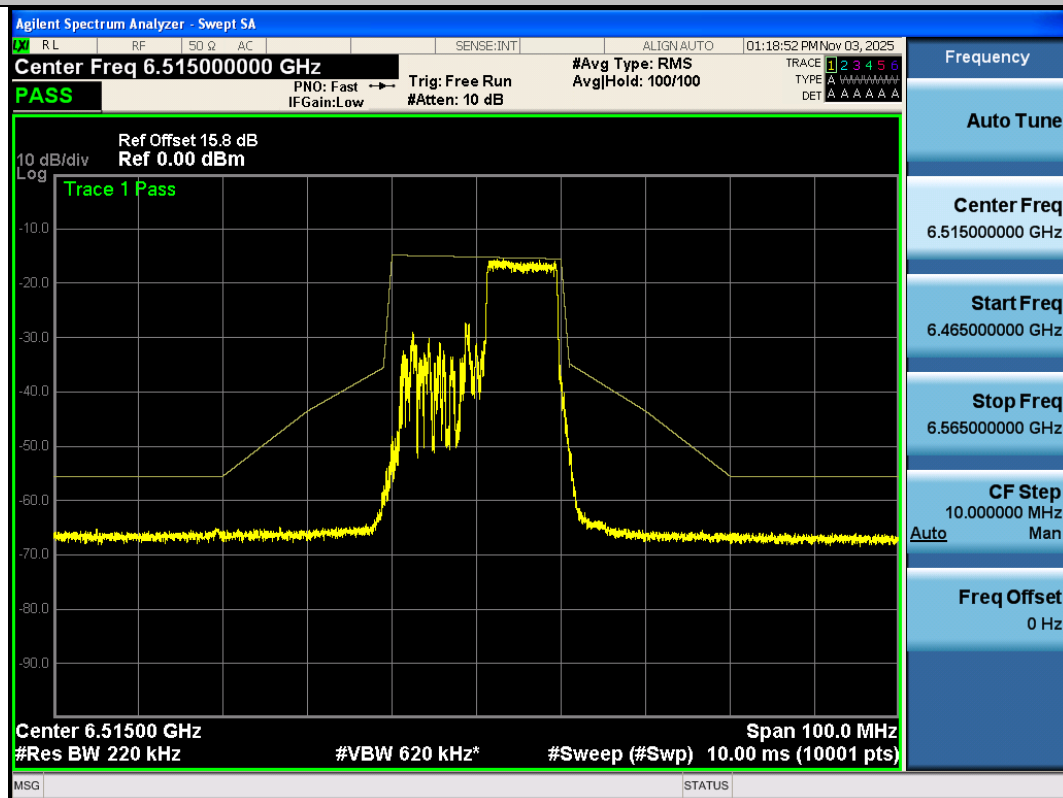
NTNV-11AX20SISO-Ant3-6515-106Tone-RU54-PASS
