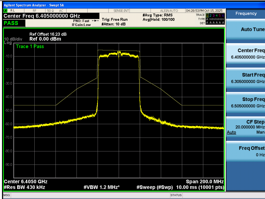
NTNV-11AX40SISO-Ant3-6405-PASS
