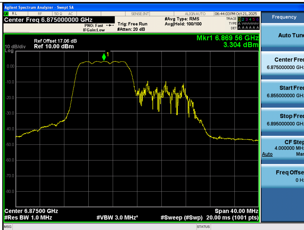
11AX20SISO-Ant2-6875-106Tone-RU53-PASS
