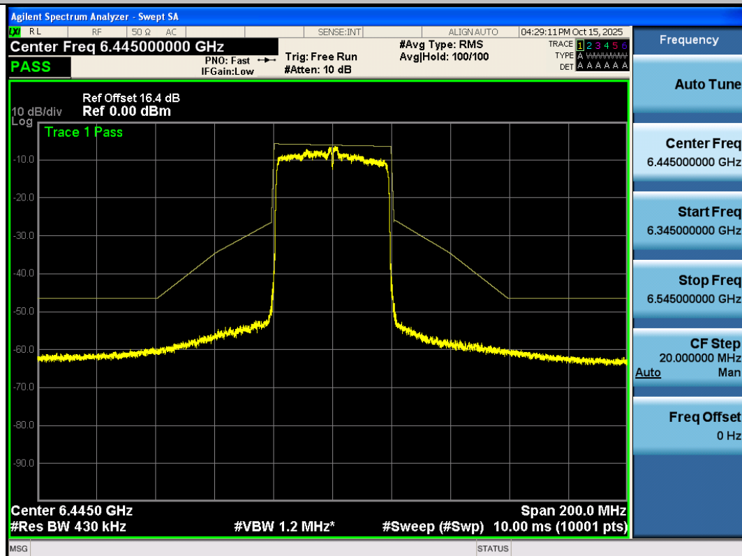
NTNV-11AX40SISO-Ant3-6445-PASS
