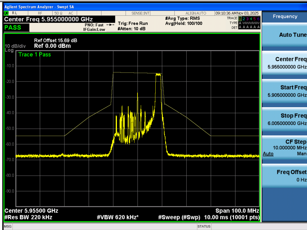
NTNV-11AX20SISO-Ant3-5955-26Tone-RU8-PASS
