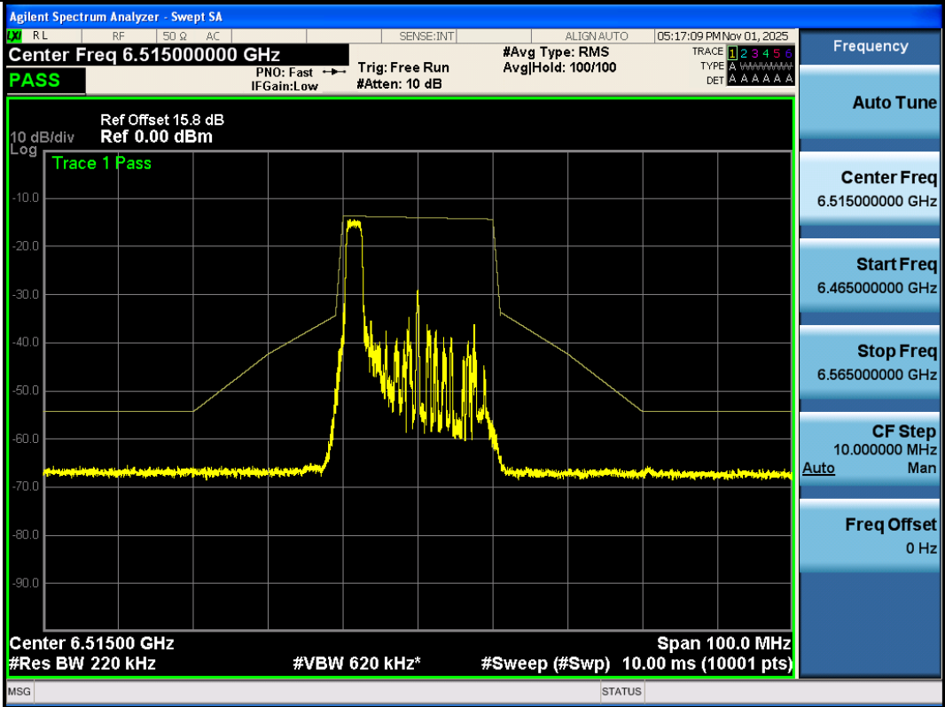
NTNV-11AX20SISO-Ant3-6515-26Tone-RU0-PASS
