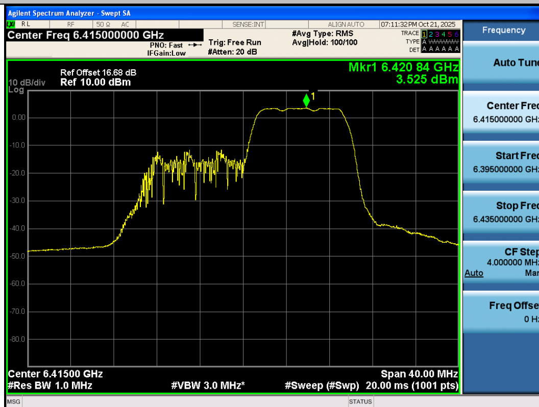
11AX20SISO-Ant2-6415-106Tone-RU54-PASS
