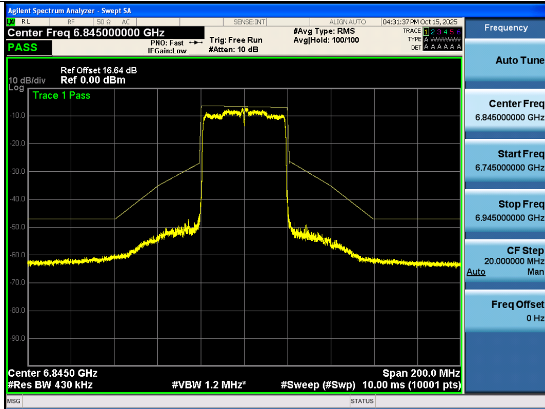
NTNV-11AX40SISO-Ant3-6845-PASS
