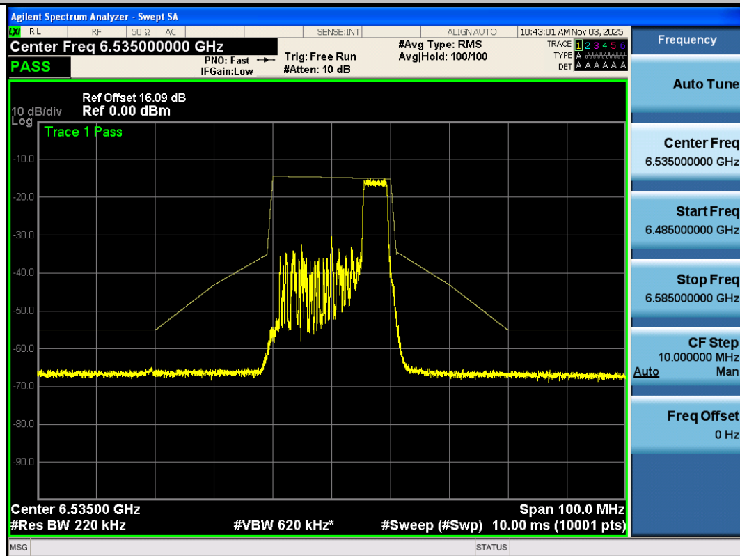
NTNV-11AX20SISO-Ant3-6535-52Tone-RU40-PASS
