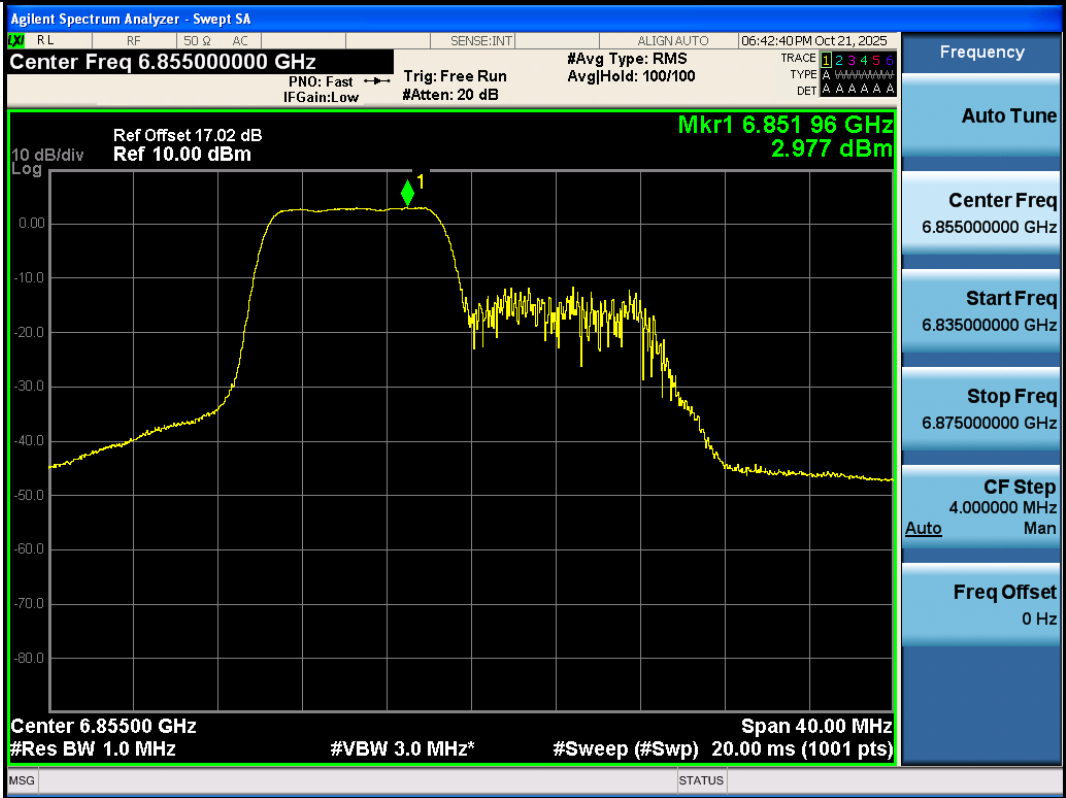
11AX20SISO-Ant2-6855-106Tone-RU53-PASS
