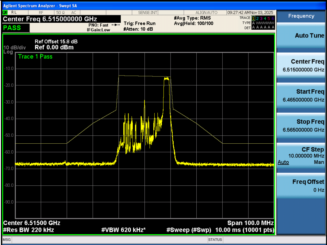
NTNV-11AX20SISO-Ant3-6515-26Tone-RU8-PASS
