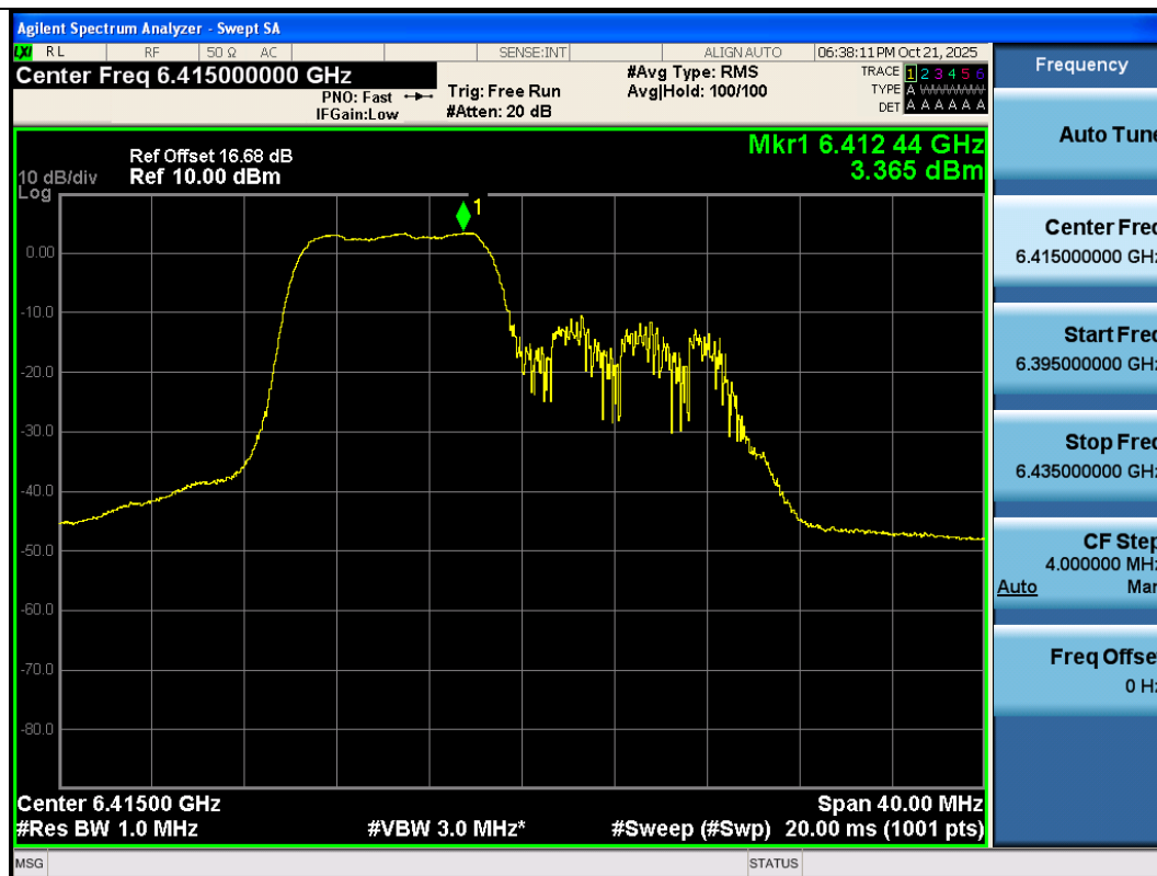
11AX20SISO-Ant2-6415-106Tone-RU53-PASS
