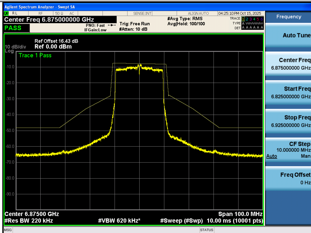
NTNV-11AX20SISO-Ant3-6875-PASS
