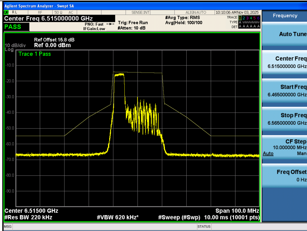
NTNV-11AX20SISO-Ant3-6515-52Tone-RU37-PASS
