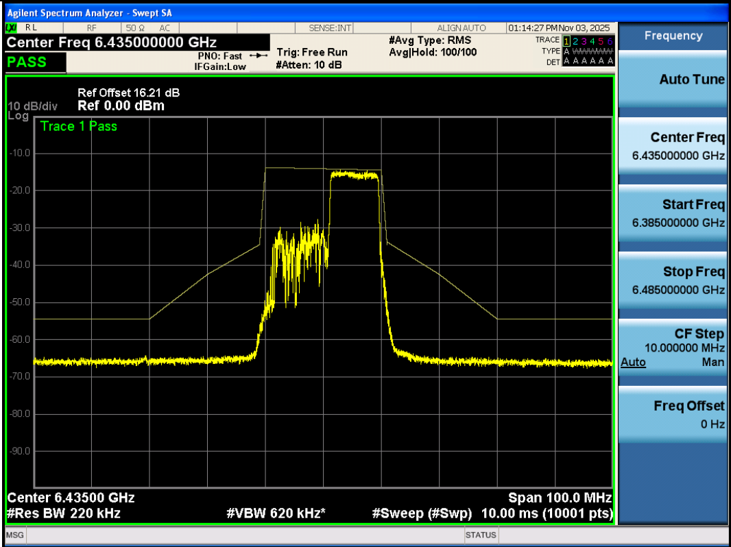
NTNV-11AX20SISO-Ant3-6435-106Tone-RU54-PASS
