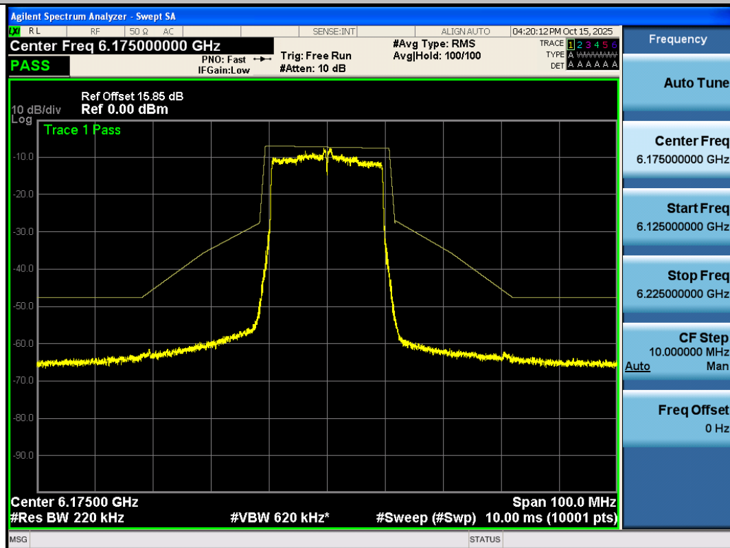
NTNV-11AX20SISO-Ant3-6175-PASS
