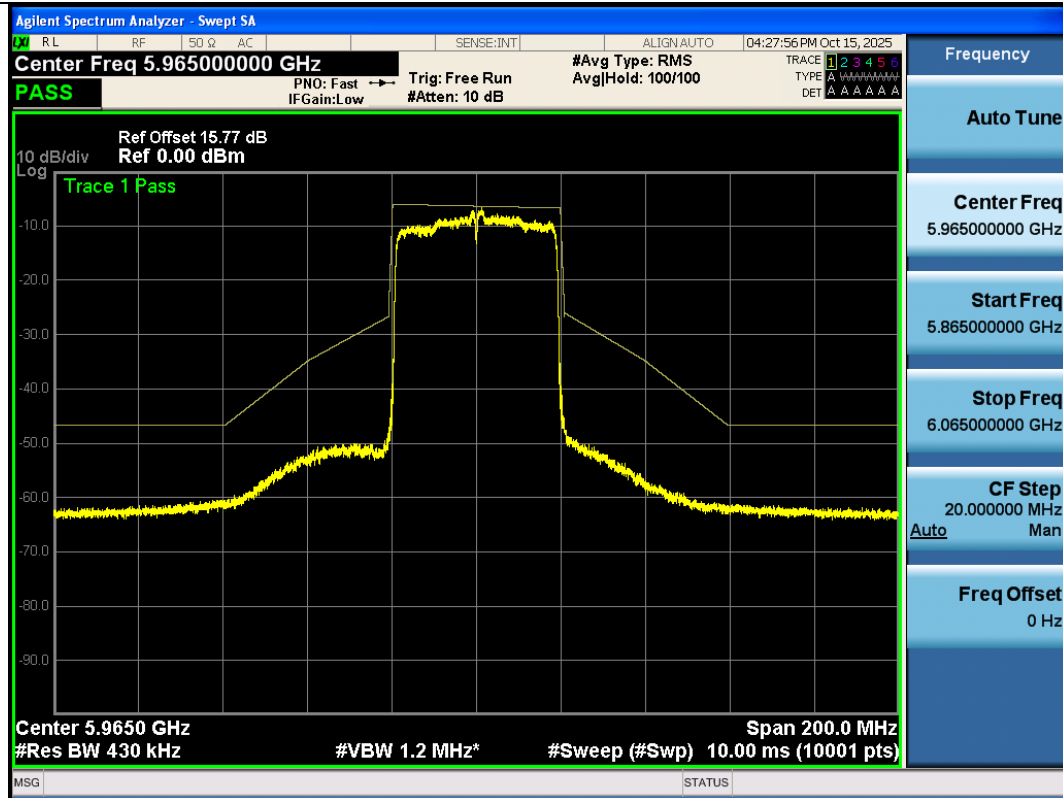
NTNV-11AX40SISO-Ant3-5965-PASS
