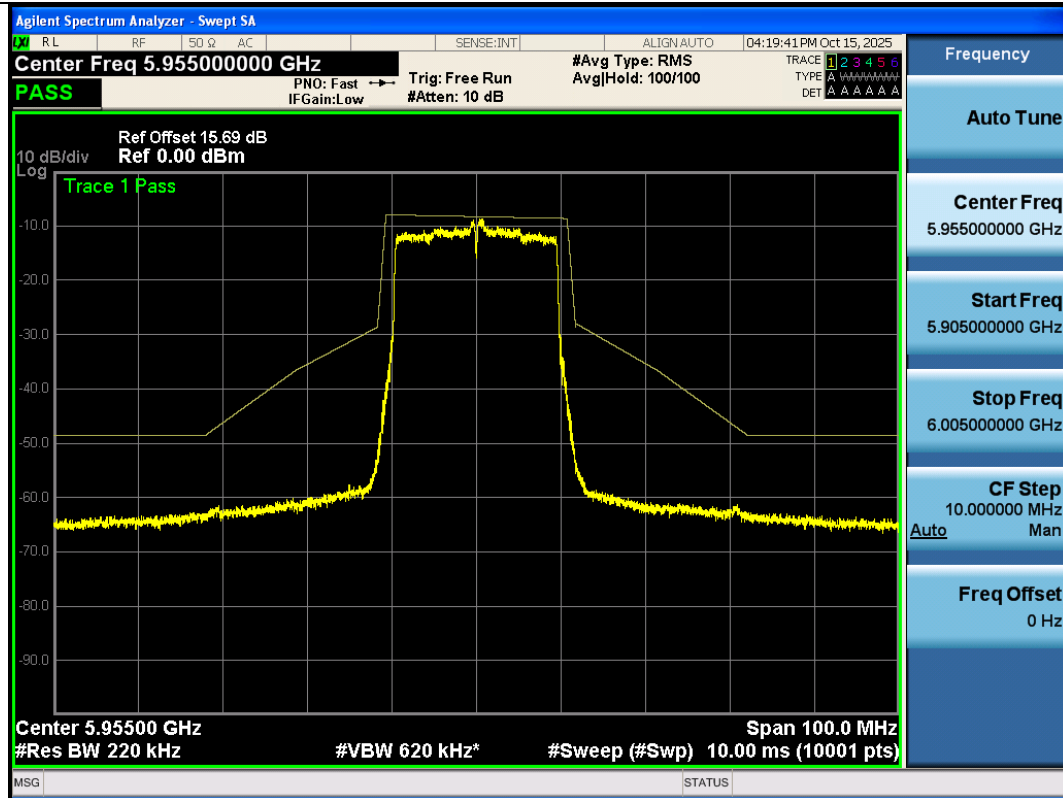
NTNV-11AX20SISO-Ant3-5955-PASS
