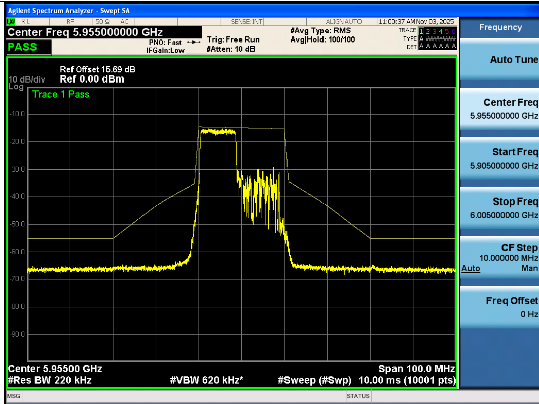
NTNV-11AX20SISO-Ant3-5955-106Tone-RU53-PASS
