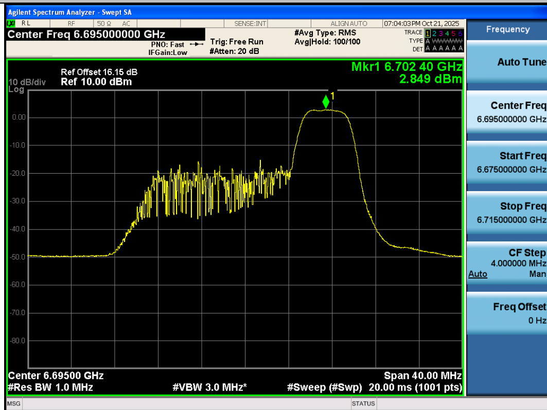
11AX20SISO-Ant2-6695-52Tone-RU40-PASS
