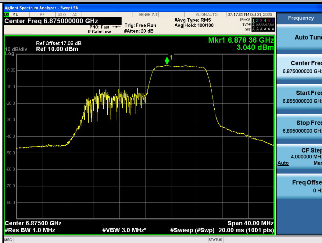
11AX20SISO-Ant2-6875-106Tone-RU54-PASS
