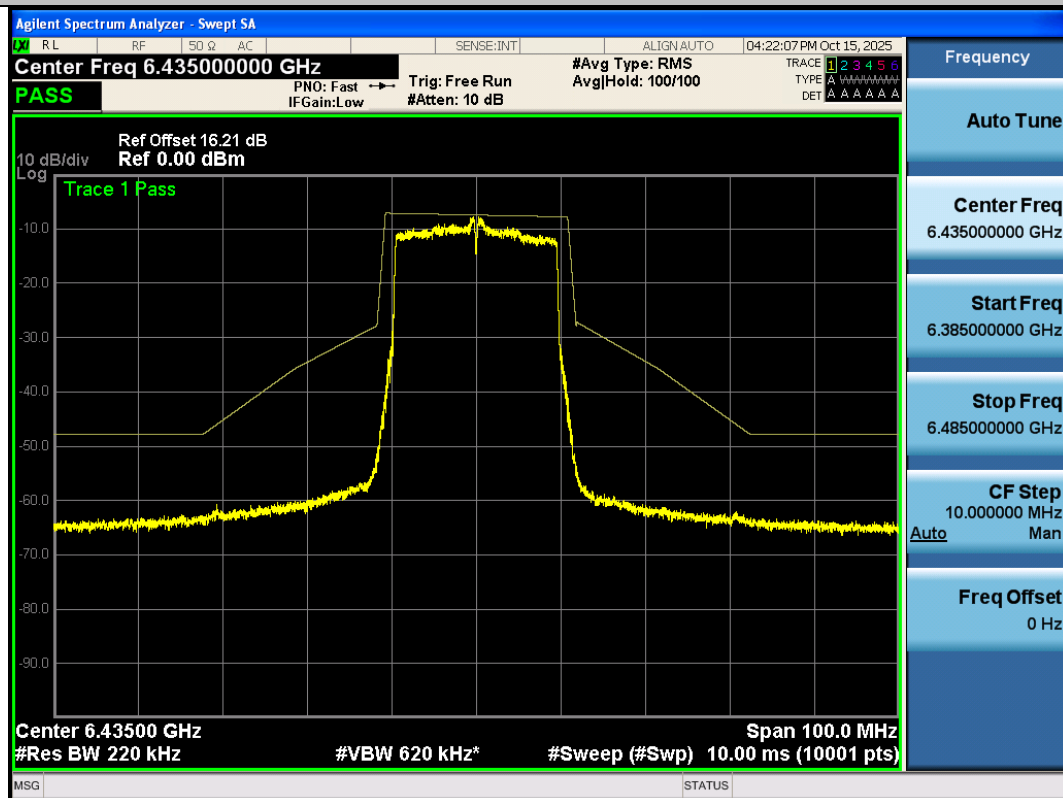
NTNV-11AX20SISO-Ant3-6435-PASS
