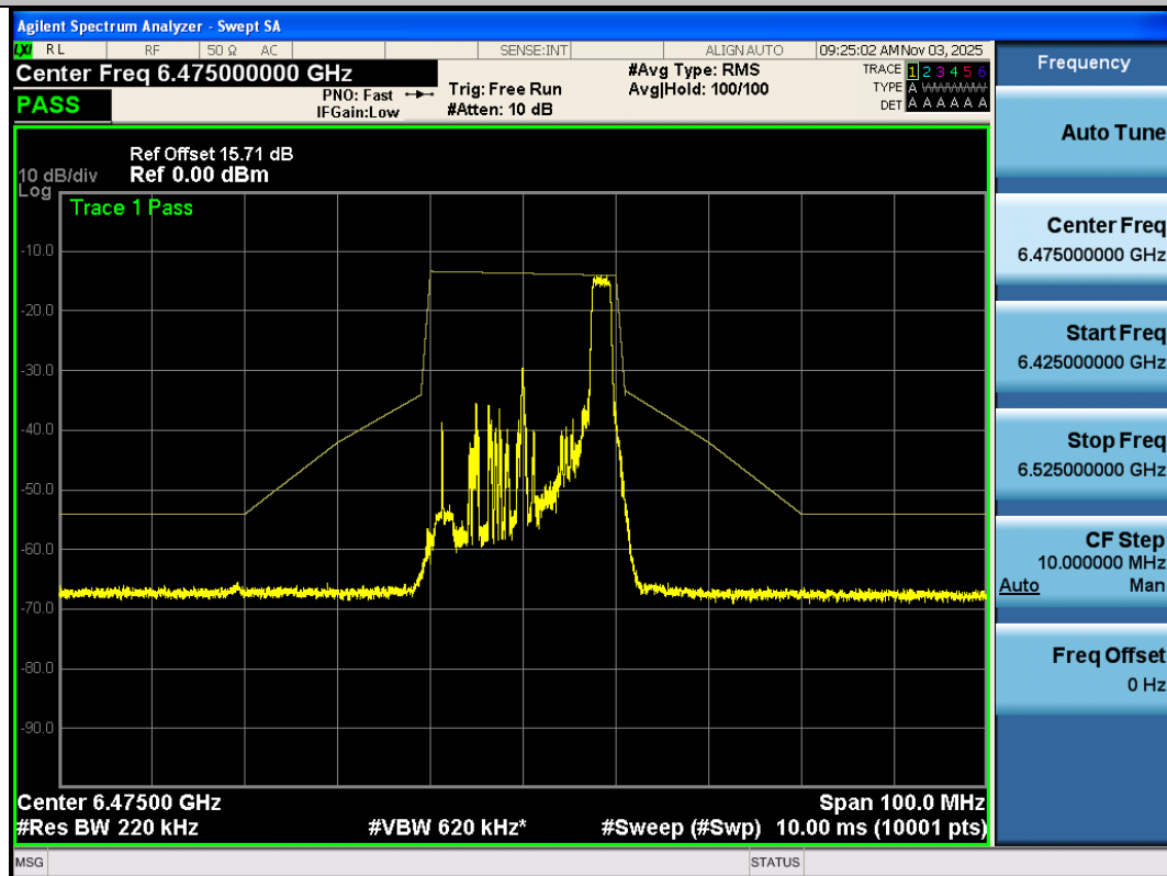
NTNV-11AX20SISO-Ant3-6475-26Tone-RU8-PASS
