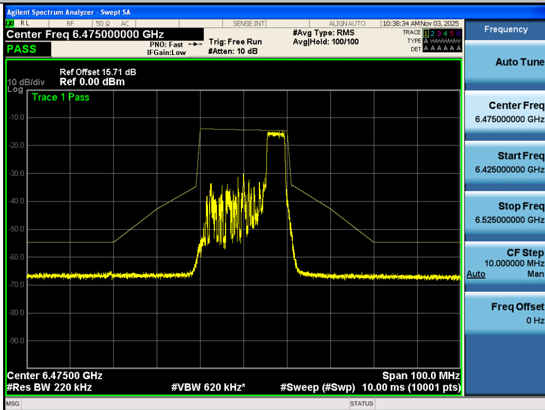
NTNV-11AX20SISO-Ant3-6475-52Tone-RU40-PASS
