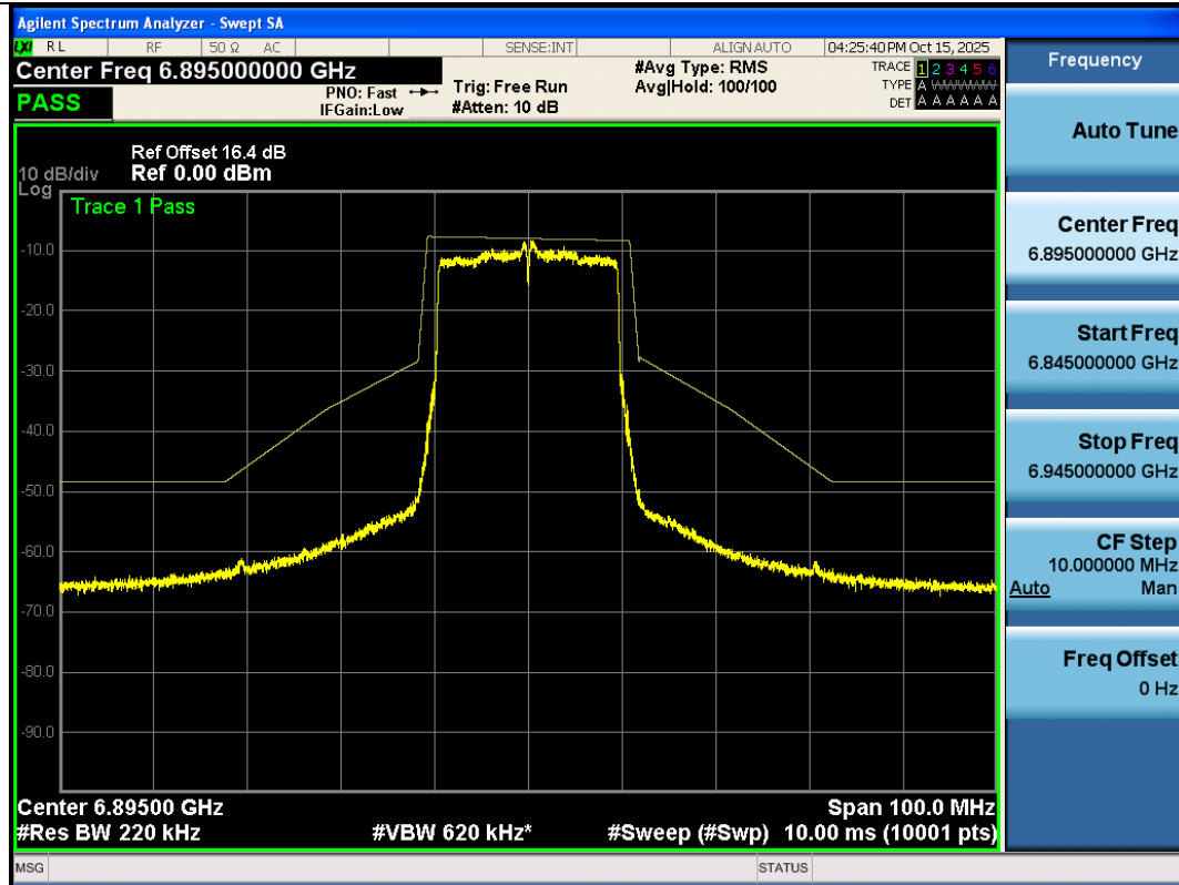
NTNV-11AX20SISO-Ant3-6895-PASS
