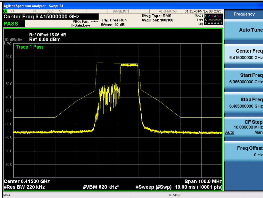
NTNV-11AX20SISO-Ant3-6415-106Tone-RU54-PASS
