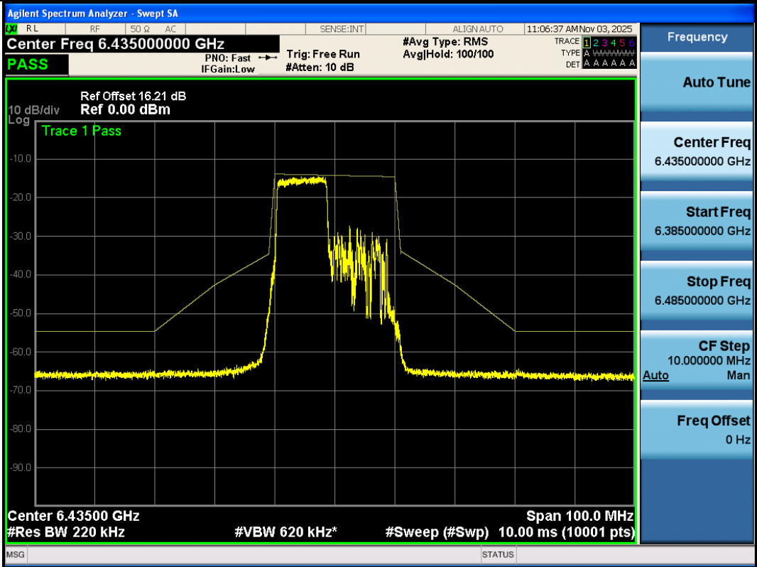
NTNV-11AX20SISO-Ant3-6435-106Tone-RU53-PASS
