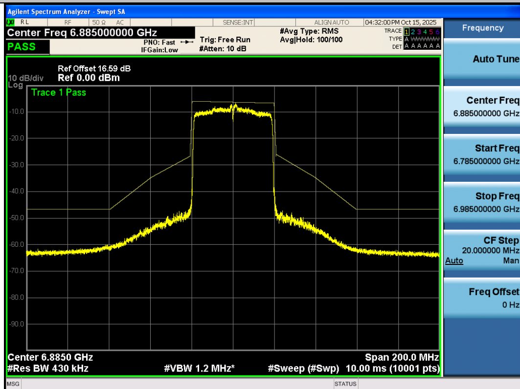
NTNV-11AX40SISO-Ant3-6885-PASS
