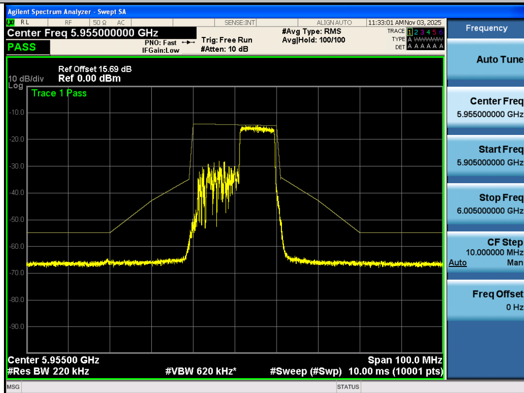
NTNV-11AX20SISO-Ant3-5955-106Tone-RU54-PASS
