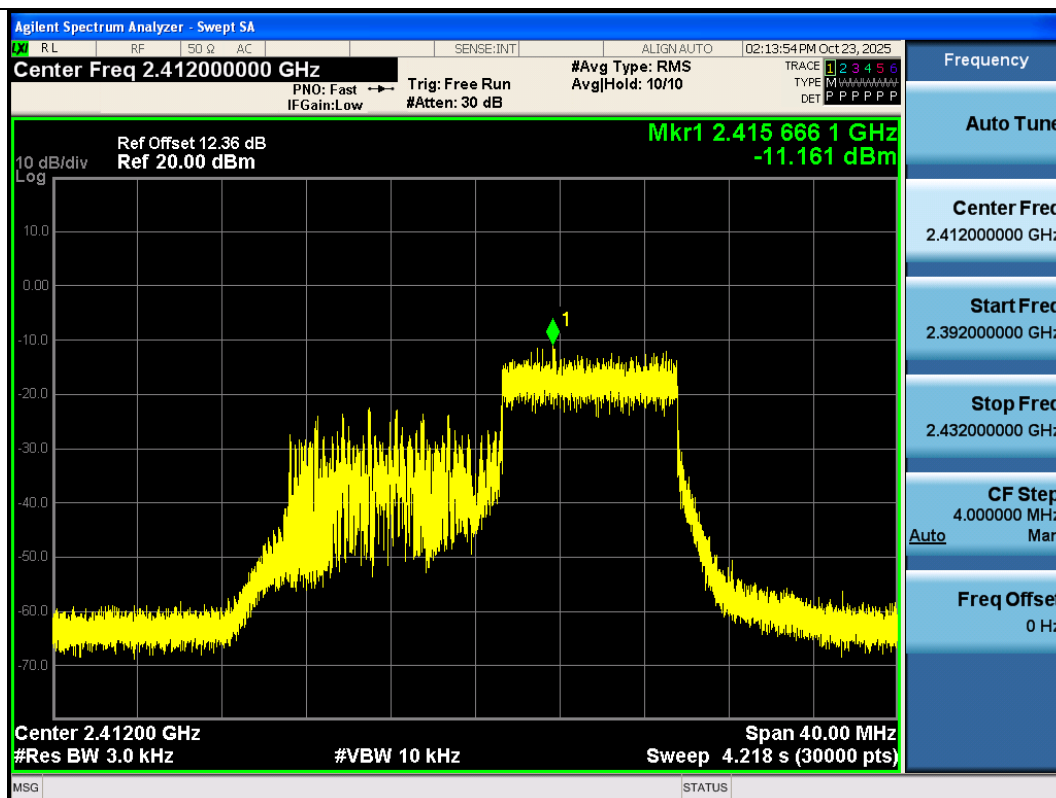
11AX20SISO-Ant3-2412-106Tone-RU54-PASS
