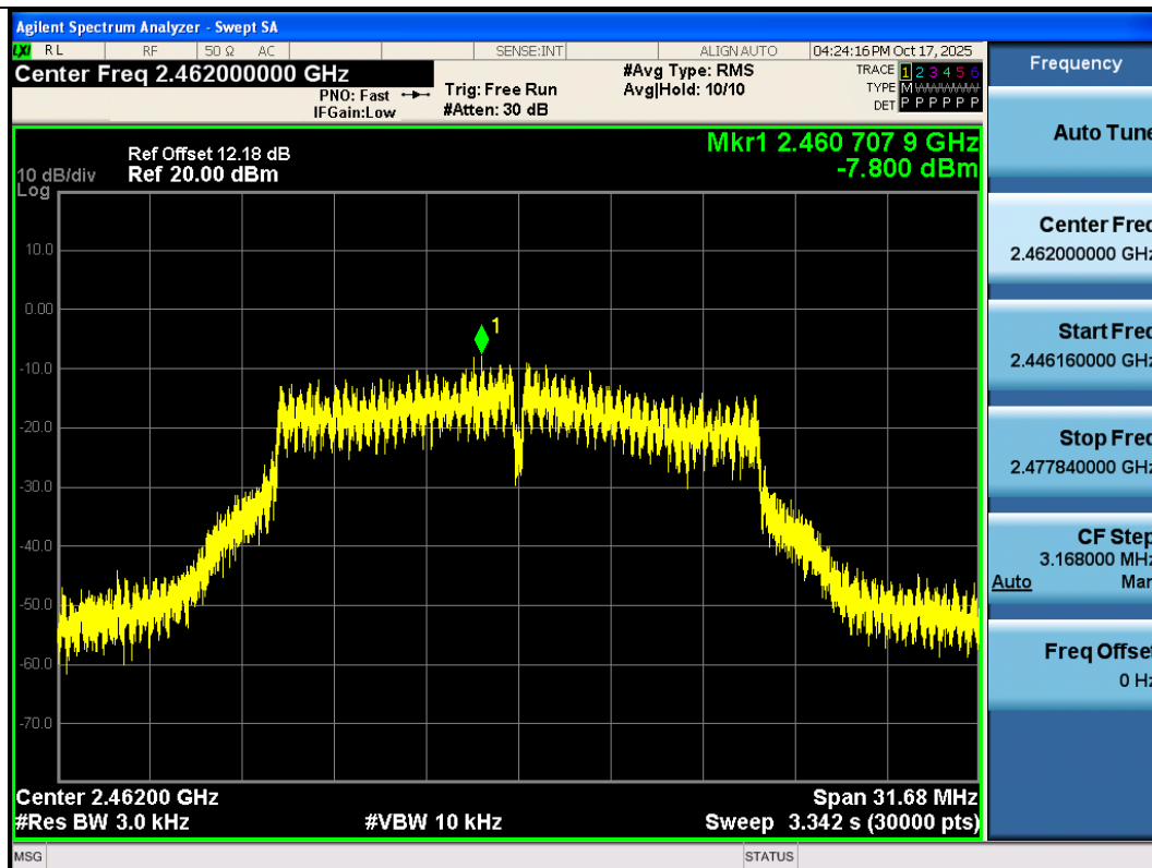
11G-Ant3-2462-PASS
