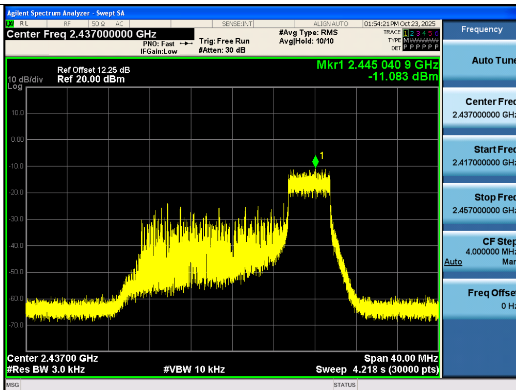
11AX20SISO-Ant3-2437-52Tone-RU40-PASS
