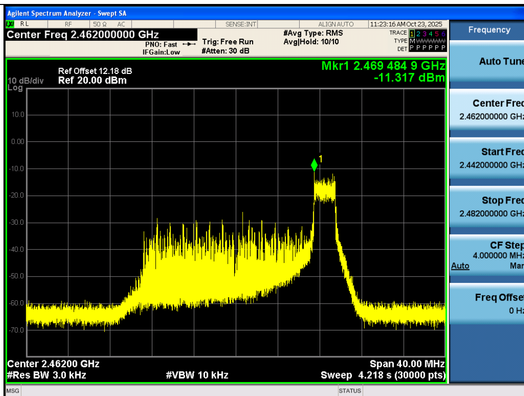
11AX20SISO-Ant3-2462-26Tone-RU8-PASS
