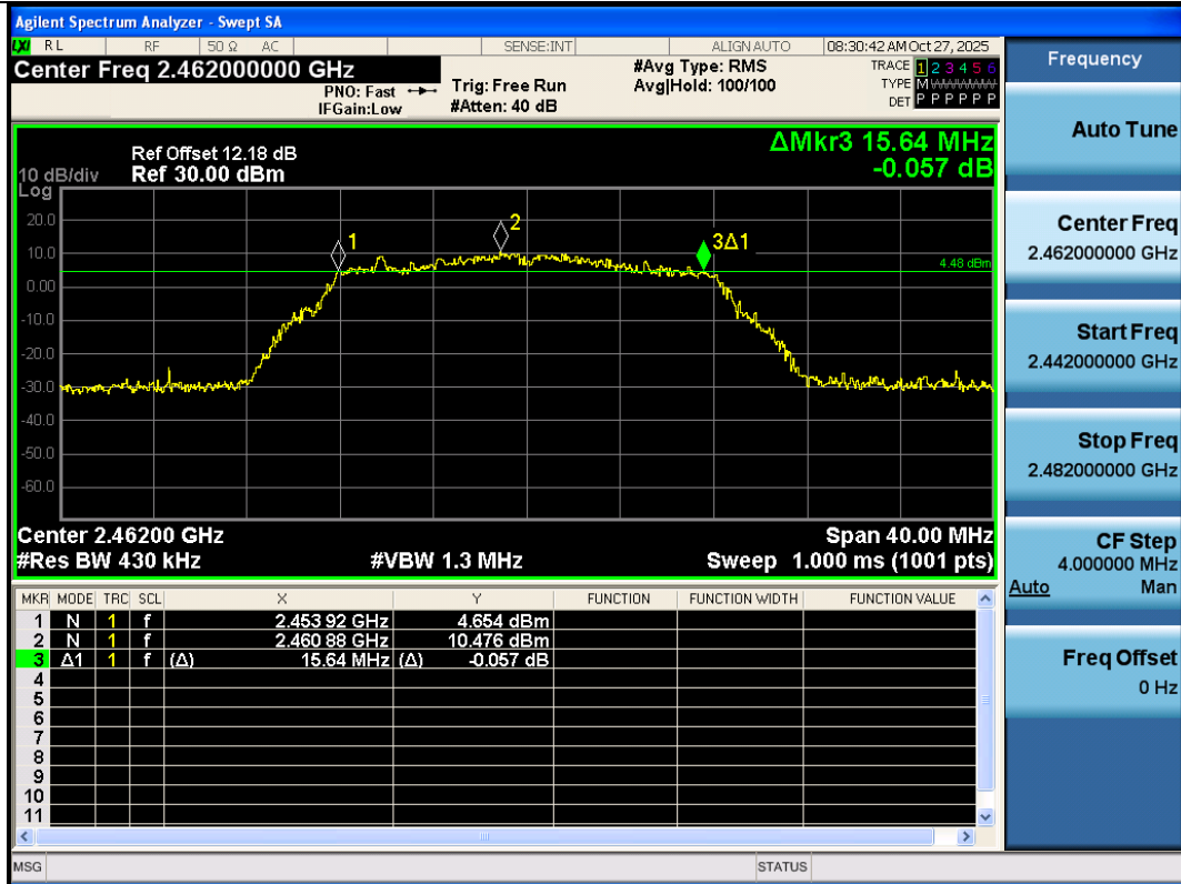
11G-Ant3-2462-PASS
