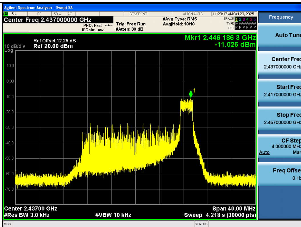
11AX20SISO-Ant3-2437-26Tone-RU8-PASS
