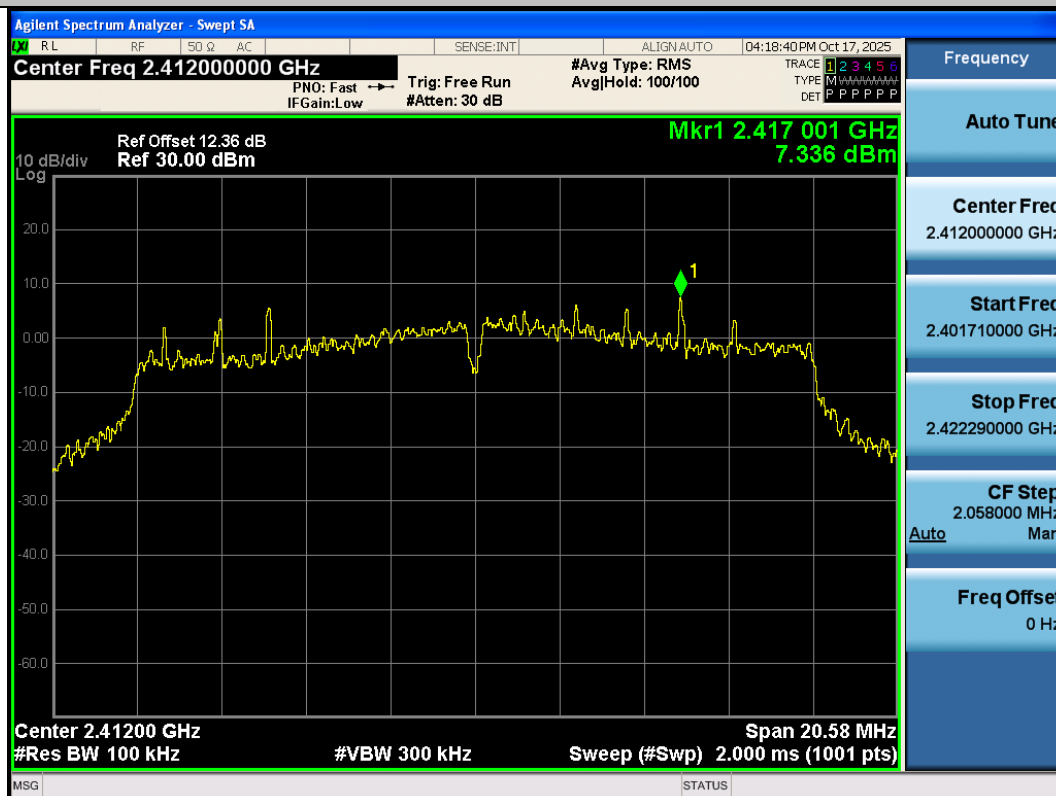
11G-Ant3-2412-PASS
