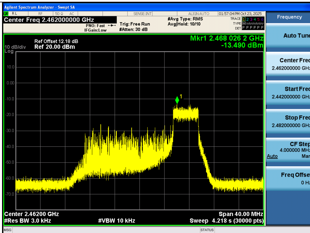
11AX20SISO-Ant3-2462-52Tone-RU40-PASS
