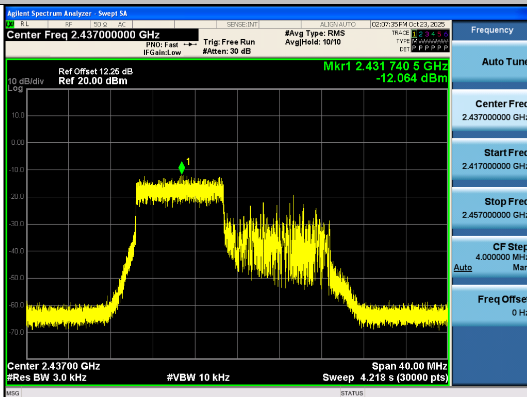
11AX20SISO-Ant3-2437-106Tone-RU53-PASS
