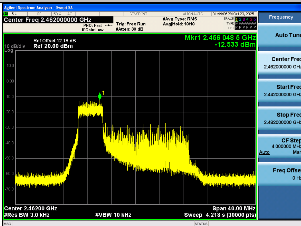
11AX20SISO-Ant3-2462-52Tone-RU37-PASS
