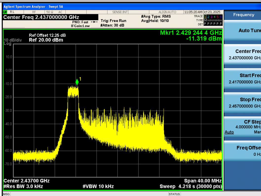
11AX20SISO-Ant3-2437-26Tone-RU0-PASS
