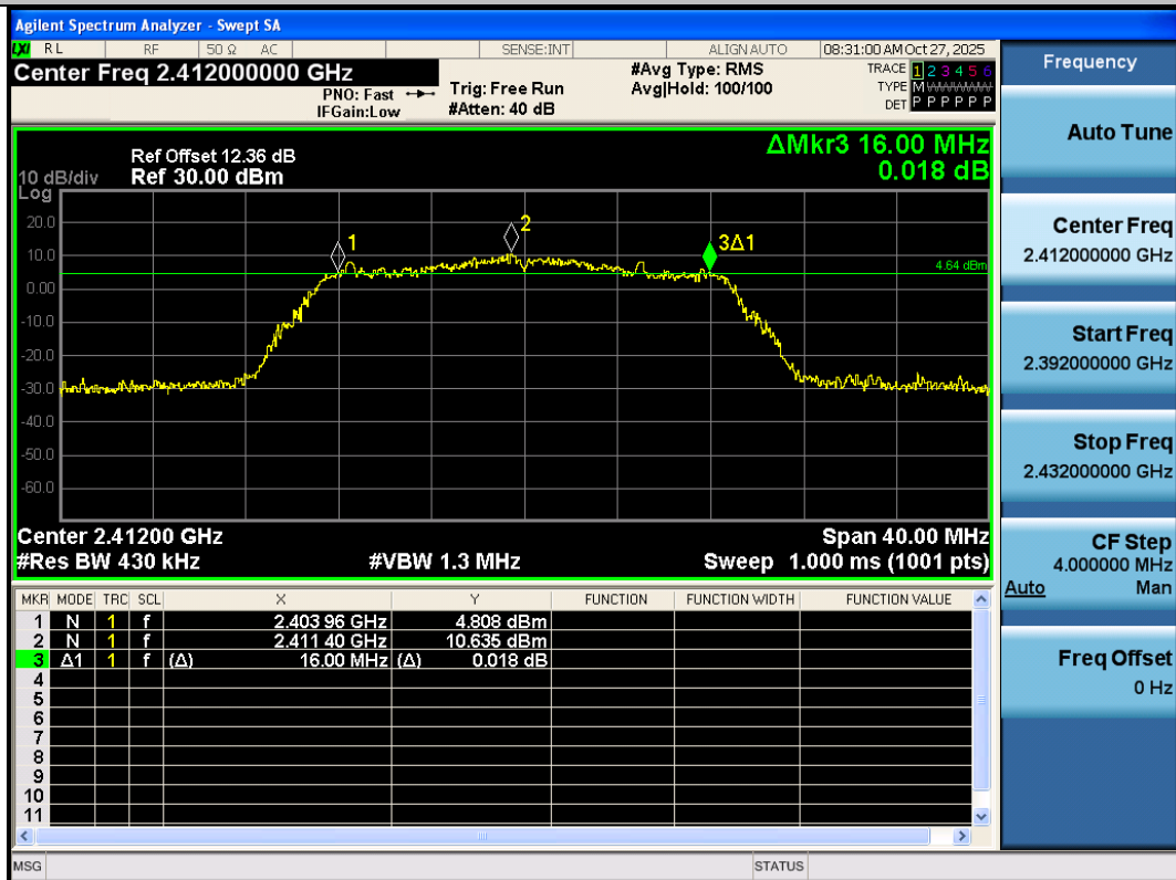
11N20SISO-Ant3-2412-PASS
