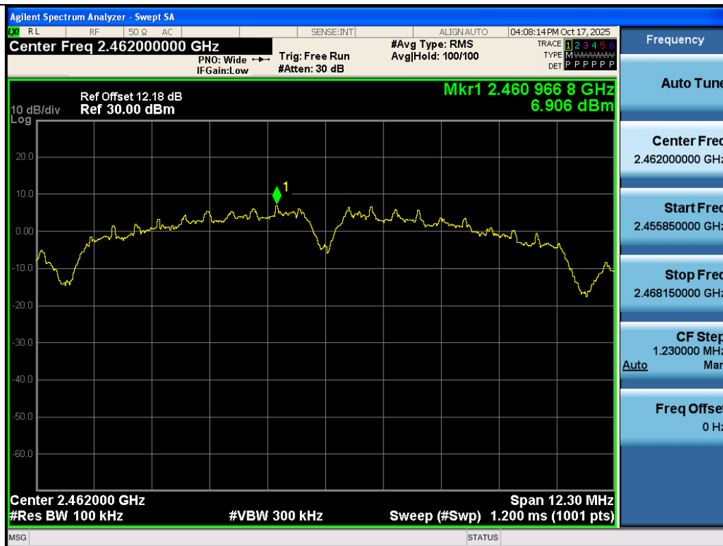
11B-Ant3-2462-PASS
