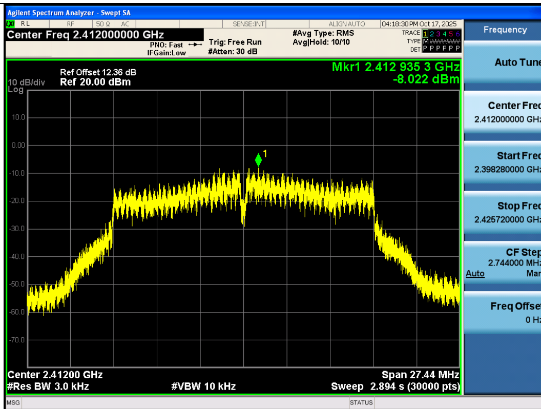
11G-Ant3-2412-PASS
