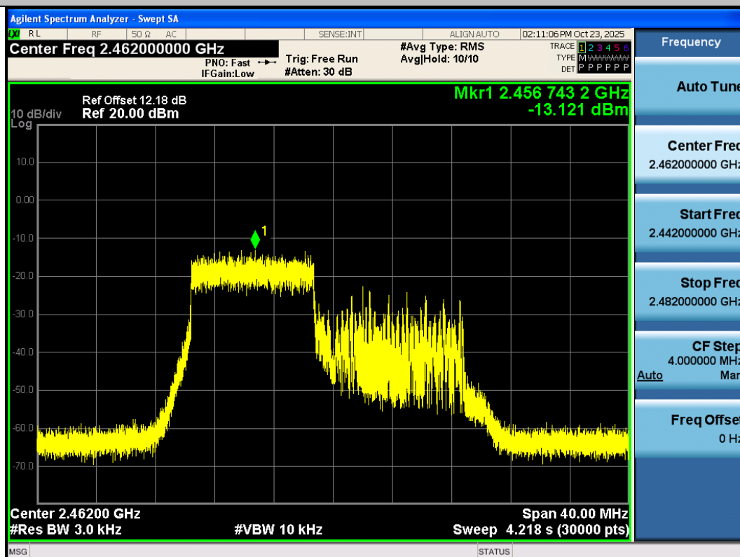
11AX20SISO-Ant3-2462-106Tone-RU53-PASS
