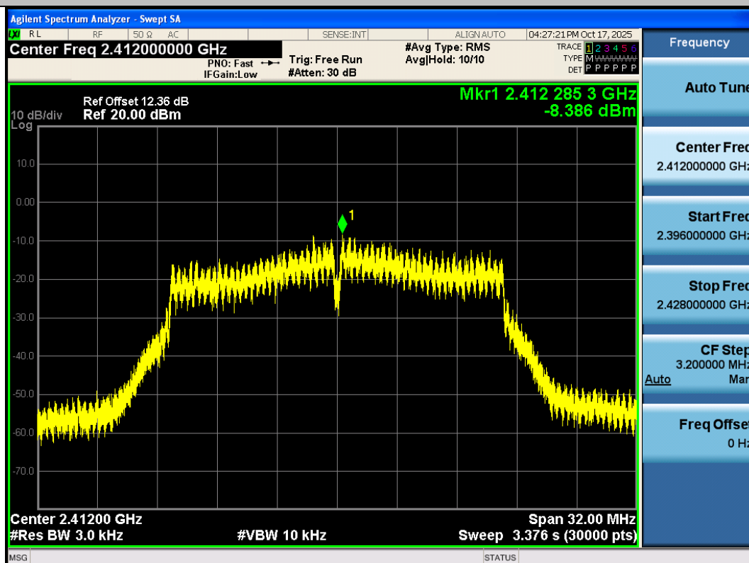
11N20SISO-Ant3-2412-PASS
