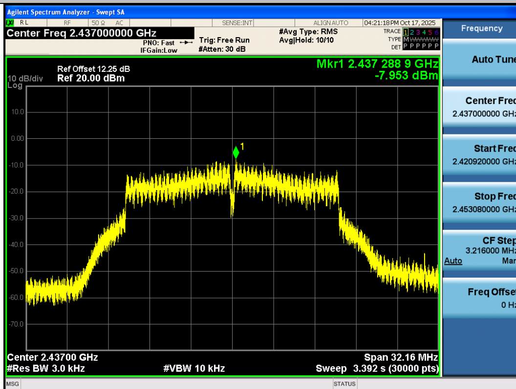
11G-Ant3-2437-PASS
