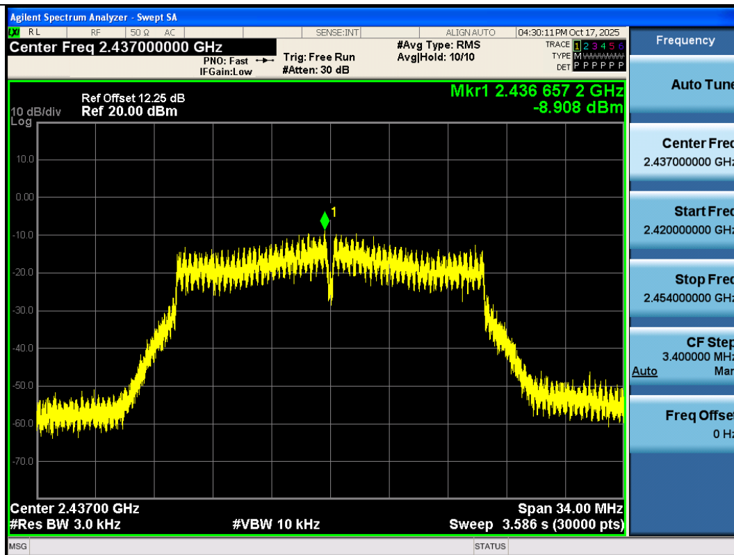
11N20SISO-Ant3-2437-PASS
