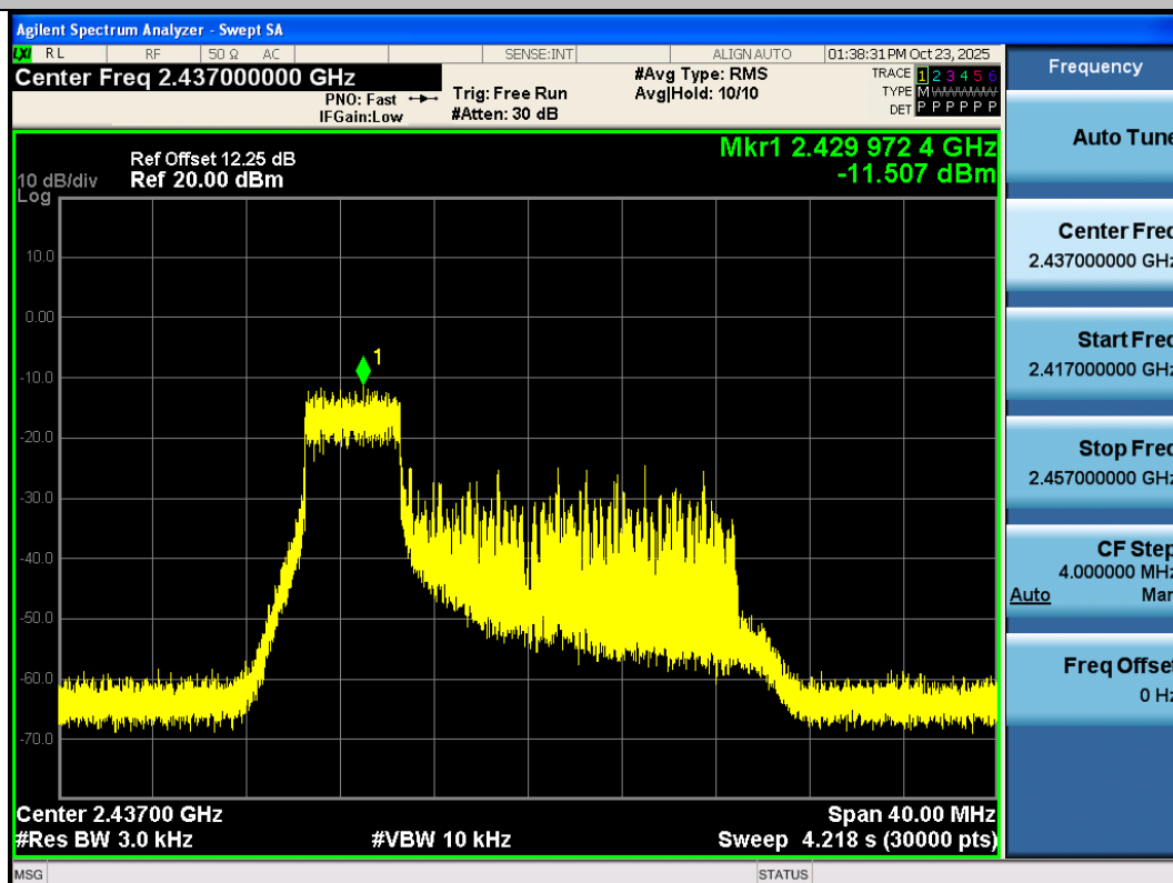
11AX20SISO-Ant3-2437-52Tone-RU37-PASS
