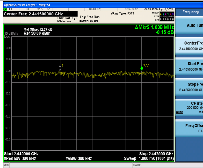
3DH5_Ant2_Hop
