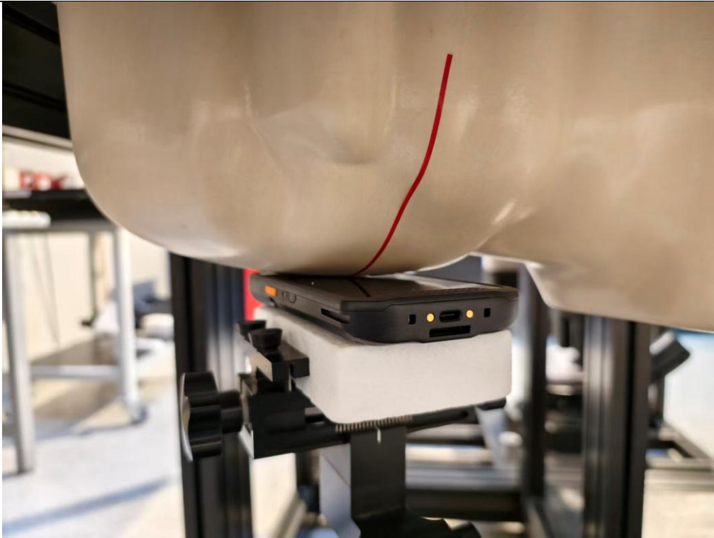
Head SAR –Right Tilted
