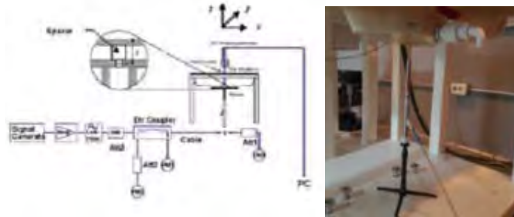
Figure 10.1 Dipole Verification Test Setup Diagram &amp; Photo
