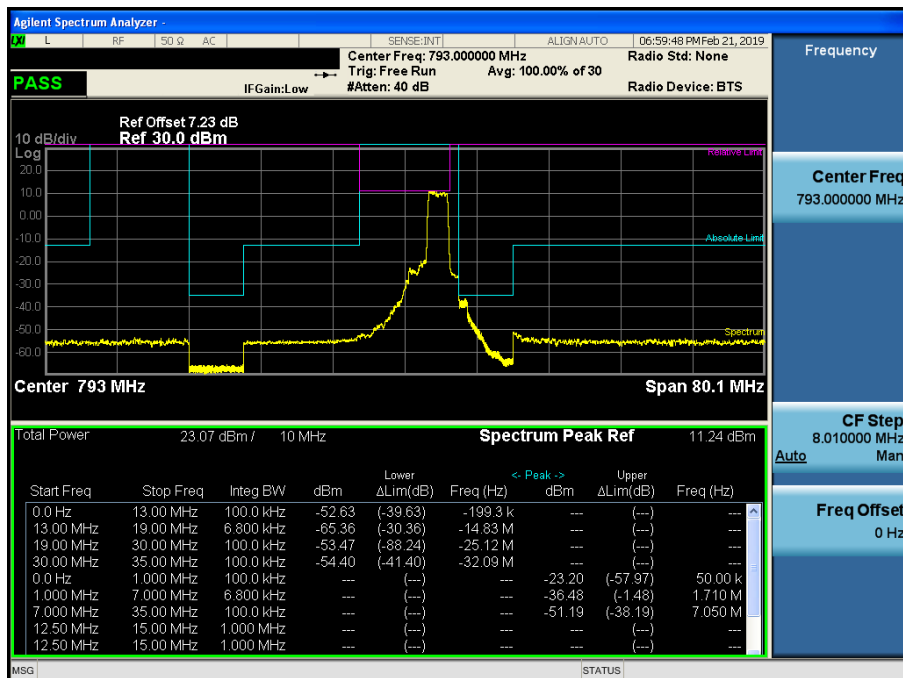
LTE Band 14 / 5MHz / QPSK - RB Size/Offset (12/13)
