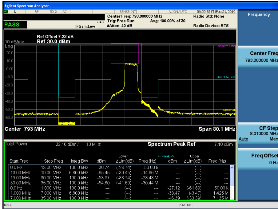
LTE Band 14 / 10MHz / 16QAM - RB Size/Offset (25/25)
