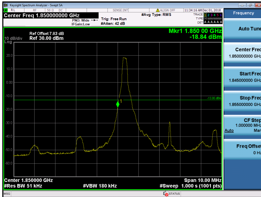
LTE Band 2 / 5MHz / 16QAM Offset/Size (1/0)
