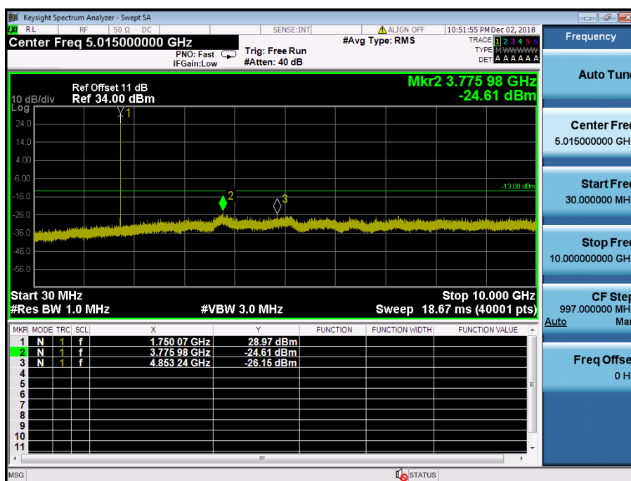
LTE Band 4 / 10MHz / QPSK - RB Size/Offset (1/25) – High Channel
