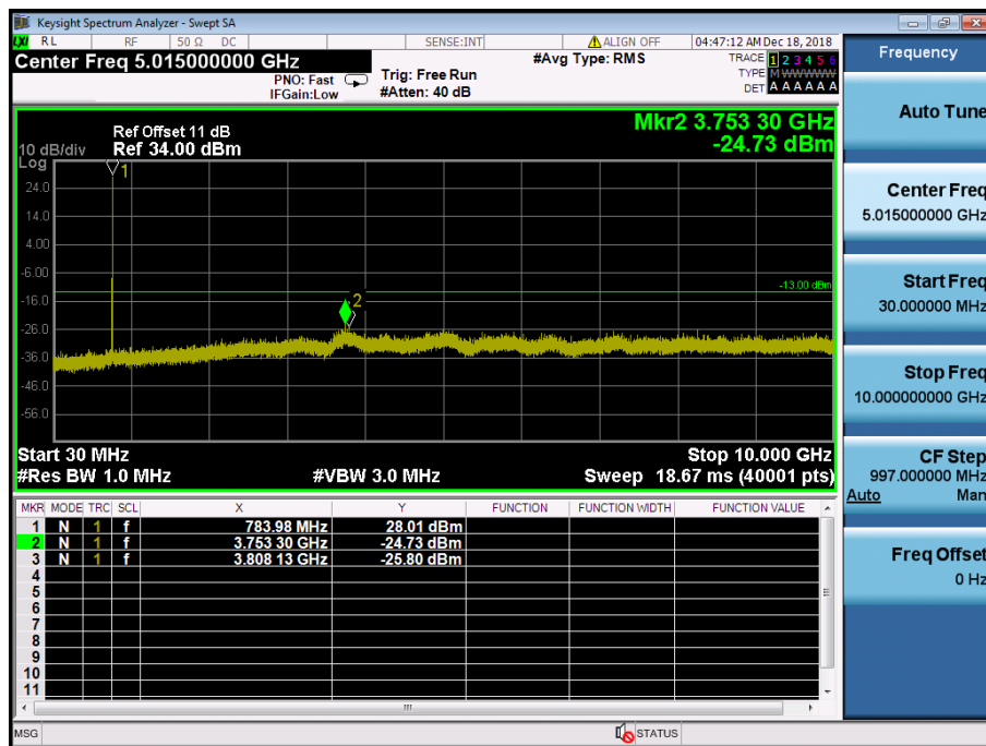
LTE Band 13 / 5MHz / 16QAM - RB Size/Offset (12/6) – High Channel
