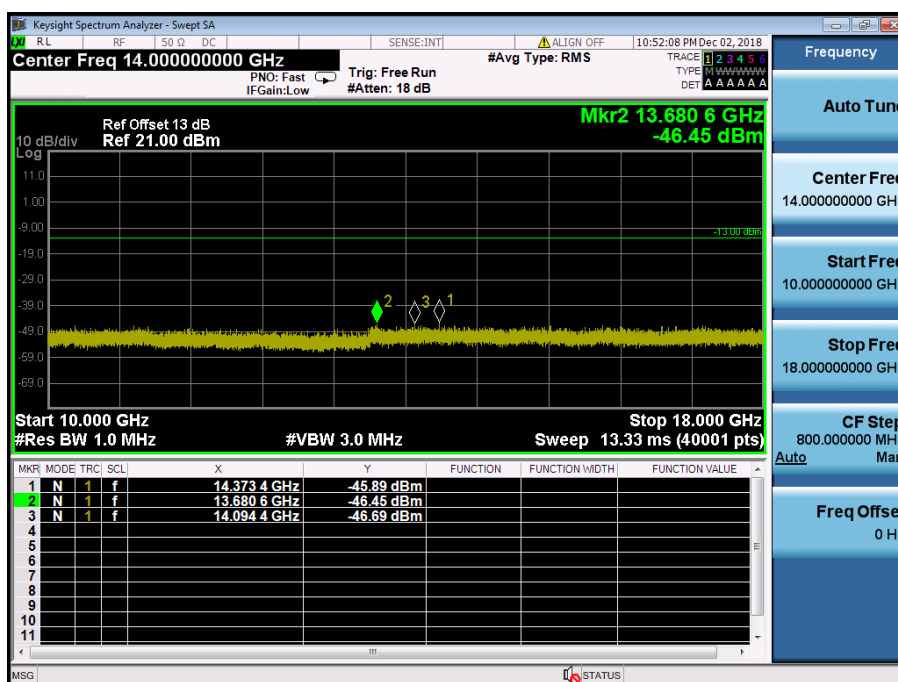
LTE Band 4 / 10MHz / QPSK - RB Size/Offset (1/25) – High Channel
