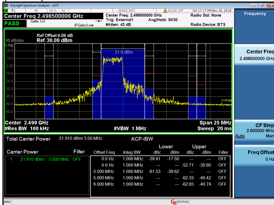
LTE Band 41 / 5MHz / QPSK - RB Size/Offset (12/0)
