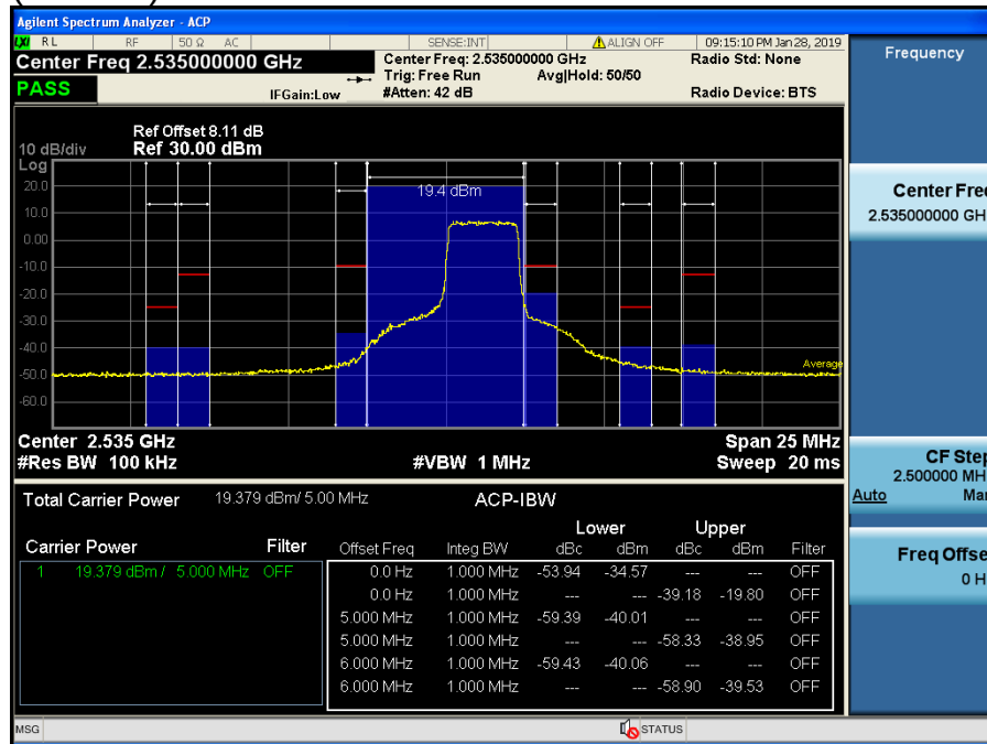
LTE Band 7 / 5MHz / 16QAM - RB Size/Offset (12/13)
