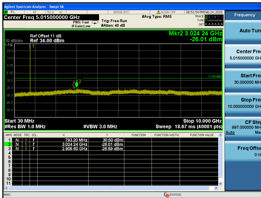
LTE Band 14 / 10MHz / QPSK - RB Size/Offset (1/25) – Low Channel
