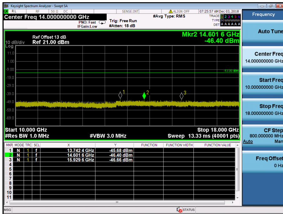
LTE Band 4 / 20MHz / 16QAM - RB Size/Offset (50/50)–Mid Channel
