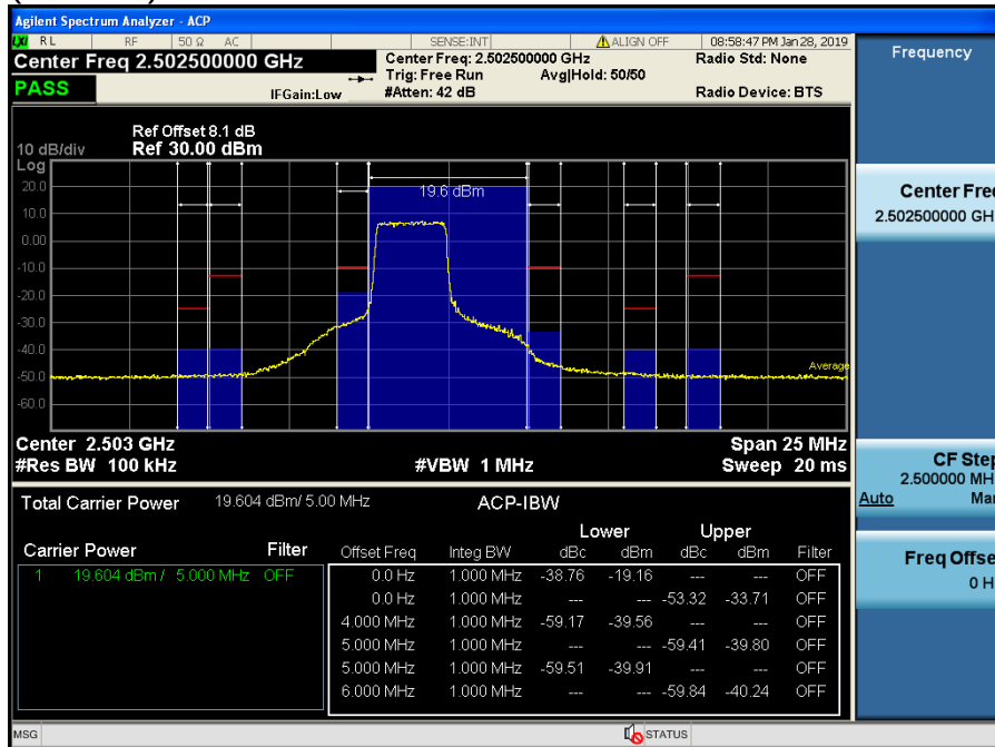
LTE Band 7 / 5MHz / 16QAM - RB Size/Offset (12/0)
