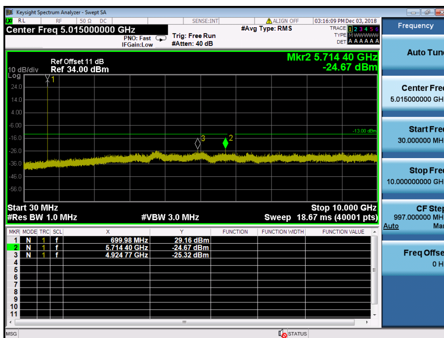
LTE Band 12 / 1.4MHz / 16QAM - RB Size/Offset (1/2) – Low Channel
