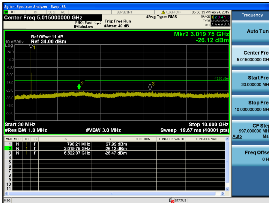
LTE Band 14 / 5MHz / 16QAM - RB Size/Offset (12/6) – Low Channel
