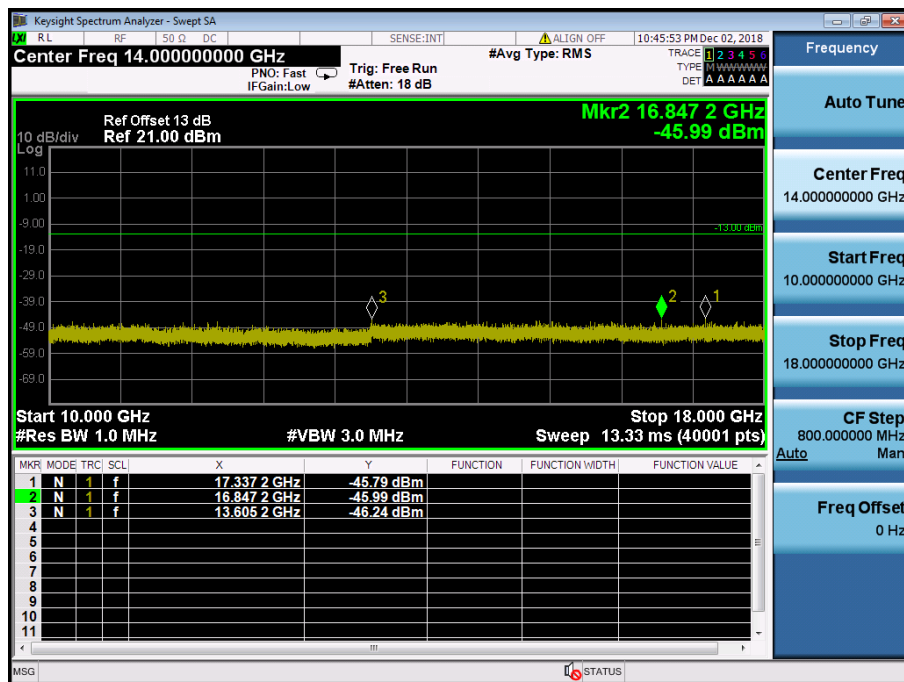
LTE Band 4 / 10MHz / QPSK - RB Size/Offset (25/25) – Mid Channel
