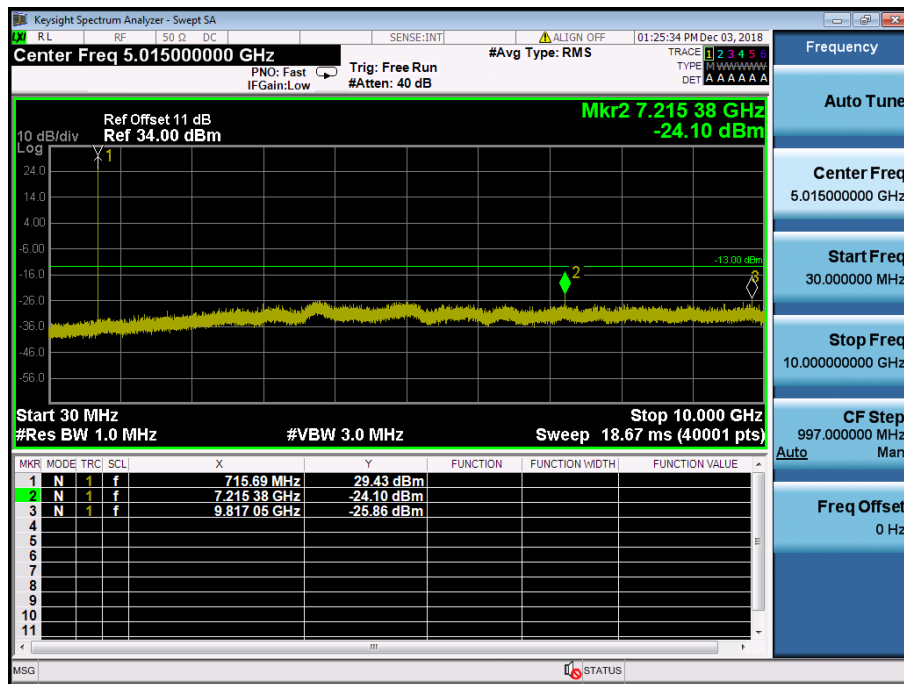
LTE Band 12 / 1.4MHz / QPSK - RB Size/Offset (3/3) – High Channel
