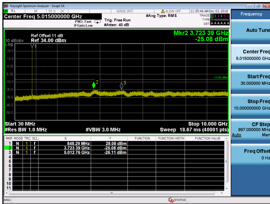
LTE Band 5 / 3MHz / 16QAM - RB Size/Offset (8/7) – High Channel
