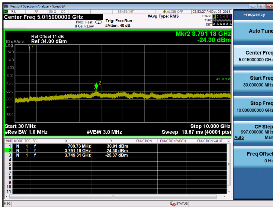
LTE Band 12 / 3MHz / 16QAM - RB Size/Offset (1/7) – Low Channel
