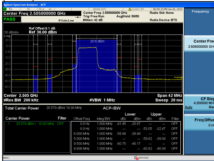
LTE Band 7 / 10MHz / QPSK - RB Size/Offset (25/0)
