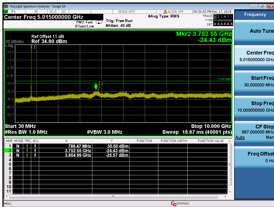
LTE Band 13 / 10MHz / 16QAM - RB Size/Offset (1/49) – Low Channel
