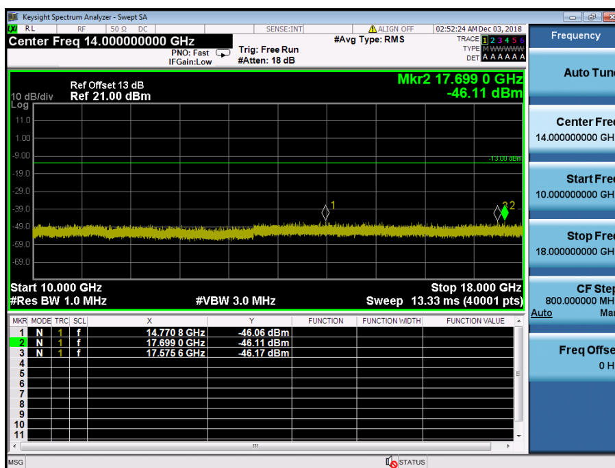
LTE Band 4 / 20MHz / QPSK - RB Size/Offset (50/25) – High Channel
