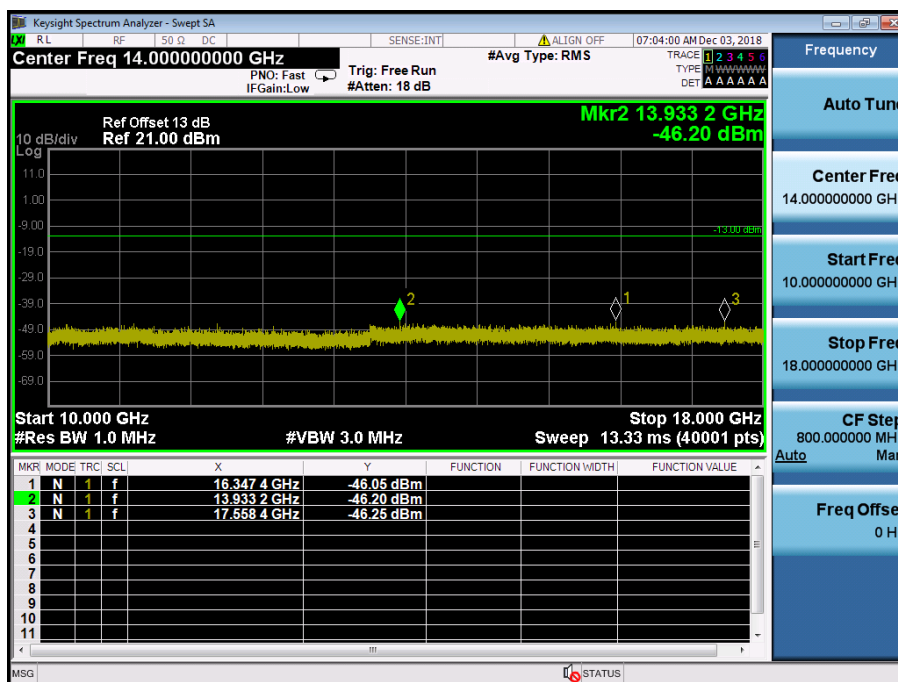
LTE Band 4 / 15MHz / 16QAM - RB Size/Offset (75/0) – High Channel
