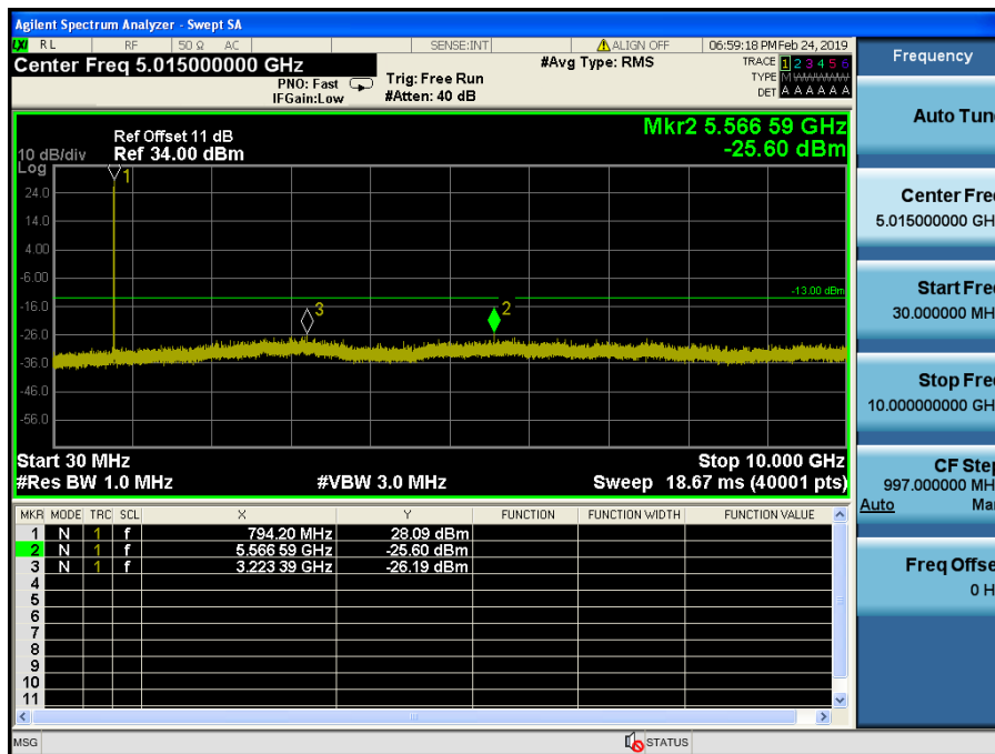
LTE Band 14 / 5MHz / 16QAM - RB Size/Offset (12/0) – High Channel
