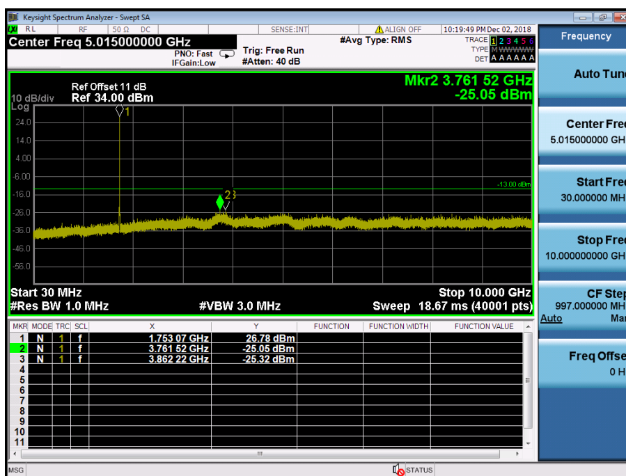
LTE Band 4 / 5MHz / QPSK - RB Size/Offset (1/24) – High Channel
