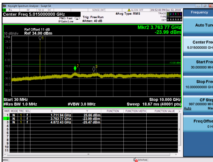
LTE Band 4 / 5MHz / QPSK - RB Size/Offset (12/6) – Low Channel
