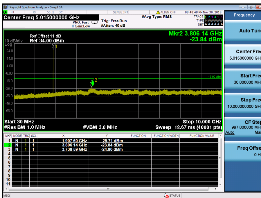
LTE Band 2 / 5MHz / QPSK - RB Size/Offset (1/12) – High Channel
