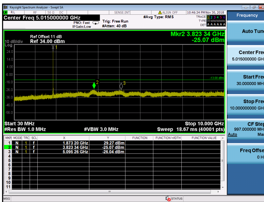
LTE Band 2 / 15MHz / QPSK - RB Size/Offset (1/0) – Mid Channel
