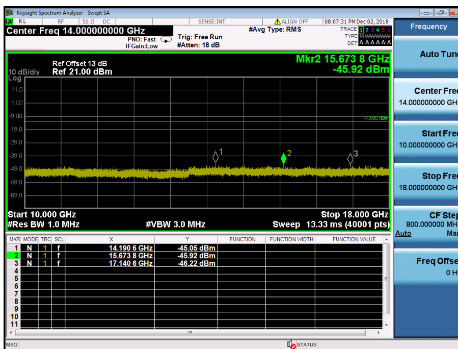
LTE Band 4 / 1.4MHz / QPSK - RB Size/Offset (3/0) – Low Channel
