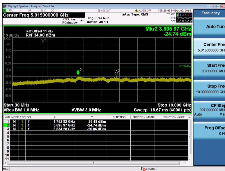
LTE Band 4 / 3MHz / QPSK - RB Size/Offset (1/14) – High Channel
