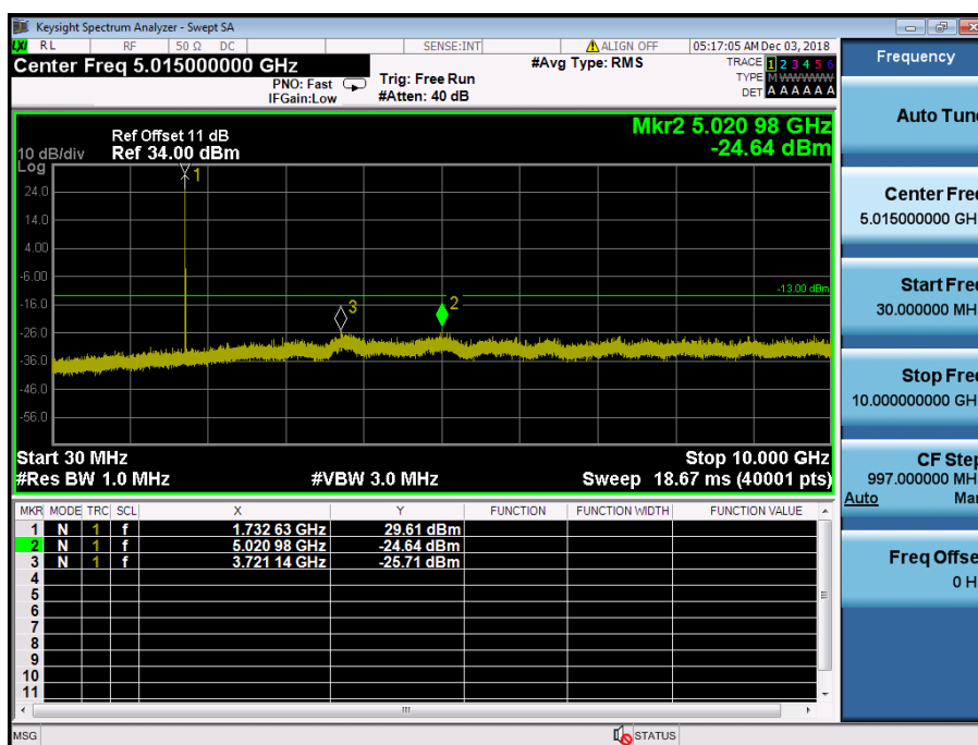
LTE Band 4 / 5MHz / 16QAM - RB Size/Offset (1/12) – Mid Channel
