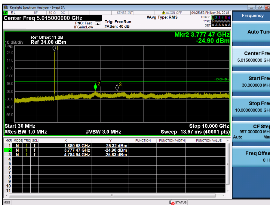
LTE Band 2 / 10MHz / QPSK - RB Size/Offset (25/25) – Mid Channel
