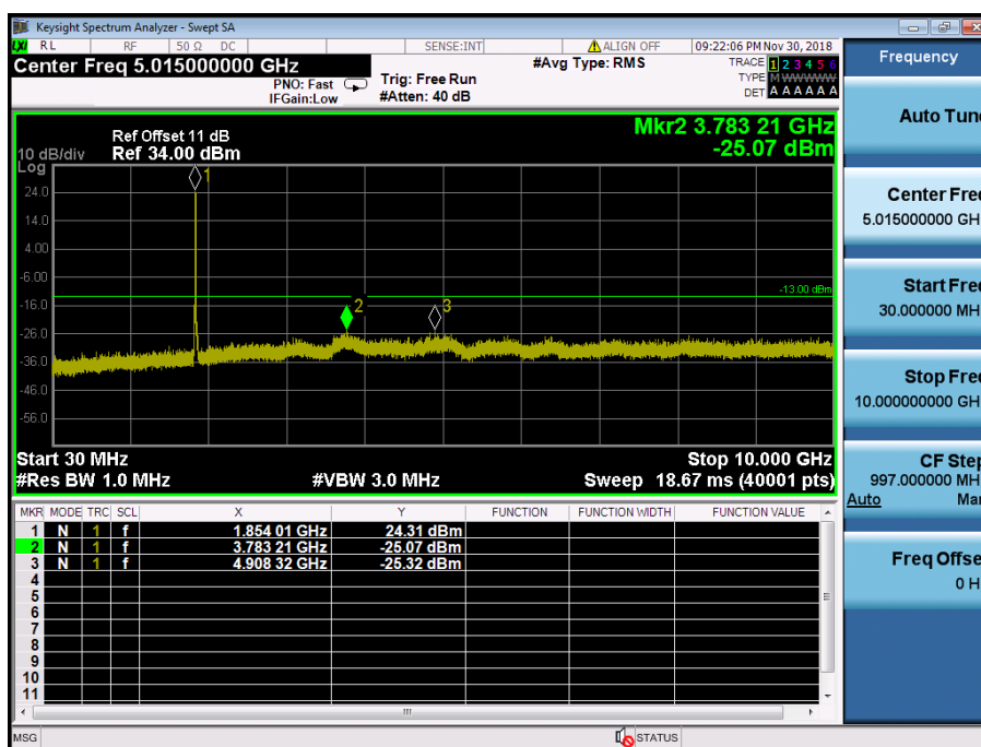
LTE Band 2 / 10MHz / QPSK - RB Size/Offset (50/0) – Low Channel
