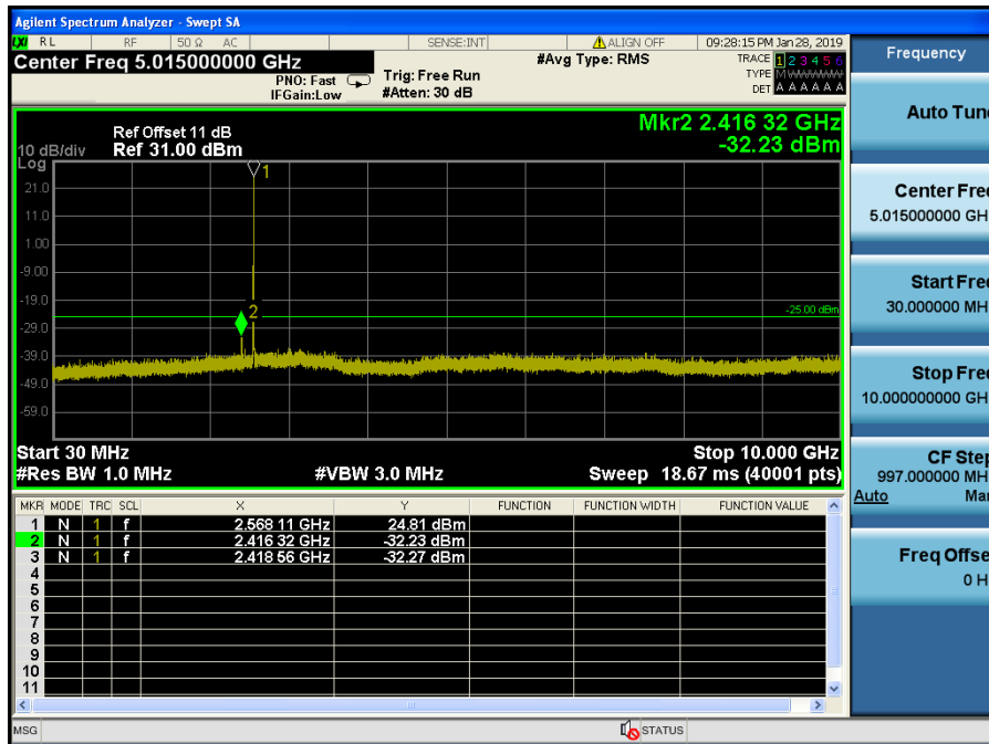
LTE Band 7 / 5MHz / 16QAM - RB Size/Offset (12/13) – High Channel
