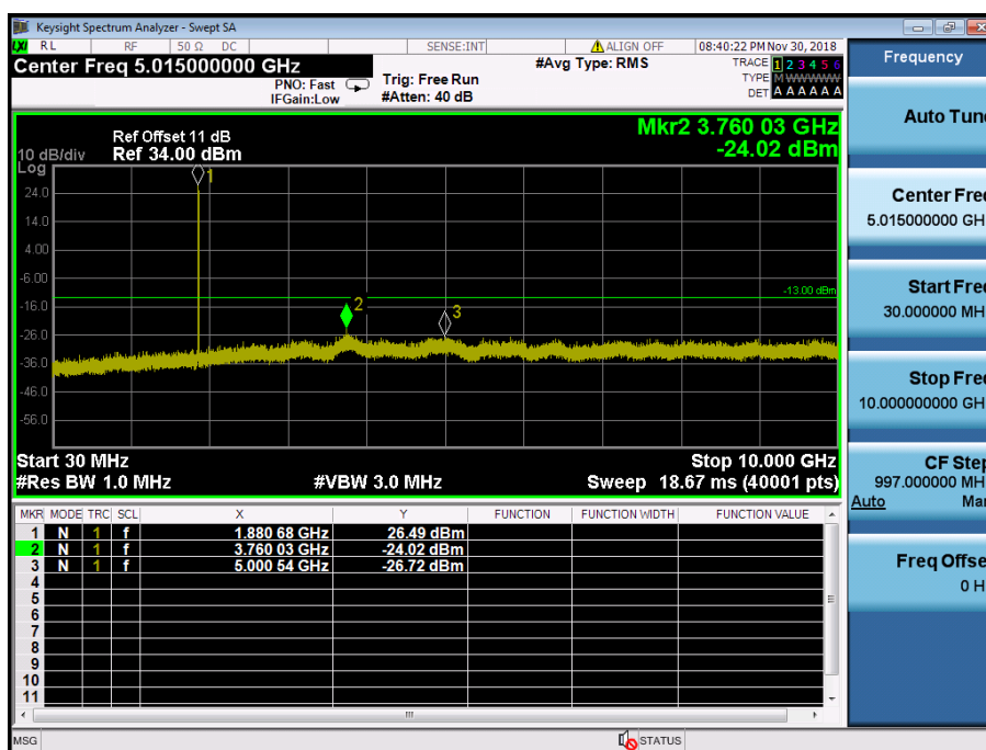
LTE Band 2 / 5MHz / QPSK - RB Size/Offset (12/6) – Mid Channel
