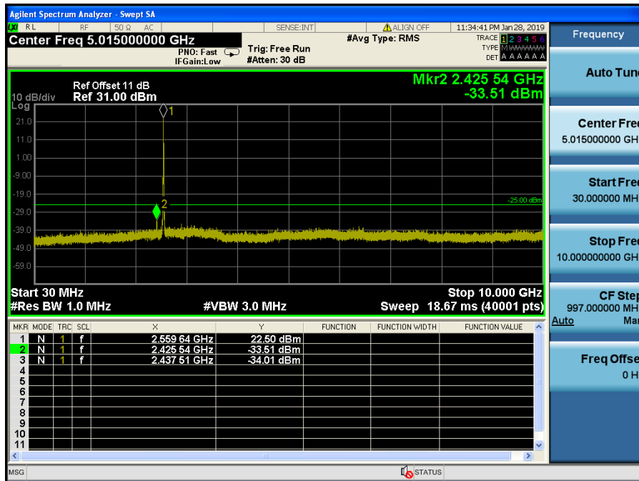
LTE Band 7 / 20MHz / 16QAM- RB Size/Offset (50/25) – High Channel
