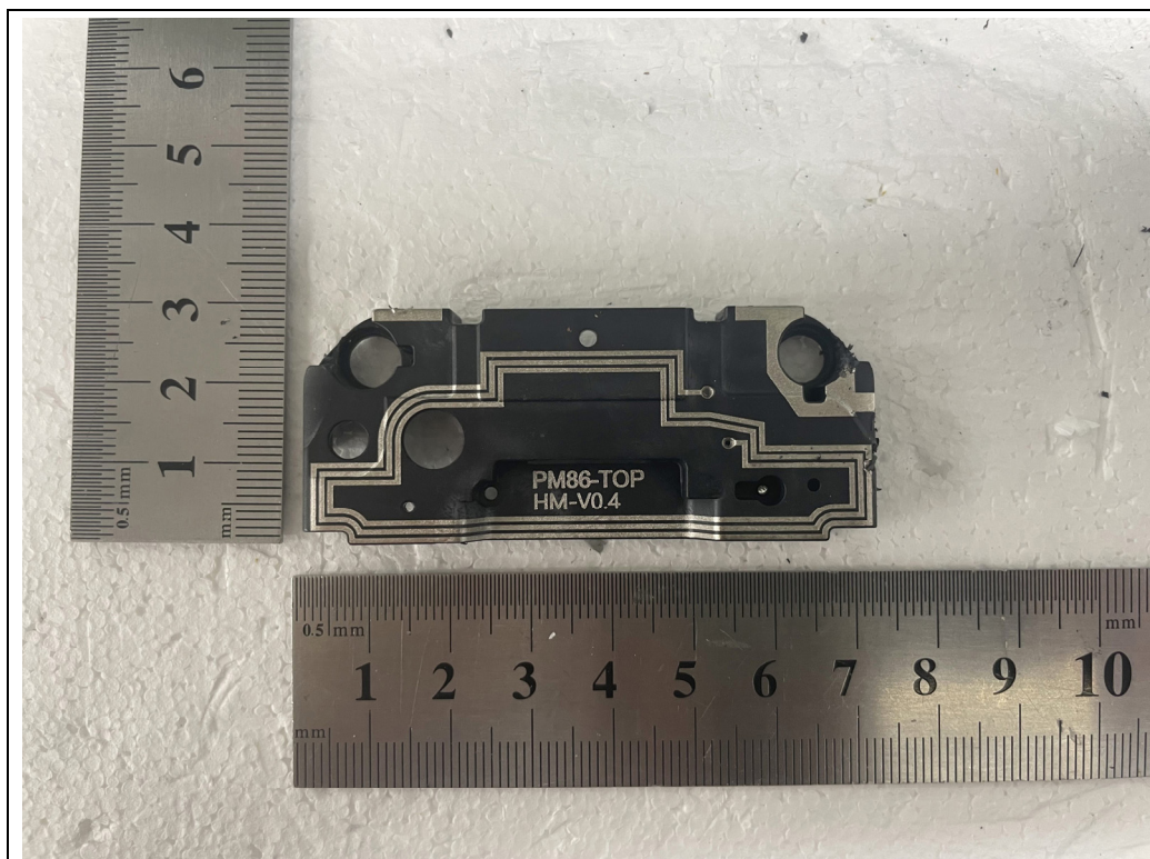
TOP(WWAN RX, BLE, WLAN, NFC) Antenna
