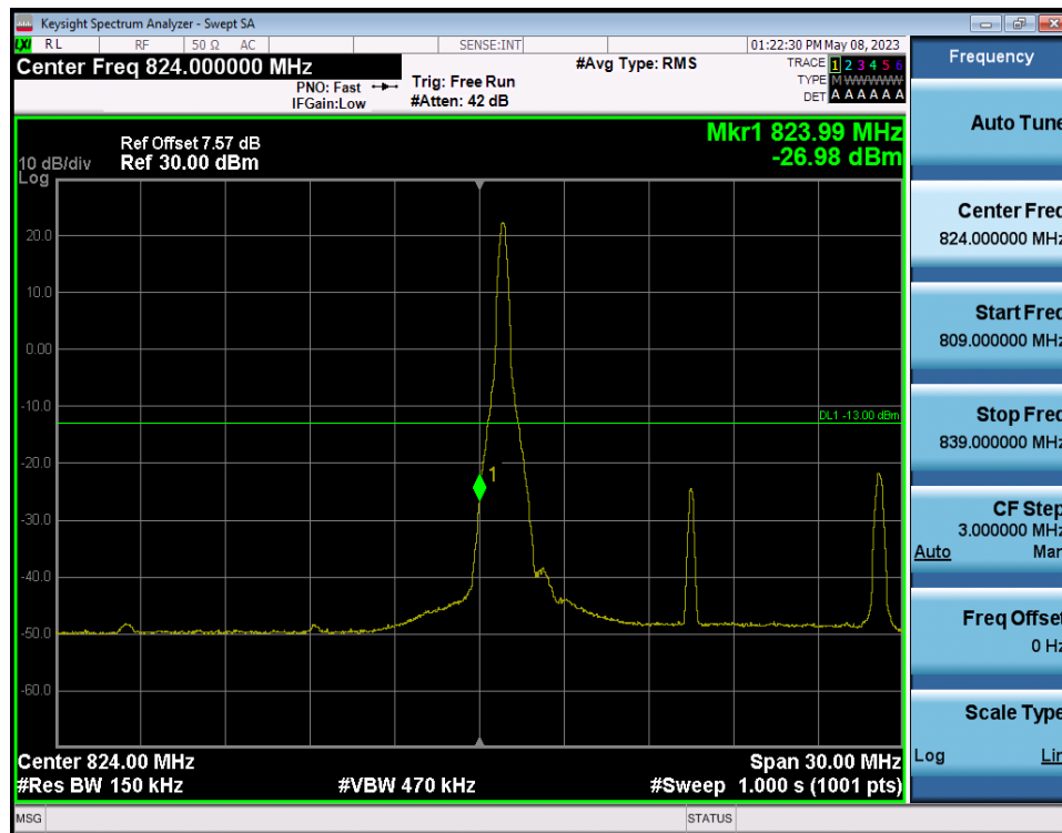
LTE Band 26 / 15MHz / QPSK - RB Size/Offset (1/0)
