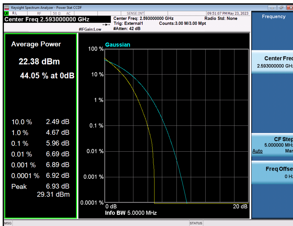
LTE Band 41(38) / 5MHz / QPSK - RB Size 25
