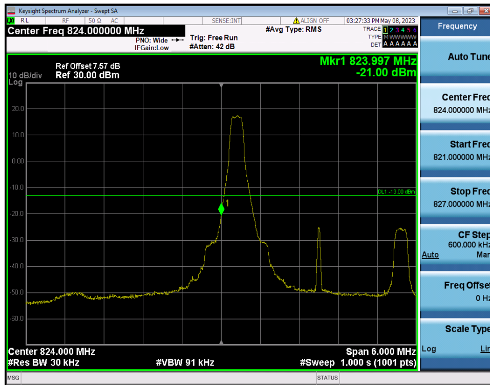
LTE Band 26(5) / 3MHz / QPSK - RB Size/Offset (1/0)
