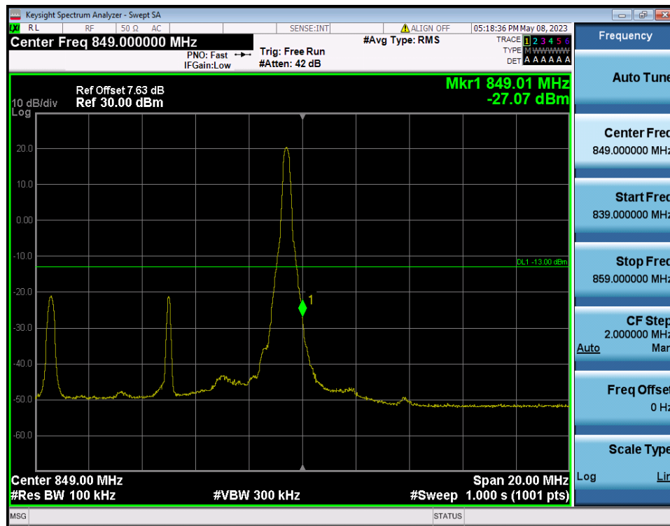
LTE Band 26(5) / 10MHz / 16QAM - RB Size/Offset (1/49)
