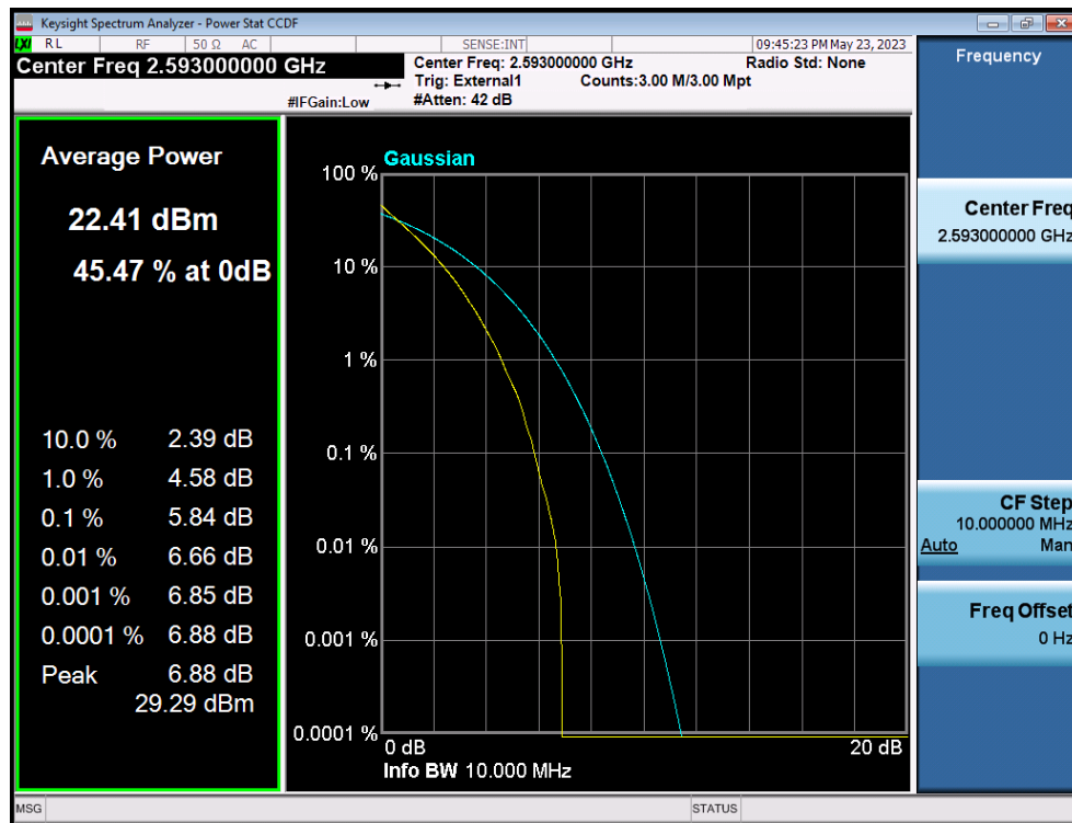
LTE Band 41(38) / 10MHz / QPSK - RB Size 50
