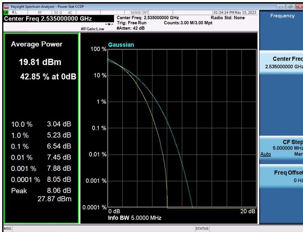
LTE Band 7 / 5MHz / 64QAM - RB Size 25
