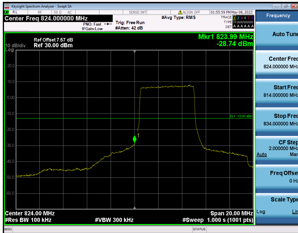
LTE Band 26(5) / 10MHz / QPSK - RB Size/Offset (25/0)
