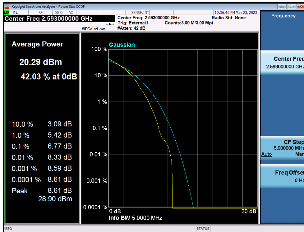
LTE Band 41(38) / 5MHz / 64QAM - RB Size 25
