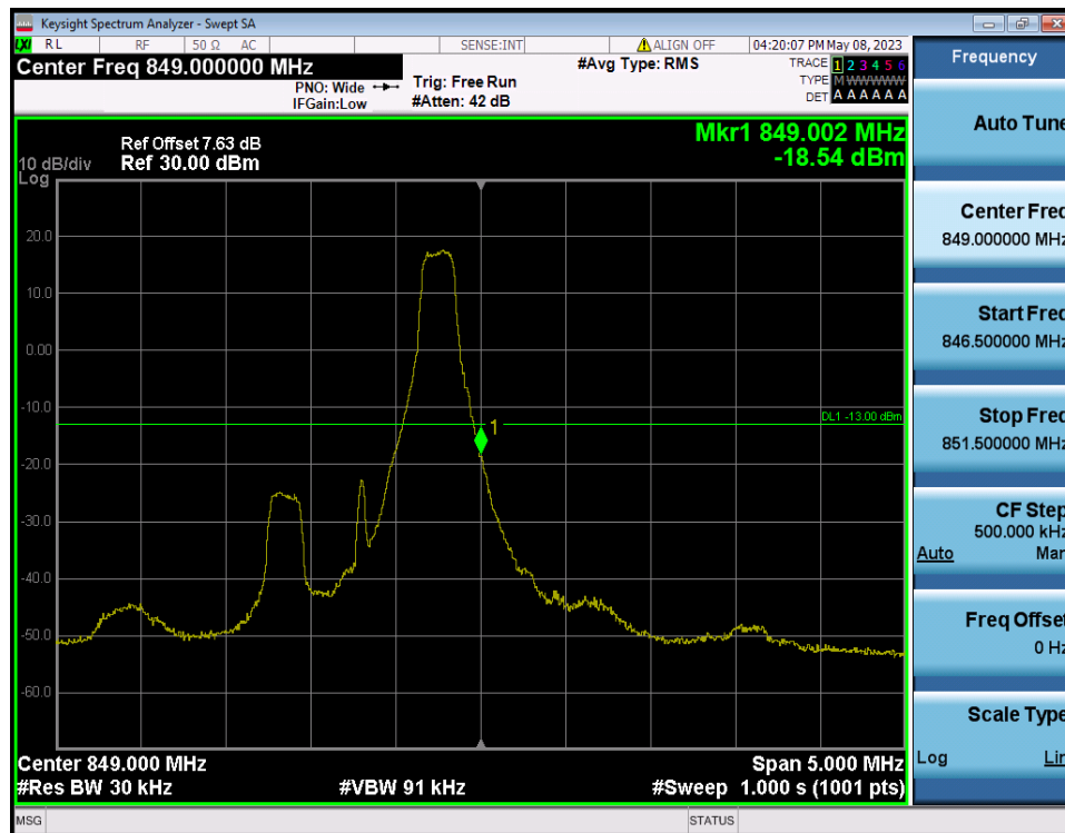
LTE Band 26(5) / 1.4MHz / QPSK - RB Size/Offset (1/5)
