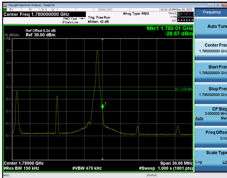
LTE Band 66(4) / 15MHz / 64QAM - RB Size/Offset (1/74)
