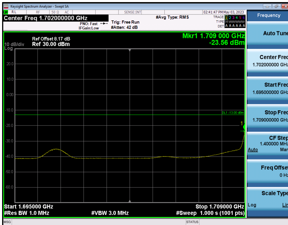
LTE Band 66(4) / 15MHz / QPSK - RB Size/Offset (1/0)
