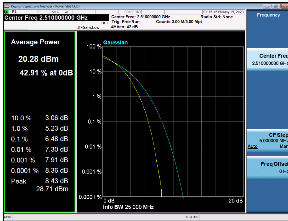
LTE Band 7 / 20MHz / 64QAM - RB Size 100
