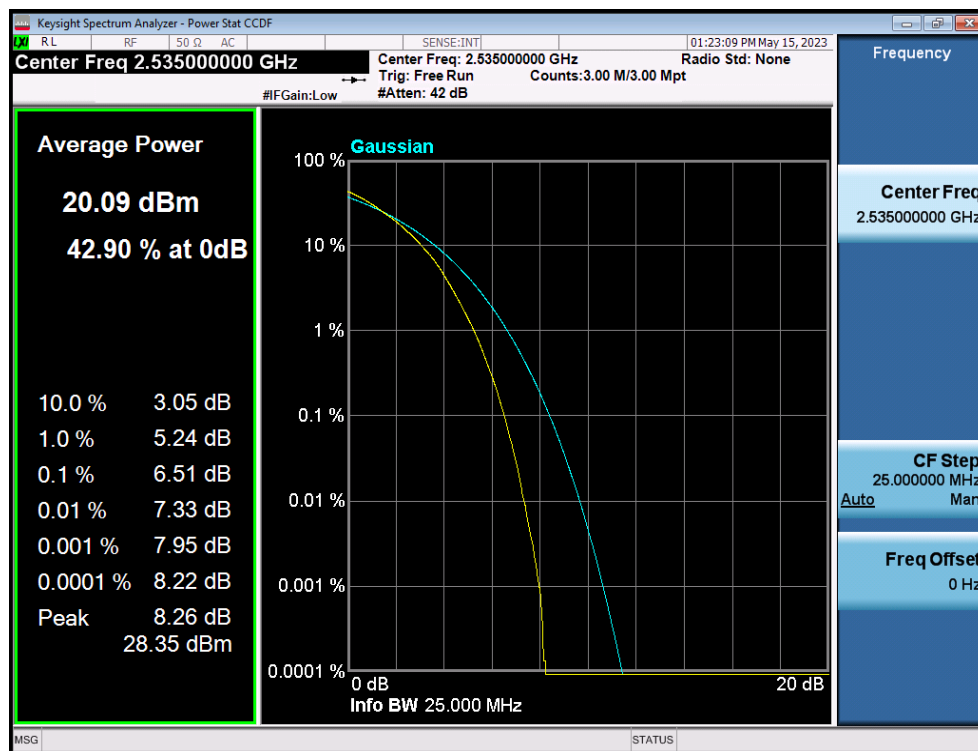
LTE Band 7 / 15MHz / 64QAM - RB Size 75
