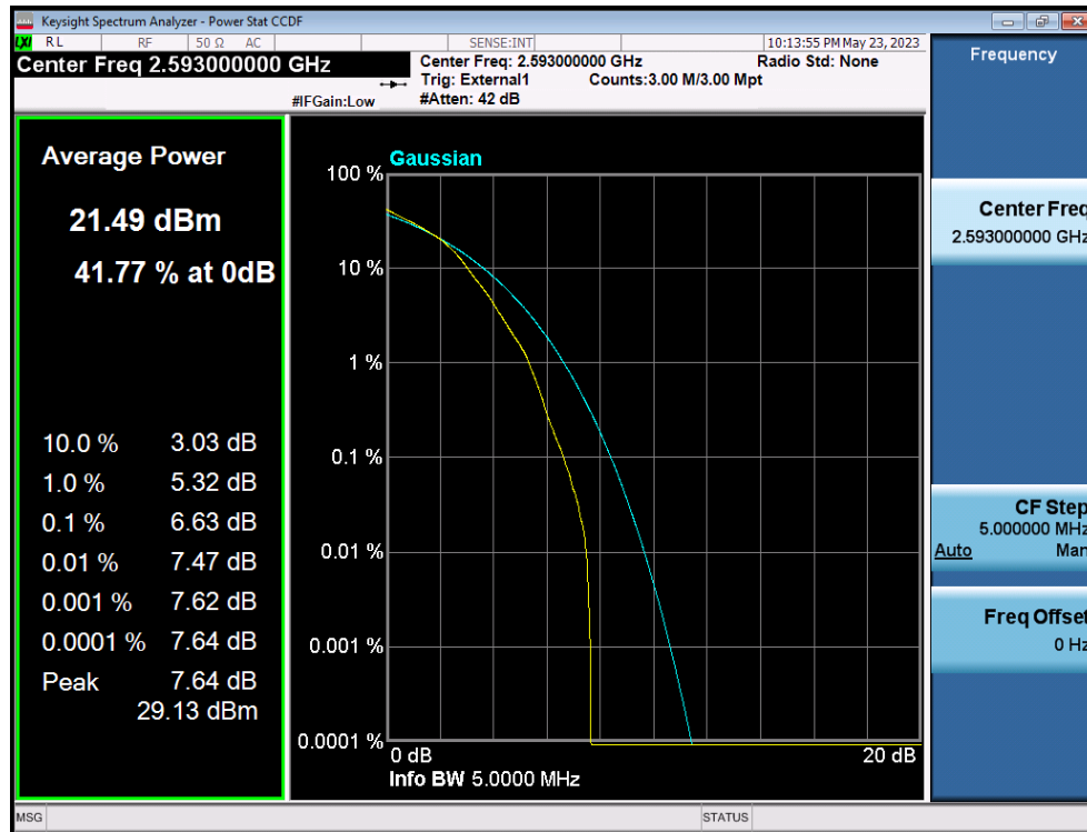
LTE Band 41(38) / 5MHz / 16QAM - RB Size 25
