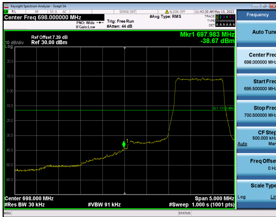
LTE Band 12 / 1.4MHz / QPSK - RB Size/Offset (6/0)
