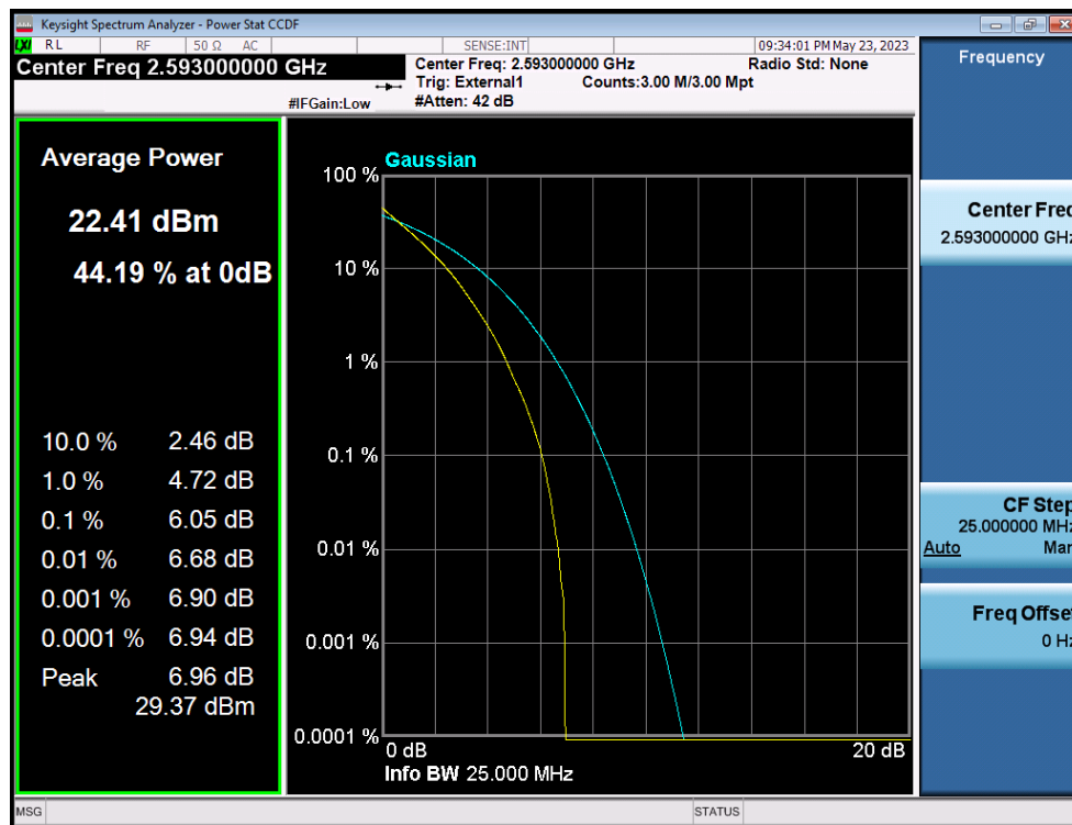
LTE Band 41(38) / 20MHz / QPSK - RB Size 100
