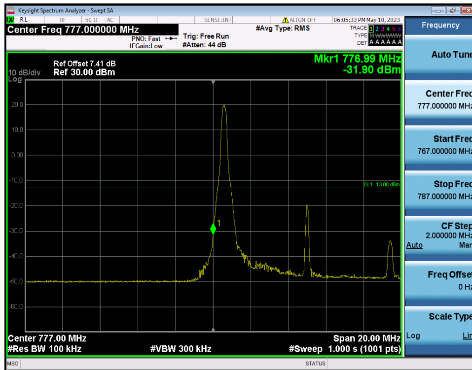
LTE Band 13 / 10MHz / 16QAM - RB Size/Offset (1/0)
