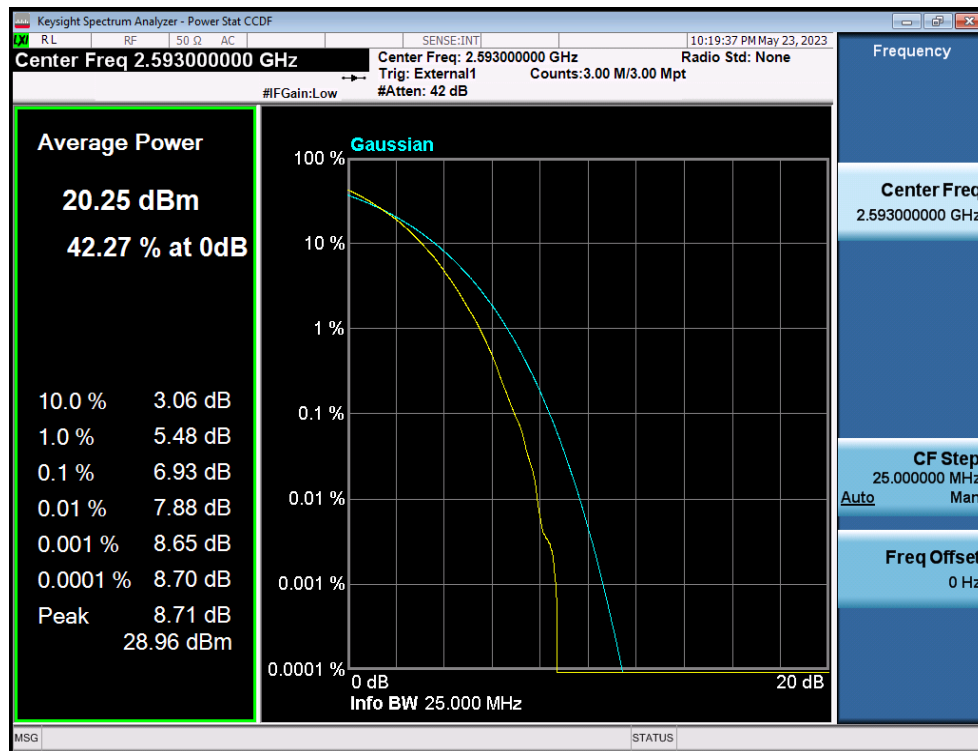
LTE Band 41(38) / 20MHz / 64QAM - RB Size 100
