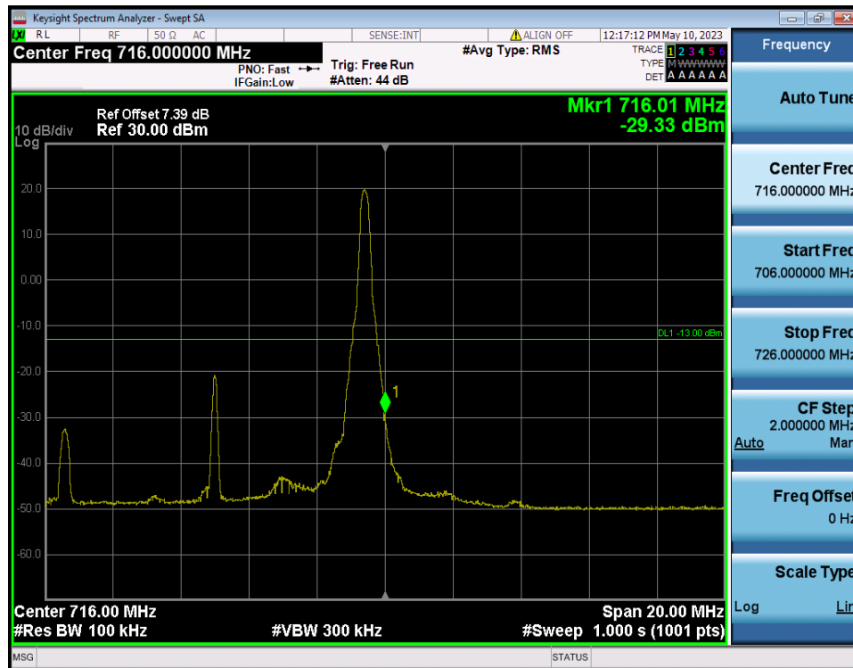
LTE Band 12(17) / 10MHz / 16QAM - RB Size/Offset (1/49)
