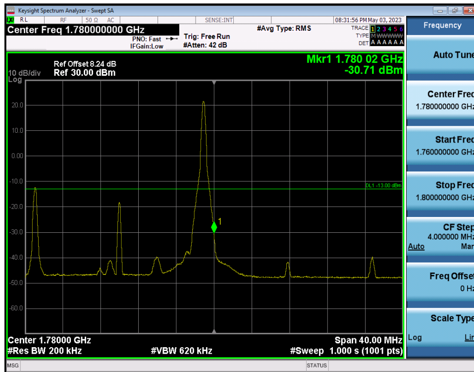
LTE Band 66(4) / 20MHz / 16QAM - RB Size/Offset (1/99)
