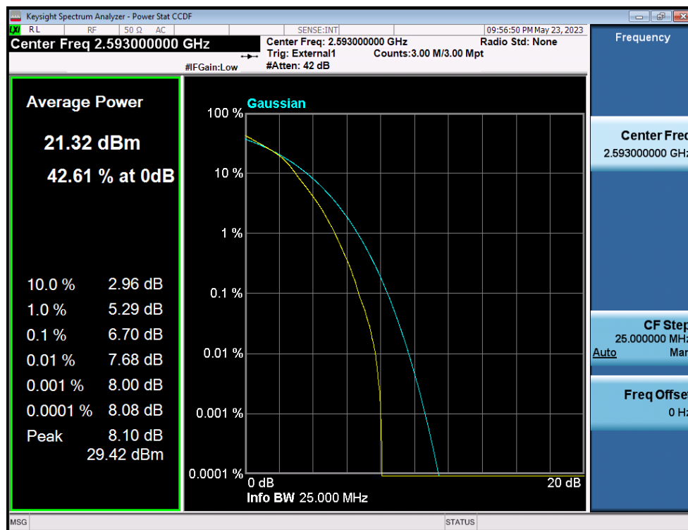
LTE Band 41(38) / 20MHz / 16QAM - RB Size 100
