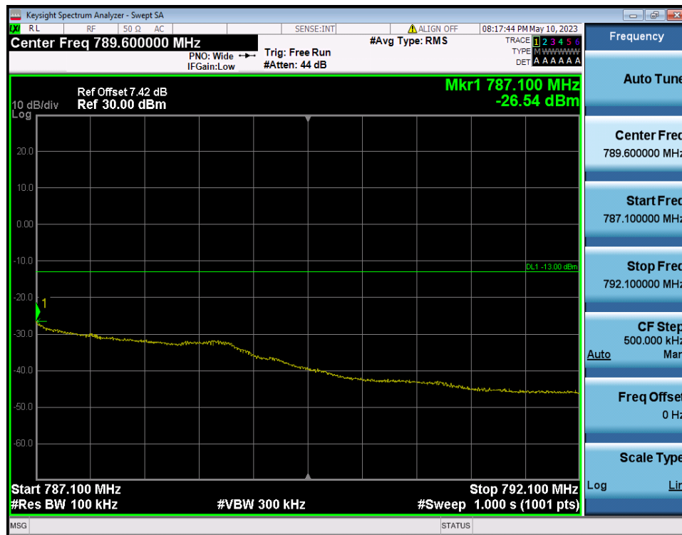
LTE Band 13 / 5MHz / QPSK - RB Size/Offset (12/13)
