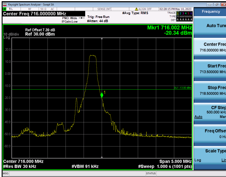
LTE Band 12 / 1.4MHz / 16QAM - RB Size/Offset (1/5)
