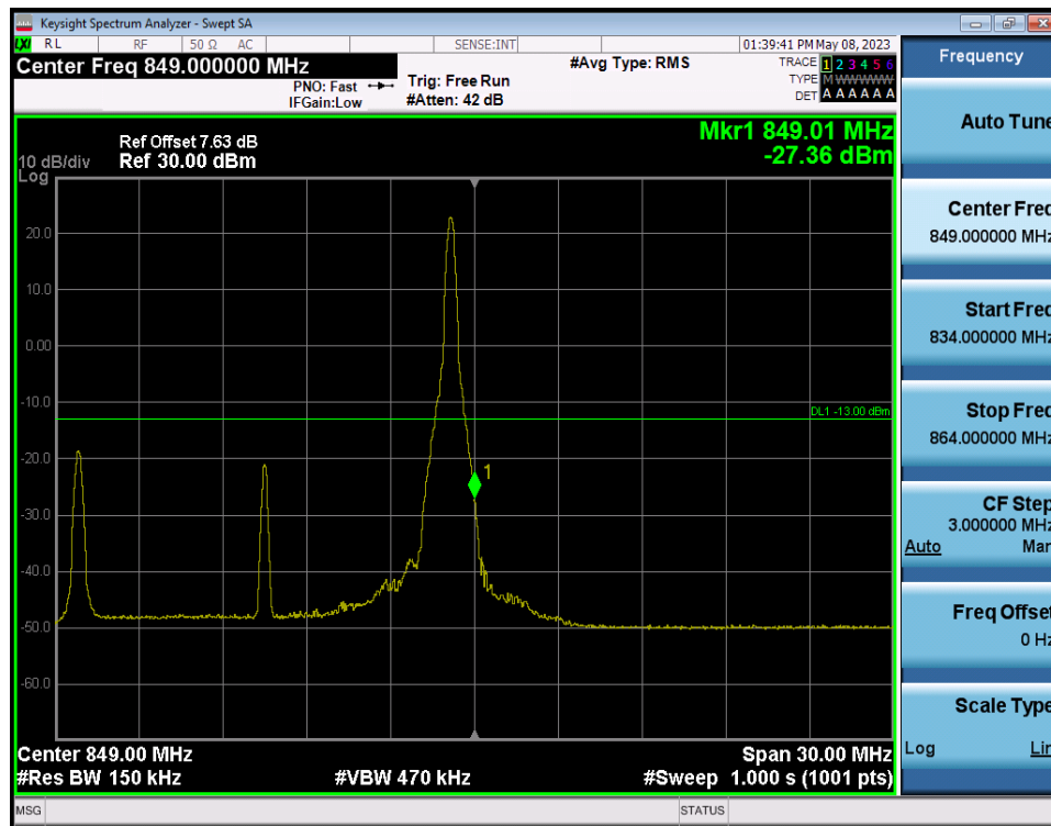
LTE Band 26 / 15MHz / QPSK - RB Size/Offset (1/74)
