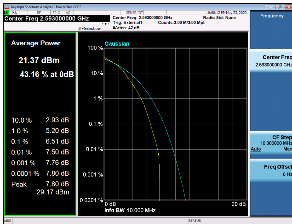
LTE Band 41(38) / 10MHz / 16QAM - RB Size 50
