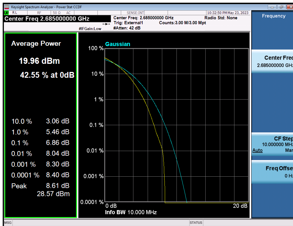
LTE Band 41(38) / 10MHz / 64QAM - RB Size 50
