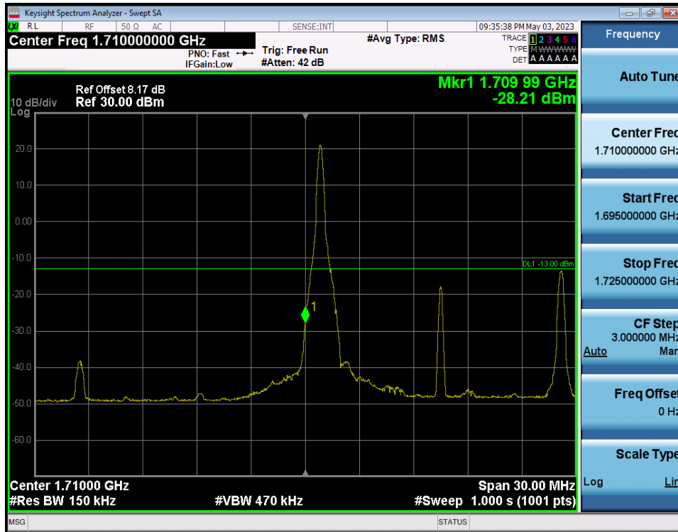
LTE Band 66(4) / 15MHz / 16QAM - RB Size/Offset (1/0)
