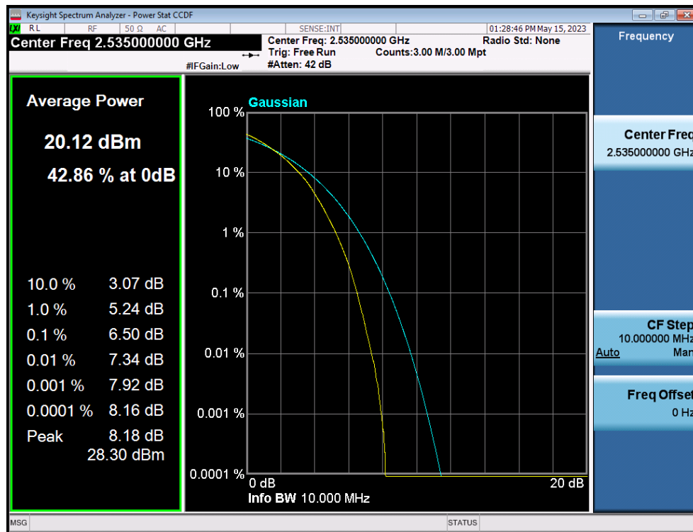
LTE Band 7 / 10MHz / 64QAM - RB Size 50
