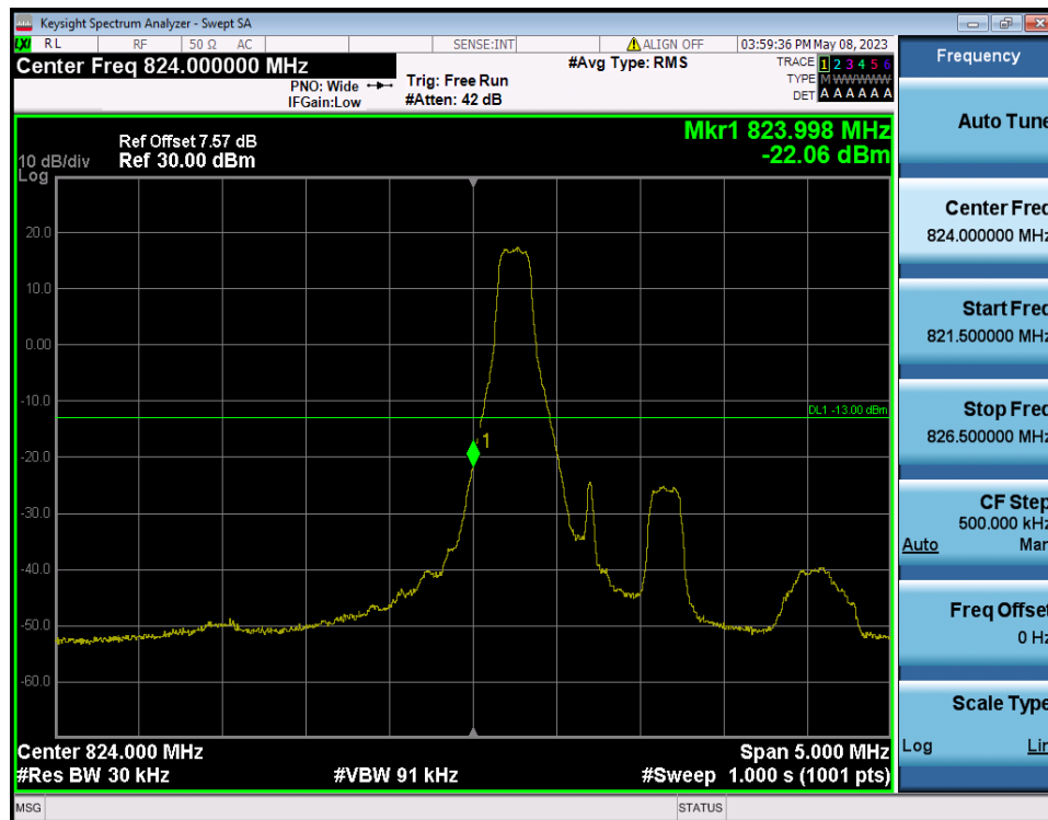
LTE Band 26(5) / 1.4MHz / QPSK - RB Size/Offset (1/0)
