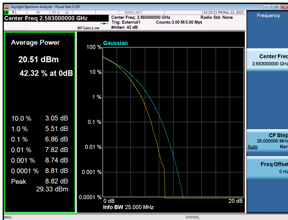
LTE Band 41(38) / 15MHz / 64QAM - RB Size 75
