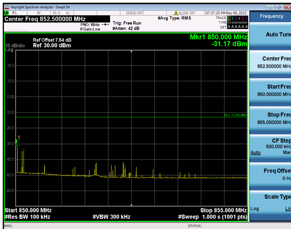
LTE Band 26(5) / 1.4MHz / 16QAM - RB Size/Offset (1/0)
