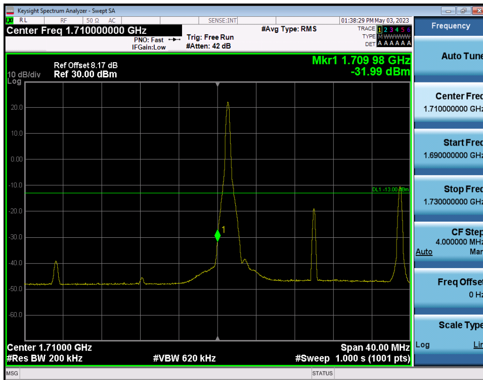
LTE Band 66(4) / 20MHz / QPSK - RB Size/Offset (1/0)
