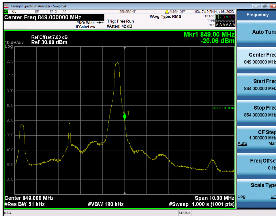
LTE Band 26(5) / 5MHz / QPSK - RB Size/Offset (1/24)
