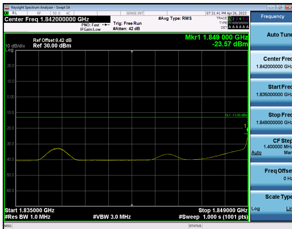
LTE Band 25(2) / 15MHz / QPSK - RB Size/Offset (1/0)
