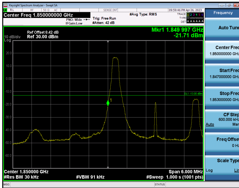
LTE Band 25(2) / 3MHz / QPSK - RB Size/Offset (1/0)
