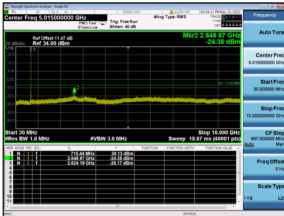
LTE Band 12(17) / 10MHz / 64QAM - RB Size/Offset (1/49) – High Channel
