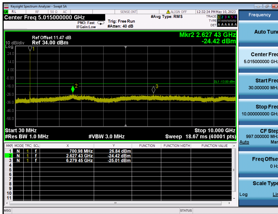
LTE Band 12(17) / 5MHz / 16QAM - RB Size/Offset (12/0) - Low Channel
