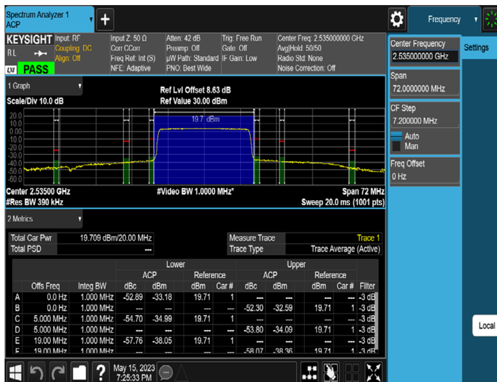
LTE Band 7 / 20MHz / QPSK - RB Size/Offset (100/0)
