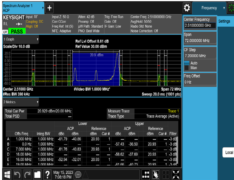
LTE Band 7 / 20MHz / QPSK - RB Size/Offset (1/99)
