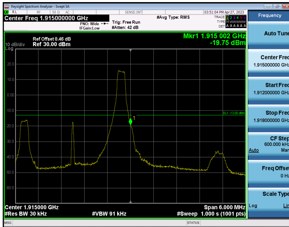
LTE Band 25(2) / 3MHz / 16QAM - RB Size/Offset (1/14)
