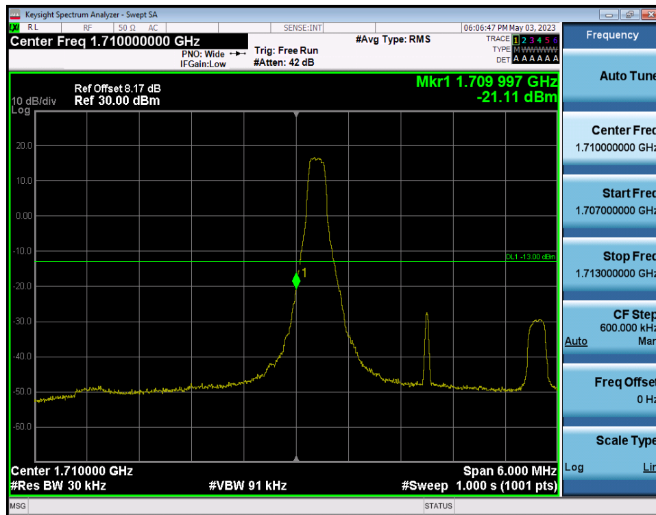
LTE Band 66(4) / 3MHz / QPSK - RB Size/Offset (1/0)
