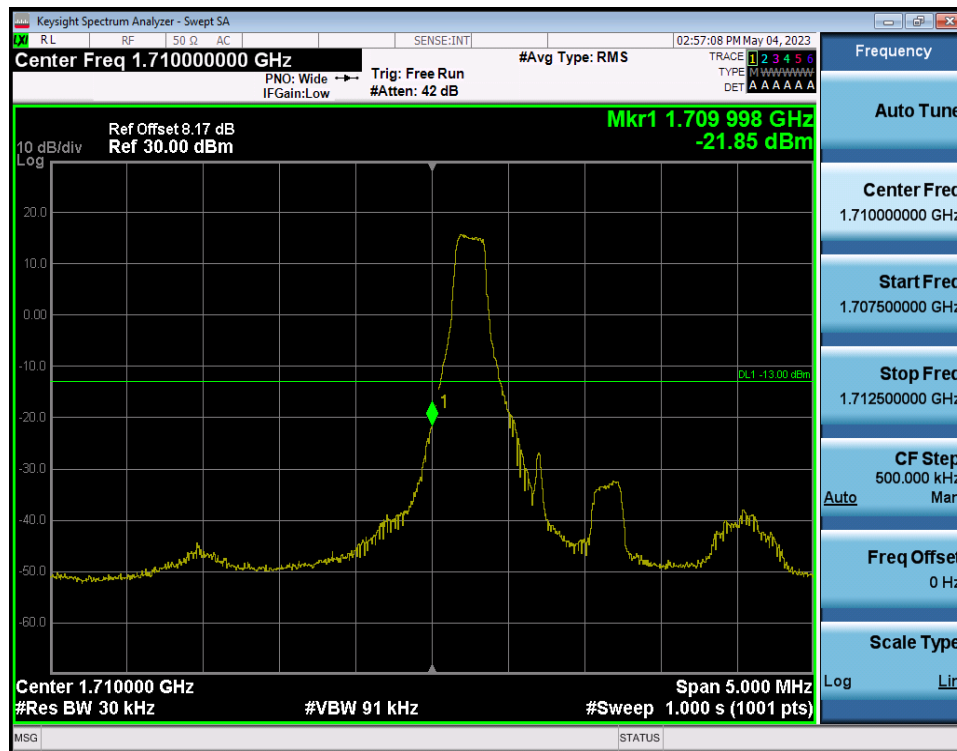
LTE Band 66(4) / 1.4MHz / 16QAM - RB Size/Offset (1/0)
