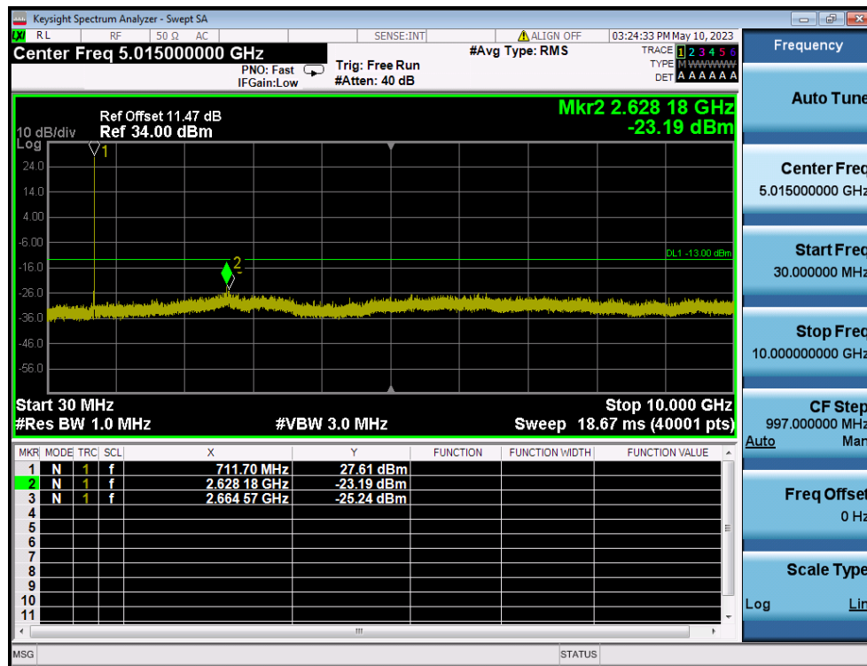
LTE Band 12(17) / 5MHz / 64QAM - RB Size/Offset (12/0) - High Channel
