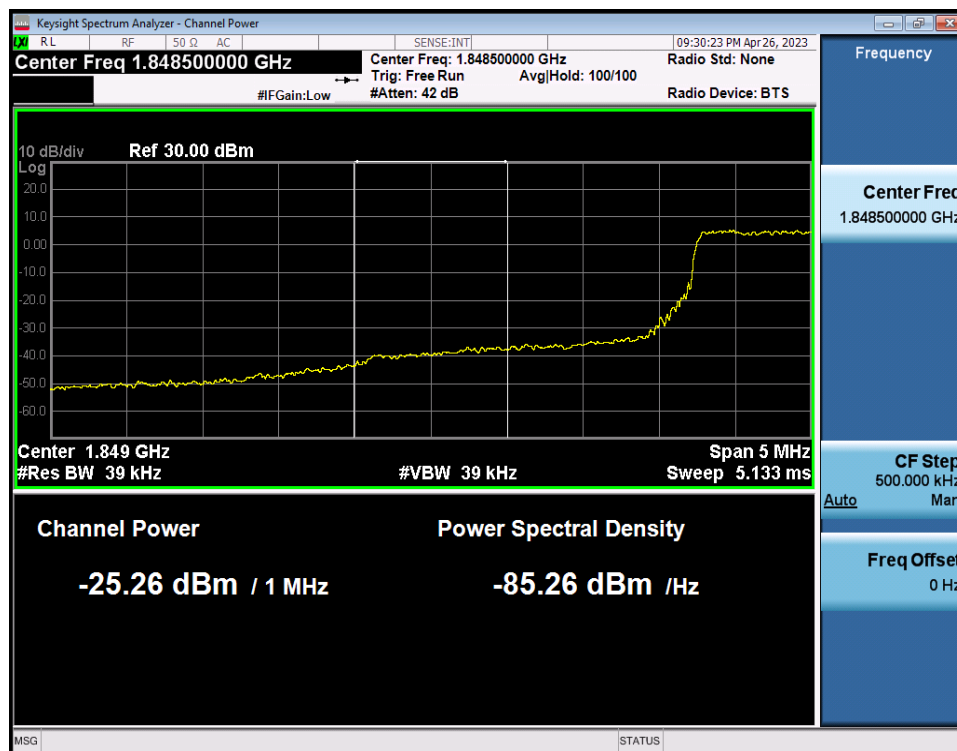
LTE Band 25(2) / 5MHz / QPSK - RB Size/Offset (12/0)
