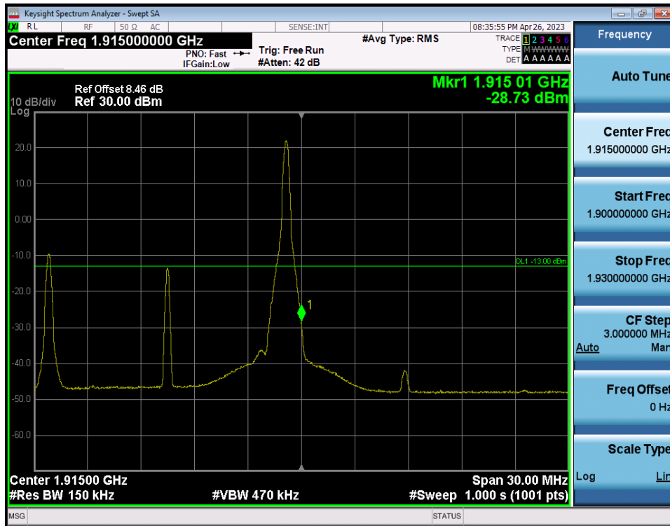
LTE Band 25(2) / 15MHz / QPSK - RB Size/Offset (1/74)
