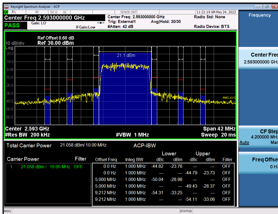
LTE Band 41(38) / 10MHz / 16QAM - RB Size/Offset (50/0)
