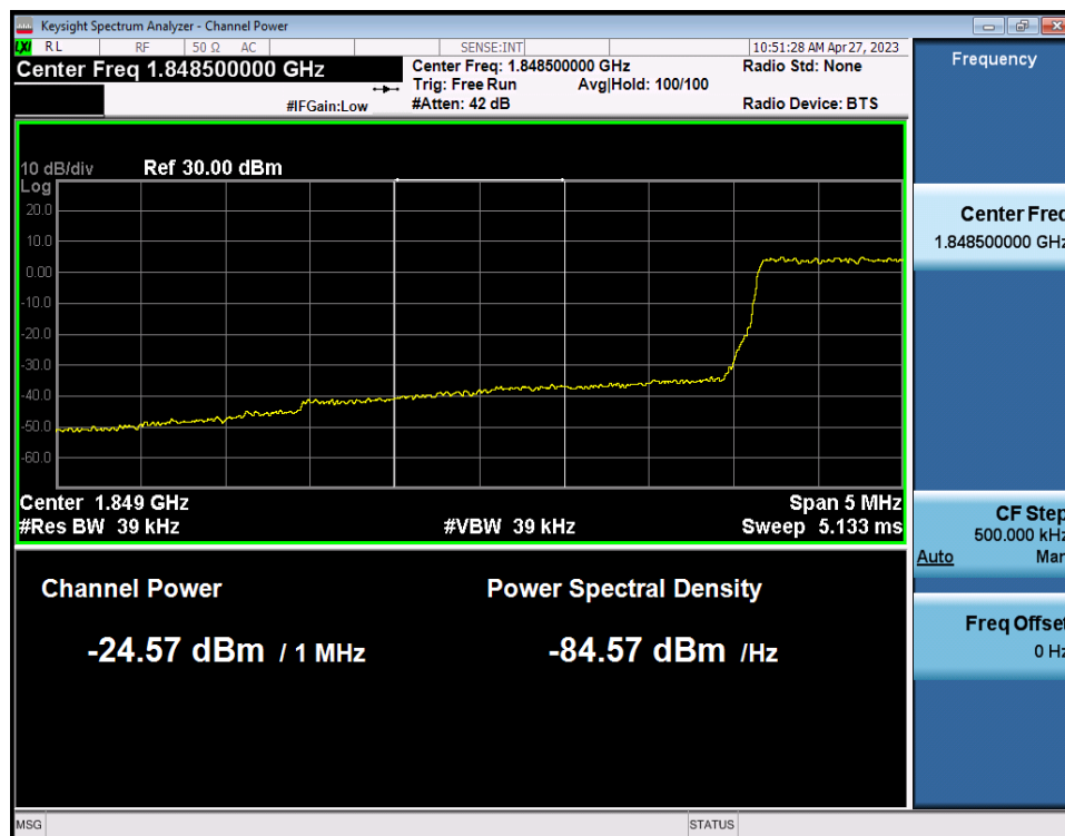
LTE Band 25(2) / 3MHz / QPSK - RB Size/Offset (15/0)
