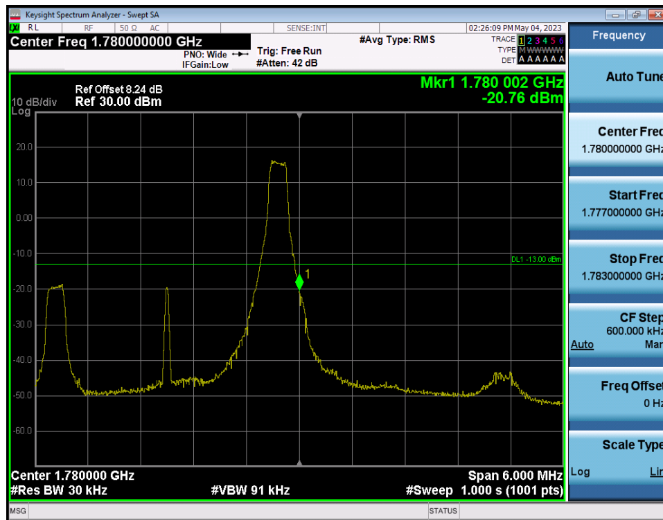
LTE Band 66(4) / 3MHz / 16QAM - RB Size/Offset (1/14)
