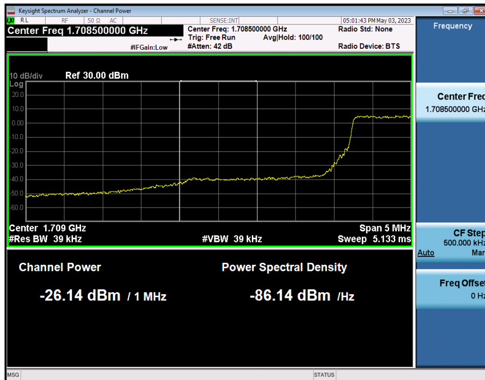
LTE Band 66(4) / 5MHz / QPSK - RB Size/Offset (12/0)
