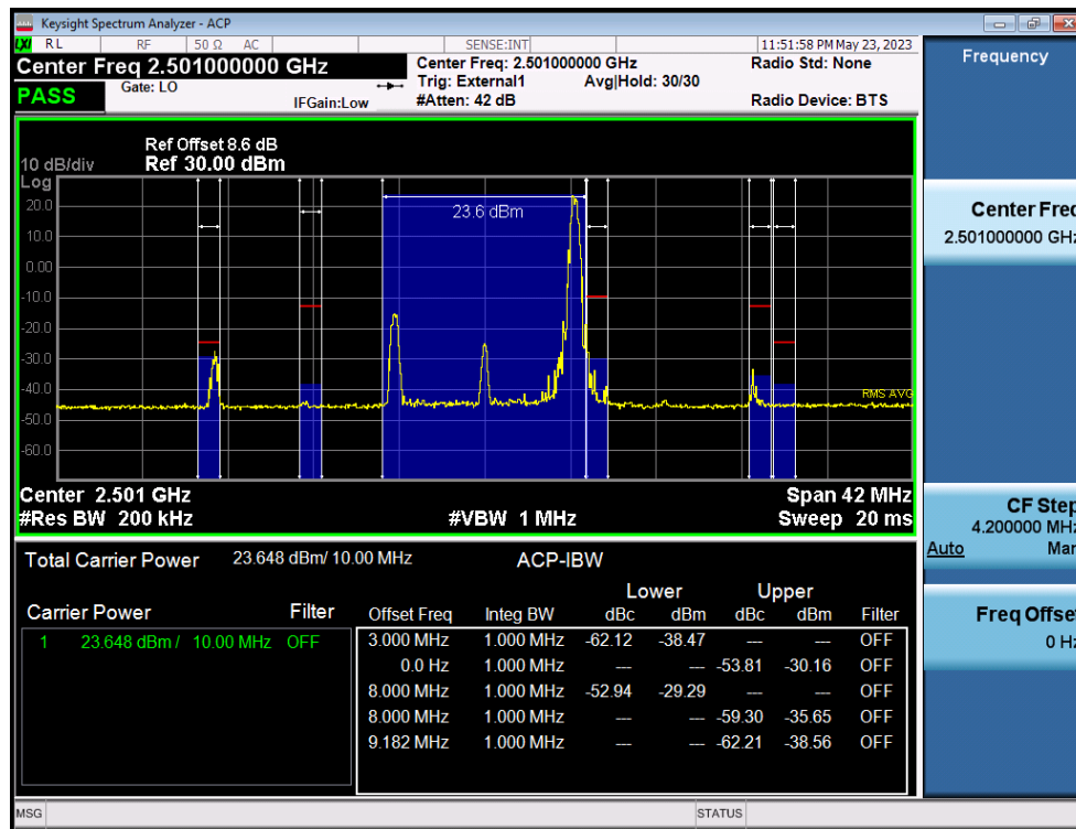
LTE Band 41(38) / 10MHz / QPSK - RB Size/Offset (1/49)
