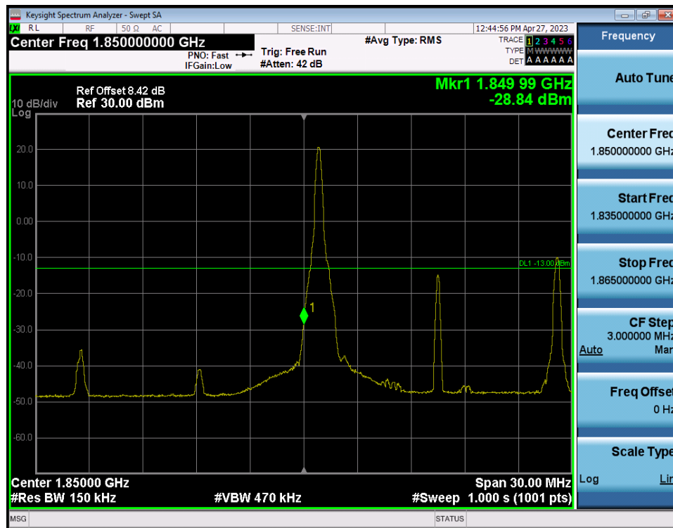
LTE Band 25(2) / 15MHz / 16QAM - RB Size/Offset (1/0)
