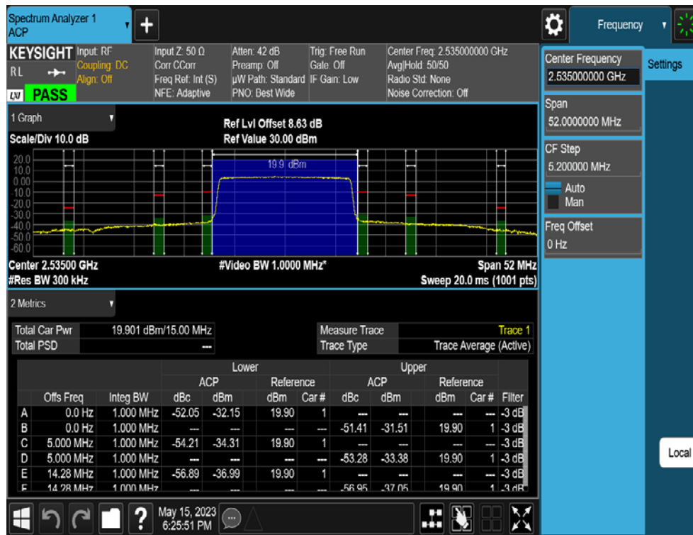
LTE Band 7 / 15MHz / QPSK - RB Size/Offset (75/0)
