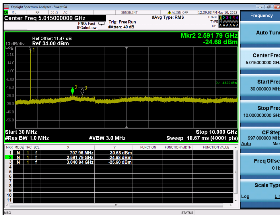
LTE Band 12(17) / 5MHz / 16QAM - RB Size/Offset (1/12) - Mid Channel
