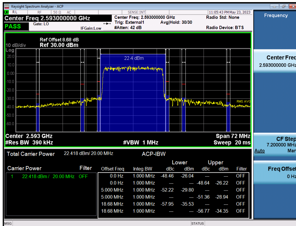
LTE Band 41(38) / 20MHz / QPSK - RB Size/Offset (100/0)
