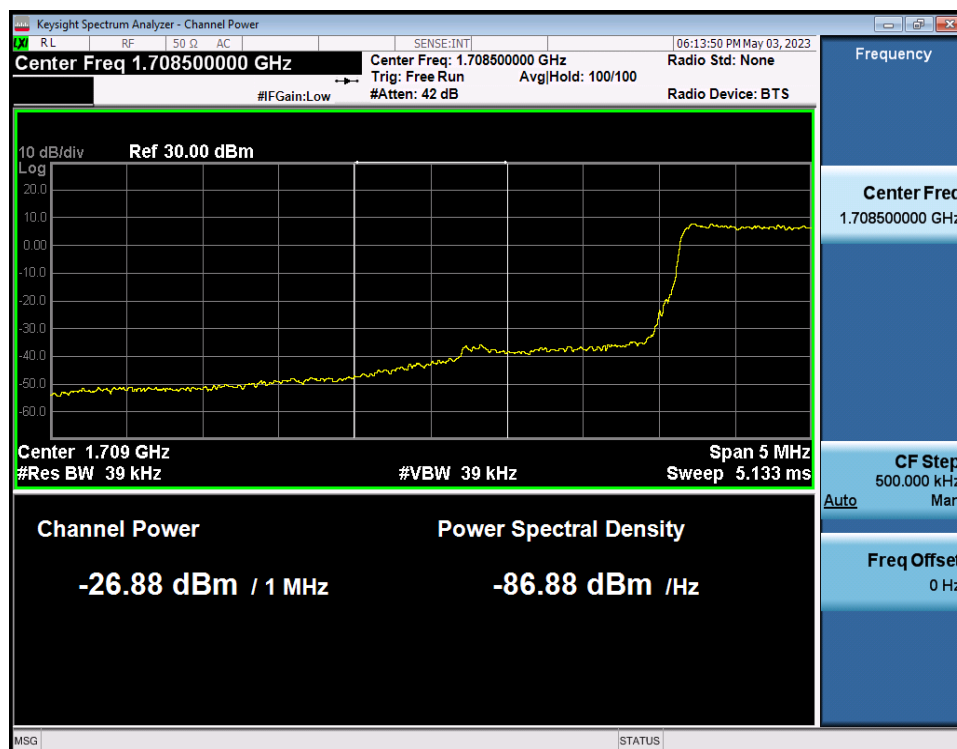
LTE Band 66(4) / 3MHz / QPSK - RB Size/Offset (8/0)
