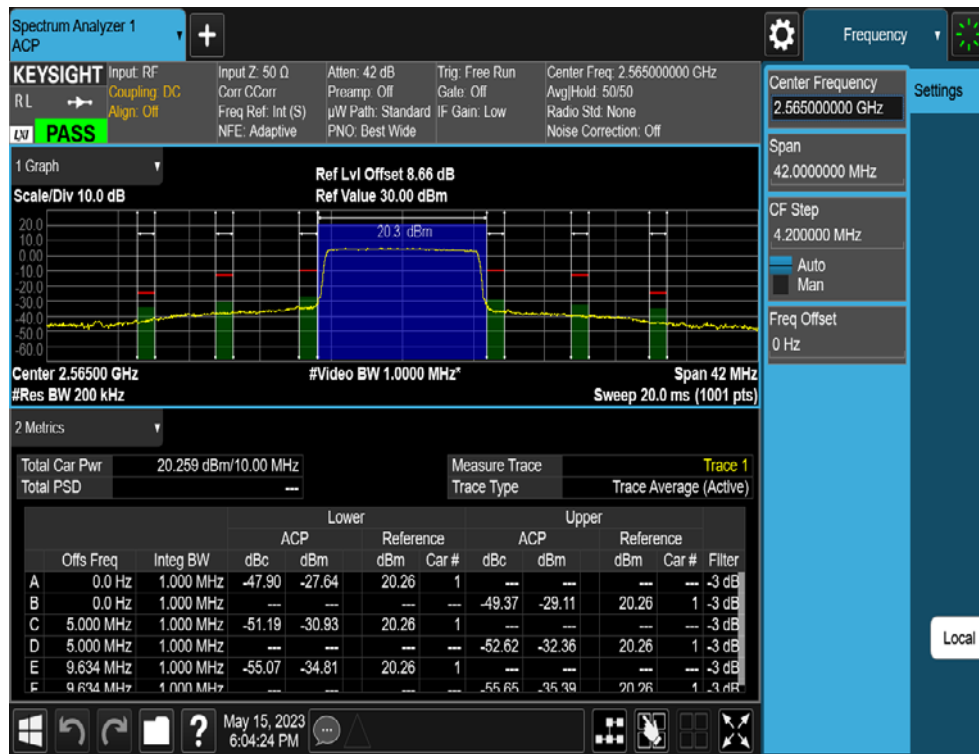
LTE Band 7 / 10MHz / QPSK - RB Size/Offset (50/0)
