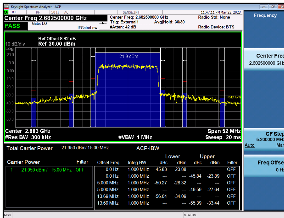
LTE Band 41(38) / 15MHz / QPSK - RB Size/Offset (75/0)
