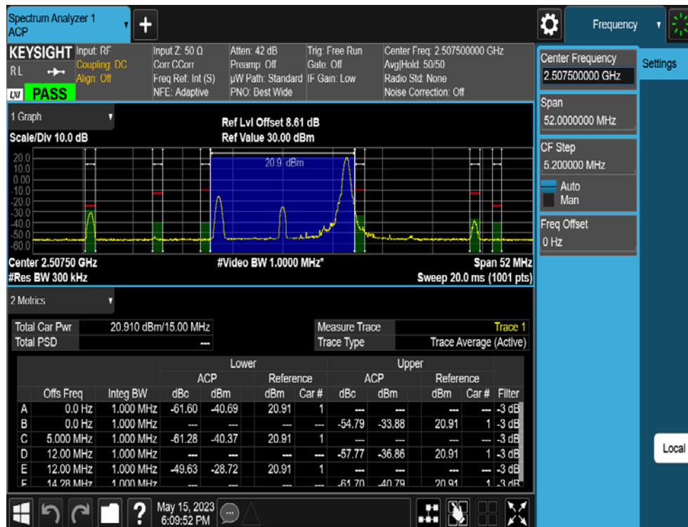
LTE Band 7 / 15MHz / QPSK - RB Size/Offset (1/74)
