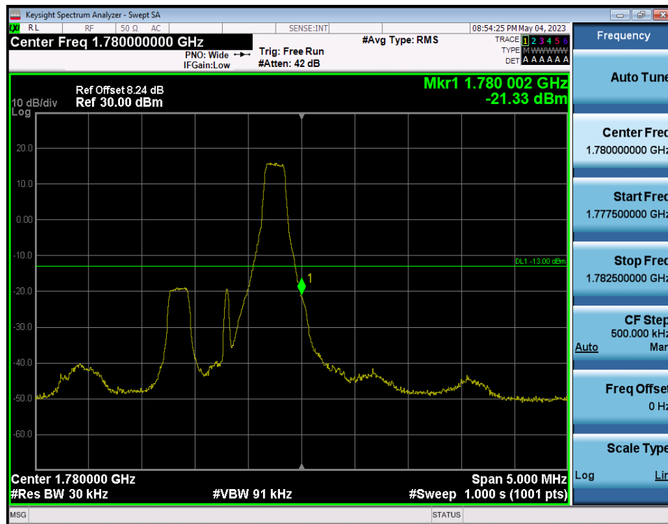
LTE Band 66(4) / 1.4MHz / 16QAM - RB Size/Offset (1/5)
