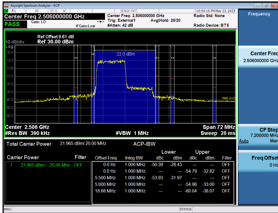
LTE Band 41(38) / 20MHz / QPSK - RB Size/Offset (50/0)
