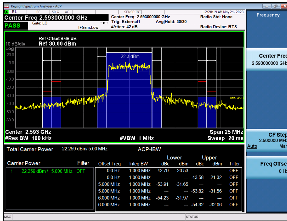
LTE Band 41(38) / 5MHz / QPSK - RB Size/Offset (25/0)
