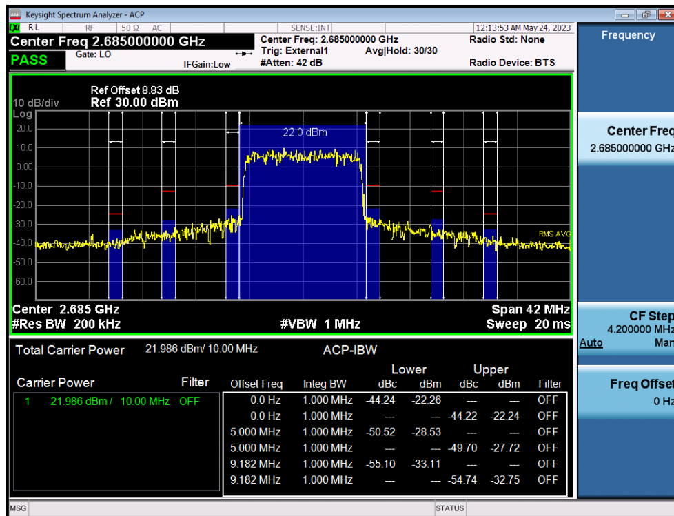
LTE Band 41(38) / 10MHz / QPSK - RB Size/Offset (50/0)
