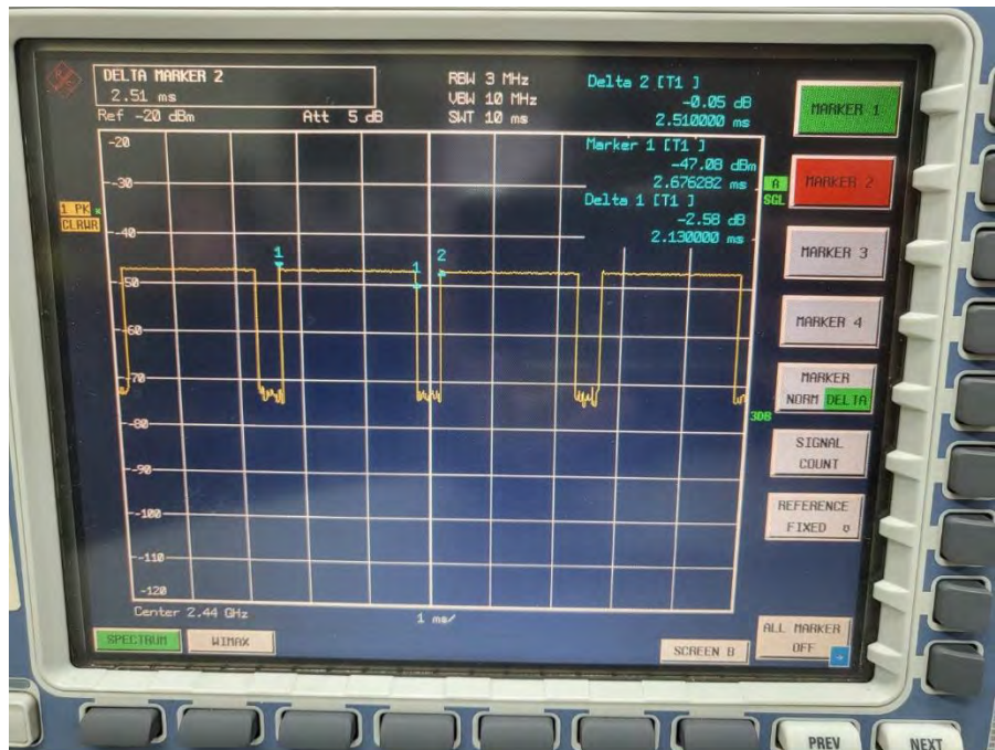
Figure 8.2.3 Bluetooth Transmission Plot
