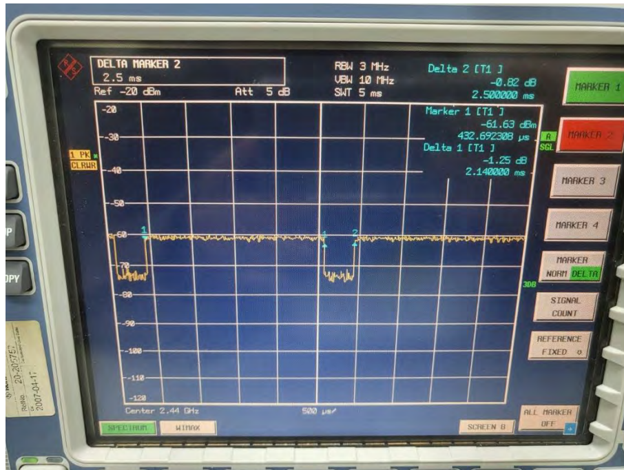
Figure 8.2.4 Bluetooth Transmission Plot
