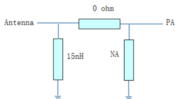
Picture 4 Matching network for DIV antenna
