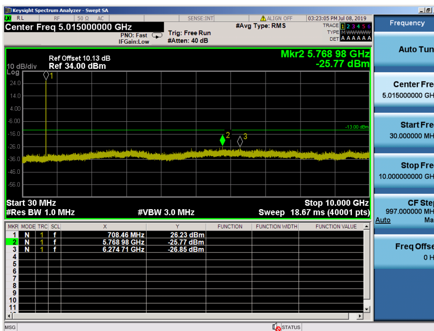
LTE Band 12 / 5MHz / QPSK - RB Size/Offset (12/13) – Mid Channel
