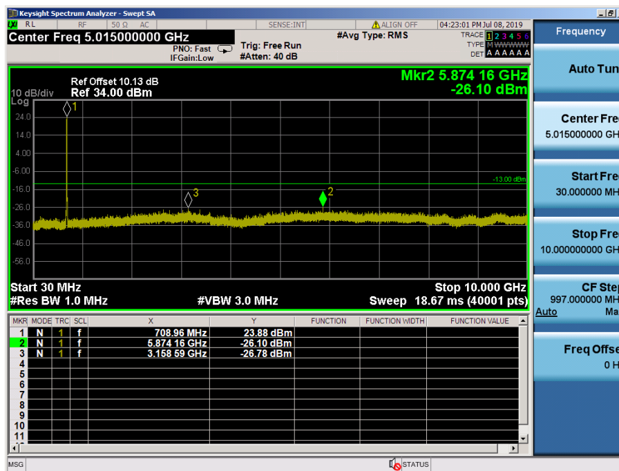
LTE Band 12 / 10MHz / QPSK - RB Size/Offset (50/0) – High Channel
