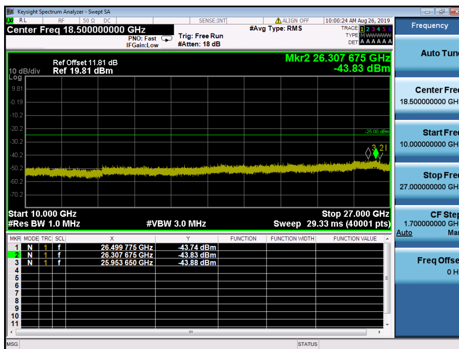
LTE Band 41 / 20MHz / 64QAM - RB Size/Offset (1/99)–Mid Channel
