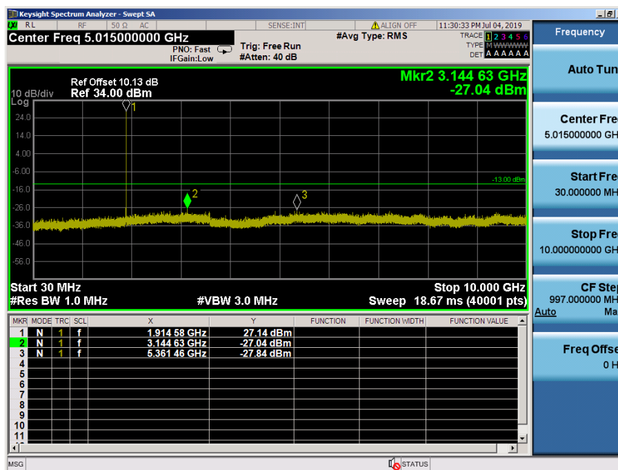
LTE Band 2, 25 / 10MHz / 64QAM - RB Size/Offset (1/49) – High Channel
