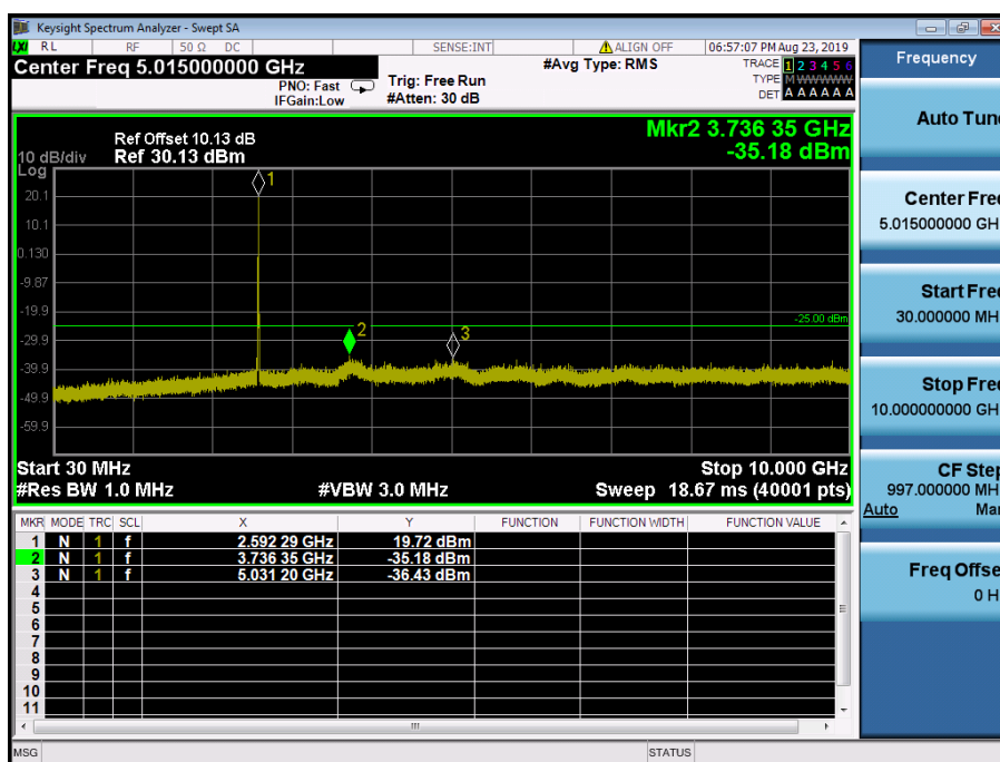
LTE Band 41 / 10MHz / 64QAM - RB Size/Offset (25/12) – Mid Channel
