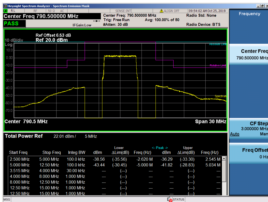
LTE Band 14 / 5MHz / QPSK - RB Size/Offset (25/0) - Low Channel
