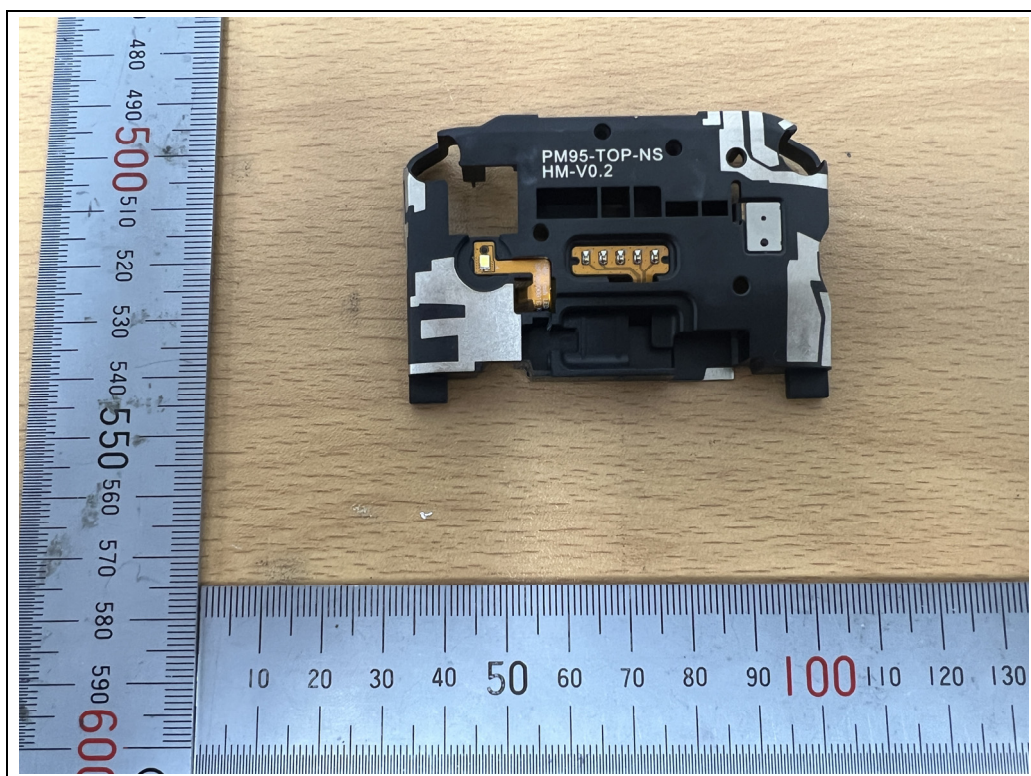
WWAN TRX, BT, WLAN(TOP) Antenna
