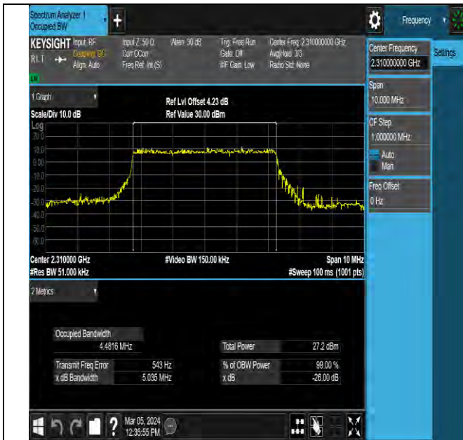
NTVN-N30-PC3-15-5-M-DFT-256QAM-Outer_Full-Ant10-PAS S
