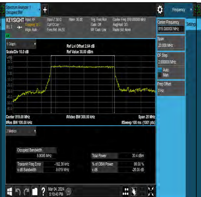
NTNV-N26-814-824-PC3-15-10-M-DFT-P12BPSK-Outer_Full-Ant0-PASS
