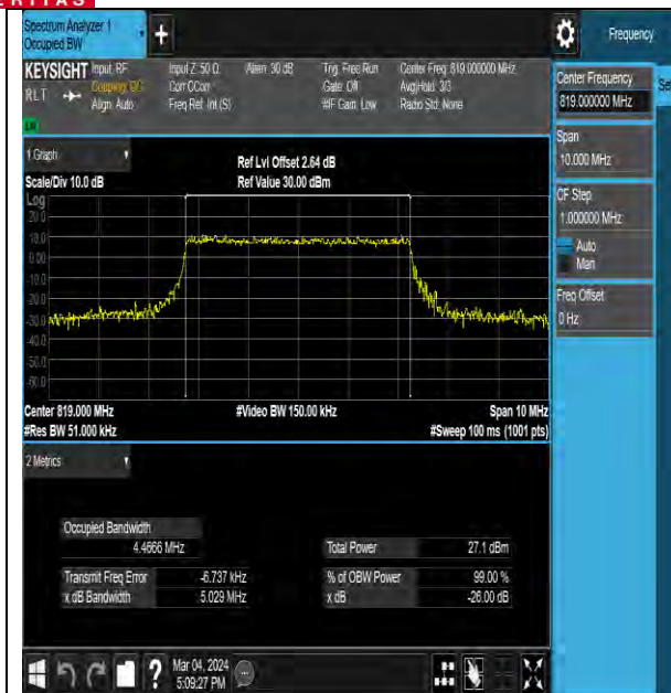
NTNV-N26-814-824-PC3-15-5-M-DFT-256QAM-Outer_Full-Ant0-PASS
