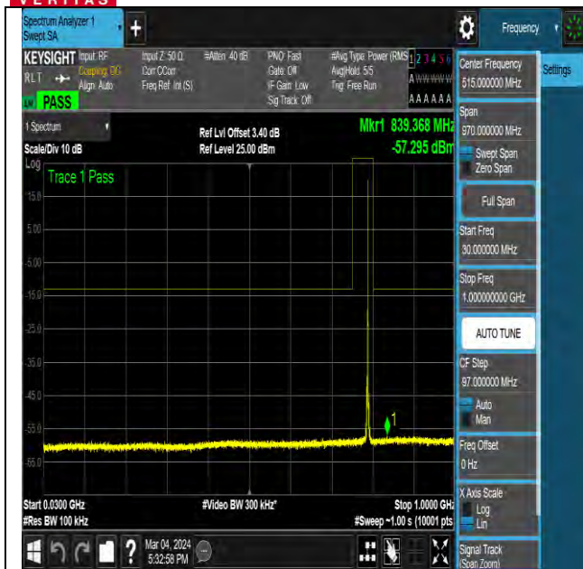
NTNV-N14-PC3-15-5-H-DFT-QPSK-Edge_1RB_Left-Ant0- PASS
