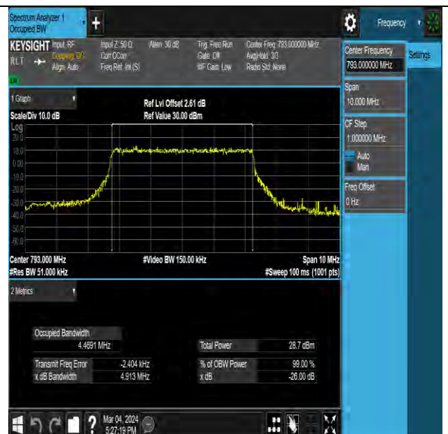
NTNV-N14-PC3-15-5-M-DFT-QPSK-Outter_Full-Ant0-PASS
