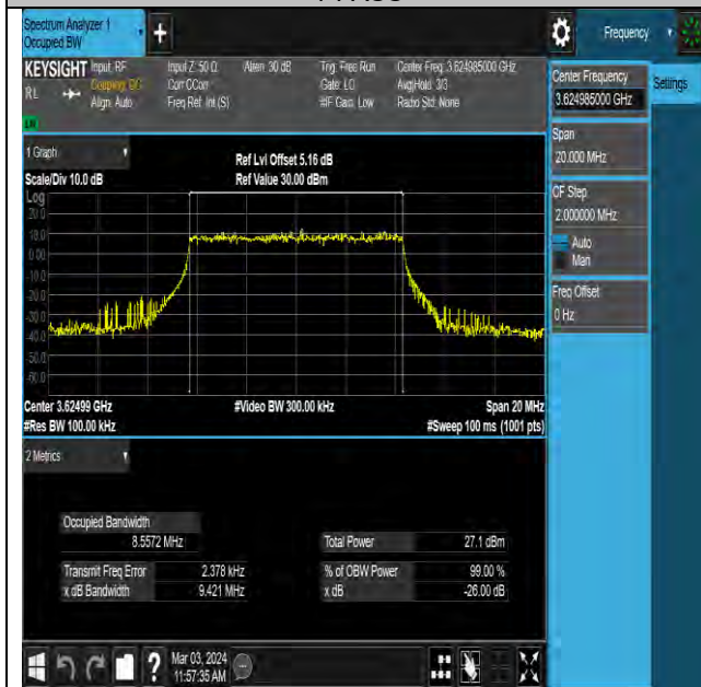
NTNV-N48-PC3-30-10-M-DFT-16QAM-Outter_Full-Ant11-PASS
