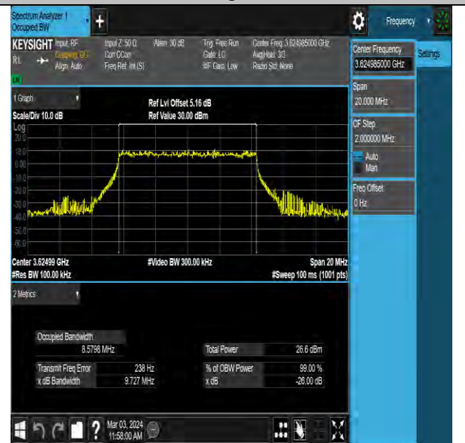
NTNV-N48-PC3-30-10-M-DFT-64QAM-Outter_Full-Ant11-PASS
