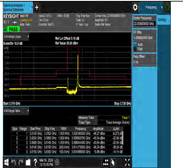
NTNV-48-PC3-30-20-M-DFT-QPSK-Edge_1RB_Right-Ant11-PASS
