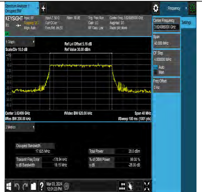
NTNV-N48-PC3-30-20-M-DFT-256QAM-Outer_Full-Ant11-PASS
