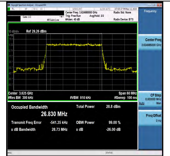
NTNV-N48-PC3-30-30-M-DFT-QPSK-Outer_Full-Ant11-PASS
