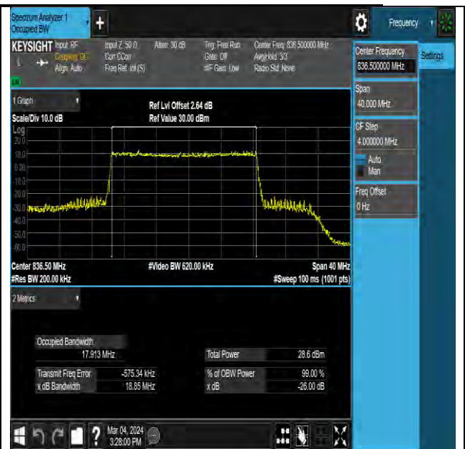
NTNV-N26-824-849-PC3-15-20-M-DFT-16QAM-Outer_Full-Ant0-PASS
