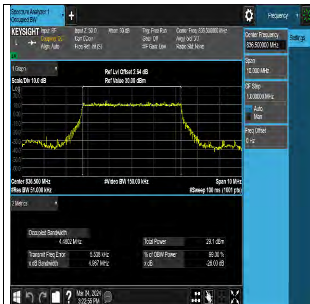
NTNV-N26-824-849-PC3-15-5-M-DFT-PI2BPSK- Outer_Full-Ant0-PASS
