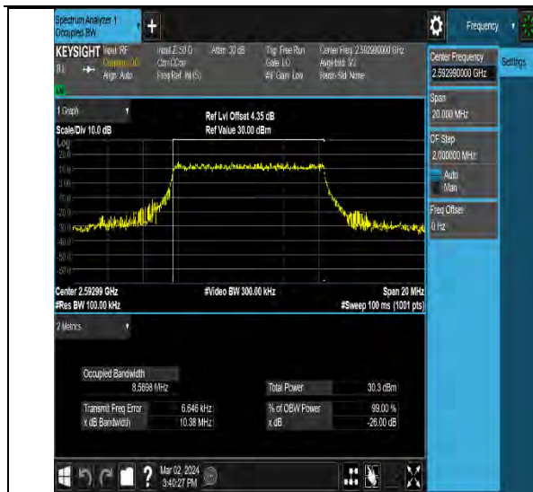
NTNV-N41-PC2-30-10-M-DFT-256QAM-Outer_Full- Ant10-PASS
