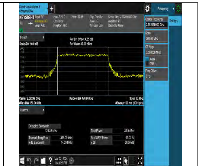
NTNV-N41-PC2-30-15-M-DFT-PI2BPSK-Outer_Full- Ant10-PASS
