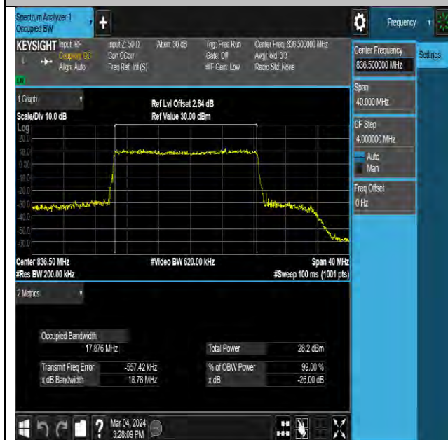
NTNV-N26-824-849-PC3-15-20-M-DFT-64QAM-Outer_Full-Ant0-PASS
