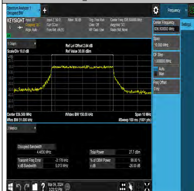
NTNV-N26-824-849-PC3-15-5-M-DFT-16QAM- Outer_Full-Ant0-PASS
