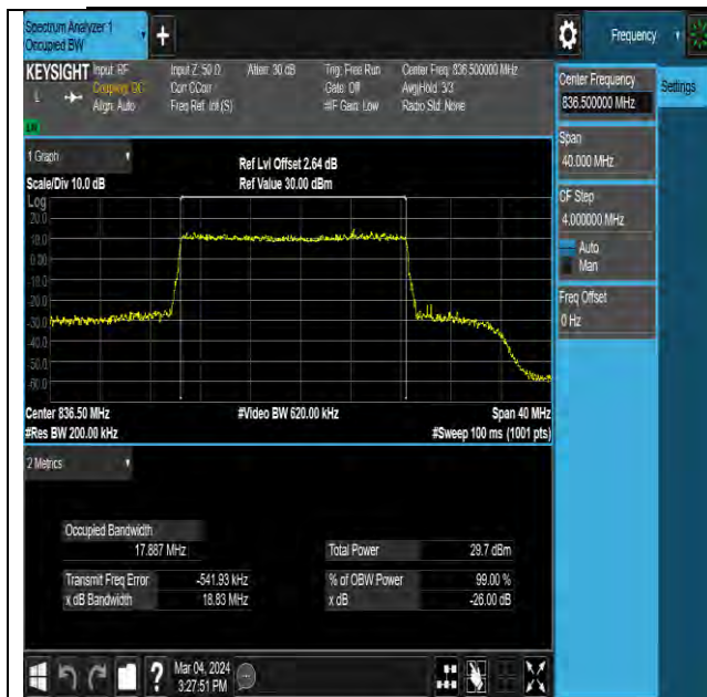
NTNV-N26-824-849-PC3-15-20-M-DFT-QPSK-Outer_Full-Ant0-PASS
