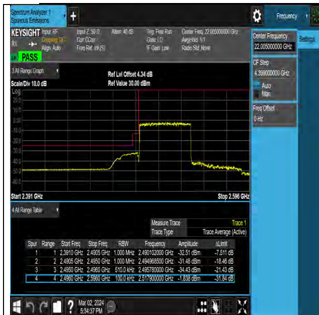
NTNV-N41-PC2-30-50-L-DFT-QPSK-Outer_Full-Ant10- PASS
