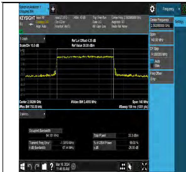
NTVN-N41-PC2-30-70-M-DFT-QPSK-Outer_Full-Ant10- PASS
