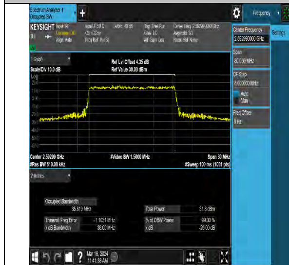
NTNV-N41-PC2-30-40-M-DFT-16QAM-Outer_Full-Ant10- PASS
