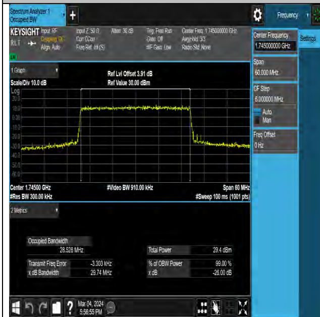
NTNV-N66-PC3-15-30-M-DFT-QPSK-Outer_Full-Ant1- PASS
