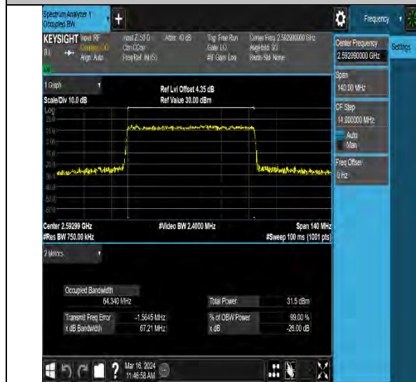
NTVN-N41-PC2-30-70-M-DFT-64QAM-Outer_Full-Ant10- PASS
