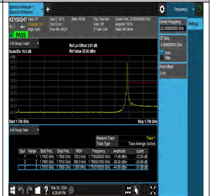
NTVN-N66-PC3-15-40-H-DFT-QPSK-Edge_1RB_Right- Ant1-PASS
