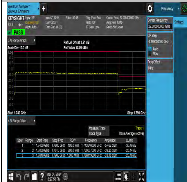
NTVN-N66-PC3-15-40-H-DFT-QPSK-Outer_Full-Ant1- PASS
