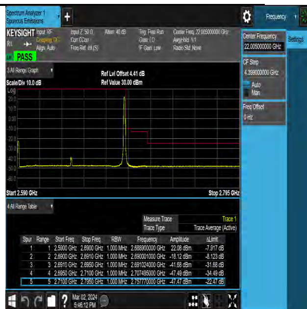
NTNV-N41-PC2-30-100-H-DFT-QPSK-Edge_1RB_Right- Ant10-PASS
