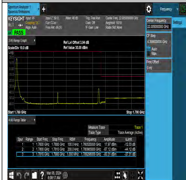
NTNV-N66-PC3-15-20-H-DFT-QPSK-Edge_1RB_Left-Ant1-PASS
