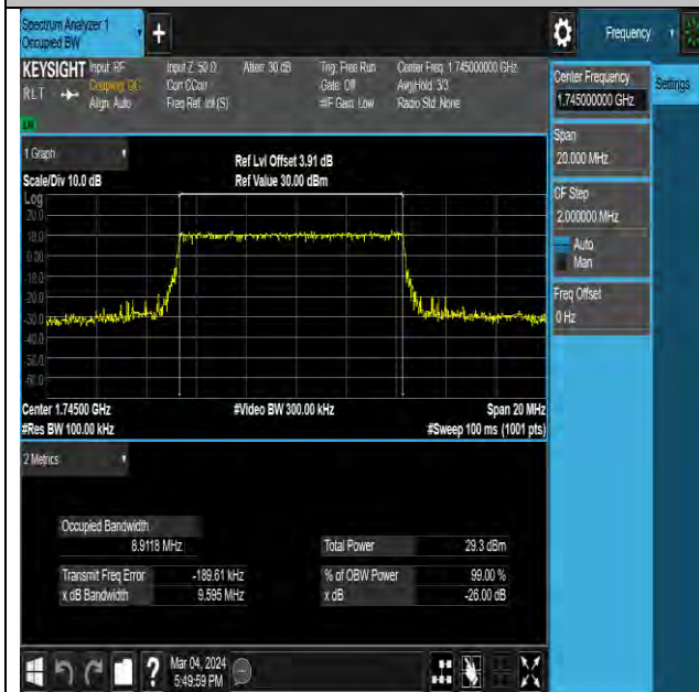
NTNV-N66-PC3-15-10-M-DFT-QPSK-Outer_Full-Ant1- PASS
