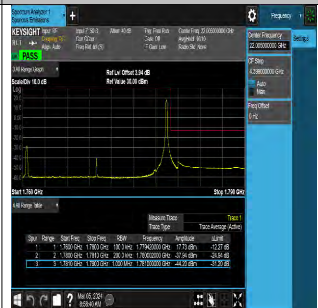
NTNV-N66-PC3-15-20-H-DFT-QPSK-Edge_1RB_Right-Ant1-PASS
