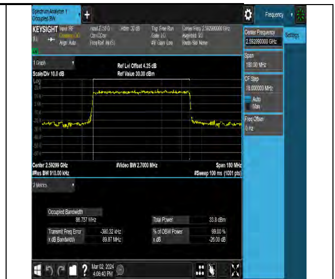
NTNV-N41-PC2-30-90-M-DFT-PI2BPSK-Outer_Full- Ant10-PASS
