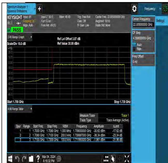
NTNV-N66-PC3-15-20-L-DFT-QPSK-Outer_Full-Ant1-PASS
