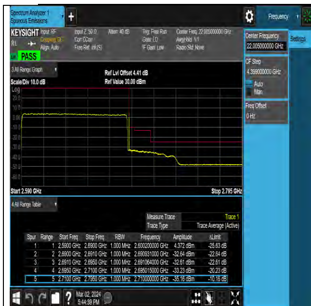
NTNV-N41-PC2-30-100-H-DFT-QPSK-Outer_Full-Ant10- PASS
