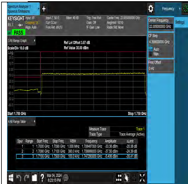
NTVN-N66-PC3-15-40-L-DFT-QPSK-Outer_Full-Ant1- PASS
