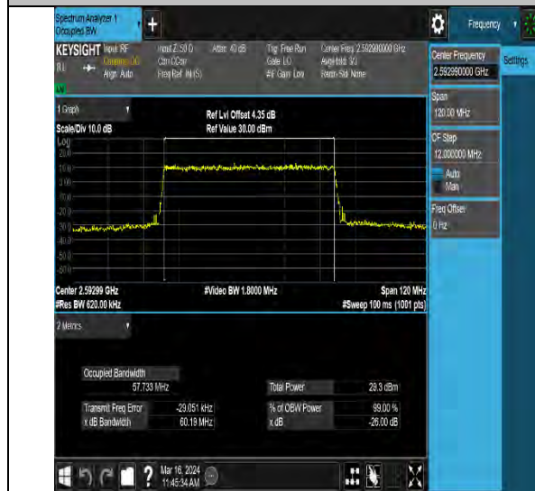
NTNV-N41-PC2-30-60-M-DFT-256QAM-Outet_Full- Ant10-PASS
