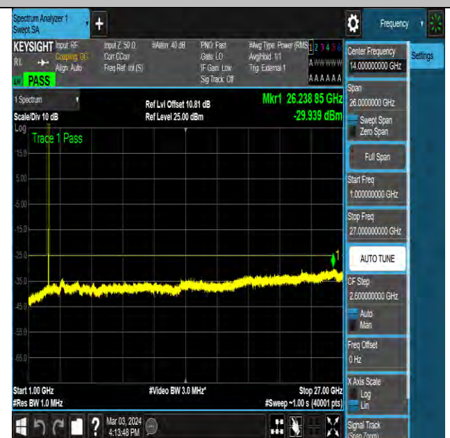
NTNV-N41-PC2-30-50-H-DFT-QPSK-Edge_1RB_Left-Ant10-PASS
