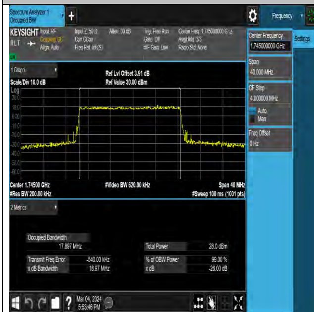
NTNV-N66-PC3-15-20-M-DFT-64QAM-Outer_Full-Ant1- PASS
