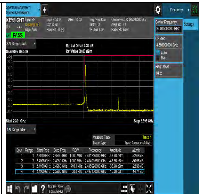
NTNV-N41-PC2-30-50-L-DFT-QPSK-Edge_1RB_Left- Ant10-PASS
