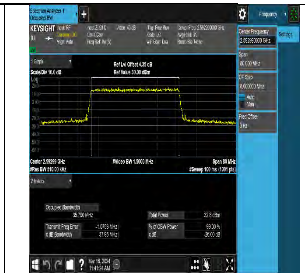
NTNV-N41-PC2-30-40-M-DFT-QPSK-Outer_Full-Ant10- PASS
