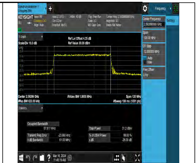
NTNV-N41-PC2-30-60-M-DFT-64QAM-Outet_Full-Ant10- PASS
