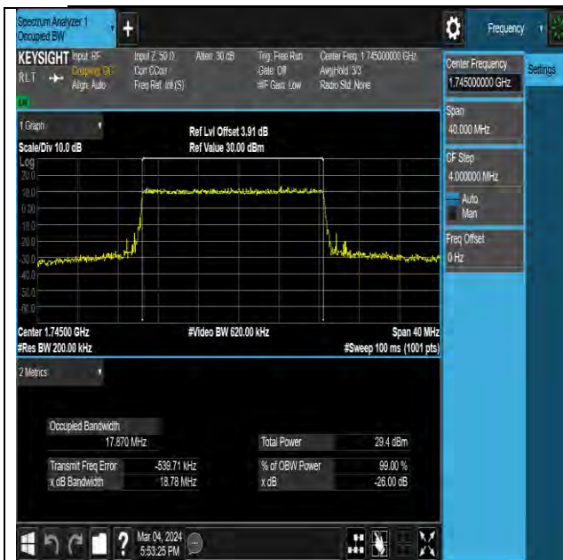
NTNV-N66-PC3-15-20-M-DFT-QPSK-Outer_Full-Ant1- PASS
