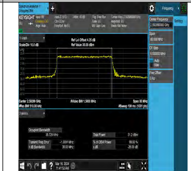
NTNV-N41-PC2-30-40-M-DFT-64QAM-Outer_Full-Ant10- PASS
