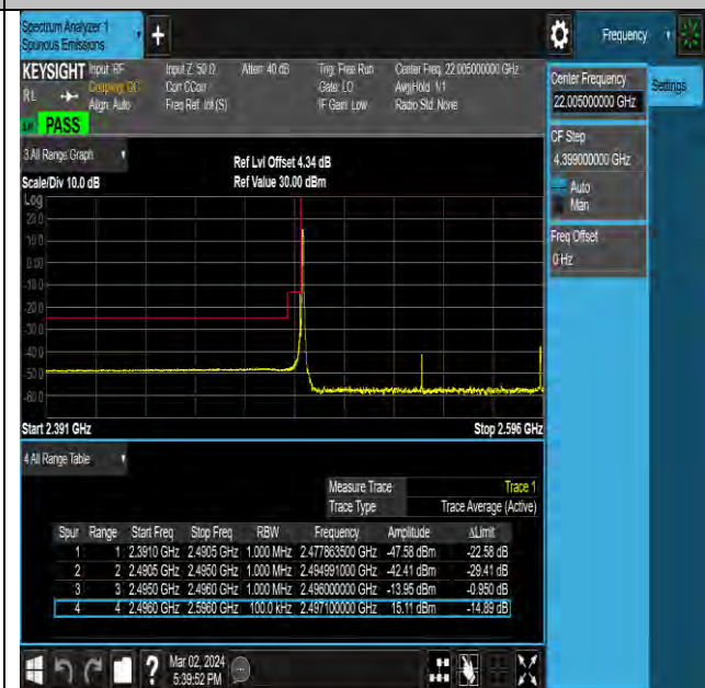
NTNV-N41-PC2-30-100-L-DFT-QPSK-Edge_1RB_Left- Ant10-PASS
