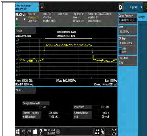
NTNV-N41-PC2-30-80-M-DFT-PI2BPSK-Outer_Full- Ant10-PASS
