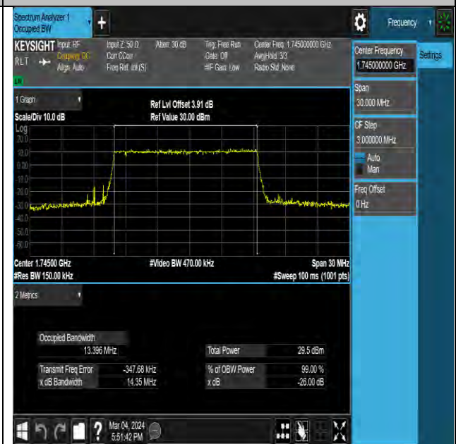
NTNV-N66-PC3-15-15-M-DFT-QPSK-Outer_Full-Ant1- PASS
