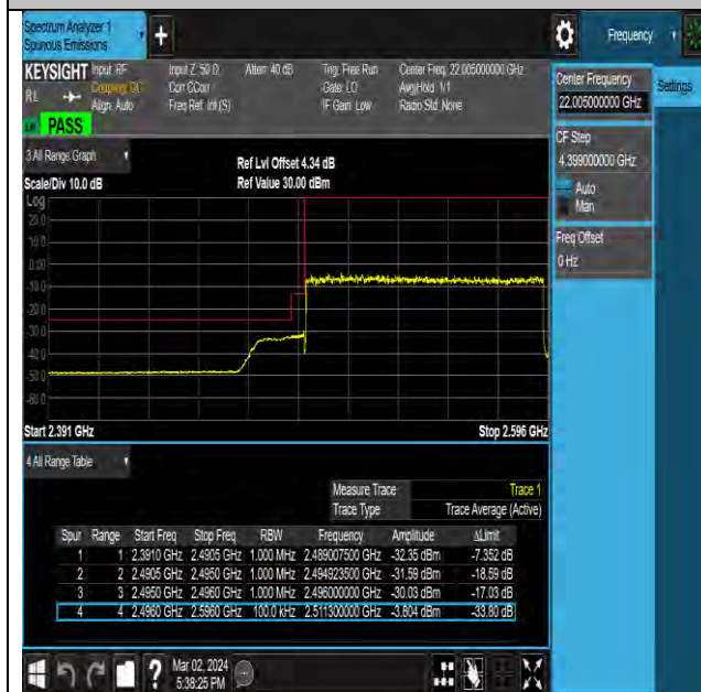
NTNV-N41-PC2-30-100-L-DFT-QPSK-Outer_Full-Ant10- PASS
