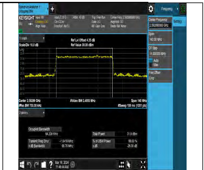
NTVN-N41-PC2-30-70-M-DFT-16QAM-Outer_Full-Ant10- PASS
