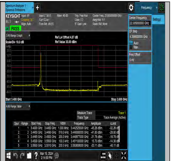
NTNV-N77-3450-3550-PC2-30-100-M-DFT-QPSK- Edge_1RB_Left-Ant11-PASS
