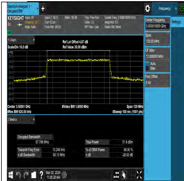
NTNV-N77-3450-3550-PC2-30-60-M-DFT-16QAM- Outer_Full-Ant11-PASS
