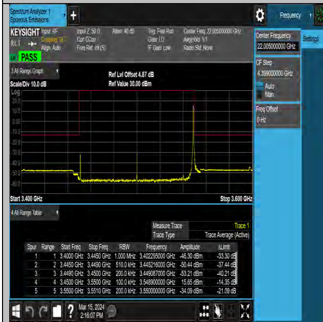
NTNV-N77-3450-3550-PC2-30-100-M-DFT-QPSK- Edge_1RB_Right-Ant11-PASS
