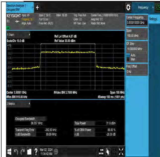
NTNV-N77-3450-3550-PC2-30-90-M-DFT-64QAM- Outer_Full-Ant11-PASS
