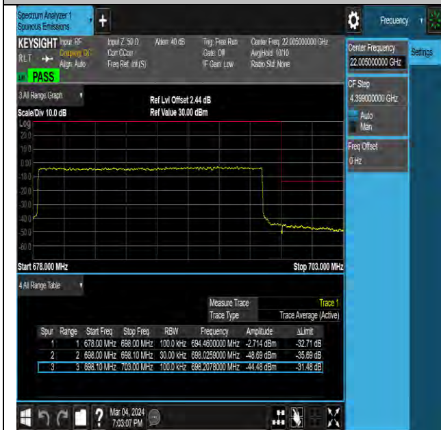
NTNV-N71-PC3-15-20-H-DFT-QPSK-Outter_Full-Ant0- PASS
