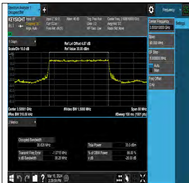
NTNV-N77-3450-3550-PC2-30-40-M-DFT-PI2BPSK- Outer_Full-Ant11-PASS
