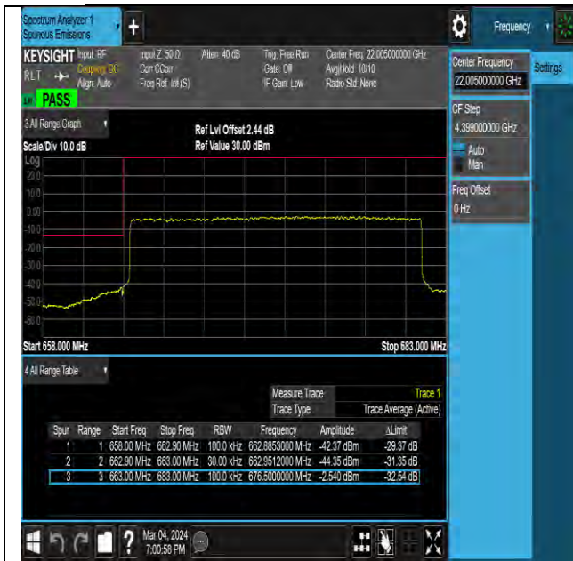
NTNV-N71-PC3-15-20-L-DFT-QPSK-Outter_Full-Ant0- PASS
