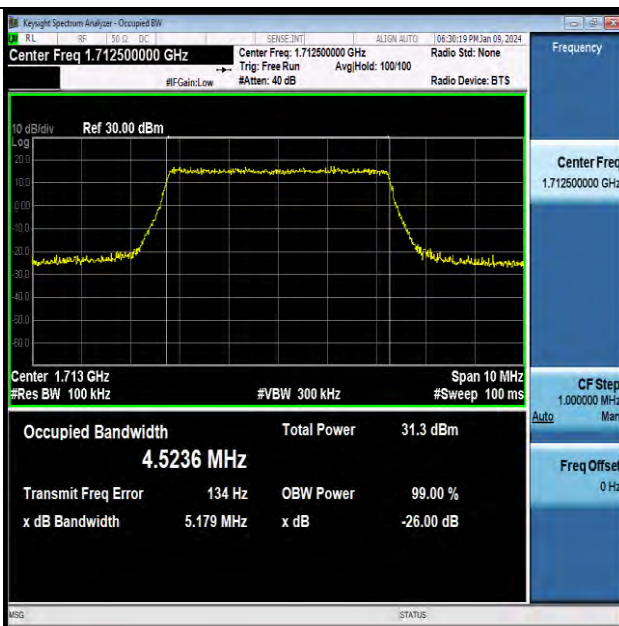
Band66-5MHz-QPSK-131997-25RB#0-PASS
