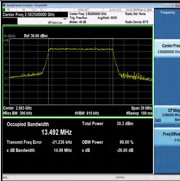
Band7-15MHz-16QAM-21375-75RB#0-PASS
