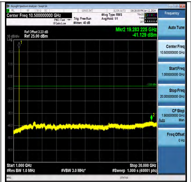
Band4-1513-1000~20000MHz-PASS
