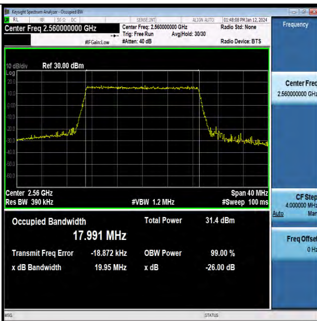
Band7-20MHz-QPSK-21350-100RB#0-PASS
