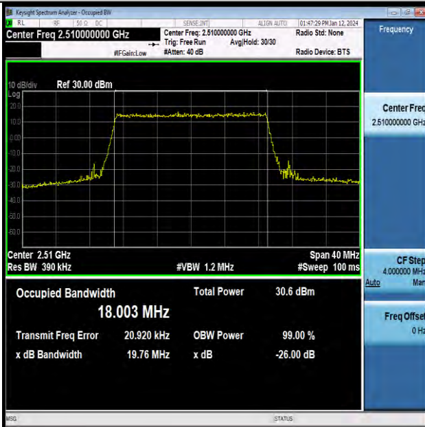
Band7-20MHz-16QAM-20850-100RB#0-PASS
