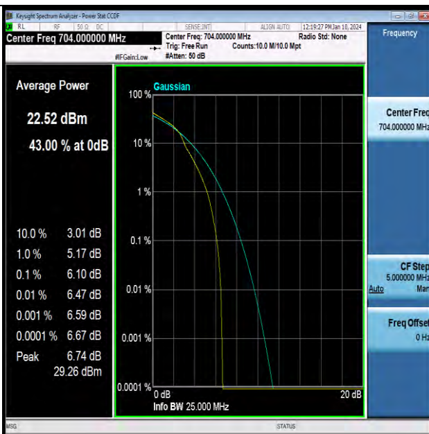
Band12-10MHz-16QAM-23060-1RB#0-PASS
