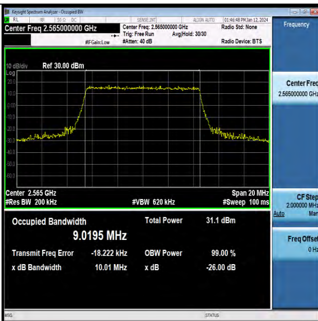
Band7-10MHz-QPSK-21400-50RB#0-PASS
