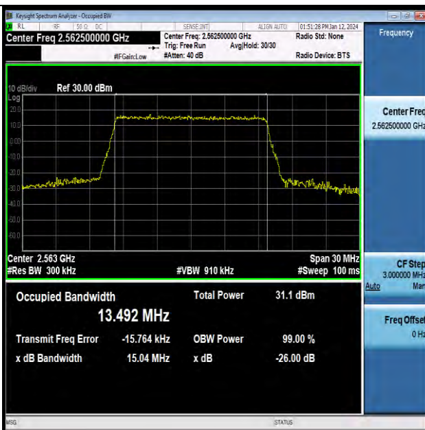
Band7-15MHz-QPSK-21375-75RB#0-PASS
