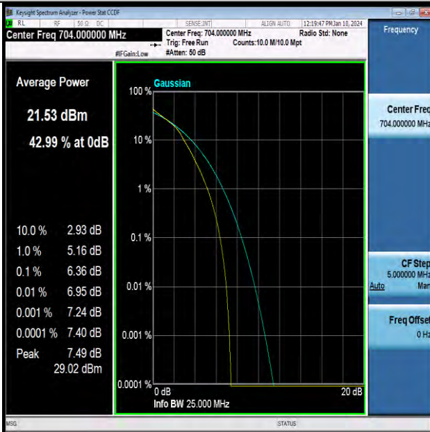
Band12-10MHz-16QAM-23060-50RB#0-PASS
