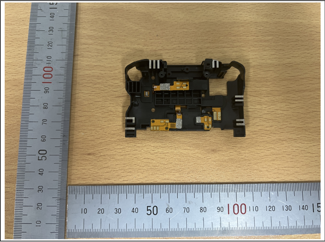
BT, BLE, WLAN(TOP) Antenna
