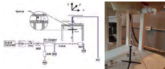
Figure 7.1 Dipole Verification Test Setup Diagram & Photo
