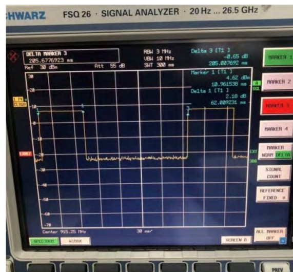
Figure 6.1.2 RFID Transmission Plot
