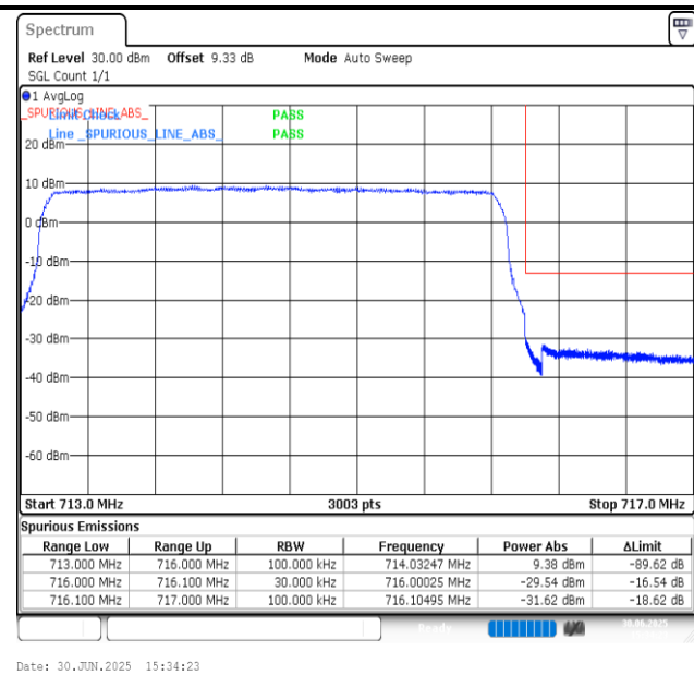
Band12-3MHz-QPSK-23165-15RB#0-PASS
