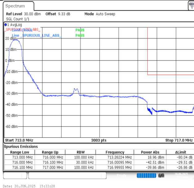
Band12-3MHz-64QAM-23165-1RB#0-PASS
