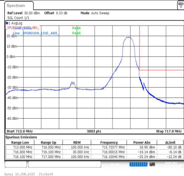
Band12-3MHz-64QAM-23165-1RB#14-PASS
