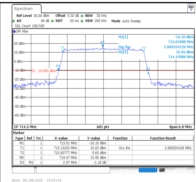
Band12-3MHz-16QAM-23165-15RB#0-PASS
