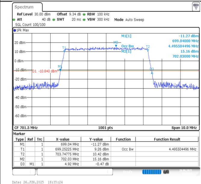
Band12-5MHz-64QAM-23035-25RB#0-PASS
