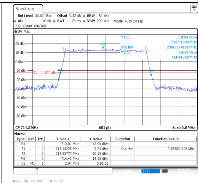
Band12-3MHz-64QAM-23165-15RB#0-PASS
