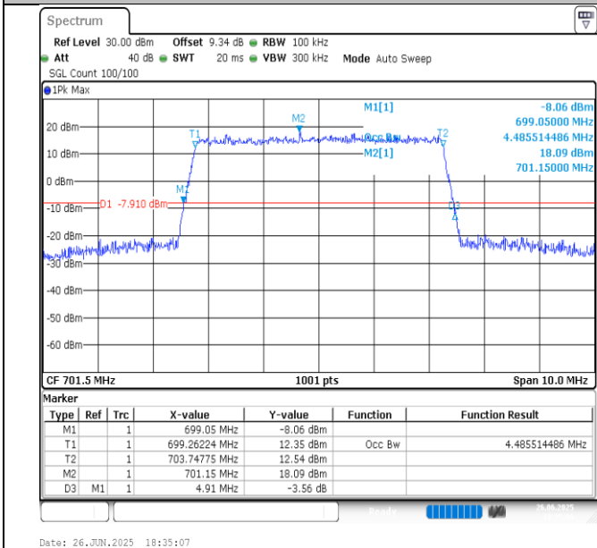
Band12-5MHz-QPSK-23035-25RB#0-PASS
