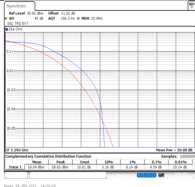
Band41-15MHz-QPSK-40620-75RB#0-PASS
