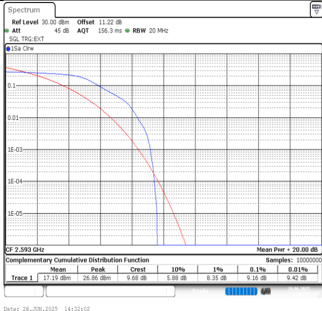
Band41-15MHz-QPSK-40620-1RB#0-PASS
