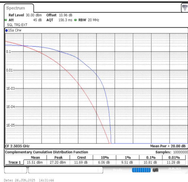
Band41-15MHz-16QAM-39725-75RB#0-PASS
