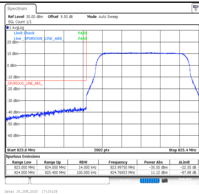
Band5-1.4MHz-64QAM-20407-6RB#0-PASS
