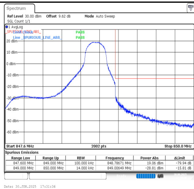
Band5-1.4MHz-64QAM-20643-1RB#5-PASS
