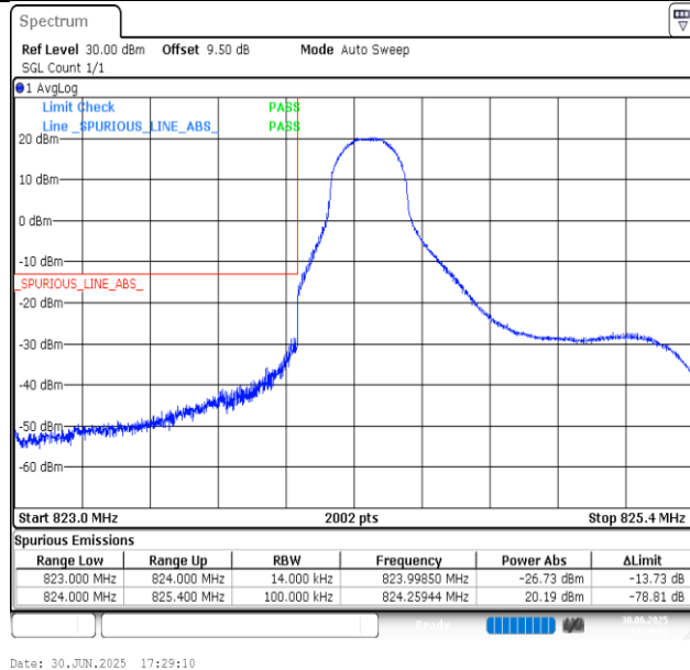
Band5-1.4MHz-16QAM-20407-1RB#0-PASS
