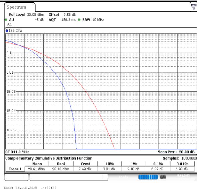
Band5-10MHz-16QAM-20600-50RB#0-PASS
