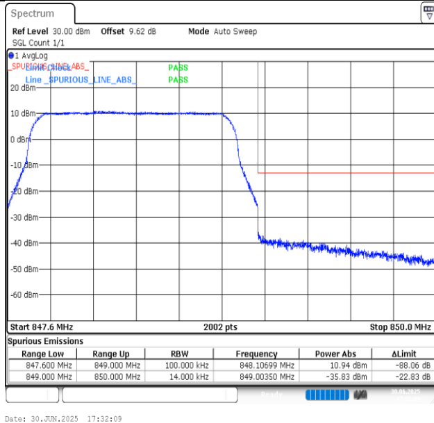
Band5-1.4MHz-64QAM-20643-6RB#0-PASS
