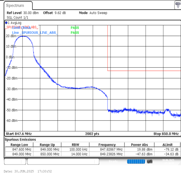
Band5-1.4MHz-16QAM-20643-1RB#0-PASS
