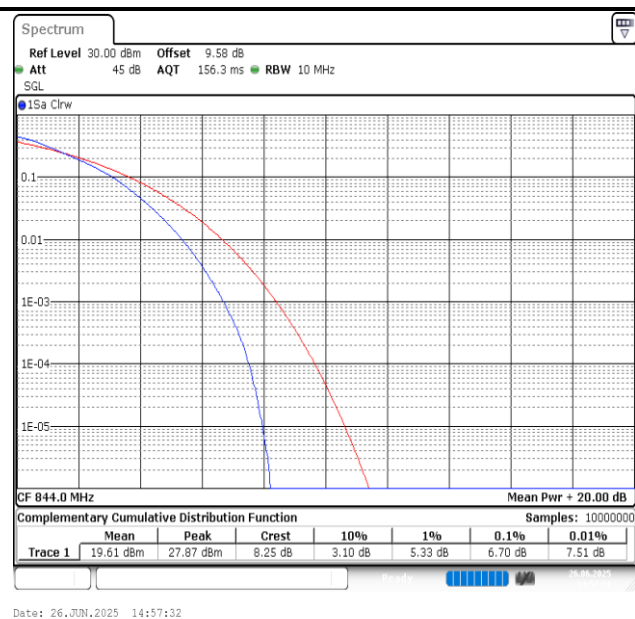
Band5-10MHz-64QAM-20600-50RB#0-PASS
