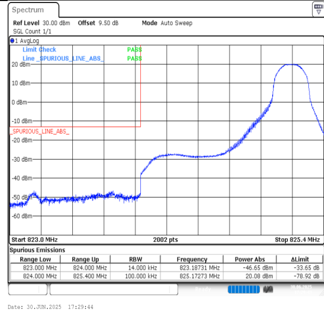
Band5-1.4MHz-16QAM-20407-1RB#5-PASS
