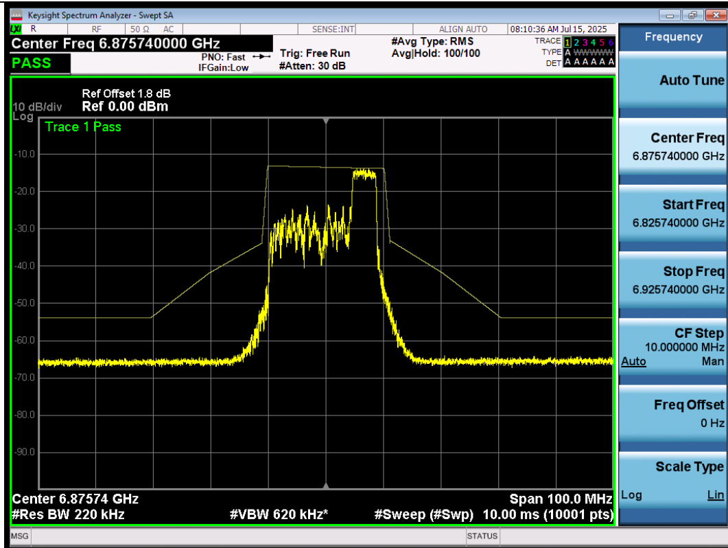
NTNV-11AX20SISO-Ant1-6875-106Tone-RU54-PASS
