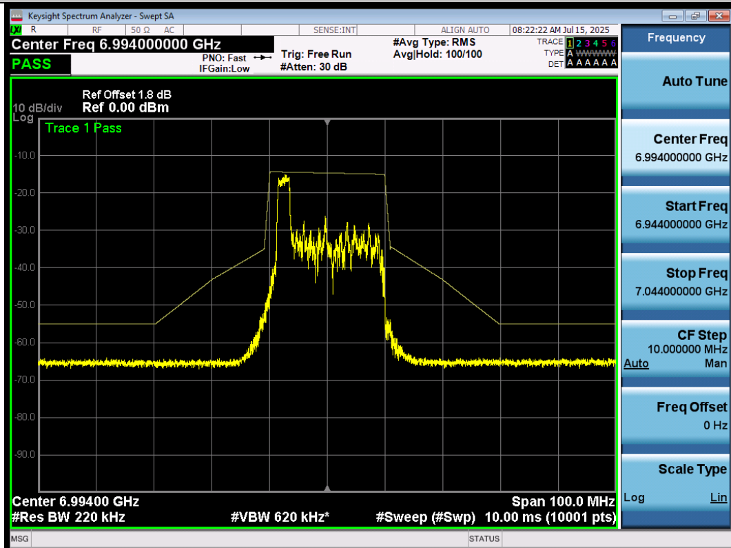
NTNV-11AX20SISO-Ant1-6995-52Tone-RU37-PASS
