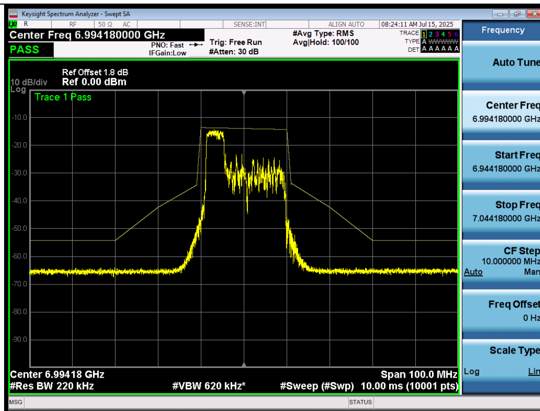
NTNV-11AX20SISO-Ant1-6995-106Tone-RU53-PASS
