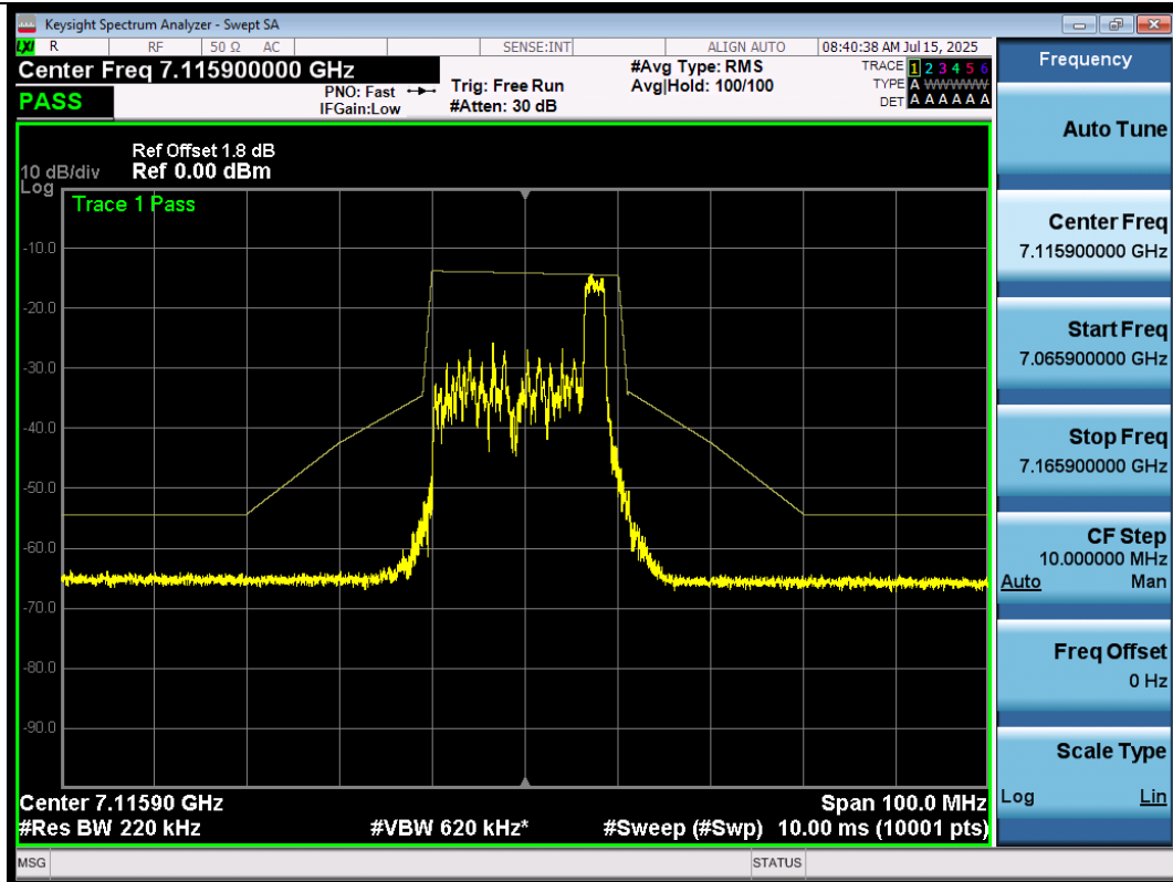
NTNV-11AX20SISO-Ant1-7115-52Tone-RU40-PASS
