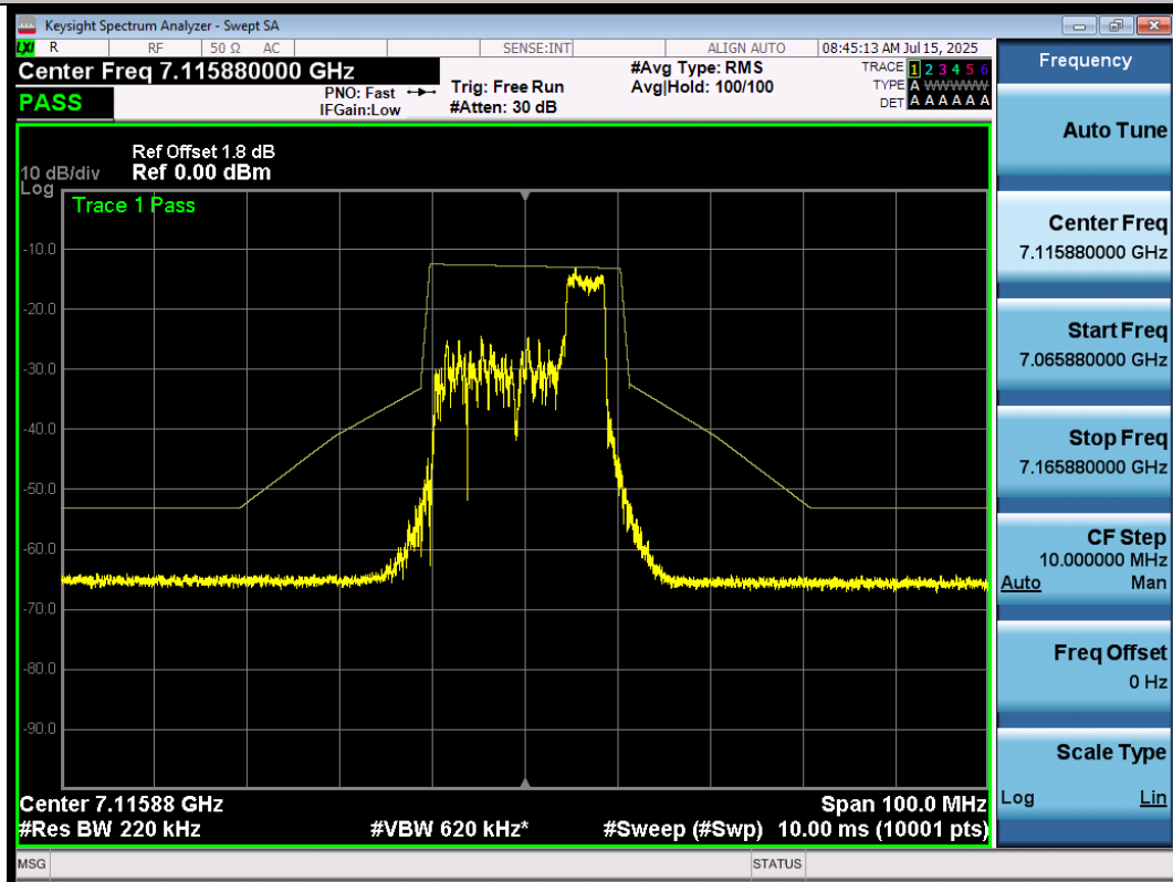
NTNV-11AX20SISO-Ant1-7115-106Tone-RU54-PASS
