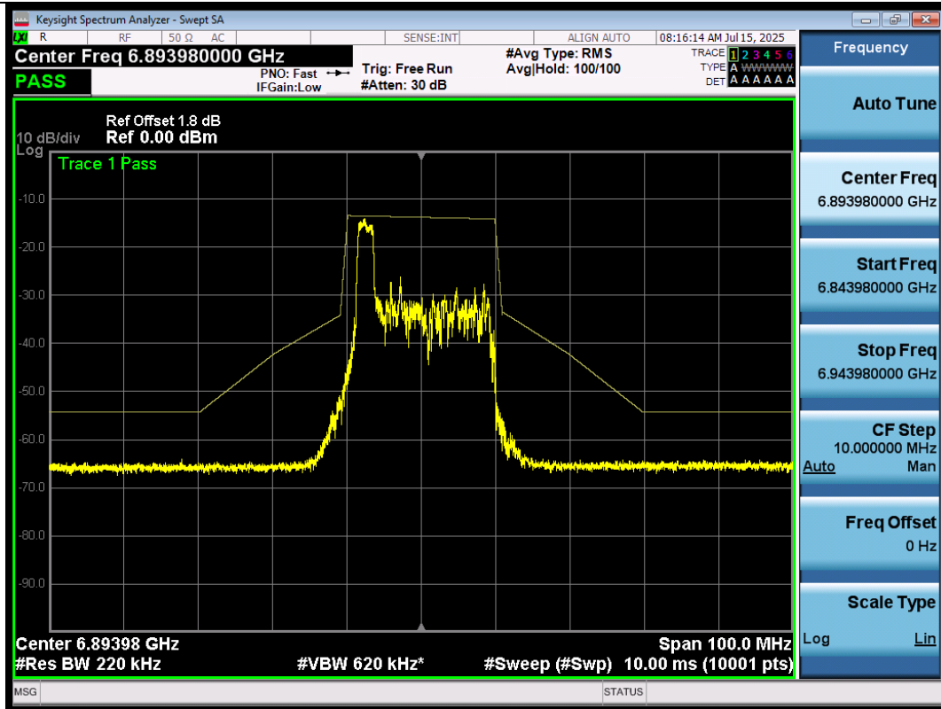
NTNV-11AX20SISO-Ant1-6895-52Tone-RU37-PASS
