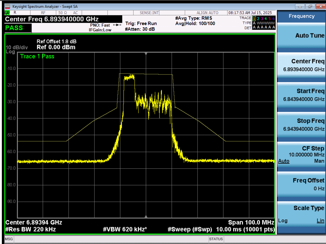
NTNV-11AX20SISO-Ant1-6895-106Tone-RU53-PASS
