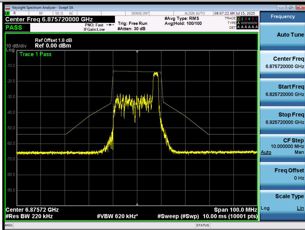
NTNV-11AX20SISO-Ant1-6875-52Tone-RU40-PASS
