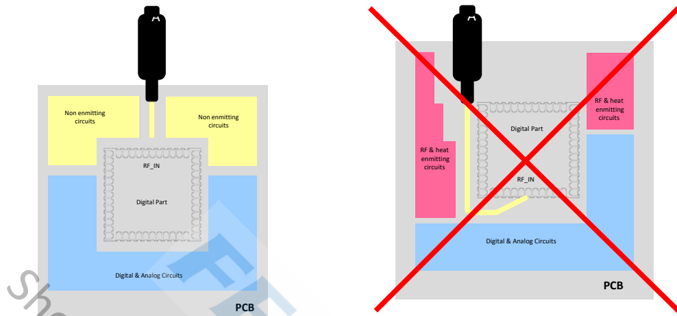
Figure 10: Placement the Module on a System Board
