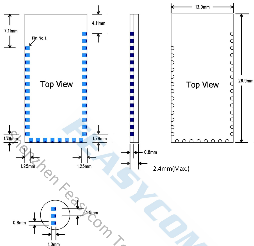
Figure 7: FSC-BT986 footprint
